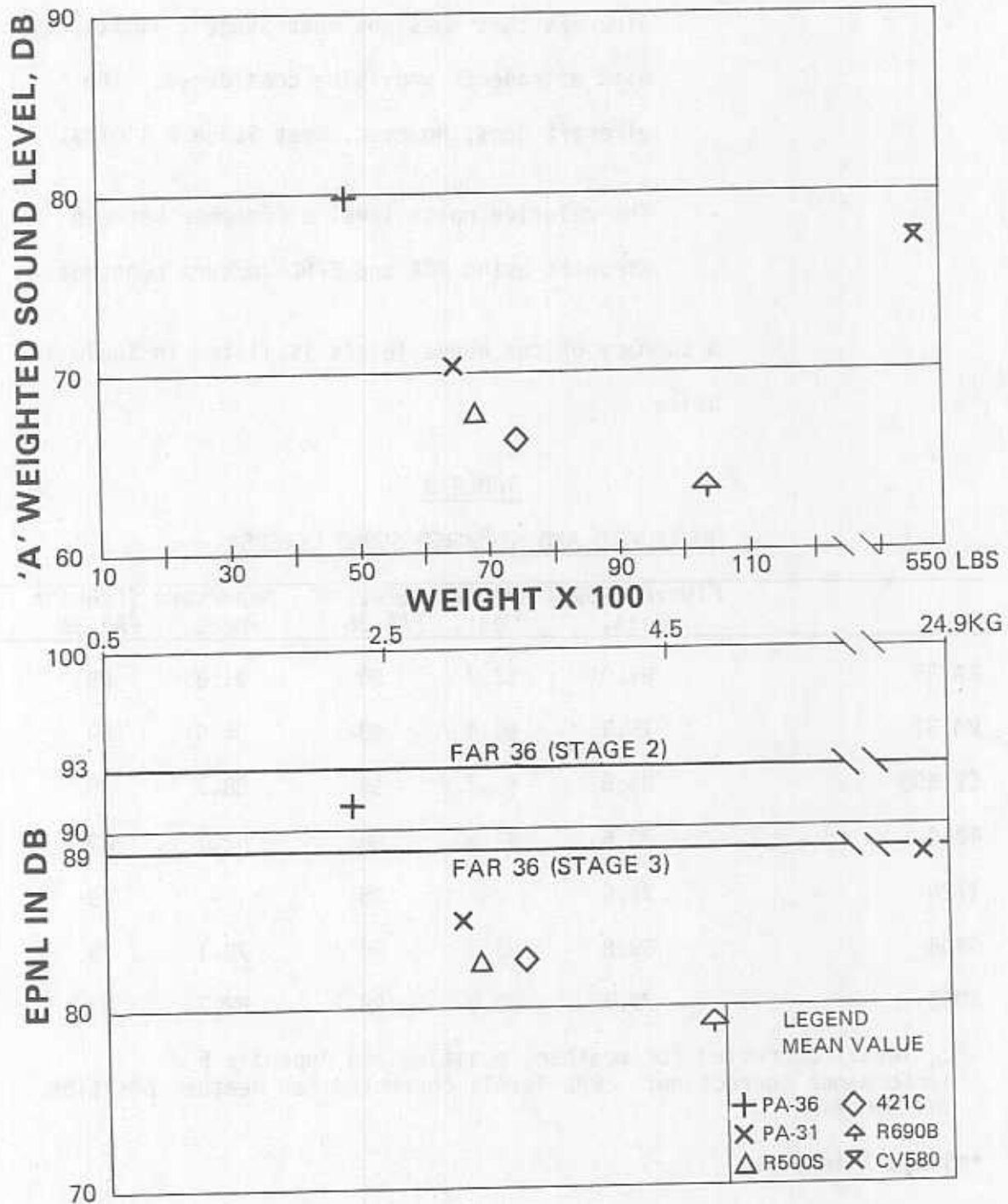
DEPARTURE DATA VS NOISE STANDARDS FIGURE 20
