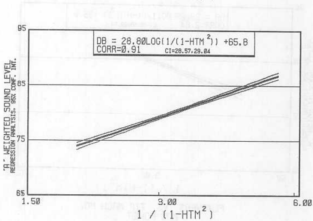
FLYOVERS VS TIP MACH NO. TEST DATA + REF. 6 FIGURE 28
