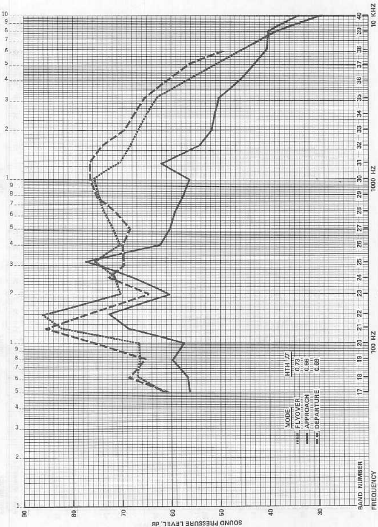
CONVAIR 580 — 1/3 OCTAVE SPECTRA — FIGURE 36
