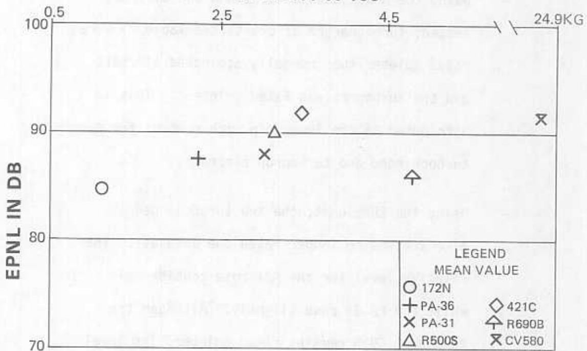
FLYOVER LEVELS VS WEIGHT FIGURE 18
