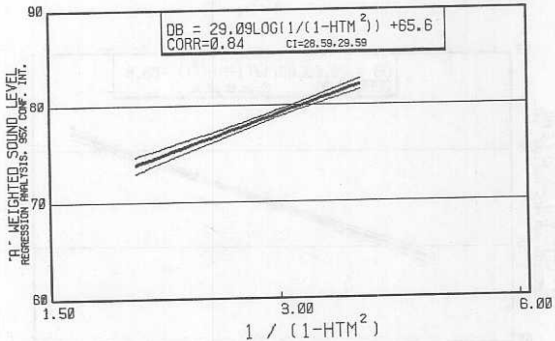
FLYOVERS VS TIP MACH NO. MAX POWER FIGURE 27
