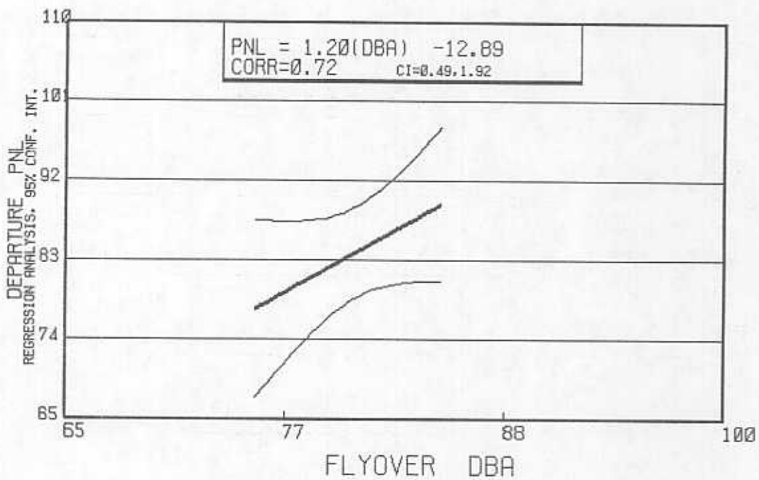
DEPARTURE DATA VS FLYOVER DATA FIGURE 40
