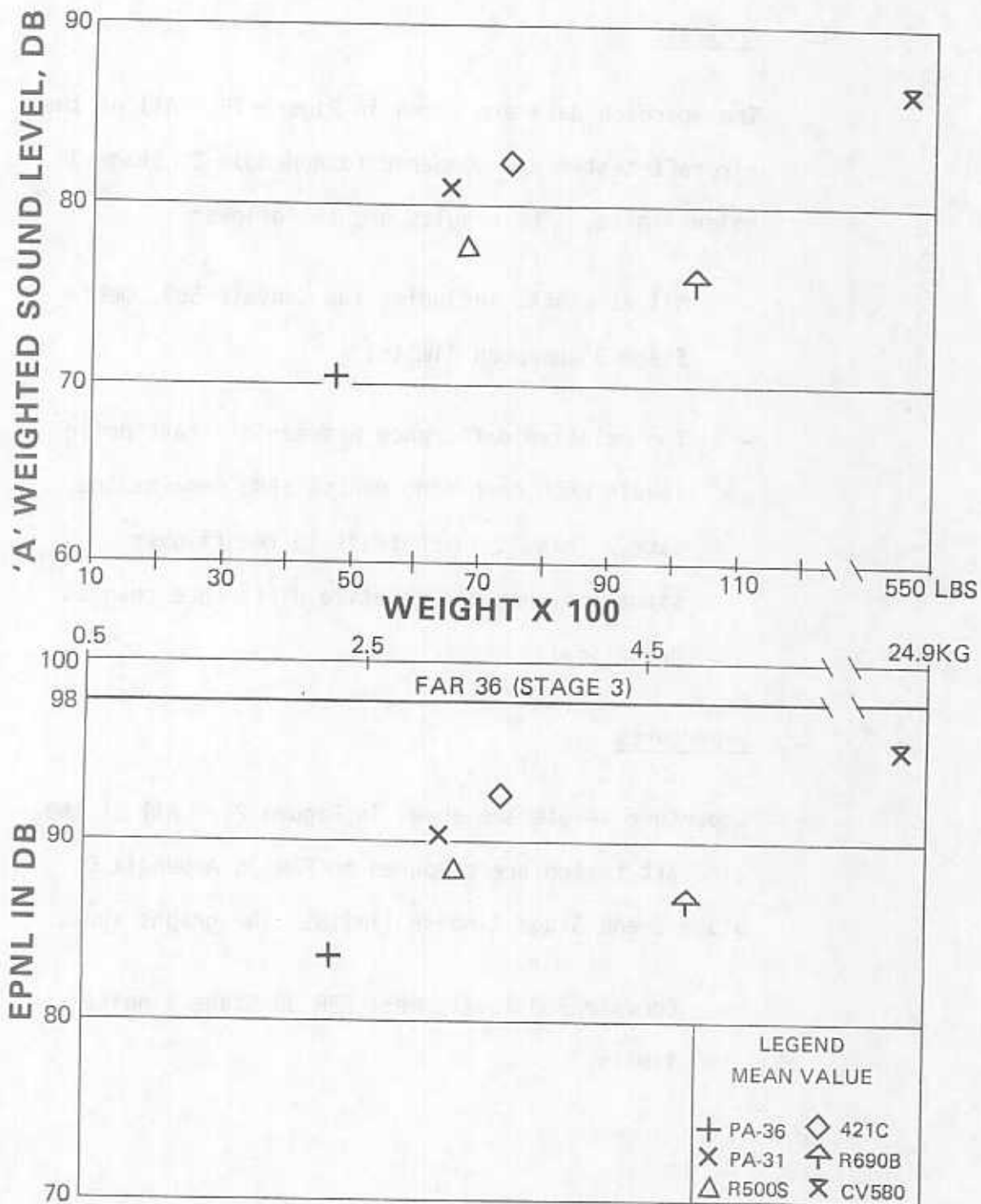
ARRIVAL DATA VS NOISE STANDARDS FIGURE 19
