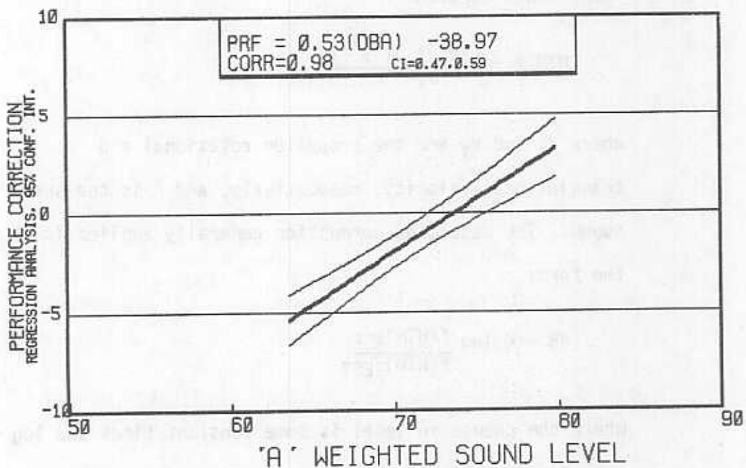
DEPARTURE VS PRF FIGURE 24
