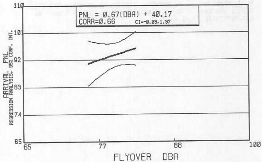
ARRIVAL DATA VS FLYOVER DATA FIGURE 41
