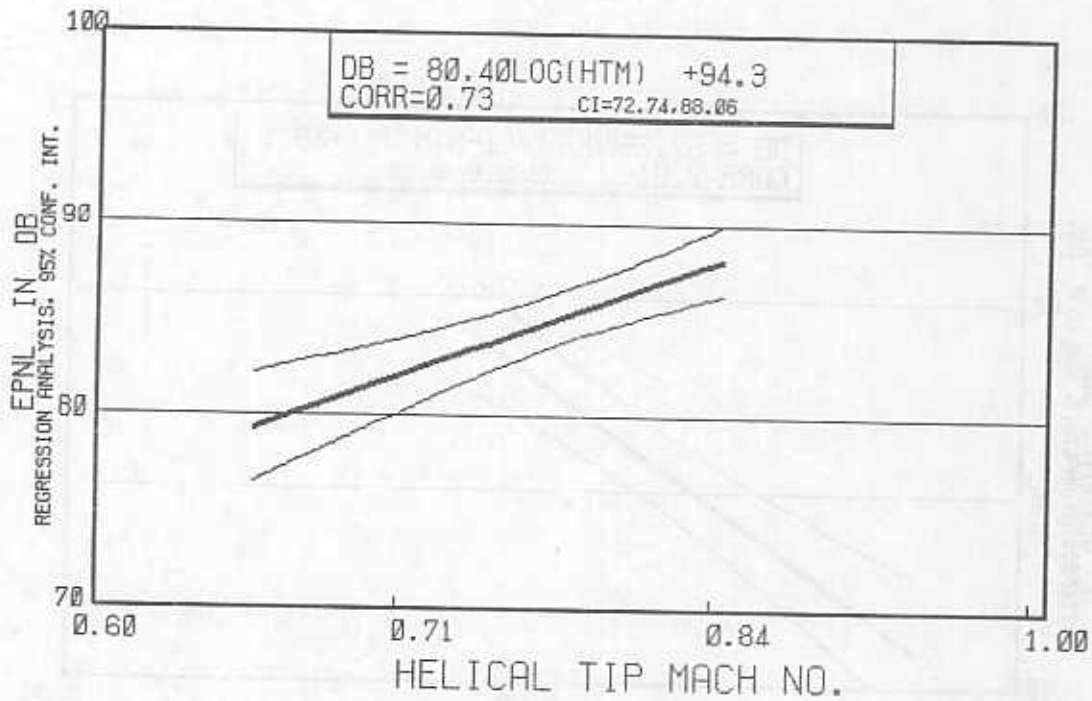
DEPARTURE VS TIP MACH NO.
