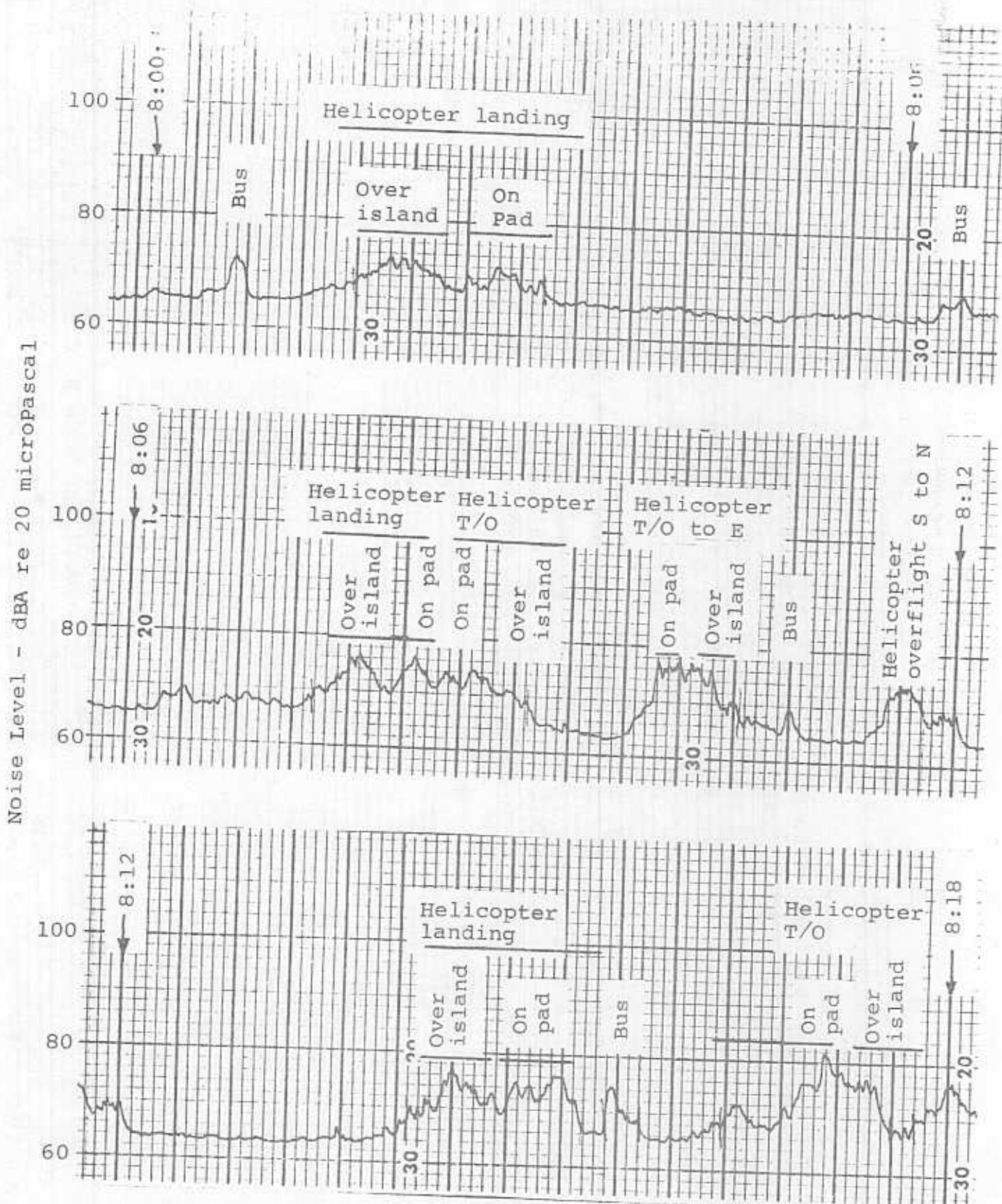
Figure 11. Noise-Level Time History Data - Site No. 7 Roosevelt Island - South of Apartment Complex East 60th Street Heliport Operations New York, New York - November 17, 1982
