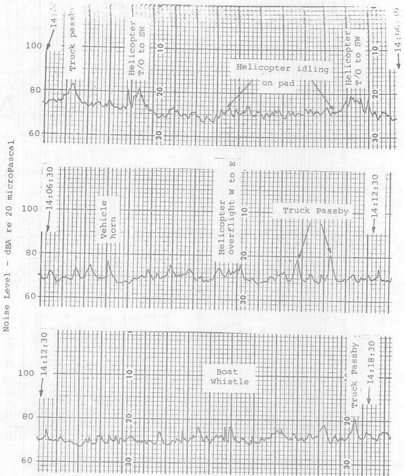
Figure 9. Noise-Level Time History Data - Site No. 2 Vicinity of Downtown Heliport South Street, New York, N.Y. - November 16, 1982
