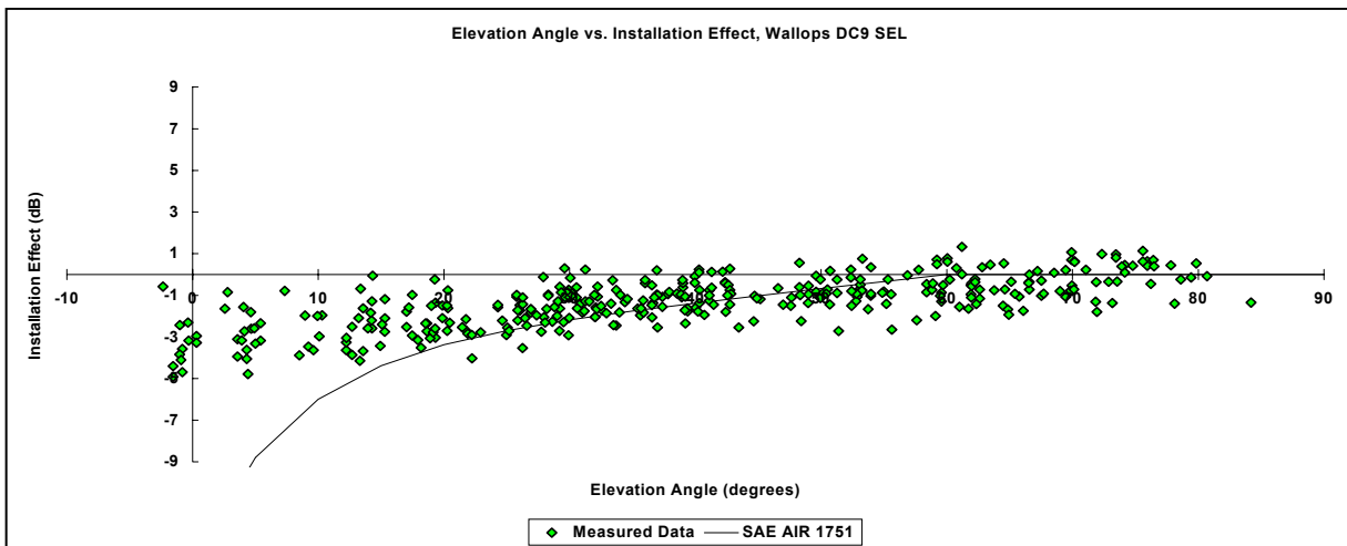
Figure 4: DC-9 Engine Installation effects, all passes
