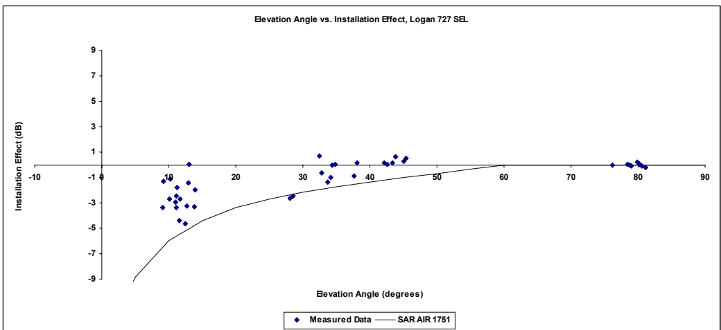
Figure 5: 727 Engine Installation effects, measured at Logan Airport
