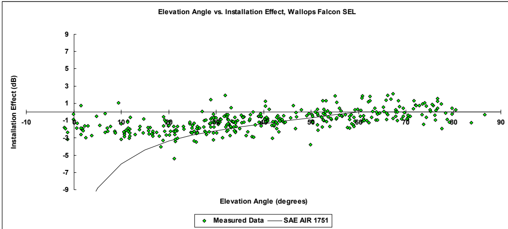
Figure 5: Dassault Falcon 2000 Engine Installation effects, all passes
