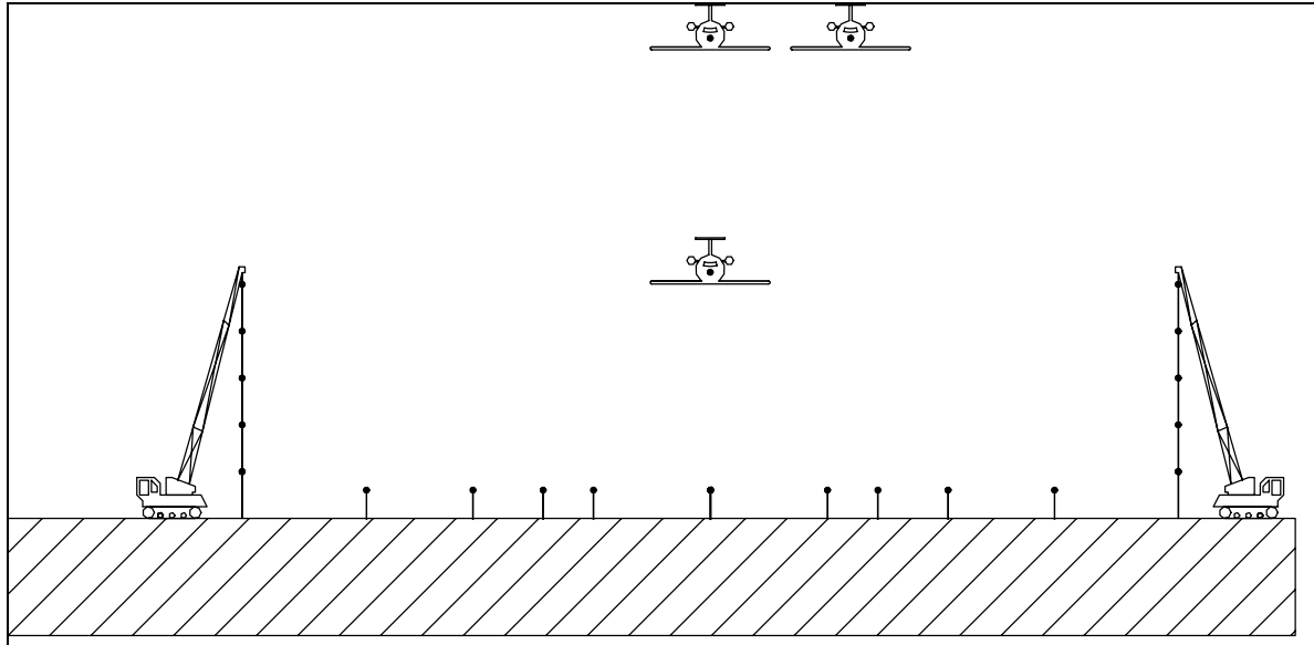
Figure 2: Microphone and airplane position schematic
