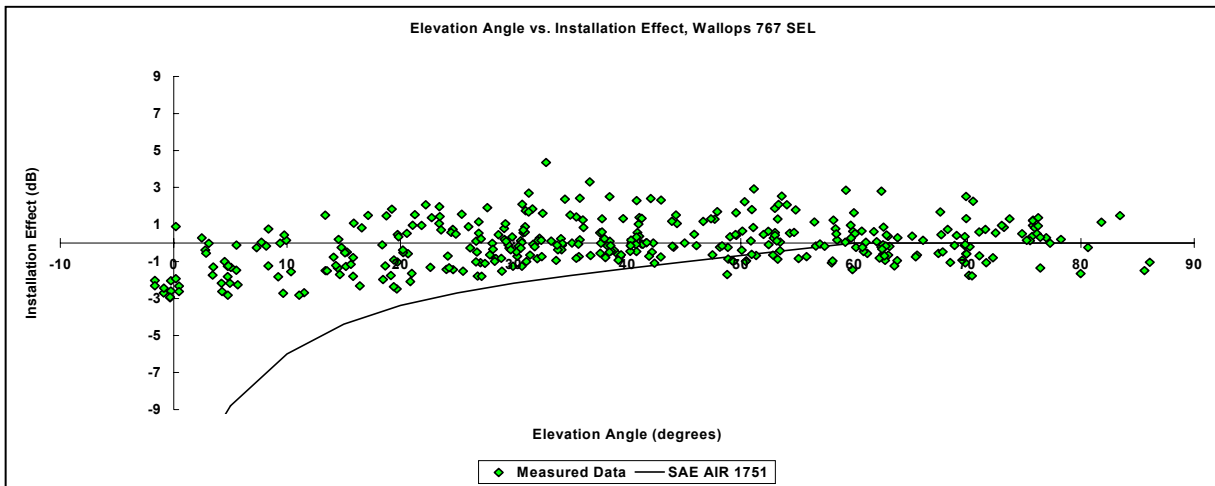
Figure 3: 767 Engine Installation effects, all passes
