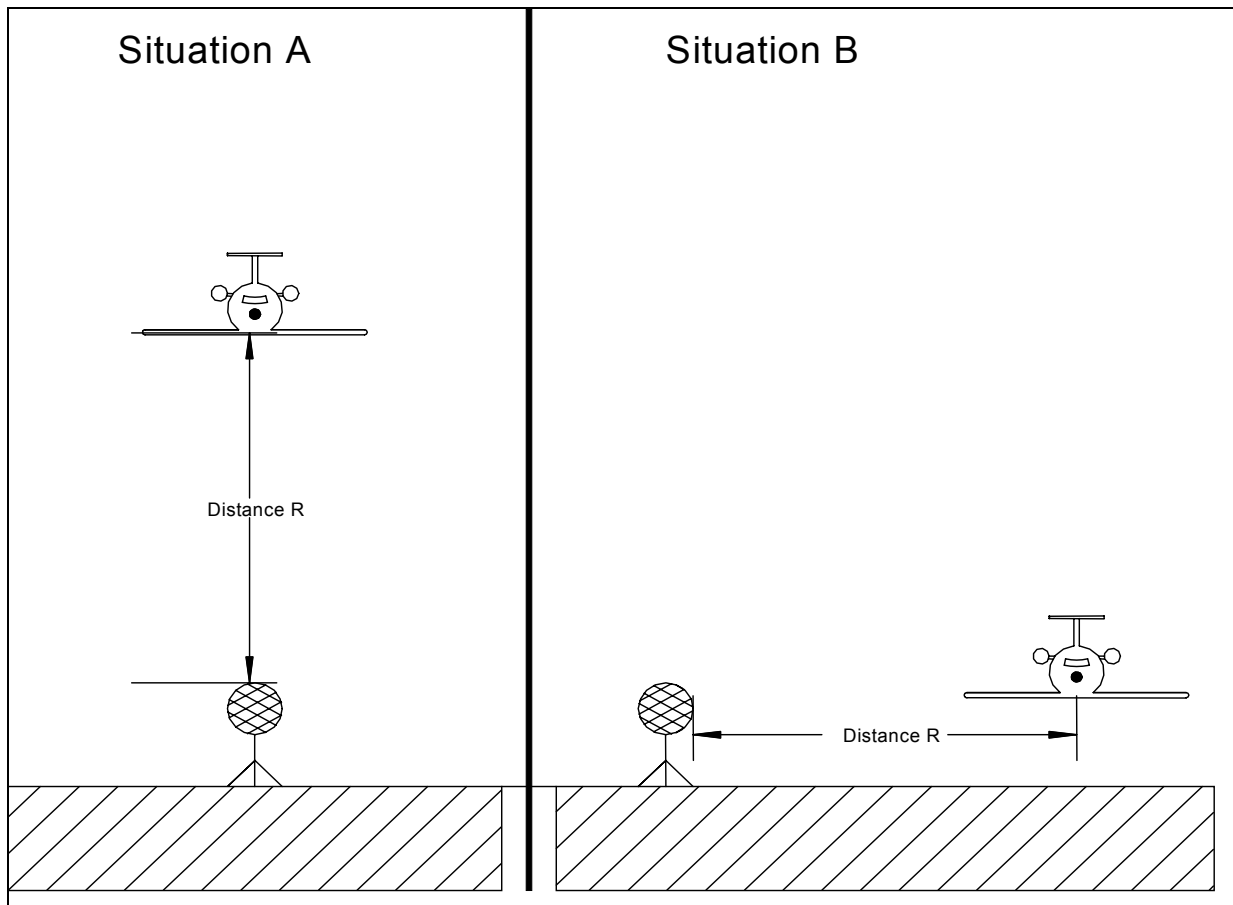
Figure 1: Lateral Attenuation schematic
