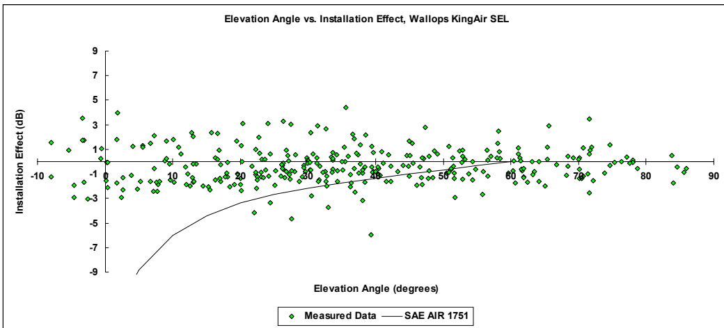
Figure 6: Beech KingAir Engine Installation effects, all passes
