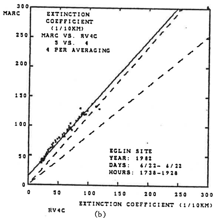
FIGURE 6-17. MARCONI MET-1 RESPONSE FOR TWO FOG-HAZE EVENTS.
