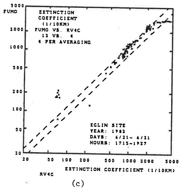
FIGURE 6-33. FUMOSSENS III RESPONSE FOR TWO STEAM FOG EVENTS.
