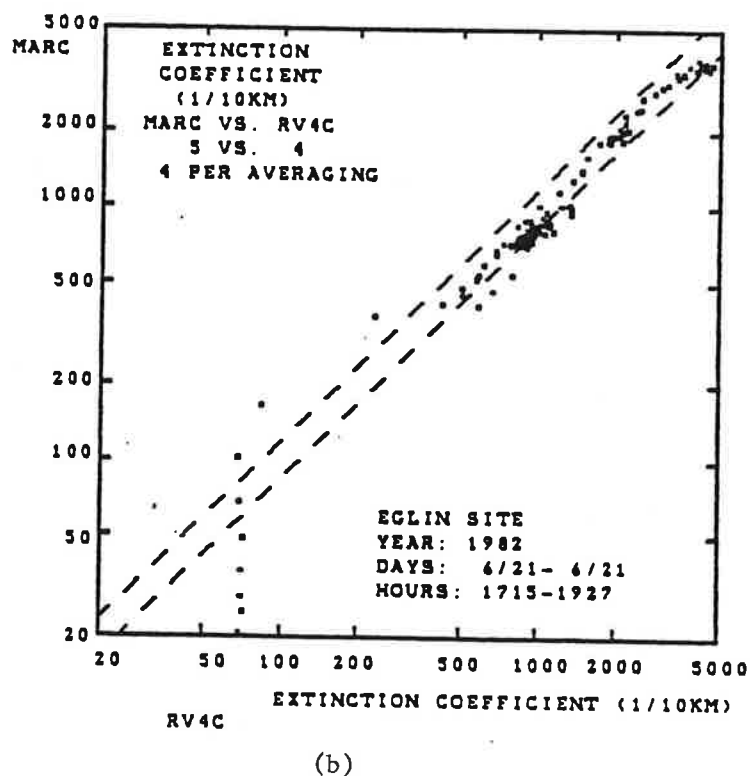
FIGURE 6-14. MARCONI RESPONSE TO TWO STEAM FOG EVENTS.
