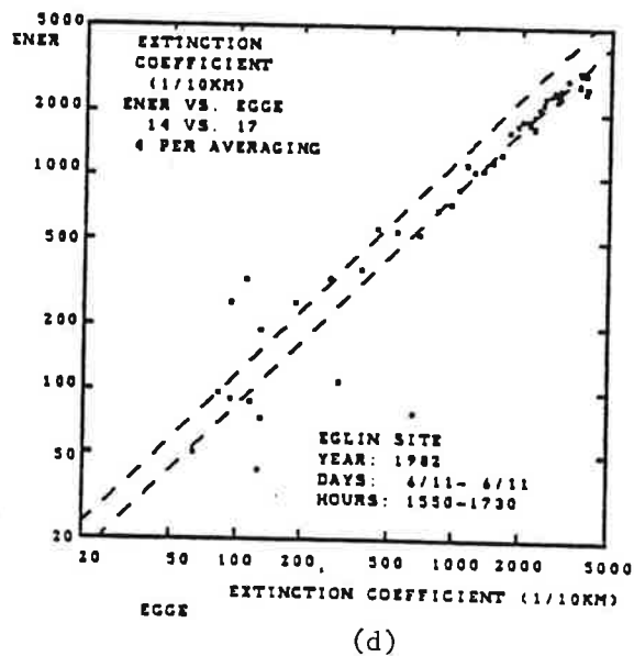
FIGURE 6-39. ENERTECH RESPONSE TO FOG EVENTS ON 6/11/82; (a), (b) STEAM, (c), (d) COOLING.
