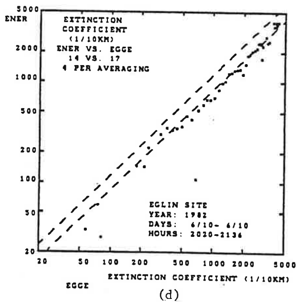
FIGURE 6-38. ENERTEC EV-1000 RESPONSE FOR TWO FOG EVENTS ON 6/10/82; (a), (b) STEAM: (c), (d) COOLING.
