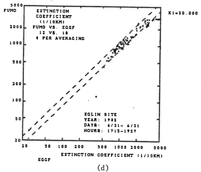
FIGURE 6-33. FUMOSSENS III RESPONSE FOR TWO STEAM FOG EVENTS.
