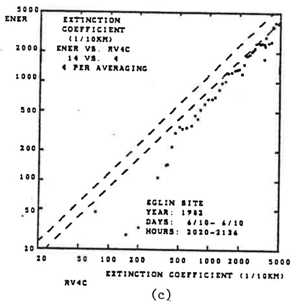
FIGURE 6-38. ENERTEC EV-1000 RESPONSE FOR TWO FOG EVENTS ON 6/10/82; (a), (b) STEAM: (c), (d) COOLING.
