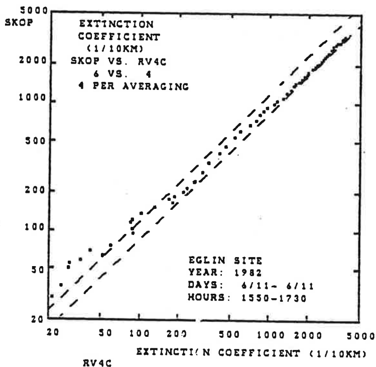
FIGURE 6-12. SKOPOGRAPH RESPONSE FOR TWO FOG EVENTS ON 6/11/82: (a) STEAM, (b) COOLING.
