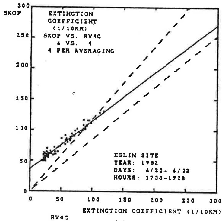
FIGURE 6-10. SKOPOGRAPH RESPONSE FOR TWO STEAM FOG EVENTS.
