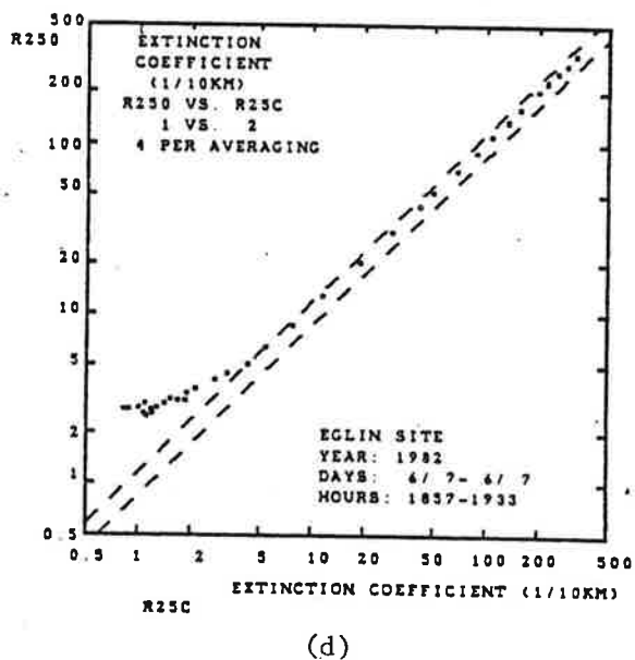
FIGURE 6-8. COMPARISONS OF THE RVR 500 TO THE RVR CALIBRATOR ON A 250-FOOT BASELINE
