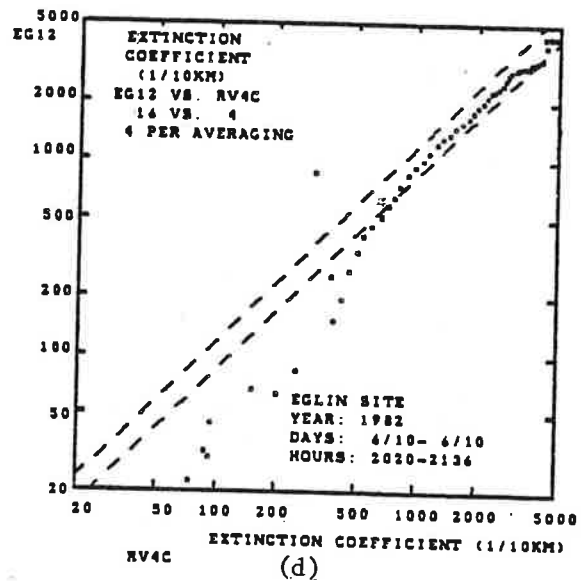
FIGURE 5-18. HOMOGENEITY OF THE COOLING FOG EVENT ON 6/10/82.
