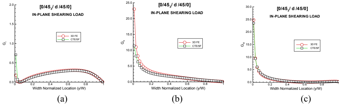
FIGURE 11. COMPARISON OF ERRs FOR A [0/45_3/d/45/0] PLATE SUBJECTED TO AN IN-PLANE SHEARING LOAD (a) MODE I, (b) MODE II, AND (c) MODE III
