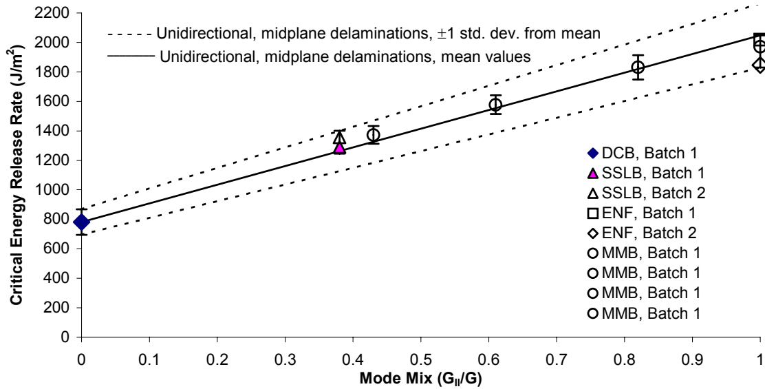
FIGURE 35. SINGULAR FIELD-BASED BASIC FRACTURE TOUGHNESS CURVE FOR T800H/3900-2 GRAPHITE/EPOXY
