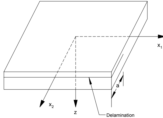
FIGURE 5. LAMINATE CONTAINING A FREE-EDGE DELAMINATION
