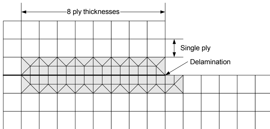
FIGURE 30. TYPICAL FE MODEL OF A UENF SPECIMEN
