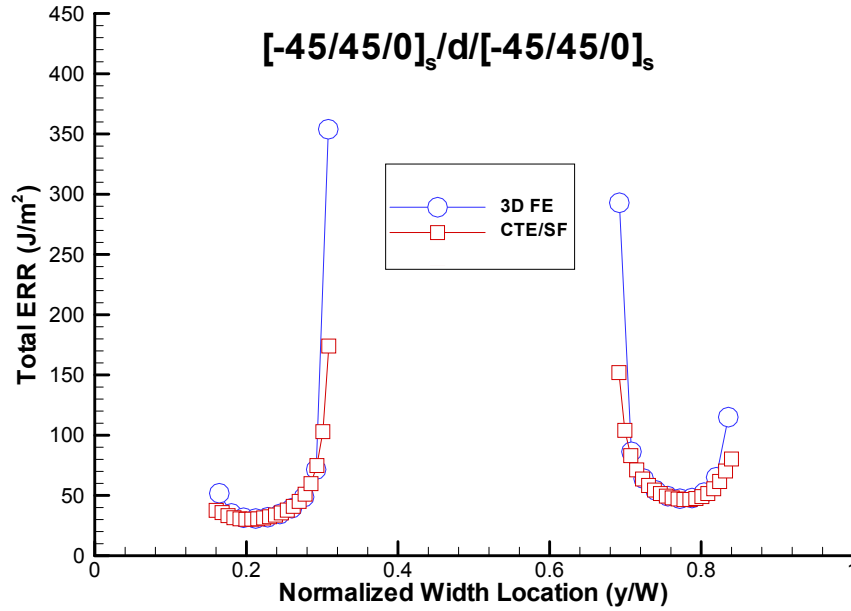
FIGURE 23. COMPARISON OF TOTAL ERRs FOR A [\mp 45/0]_s/d/[\mp 45/0]_s HAT-STIFFENED PANEL
