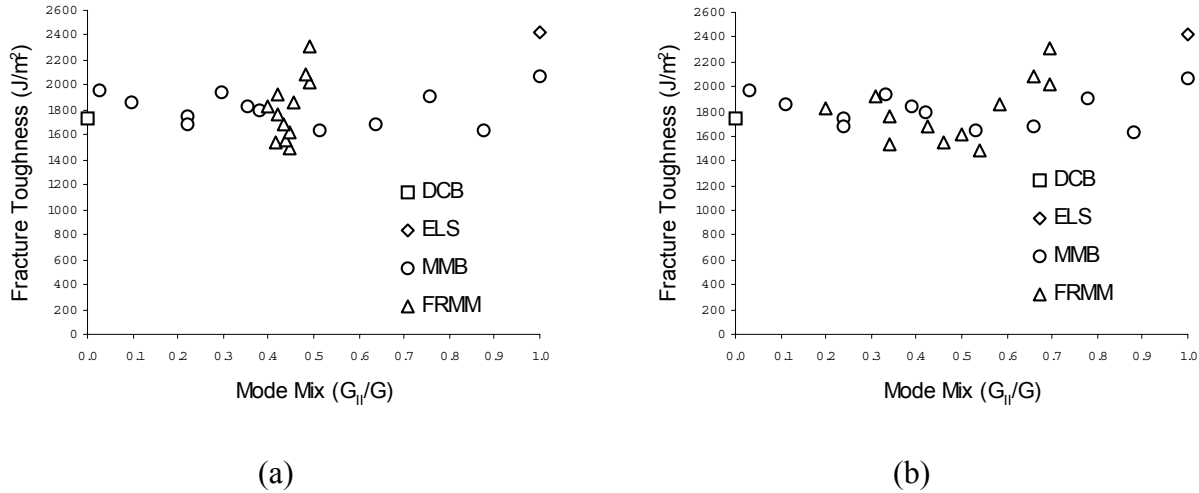
FIGURE 41. ASSESSMENT OF PREDICTIVE CAPABILITY FOR AS4/PEEK (a) SF APPROACH AND (b) NSF APPROACH
