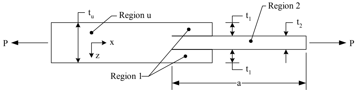
FIGURE 29. THE CRACKED DOUBLE LAP-SHEAR TEST
