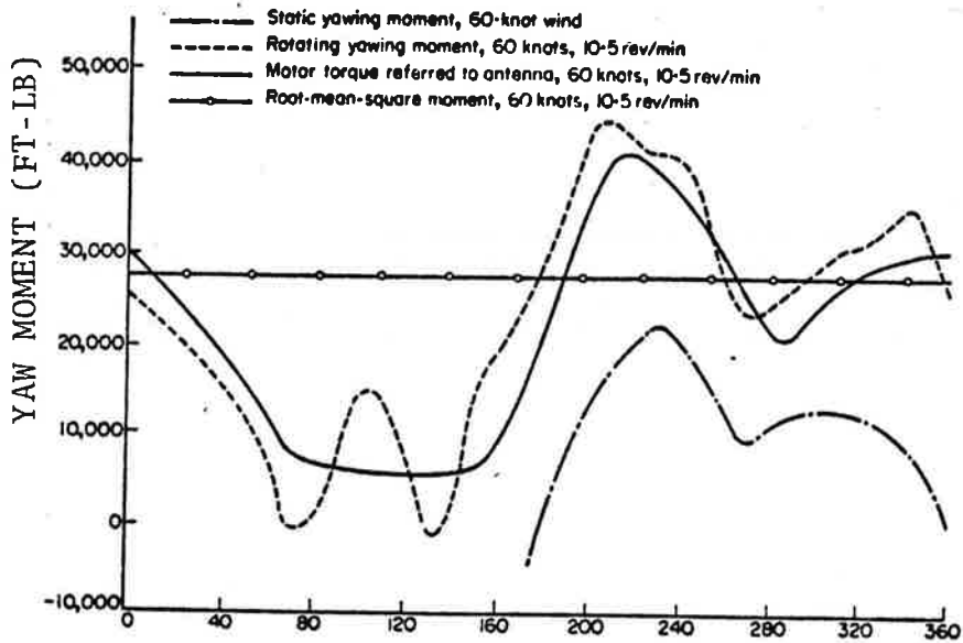
FIGURE 13B. MEASURED YAW MOMENT VS WIND ANGLE
