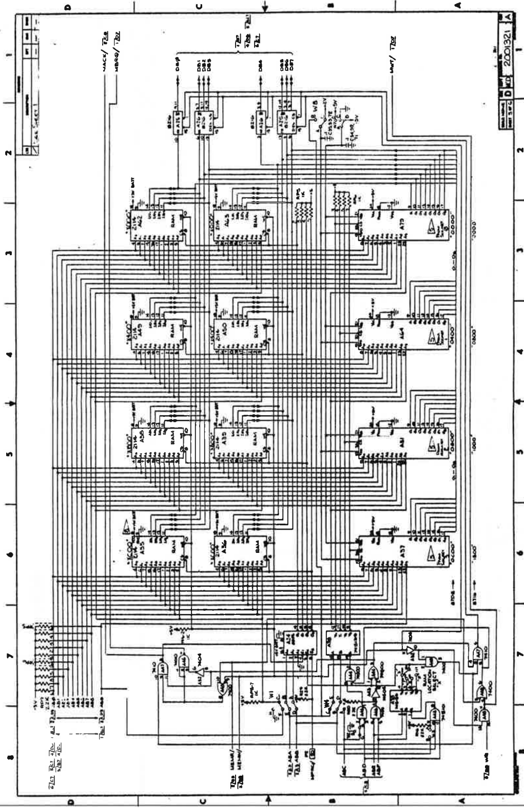
Figure A-2. SBC 80/20-4 Schematic Diagram (Sheet 3 of 6)
