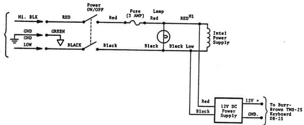
FIGURE 28. POWER WIRING DIAGRAM
