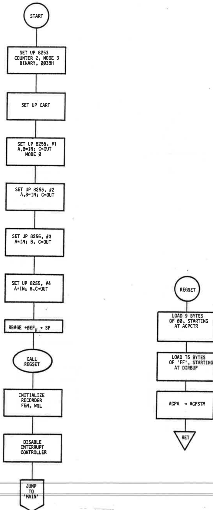
FIGURE 41. INITIALIZATION ROUTINE
