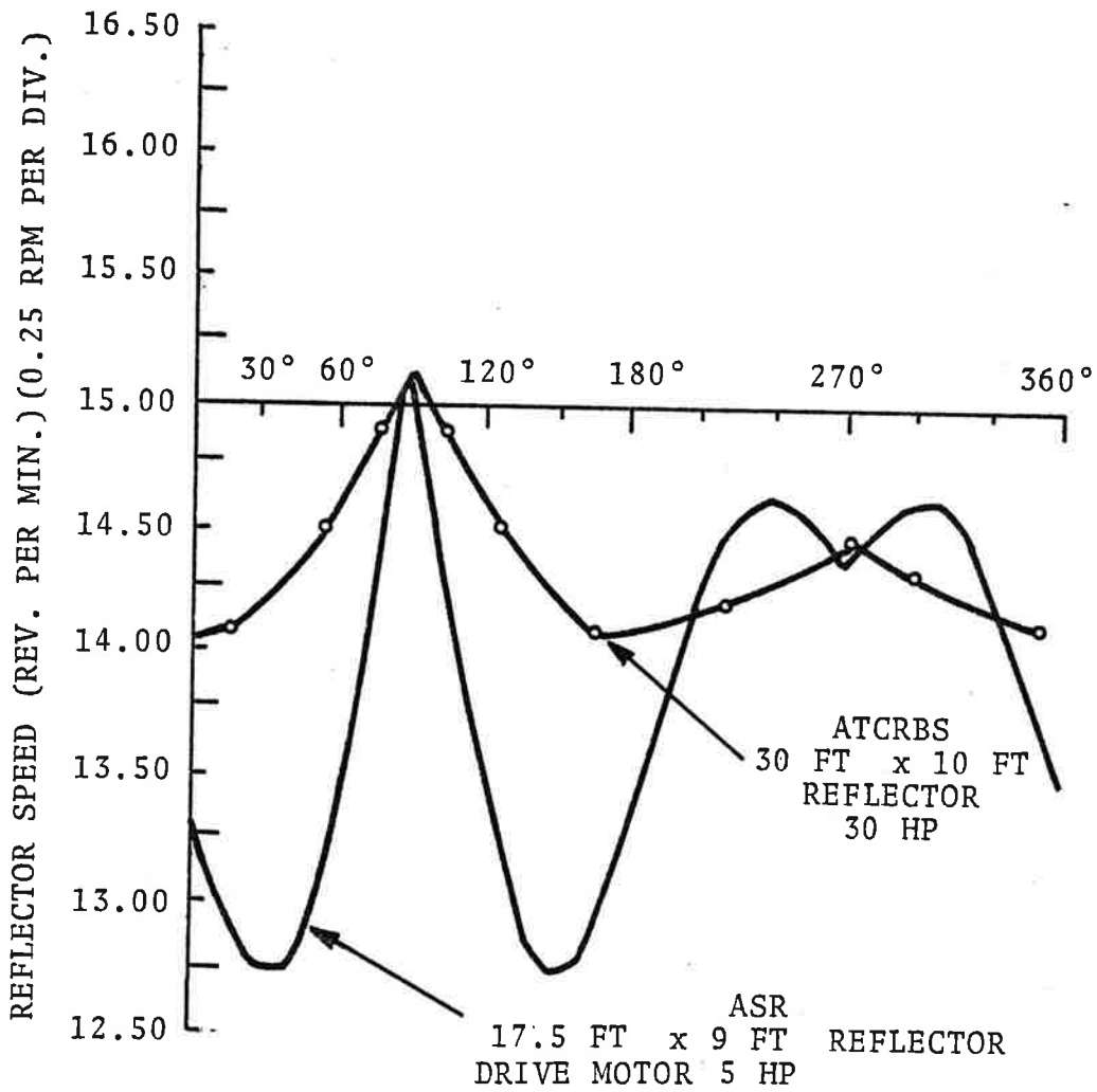
FIGURE 2. REFLECTOR SPEED VS WIND ANGLE OF INCIDENCE
