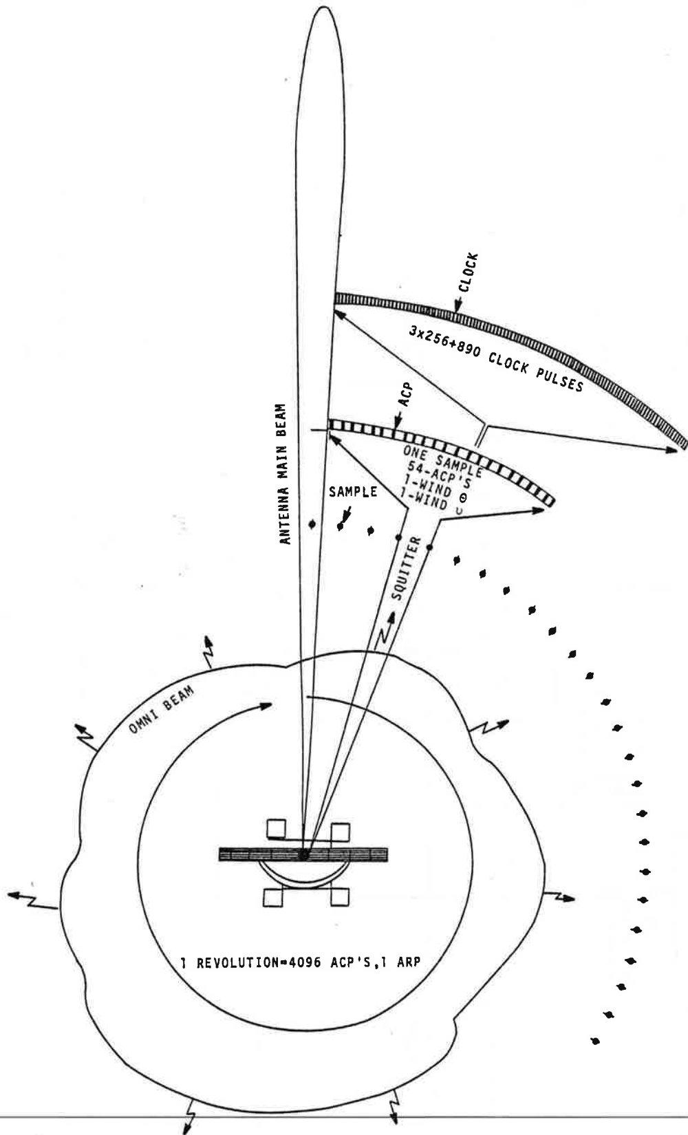
FIGURE 20. MEASUREMENT TECHNIQUE
