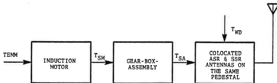
FIGURE 9. ASR-8/SSR ANTENNA SYSTEM SIMULATION MODEL
