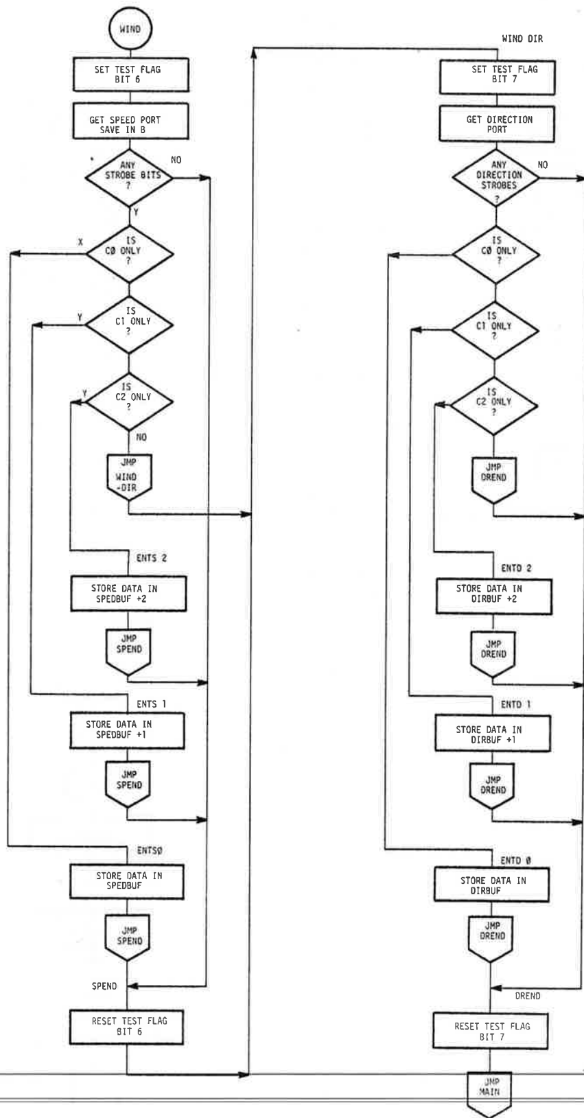
FIGURE 44. WIND SPEED AND WIND DIRECTION ROUTINES
