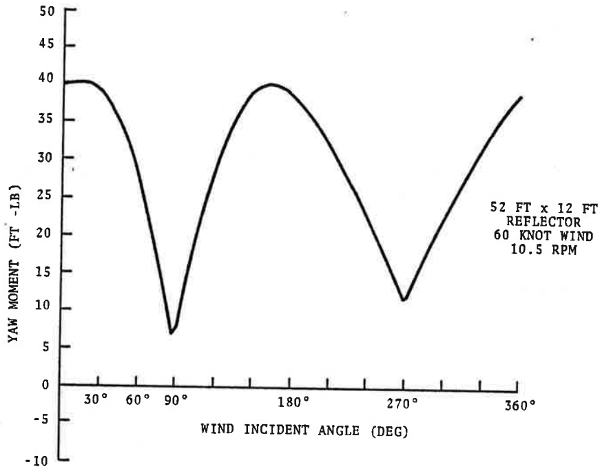
FIGURE 13A CALCULATED YAW MOMENT VS WIND ANGLE
