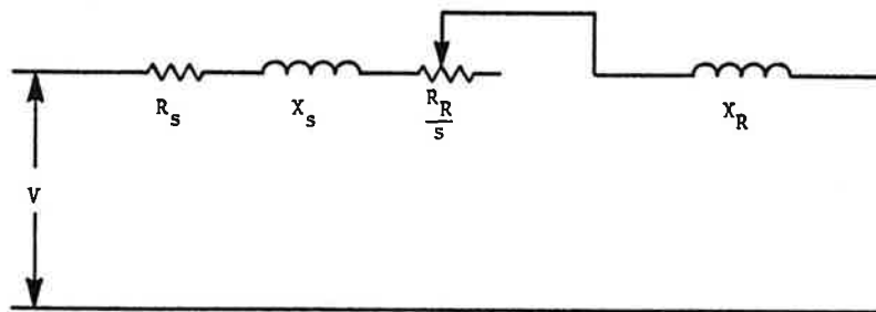
FIGURE 10. EQUIVALENT CIRCUIT OF THE INDUCTION MOTOR
