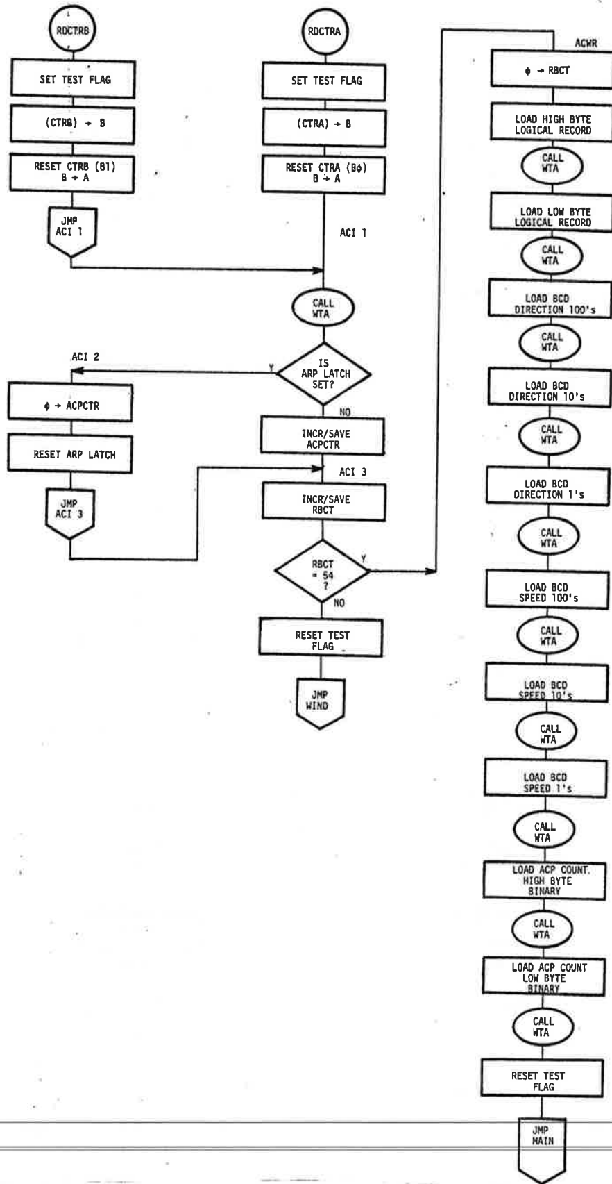
FIGURE 43. ACP COUNT LOADING AND RECORD COUNT ROUTINES
