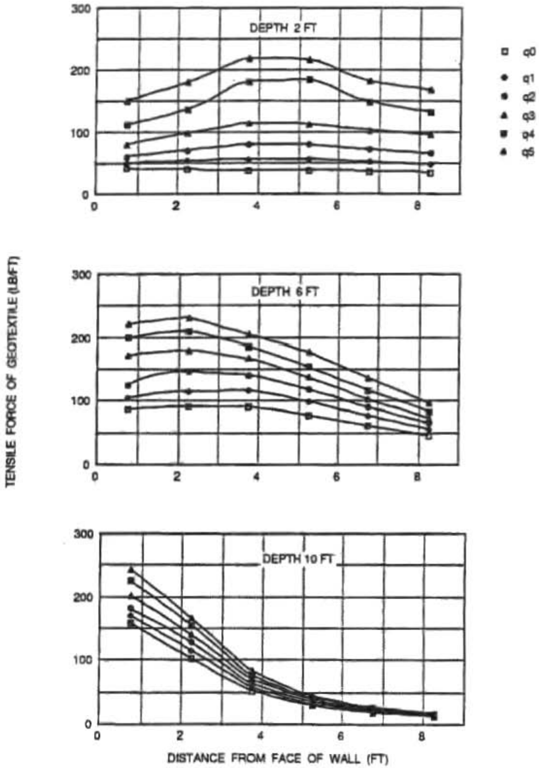
Figure 3.16 Effect of Surcharge on Geosynthetic Tensile Force- -Rigid Foundation
