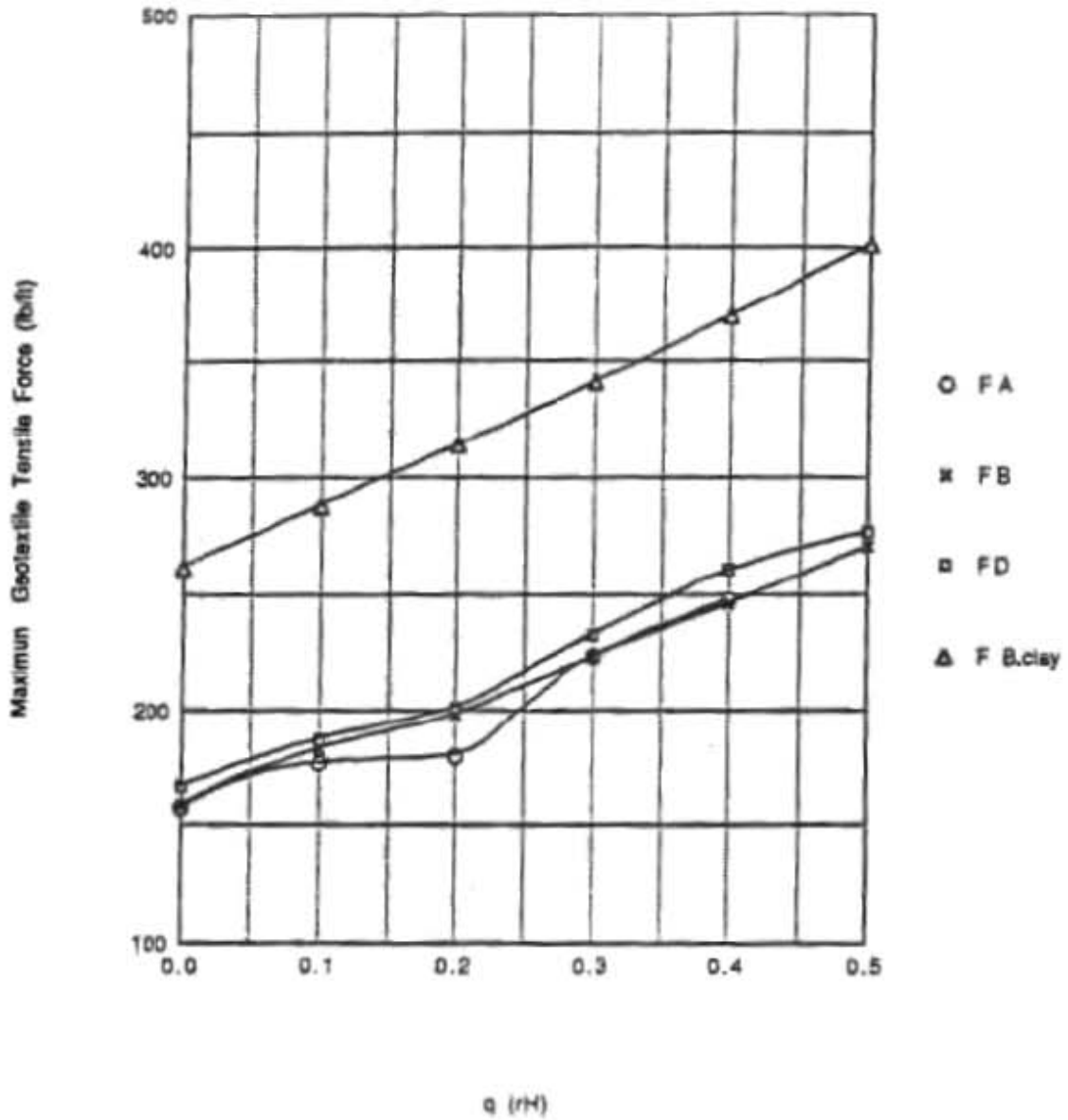
Figure 3.41 Effect of Foundation on Maximum Tensile Force in the Geosynthetic under Different Surcharge Pressures
