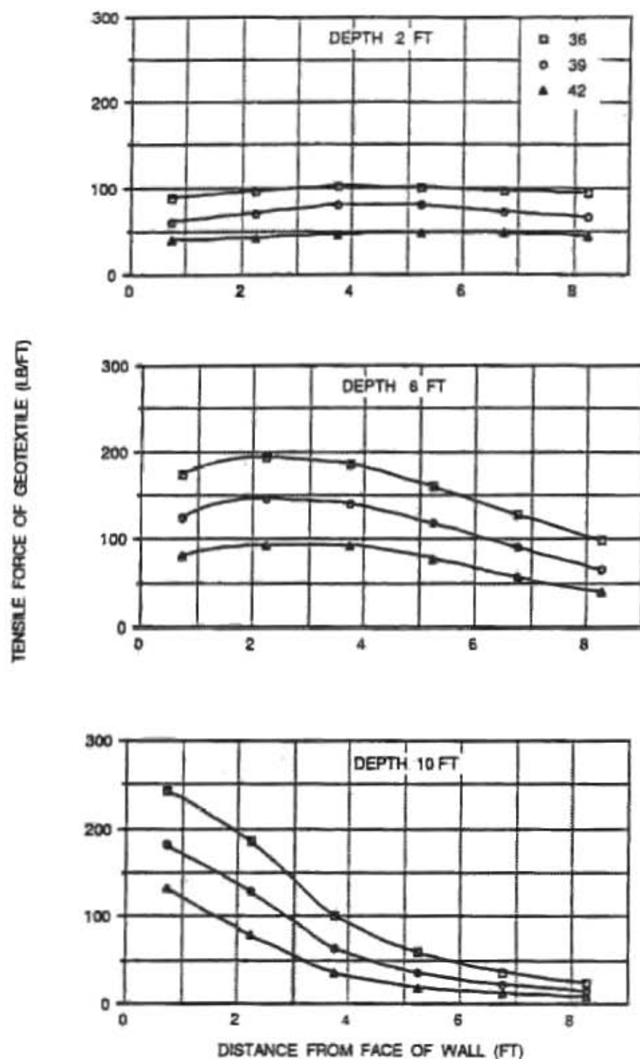
Figure 3.4 Effect of Backfill Stiffness/Strength on Geosynthetic Tensile Force--Rigid Foundation
