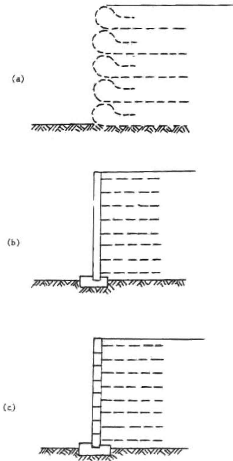
Figure 3.44 Types of Wall Facings: (a) Geosynthetic Wrap Around Facing; (b) Continuous Concrete Panels; (c) Articulated Concrete Panels
