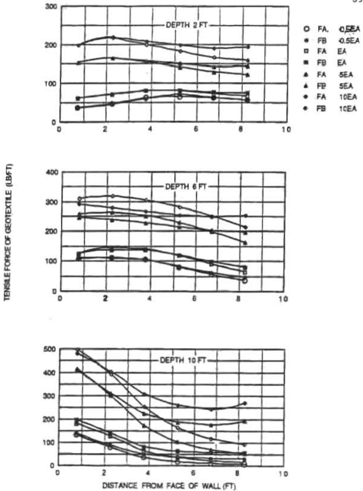
Figure 3.28 Effect of Geosynthetic Stiffness on Geosynthetic Tensile Force
