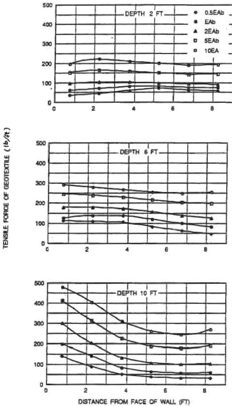
Figure 3.19 Effect of Geosynthetic Stiffness on Geosynthetic Tensile Force--Flexible Foundation
