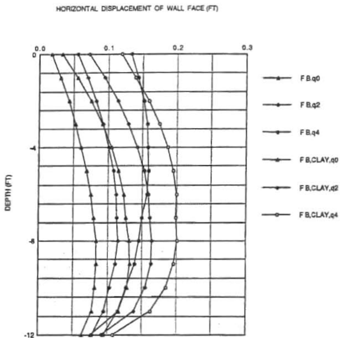
Figure 3.43 Wall Movement of the Control Wall A, with granular and Cohesive backfills, under Different Surcharge Pressures
