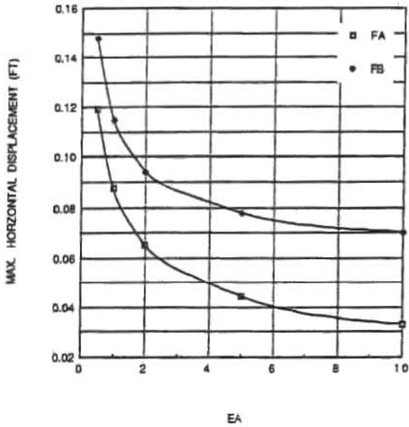
Figure 3.30 Effect of Geosynthetic Stiffness on Maximum Horizontal Wall Displacement
