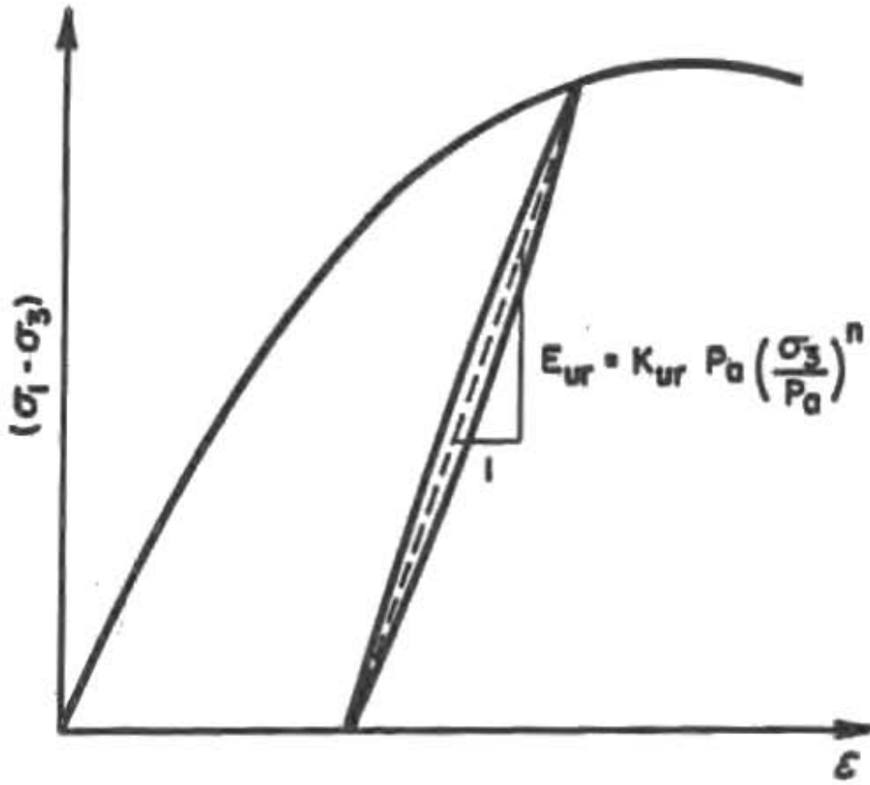
Figure 2.2 Unloading-Reloading Curve of Soil
