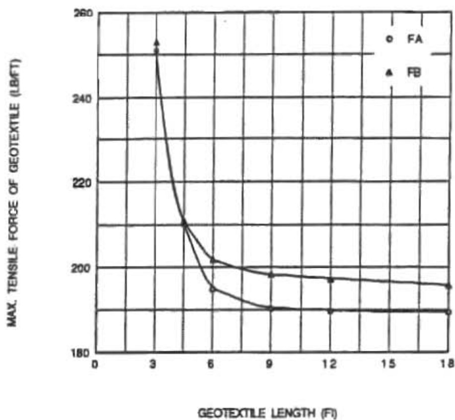
Figure 3.36 Effect of Geosynthetic Length on Maximum Tensile Force in the Geosynthetic
