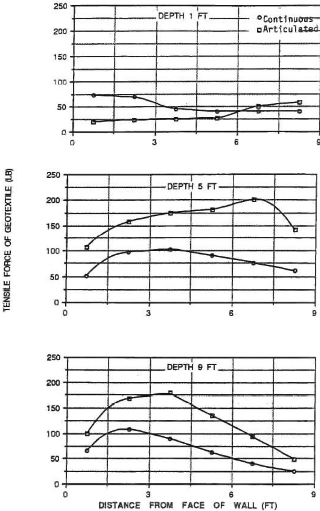
Figure 3.46 Effect of Facing on Geosynthetic Tensile Force
