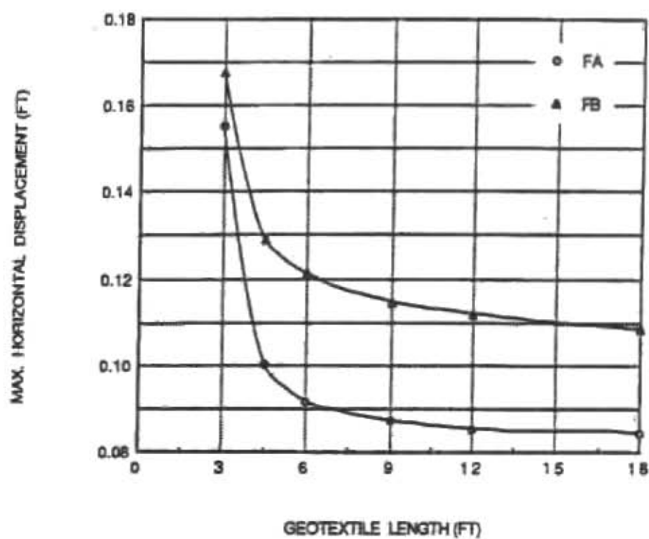
Figure 3.35 Effect of Geosynthetic Length on Maximum Horizontal Wall Displacement
