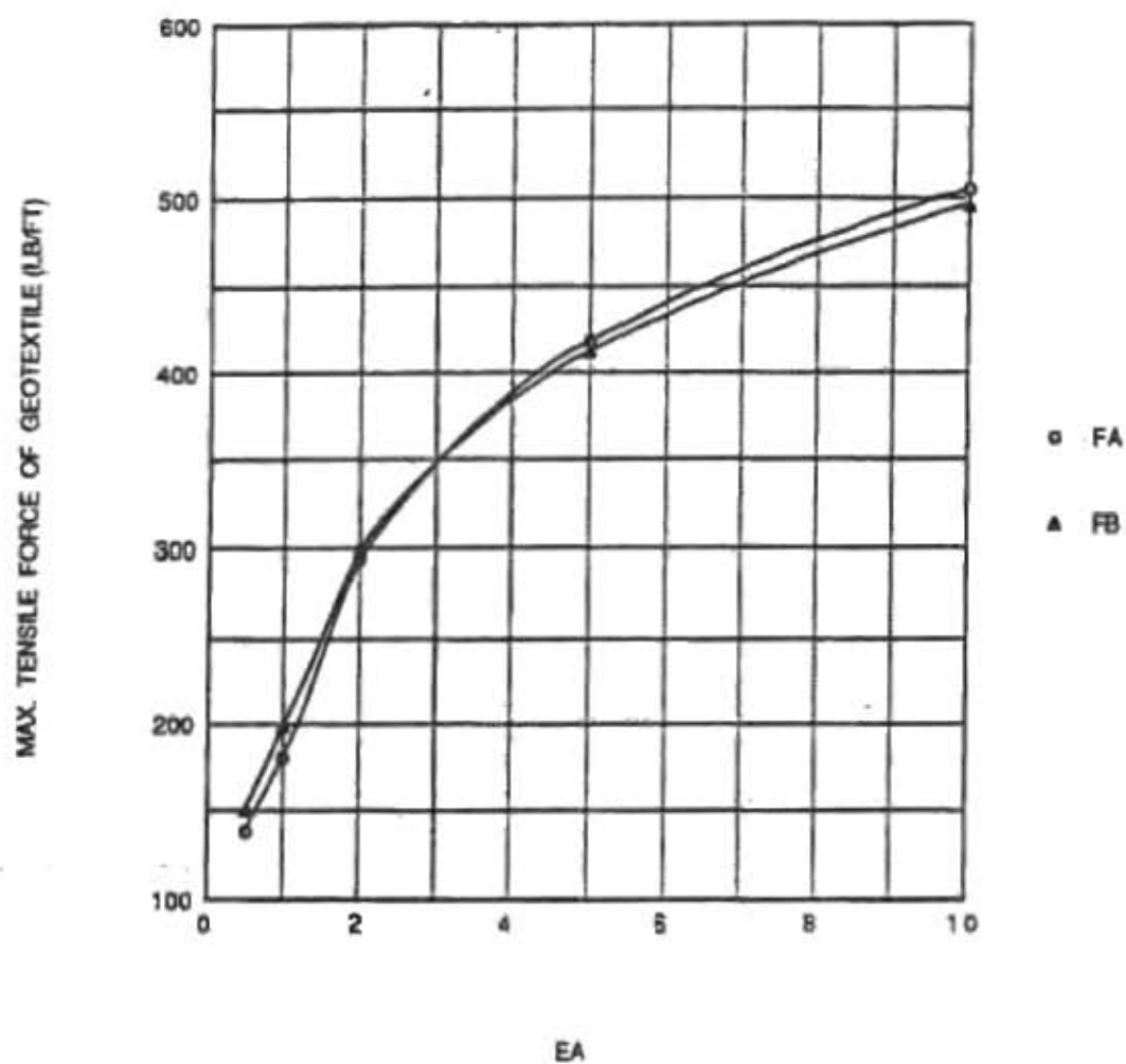
Figure 3.31 Effect of Geosynthetic Stiffness on Maximum Tensile Force in the Geosynthetic
