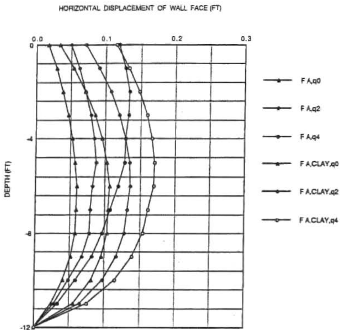
Figure 3.42 Wall Movement of the Control Wall A, with granular and Cohesive backfills, under Different Surcharge Pressures
