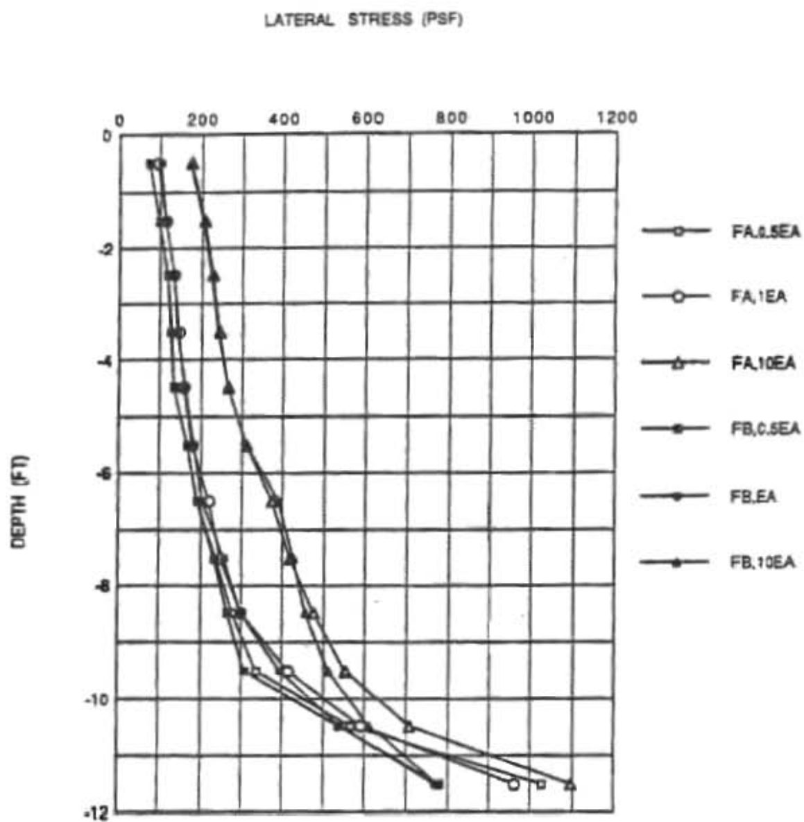
Figure 3.29 Effect of Geosynthetic Stiffness on Lateral Earth Pressure
