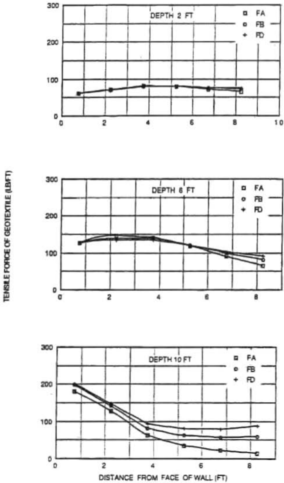
Figure 3.38 Effect of Foundation on Geosynthetic Tensile Force
