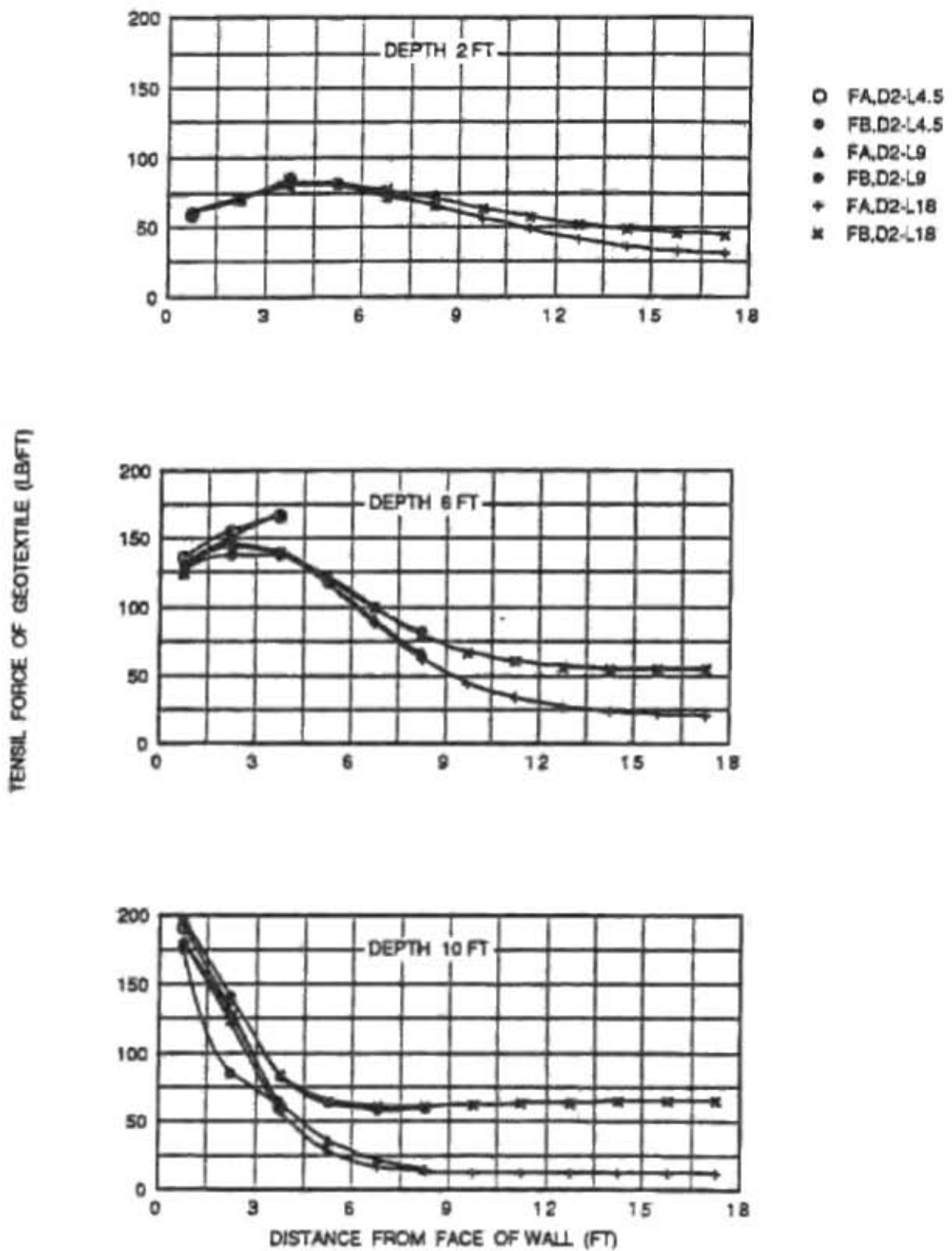
Figure 3.33 Effect of Geosynthetic Length on Geosynthetic Tensile Force
