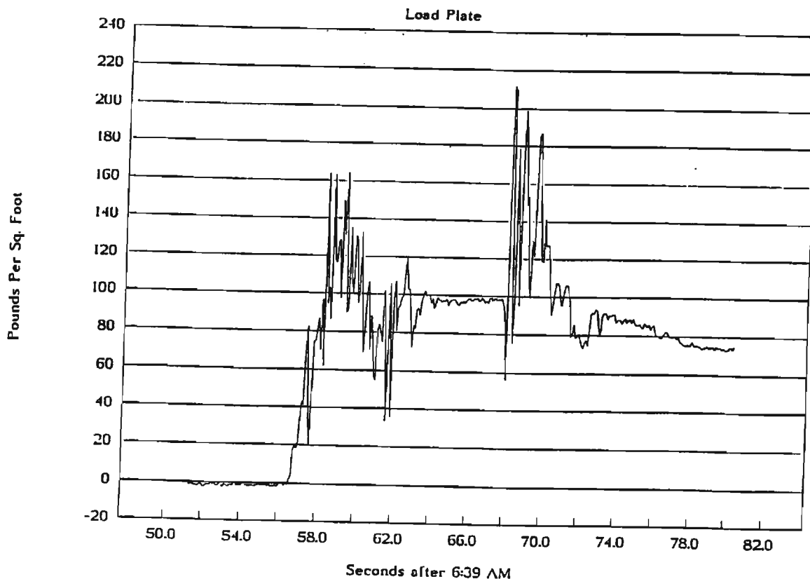
FIGURE 8. Time history of strains (equivalent static loads), on lateral-pressure paddle (top) and normal-pressure plate (bottom) from avalanche of 2/17/91. The paddle failed at 56.0 seconds, approximately 1.0 to 1.5 seconds before the main flowing mass began to produce significant loads on the normal-pressure plate. This is similar to the sequence shown in Figure 7, and also suggests the powder-blast component arrived at the shed prior to the main flowing core.
