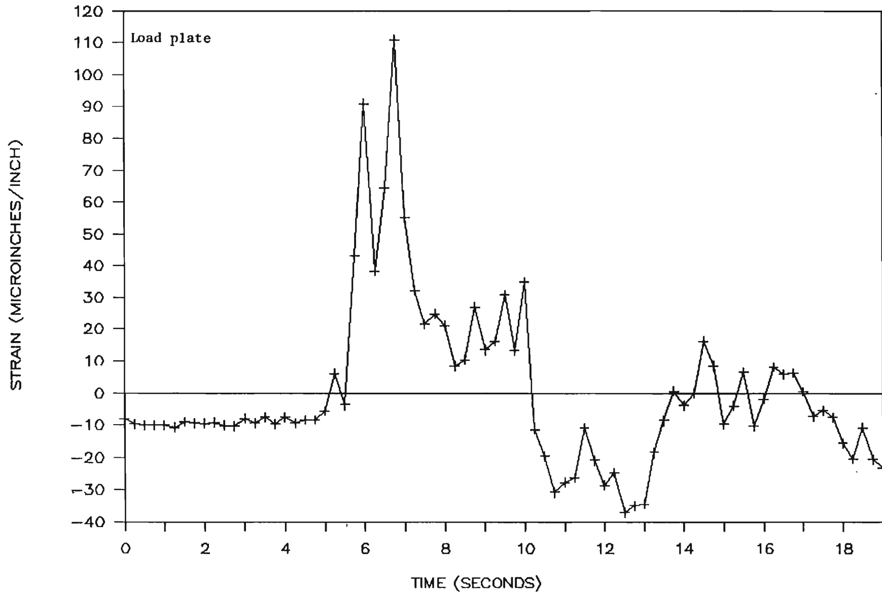
STRAIN VERSUS TIME FOR CHANNEL 31
