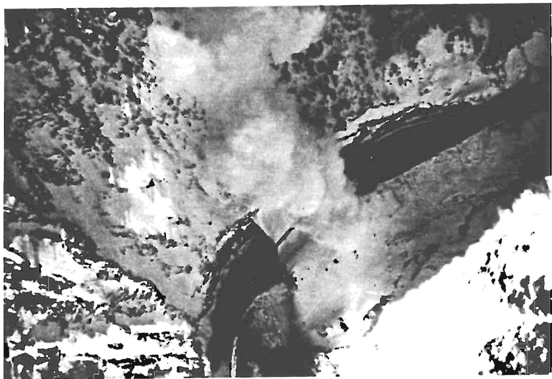
FIGURE 4. Small-volume, mixed motion, dry-snow/powder avalanche crossing shed in February, 1990. This avalanche was released by helicopter bombing by the Colorado Highway Department. Typical small events such as this one are confined by the shed, but powder blast and light debris extends beyond north and south portals and deposits a thin layer of debris on the highway. (Photograph by M. Friedman, Colorado Helitrax).
