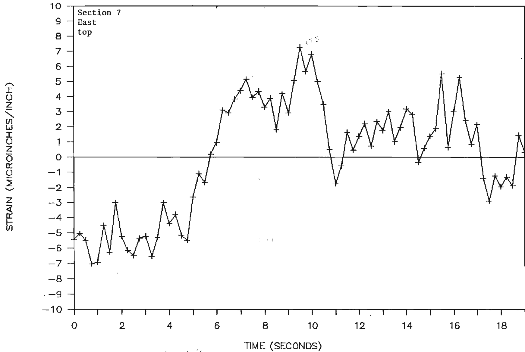
STRAIN VERSUS TIME FOR CHANNEL 24
