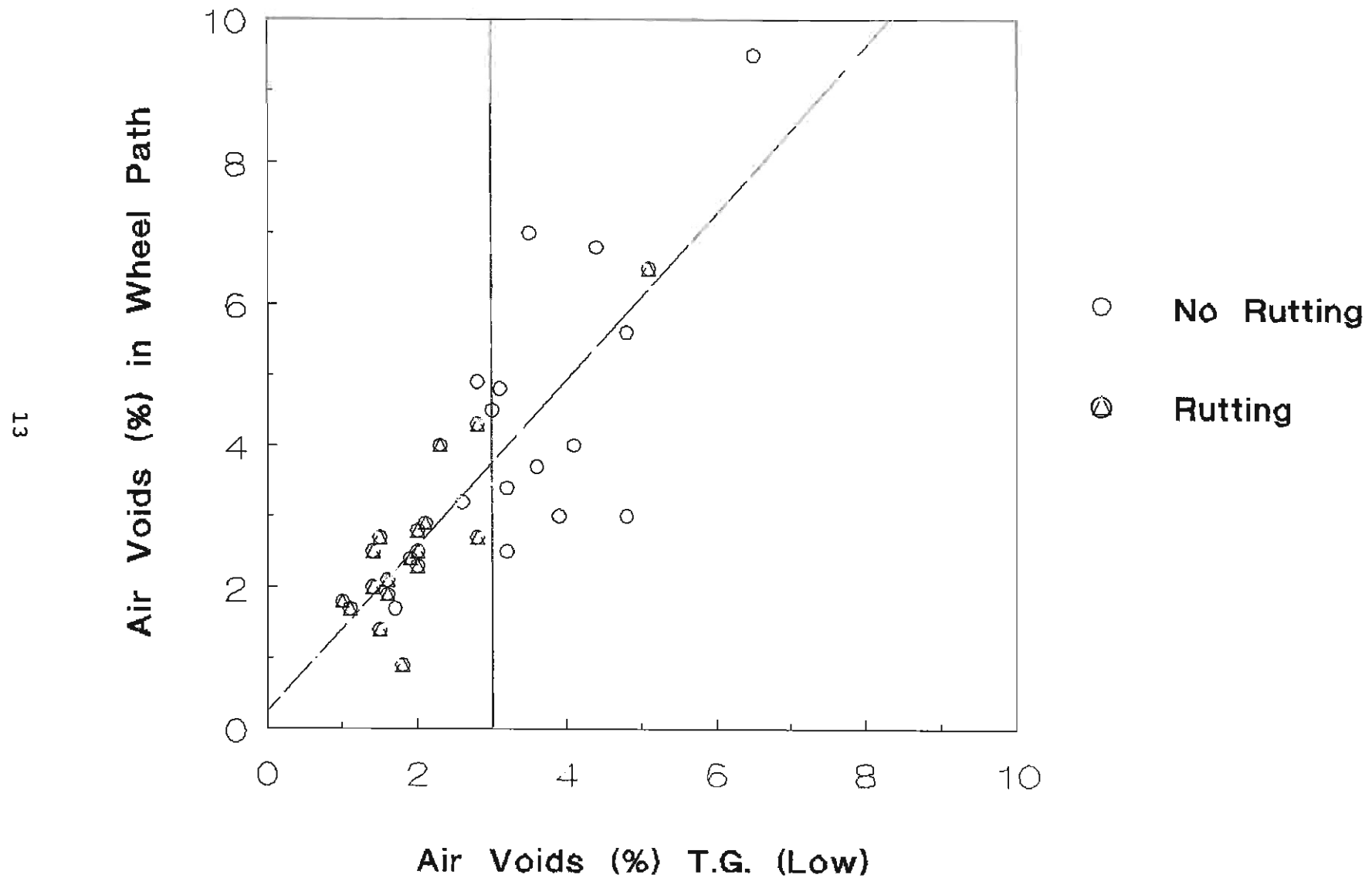
Figure 4 - Air Voids in Wheel Path Versus Air Voids T.G. (Low)
