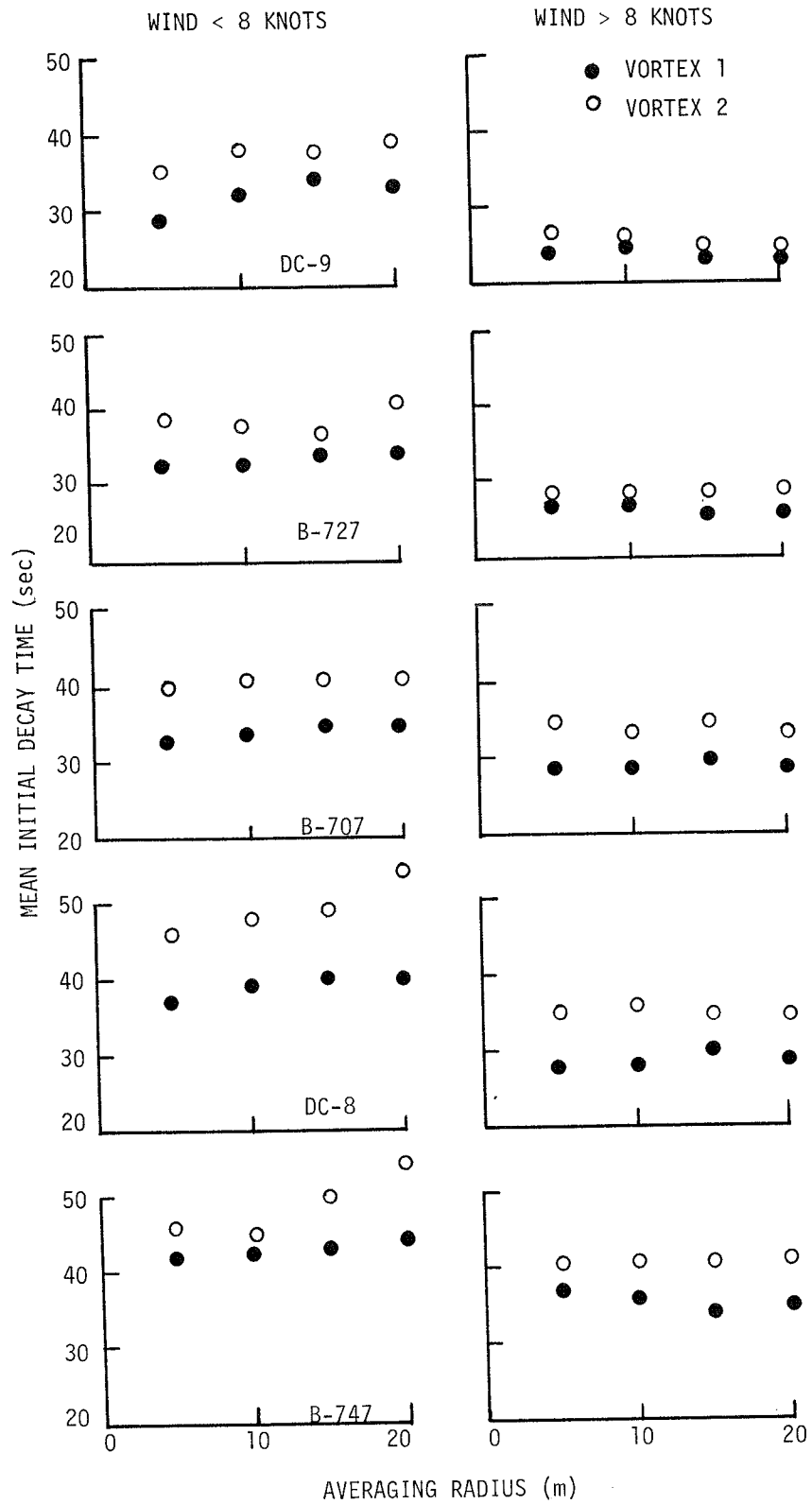
FIGURE 36. LEAST-SQUARE FITS WITH ONE FREE PARAMETER t_0 ( \sigma = 10 SECONDS, n = 2 )
