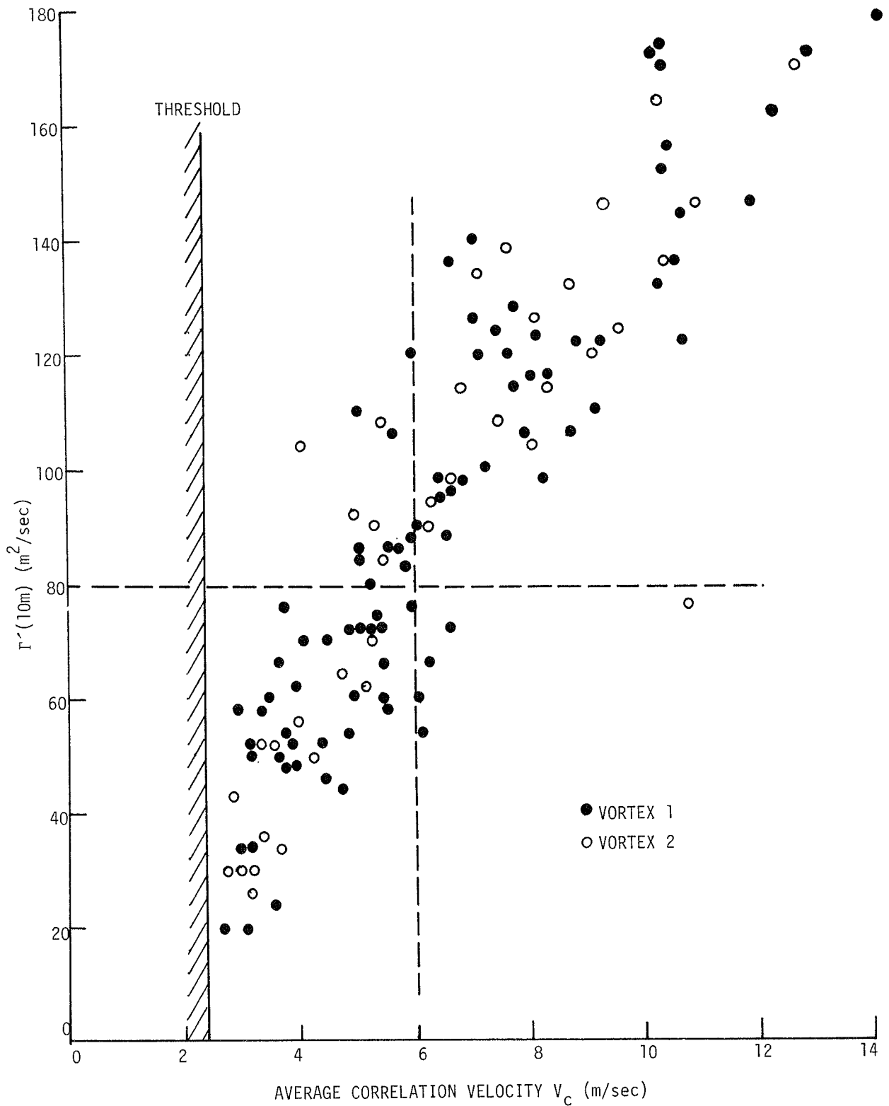
FIGURE 25. VORTEX STRENGTH VERSUS AVERAGE CORRELATION VELOCITY V_c FOR A SAMPLE OF B-707 AND DC-8 VORTICES
