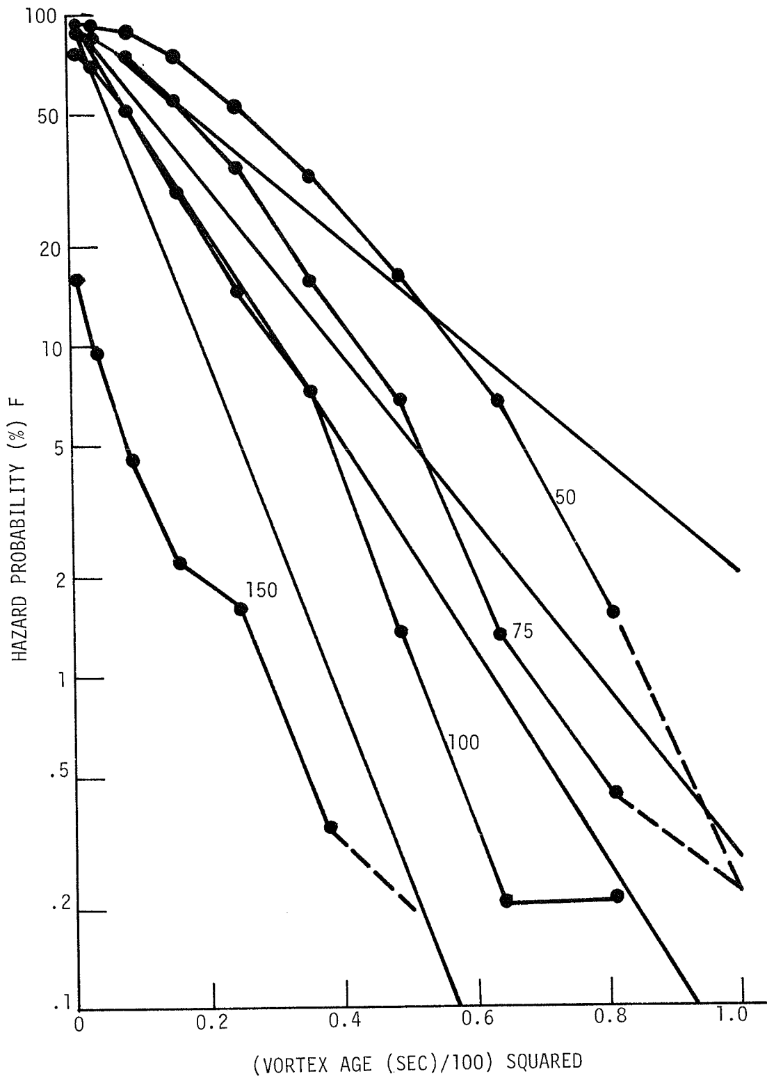
FIGURE 27. COMPARISONS OF MODEL HAZARD PROBABILITY (STRAIGHT LINES) WITH MEASUREMENTS (LINES WITH POINTS) FOR ALL B 2 -707 VORTICES WITH 10-METER AVERAGING. THE VALUES OF \Gamma_T (m 2 /SEC) ARE INDICATED.
