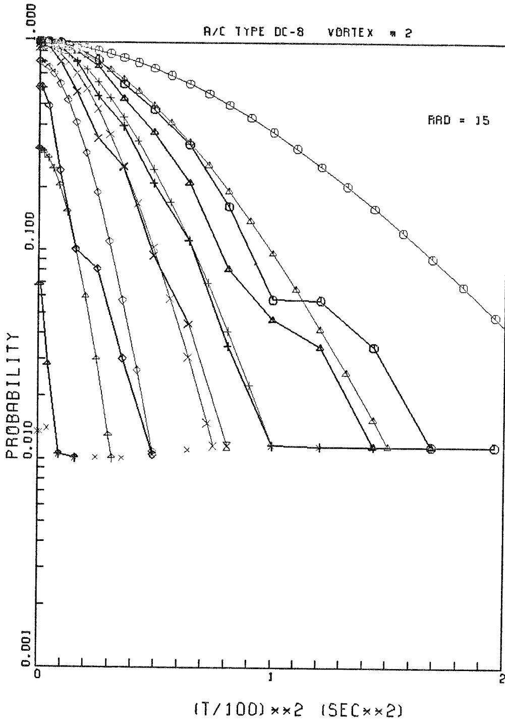
FIGURE 21. FITTED PROBABILITY DECAY CURVES FOR THE DC-8, 15-METER AVERAGING RADIUS, AND VORTEX 2. THE SIX CURVES REPRESENT T^2 VALUES OF 200, 150, 100, 75, 50, AND 30 m^2/sec , RESPECTIVELY, FROM LEFT TO RIGHT. THE MEASURED DATA ARE PLOTTED WITH THICKER LINES THAN THE FITTED CURVES. THE NUMBERS BELOW THE CURVES ARE THE VALUES OF \sigma (SEC) FOR EACH CURVE.
