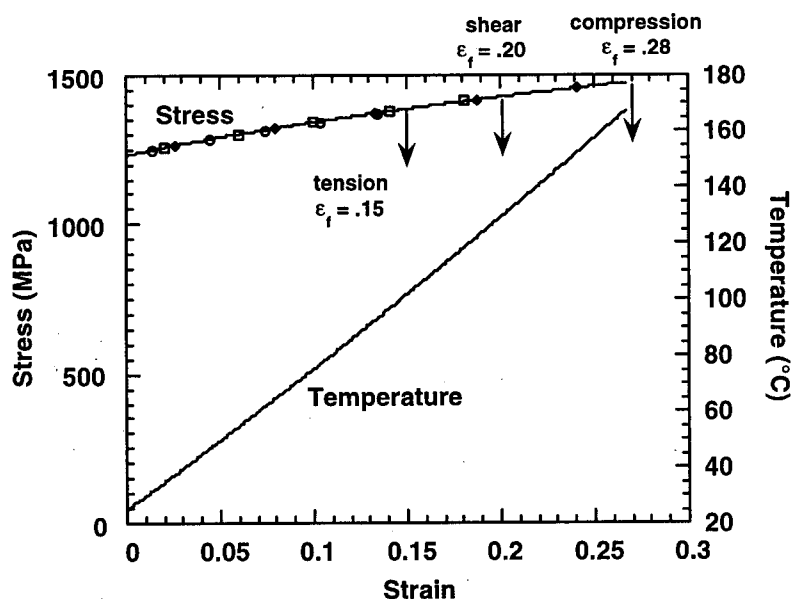
FIGURE 20. PREDICTED ADIABATIC STRESS-STRAIN RESPONSE FOR THE Ti-6Al-4V ALLOY IN TENSION, SHEAR, AND COMPRESSION AT A STRAIN RATE OF 5000 \text{ s}^{-1}
