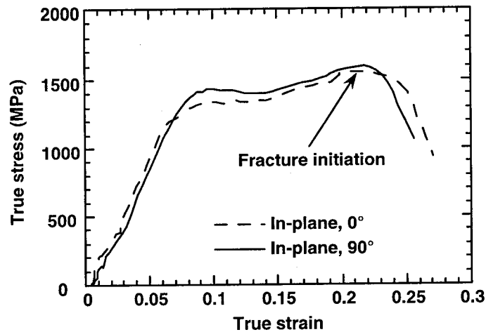
FIGURE 4. STRESS-STRAIN RESPONSE FOR Ti-6Al-4V ALLOY TESTED IN TENSION AT A STRAIN RATE OF 5200 \text{ s}^{-1}
