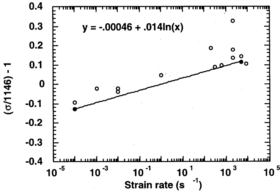
FIGURE A-2. \sigma/\sigma_1 VERSUS STRAIN RATE FOR THE Ti-6Al-4V ALLOY
