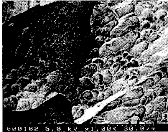
FIGURE 6. FRACTURE SURFACE OF Ti-6Al-4V SAMPLE TESTED IN COMPRESSION
