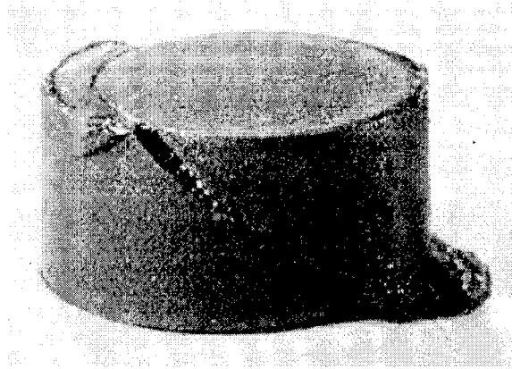
FIGURE 5. PHOTOGRAPH OF Ti-6Al-4V SAMPLE AFTER TESTING IN COMPRESSION
