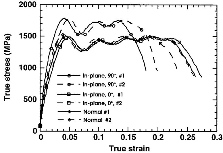
FIGURE 3. STRESS-STRAIN RESPONSE FOR Ti-6Al-4V ALLOY TESTED IN COMPRESSION AT A STRAIN RATE OF 4500 \text{ s}^{-1}
