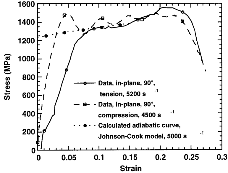
FIGURE 16. COMPARISON OF THE HIGH-STRAIN RATE, STRESS-STRAIN RESPONSE OF THE Ti-6Al-4V ALLOY PREDICTED BY THE JOHNSON-COOK MATERIAL MODEL (USING THE NEW MATERIAL PARAMETERS) WITH EXPERIMENTAL DATA IN TENSION AND COMPRESSION
