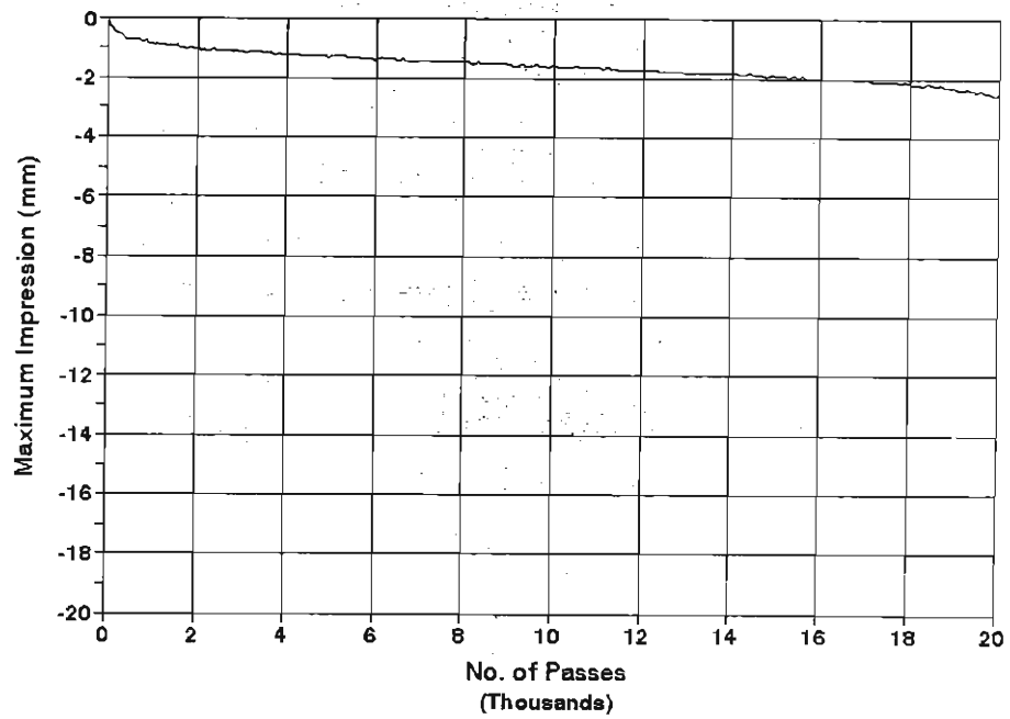
Mix 2 w/Lime,4% Water,"Mellowed" 72 hrs Temperature = 45 C
