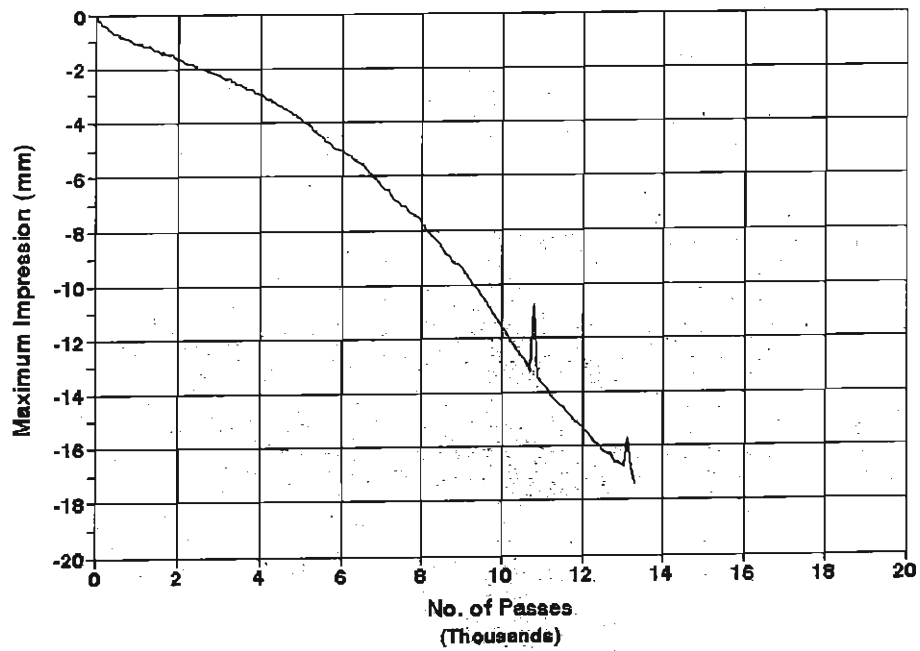
Mix 2, AC-5 Temperature = 45 C
