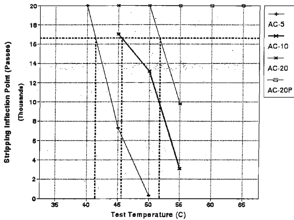
Fig. 8. Temperatures Required to Obtain a Constant Stripping Inflection Point for Various Asphalt Cement Stiffnesses for Mix 1.
