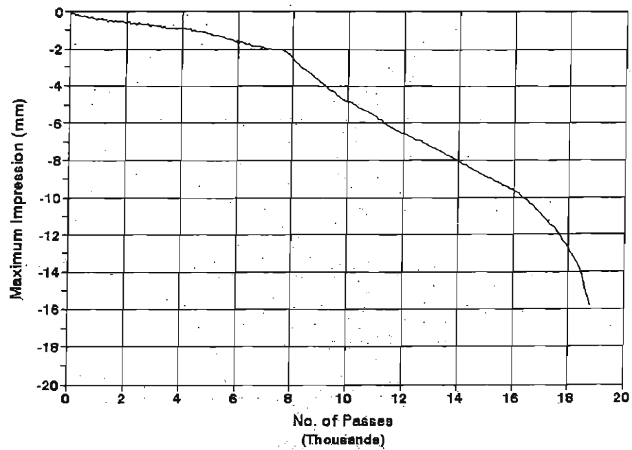
Mix 3, AC-5 Temperature = 35 C
