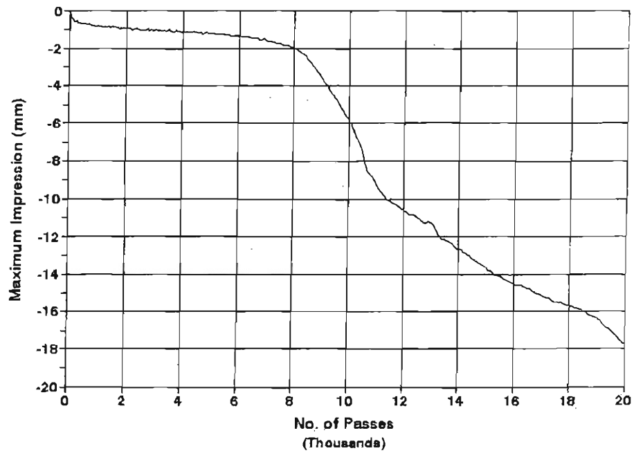
Mix 1, 4.2% Voids Temperature = 50 C
