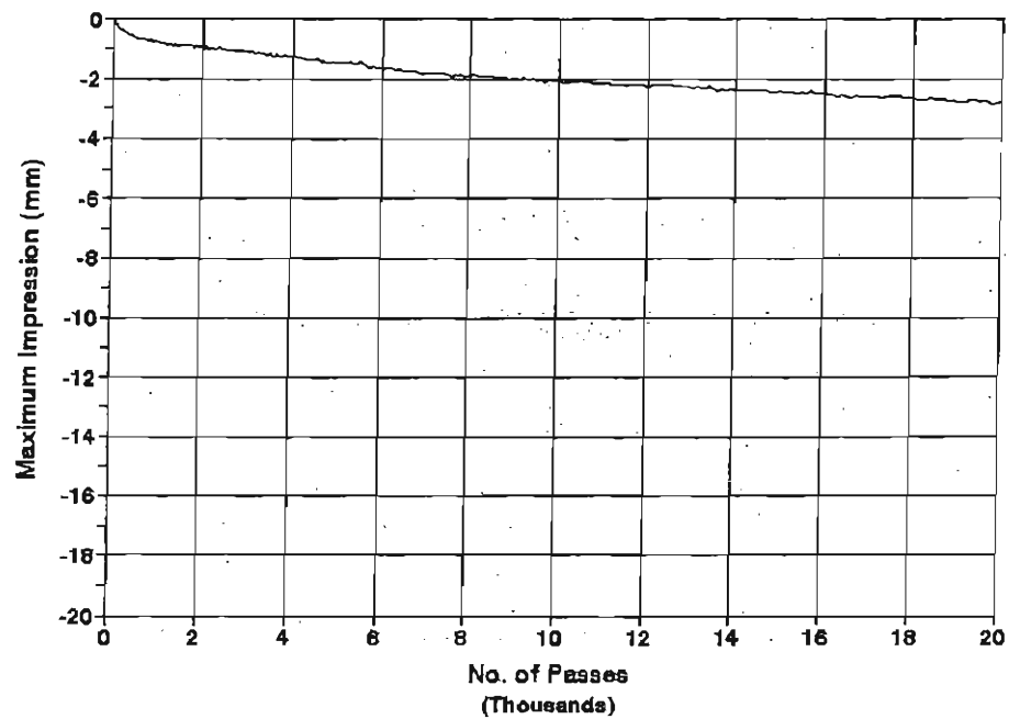
Mix 3, AC-20P Temperature = 45 C
