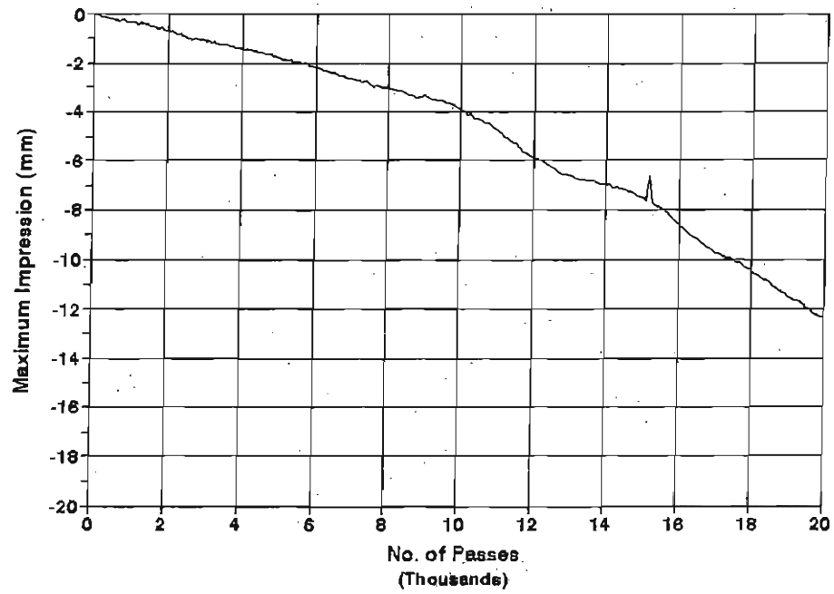
Mix 3, AC-10 Temperature = 35 C
