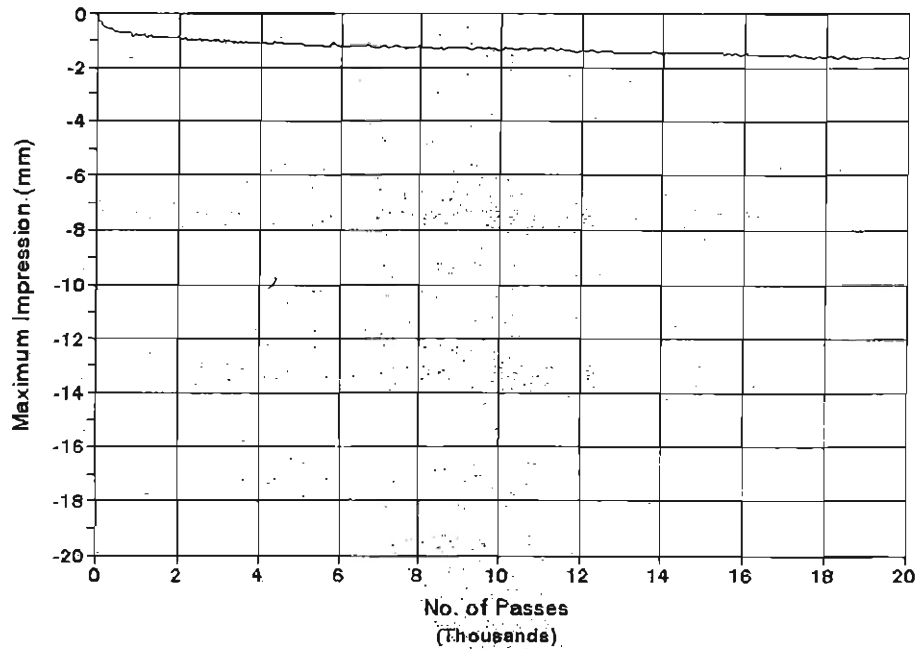
Mix 1, Short-Term Aged 8 Hours Temperature = 45 C
