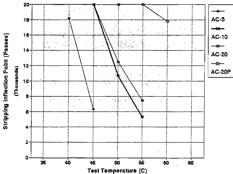
Fig. 4. Influence on Stripping Inflection Point for Various Temperatures and Asphalt Cement Stiffnesses for Mix 1.
