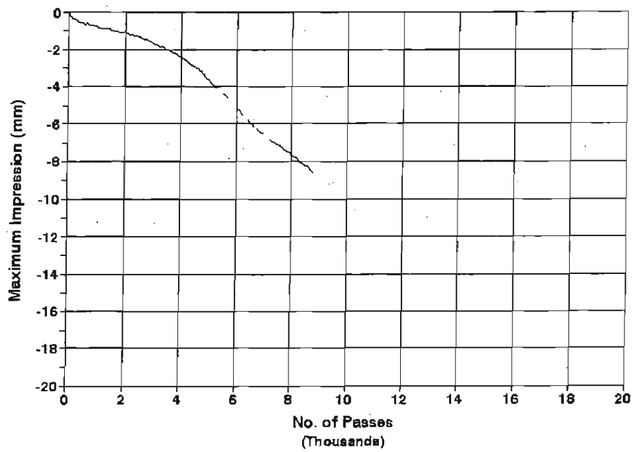
Mix 4, 7.5% Air Voids Temperature = 50 C
