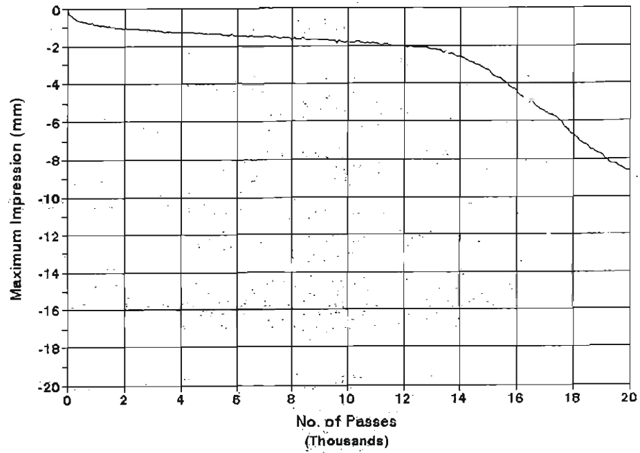
Mix 1, Short-Term Aged 4 Hours Temperature = 45 C
