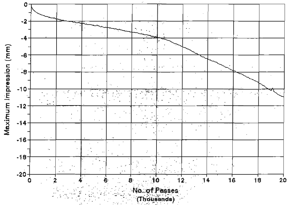
Mix 2, Short-Term Aged 4 Hours Temperature = 45 C
