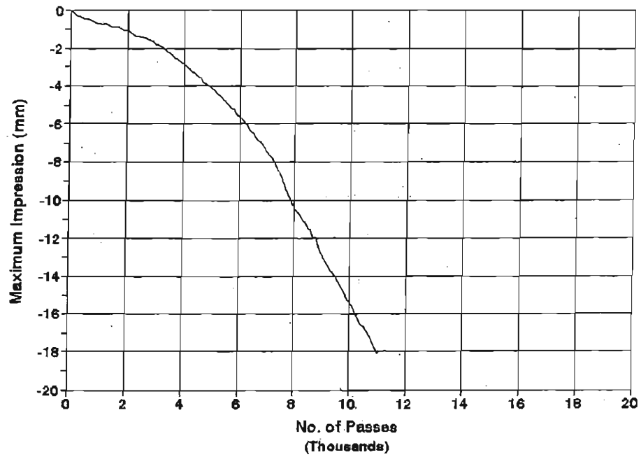
Mix 3, AC-20 Temperature = 45 C
