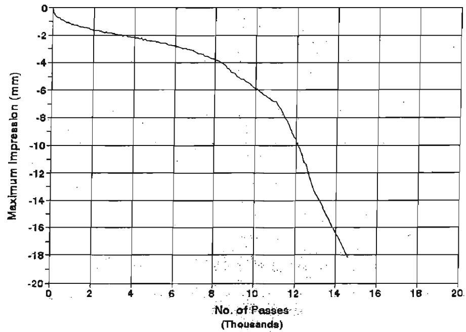
Mix 1, AC-20 Temperature = 55 C
