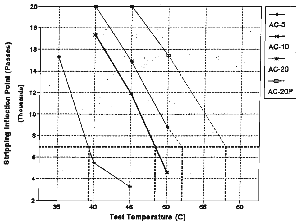
Fig. 10. Temperatures Required to Obtain a Constant Stripping Inflection Point for Various Asphalt Cement Stiffnesses for Mix 3.
