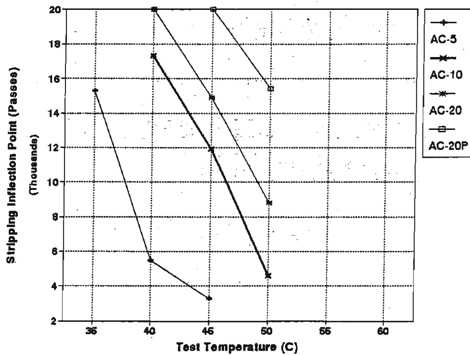
Fig. 6. Influence on Stripping Inflection Point for Various Temperatures and Asphalt Cement Stiffnesses for Mix 3.
