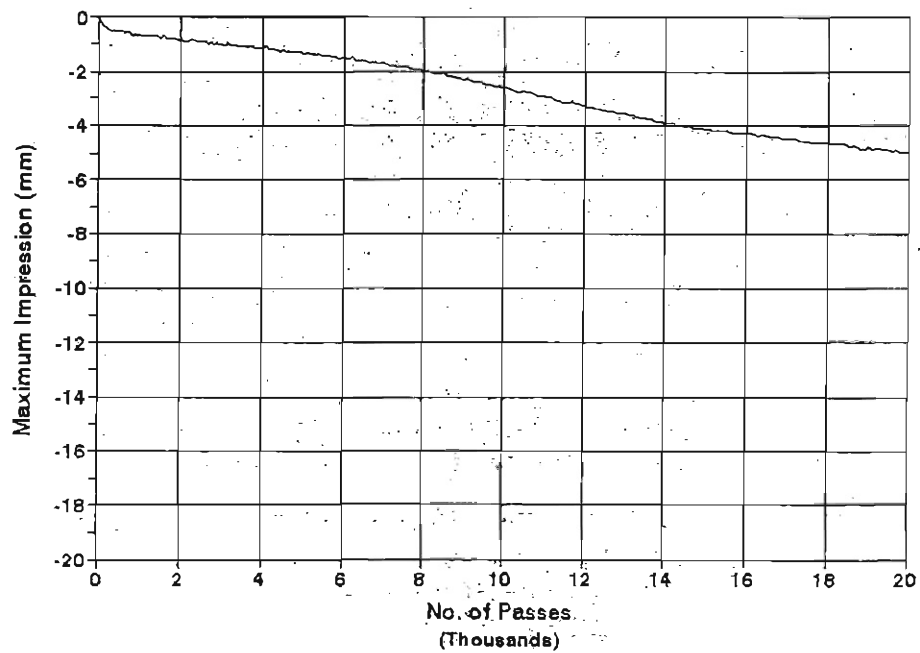
Mix 3 with Lime and 4% Water Temperature = 45 C
