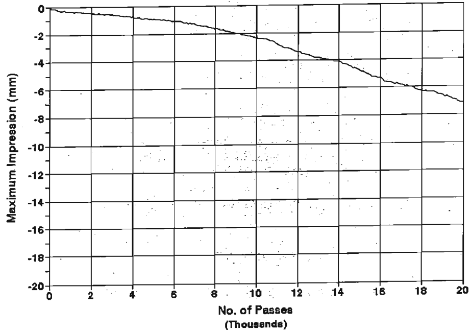
Mix 3, AC-20P Temperature = 50 C
