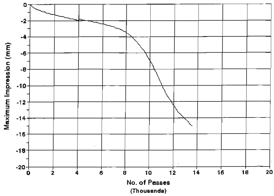
Mix 4, 9.3% Voids Temperature = 50 C
