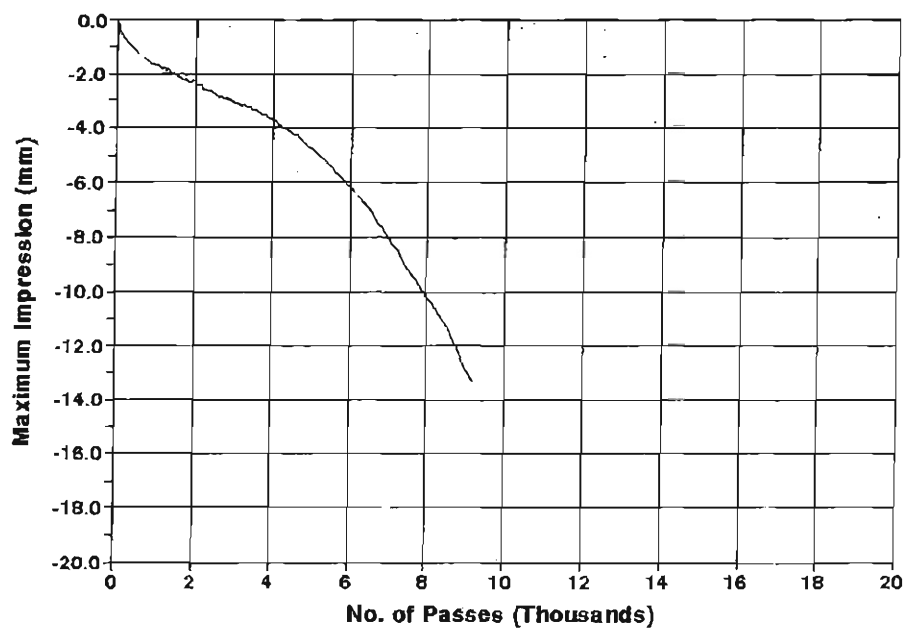
Mix 2, 8.7% Voids Temperature = 50 C
