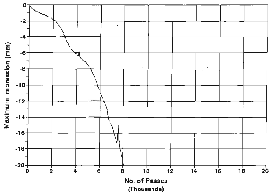
Mix 3, 10.5% Voids Temperature = 50 C
