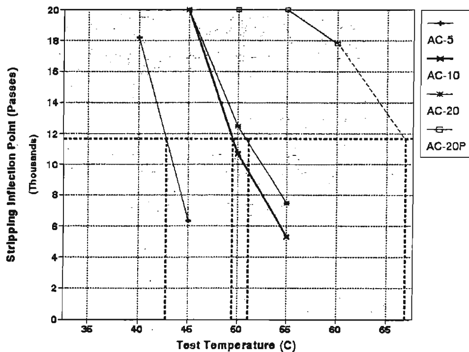
Fig. 9. Temperatures Required to Obtain a Constant Stripping Inflection Point for Various Asphalt Cement Stiffnesses for Mix 2.
