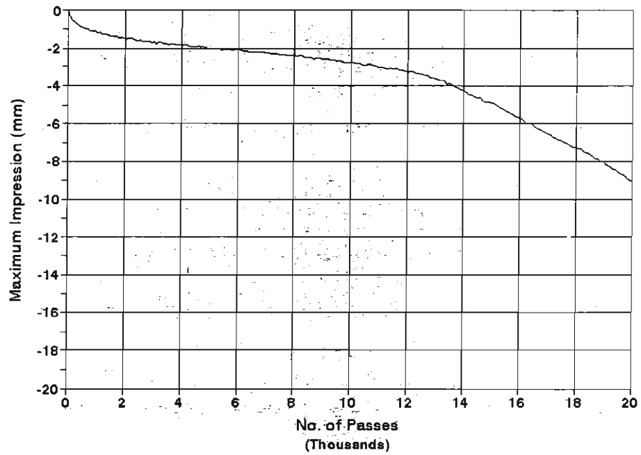
Mix 2 with Lime and 4% Water Temperature = 45 C
