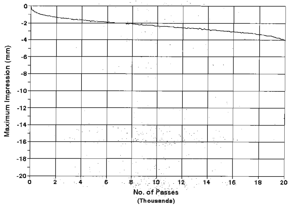
Mix 4 with Lime and 2% Water Temperature = 45 C
