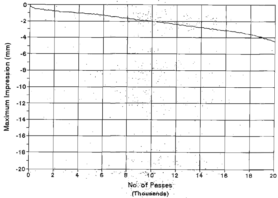
Mix 3 with Lime and Zero Water Temperature = 45 C
