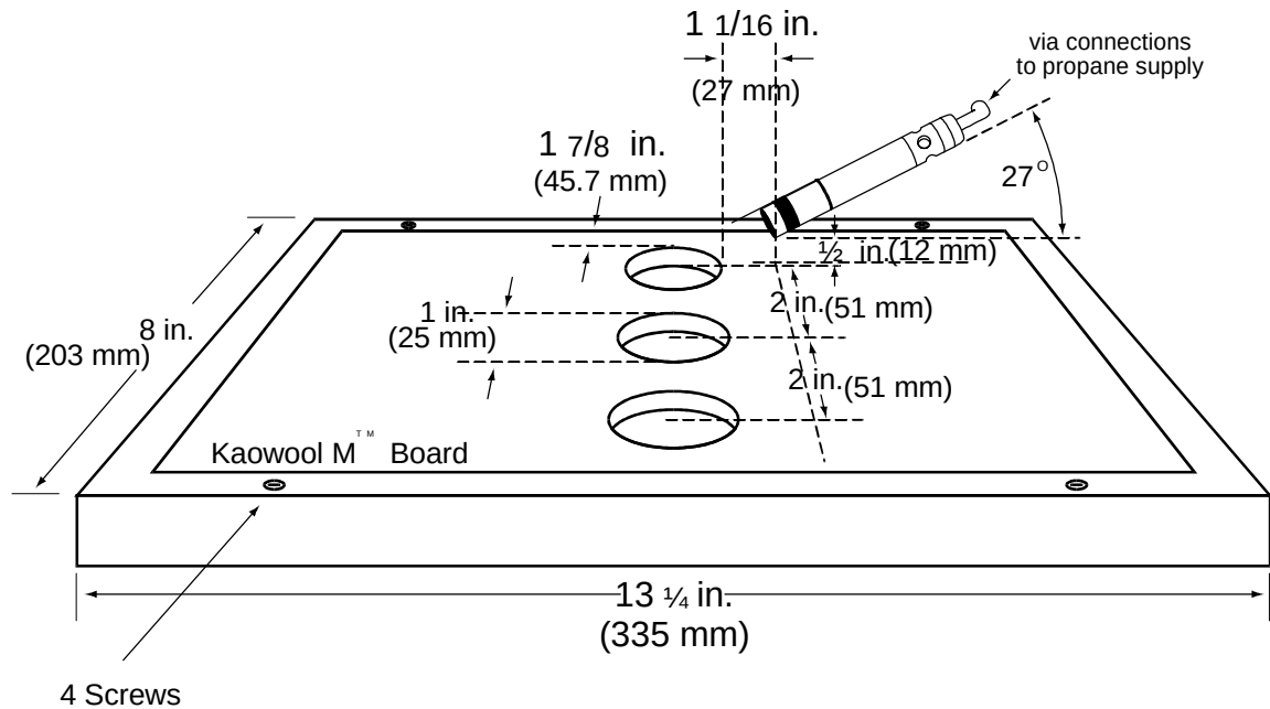
FIGURE A-8. CALORIMETER HOLDING FRAME
