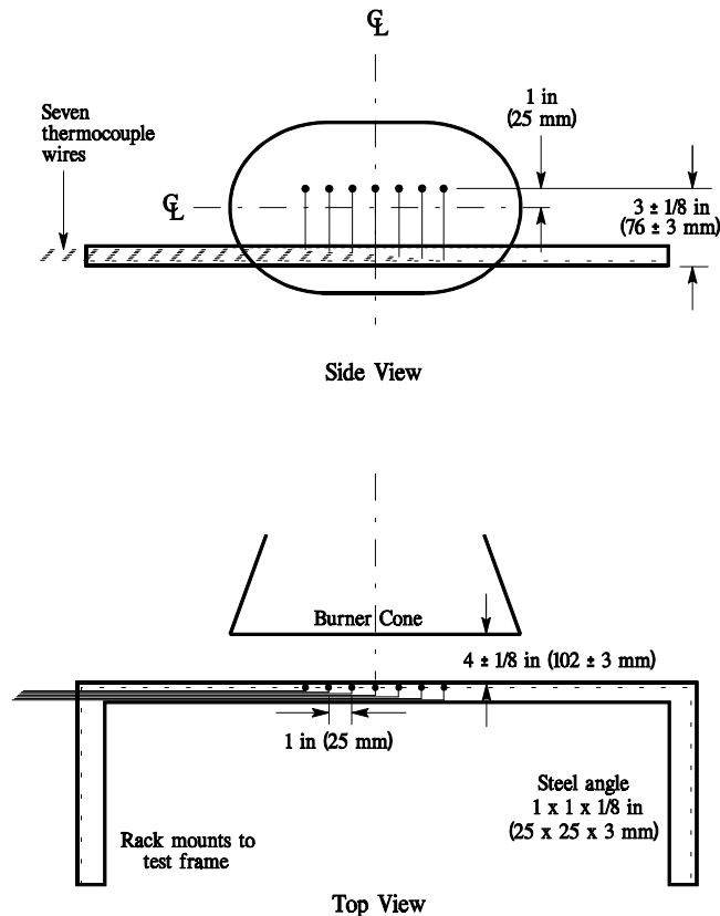
FIGURE B-5. THERMOCOUPLE RAKE POSITION RELATIVE TO BURNER CONE
