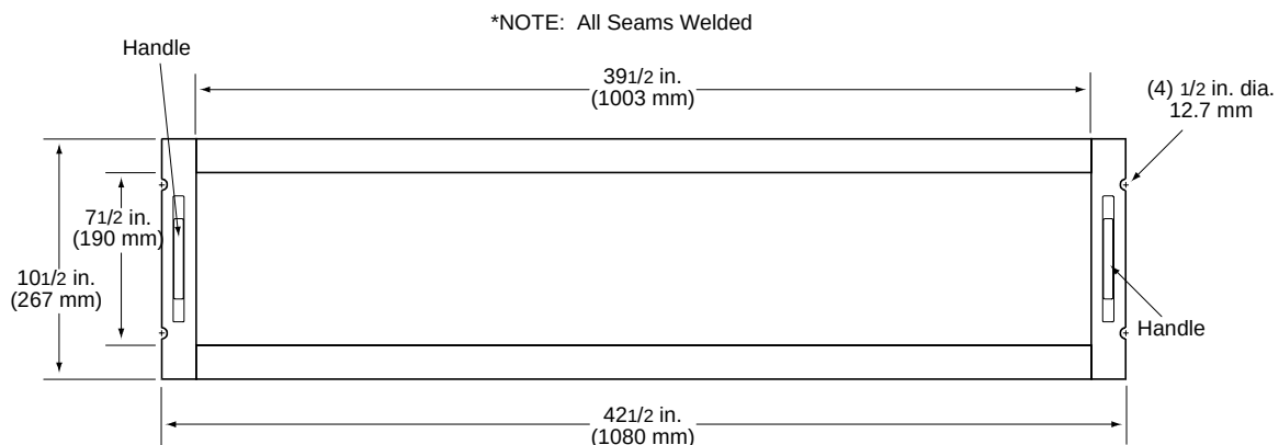
FIGURE A-6. SECURING FRAME
