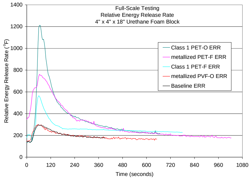
FIGURE 18. RELATIVE ENERGY RELEASE RATE CALCULATION FOR FULL-SCALE TESTS
