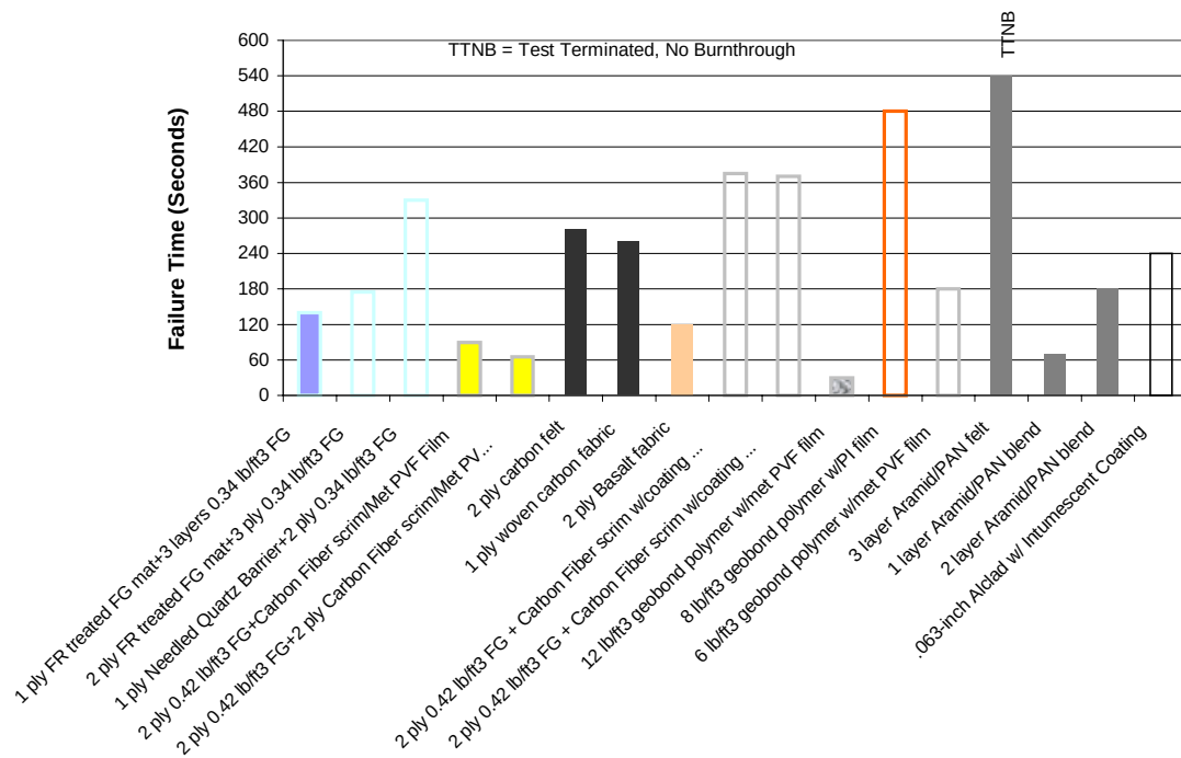
FIGURE 40. BURNTHROUGH TEST COMPARISON USING A 6-GPH BURNER AT 4 INCHES FROM THE TEST RIG
