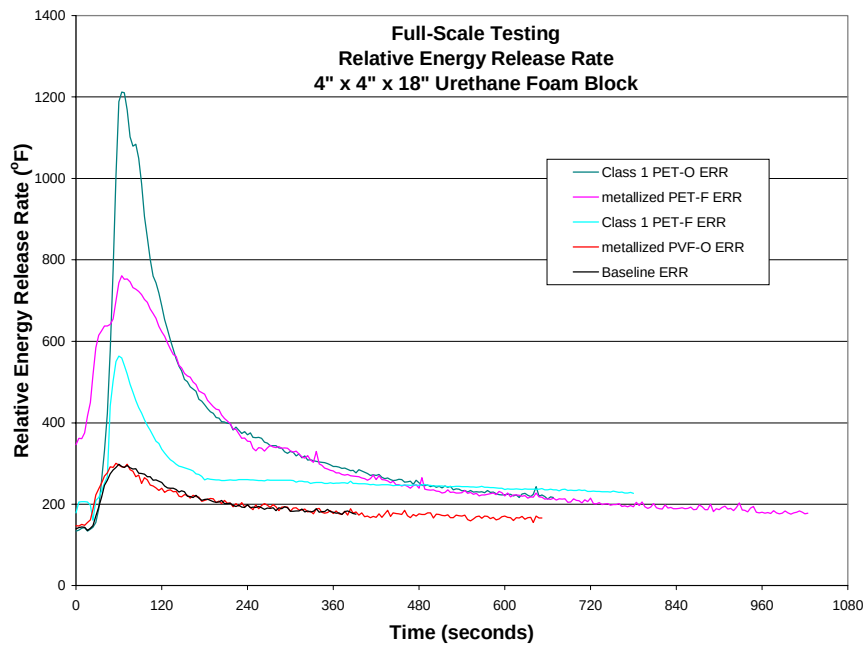
FIGURE 27. ESTIMATED ENERGY RELEASE RATES DURING FULL-SCALE TESTING
