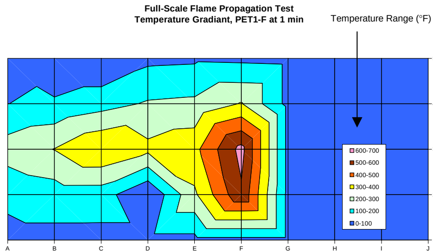
FIGURE 19. TYPICAL ISOTHERM PLOT IN DC-10 OVERHEAD AREA USING THERMOCOUPLE DATA
