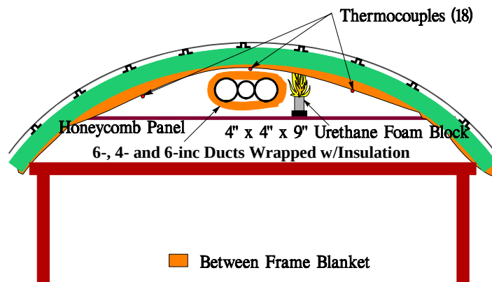
FIGURE 13. NARROW-BODY TEST CONFIGURATION USING A B707 FUSELAGE SECTION
