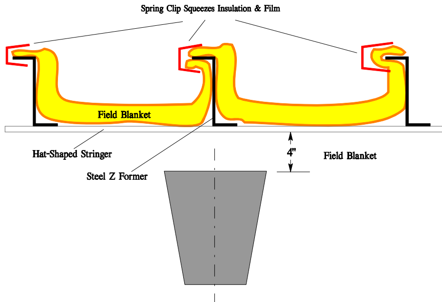
FIGURE 36. IMPROVED INSULATION BLANKET TEST SPECIMEN ATTACHMENT METHOD
