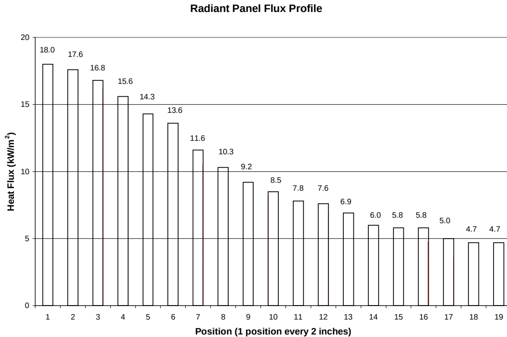
FIGURE 22. RADIANT PANEL FLUX PROFILE
