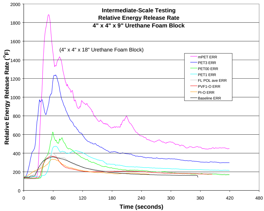
FIGURE 26. ESTIMATED ENERGY RELEASE RATES DURING MOCK-UP INTERMEDIATE-SCALE TESTING
