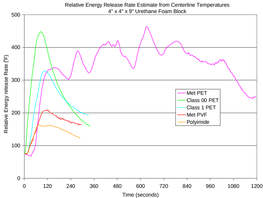
FIGURE 15. RELATIVE ENERGY RELEASE RATE CALCULATION FOR NARROW-BODY TESTS
