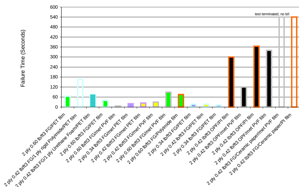
FIGURE 38. BURNTHROUGH TEST COMPARISON USING A 6-GPH BURNER AT 4 INCHES FROM THE TEST RIG
