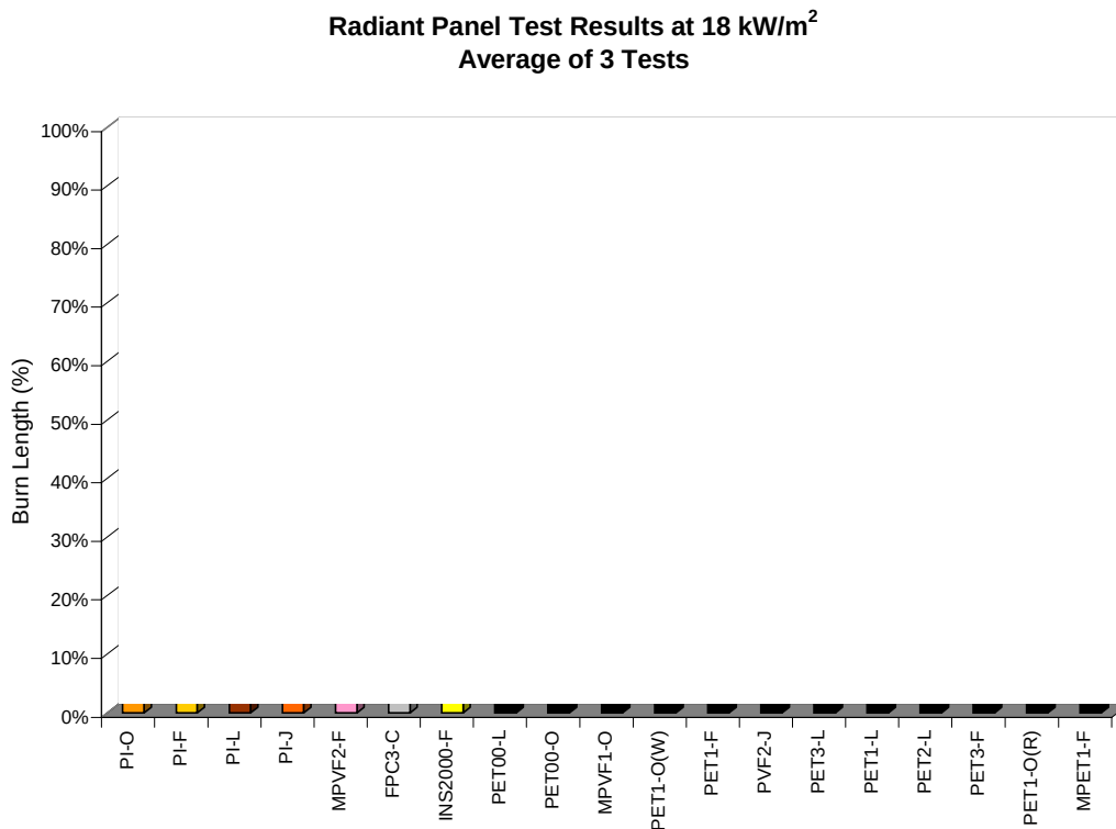
FIGURE 23. INITIAL RESULTS USING RADIANT PANEL TEST APPARATUS
