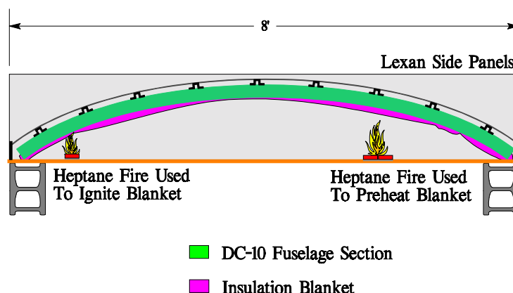
FIGURE 8. MOCK-UP ENCLOSURE USING HEPTANE FUEL FIRE
