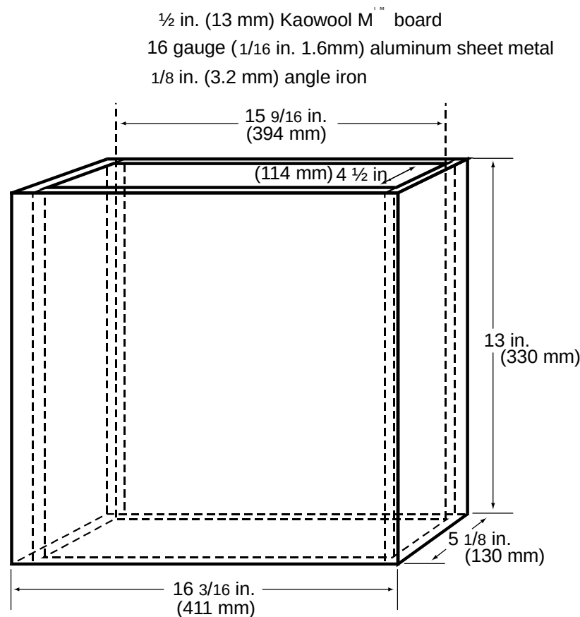
FIGURE A-2. INTERNAL CHIMNEY
