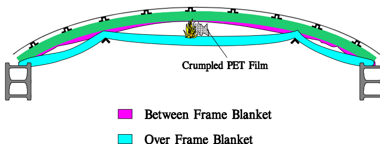
FIGURE 9. INITIAL MOCK-UP TEST CONFIGURATION USING A B747 FUSELAGE SECTION
