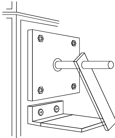
FIGURE A-9. PROPANE BURNER STOP
