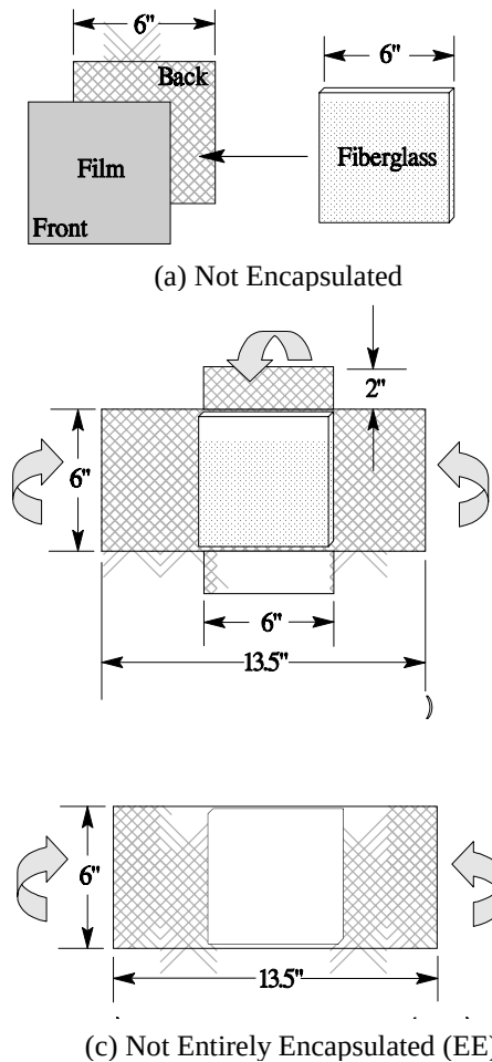
FIGURE 1. VARIOUS METHODS OF CONSTRUCTING INSULATION TEST SAMPLES FOR OSU TESTING
