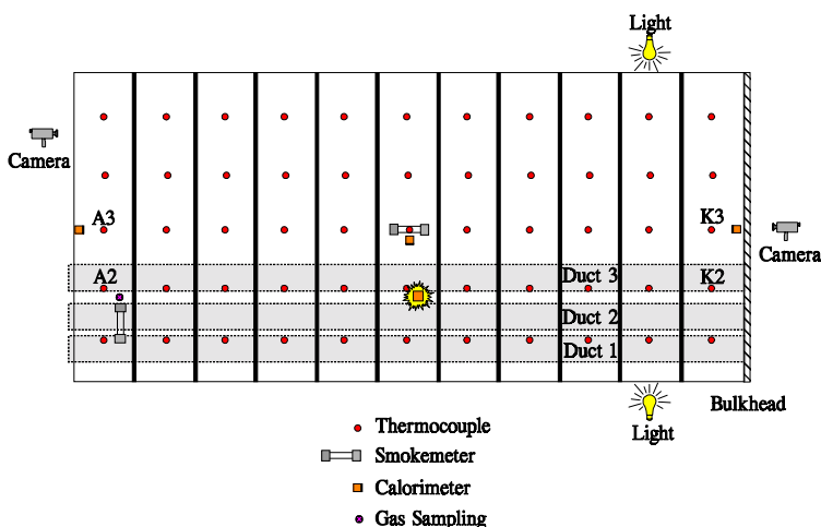
FIGURE 16. FULL-SCALE TEST CONFIGURATION IN DC-10 OVERHEAD
