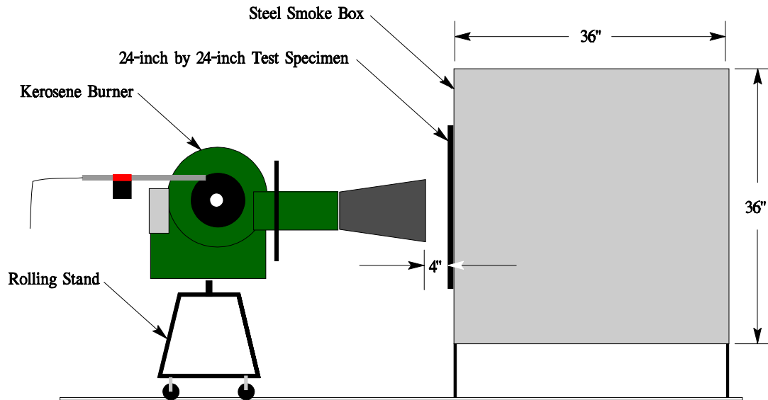
FIGURE 29. INITIAL BURNTHROUGH BOX APPARATUS
