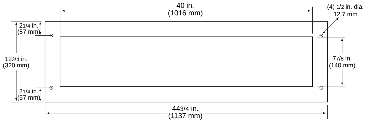
FIGURE A-5. RETAINNG FRAME
