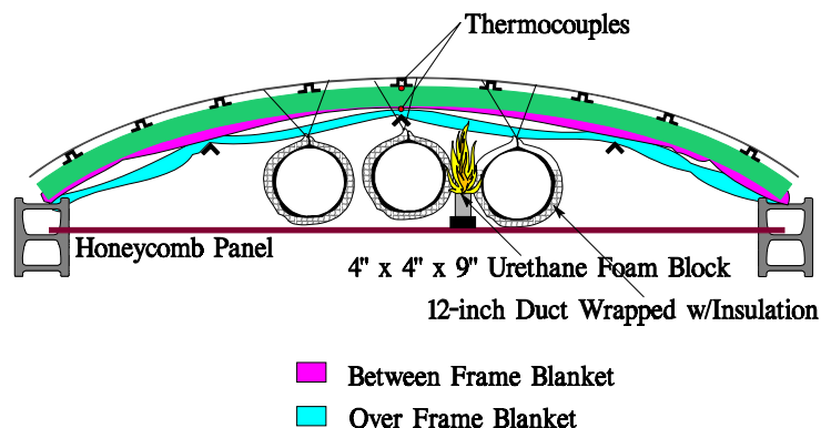
FIGURE 10. FINALIZED MOCK-UP TEST CONFIGURATION USING A B747 FUSELAGE SECTION
