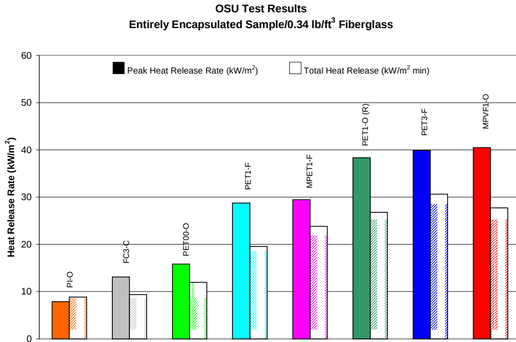
FIGURE 25. OSU TEST RESULTS OF MATERIALS COMMON TO MOCK-UP AND FULL-SCALE TESTING
