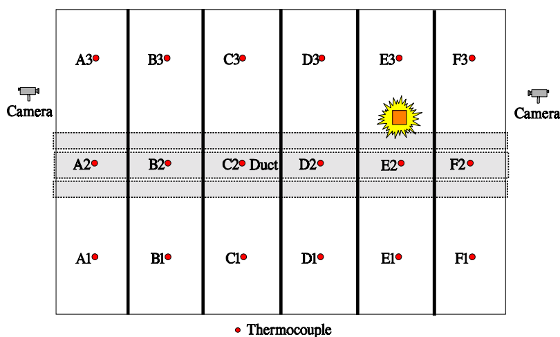
FIGURE 14. NARROW-BODY MOCK-UP TEST INSTRUMENTATION CONFIGURATION
