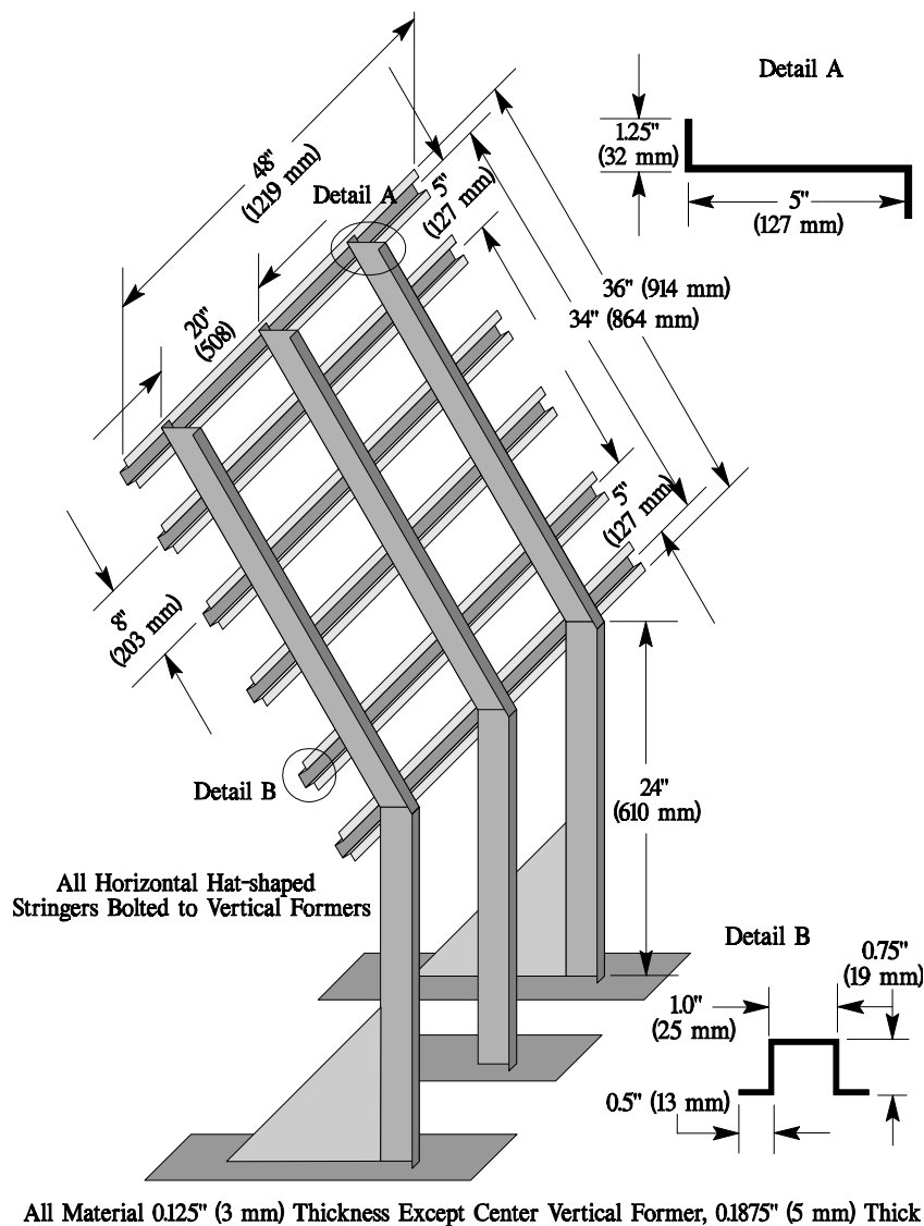
FIGURE 41. FINALIZED BURNTHROUGH TEST RIG (BURNER NOT SHOWN)
