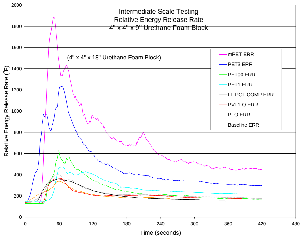
FIGURE 12. RELATIVE ENERGY RELEASE RATE CALCULATION OF MATERIALS USED IN WIDE-BODY TESTS
