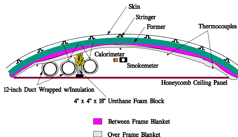
FIGURE 17. FULL-SCALE TEST CONFIGURATION IN DC-10 OVERHEAD
