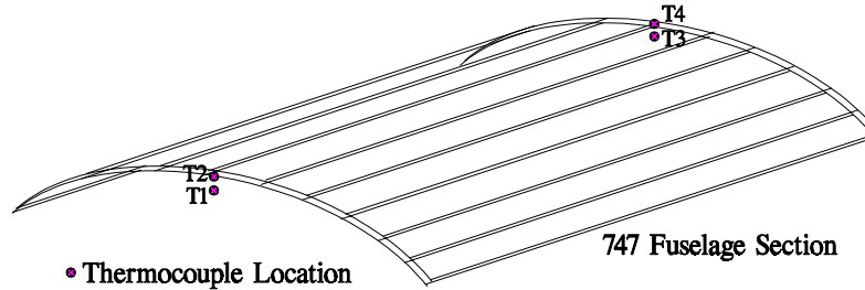
FIGURE 11. PLACEMENT OF TEMPERATURE SENSORS
