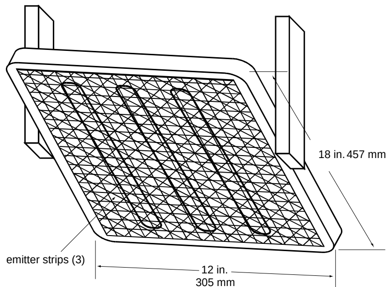
FIGURE A-3a. AIR-PROPANE RADIANT PANEL
