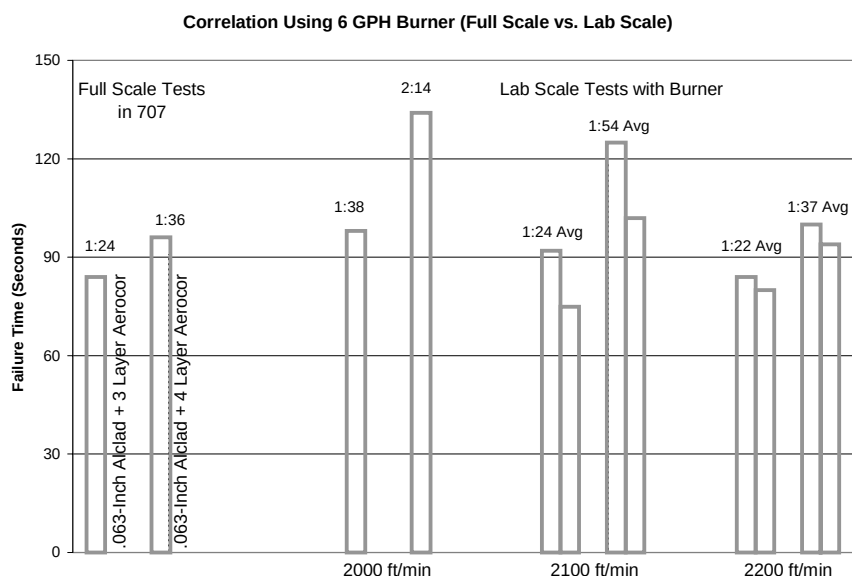
FIGURE 42. CORRELATION TEST RESULTS USING THE PROPOSED 6-GPH BURNER
