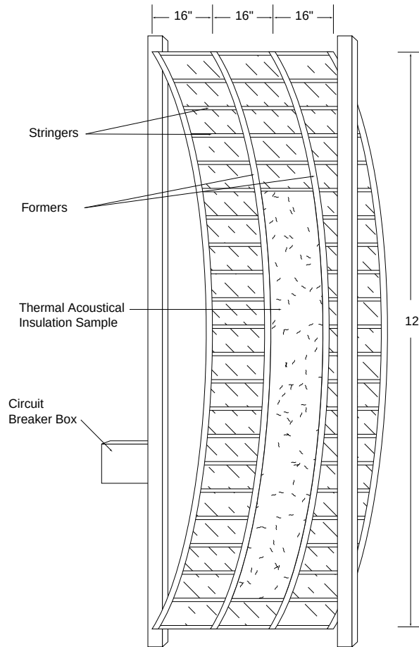
FIGURE 5. ELECTRICAL ARC TEST RIG
