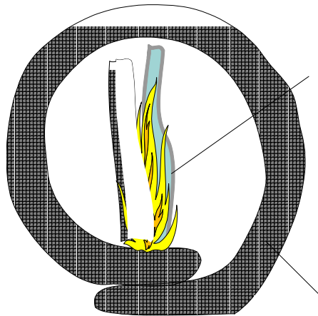
FIGURE 6. HOLLOW INSULATION TUBE TEST CONFIGURATION
