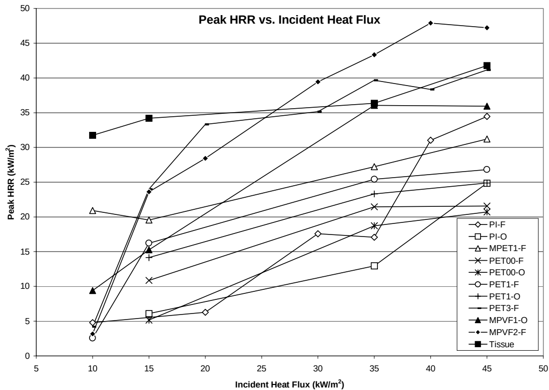
FIGURE 2. PEAK HEAT RELEASE RATE RESULTS AT VARIOUS INCIDENT HEAT FLUX LEVELS
