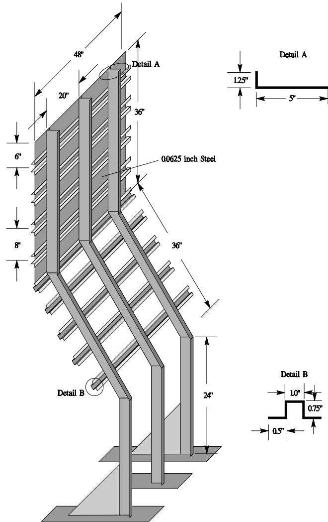
FIGURE 37. TEST RIG WITH LOWER STEEL PANEL REMOVED
