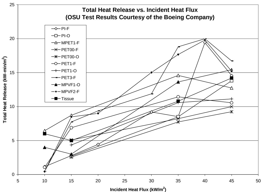
FIGURE 3. TOTAL HEAT RELEASE RESULTS AT VARIOUS INCIDENT HEAT FLUX LEVELS
