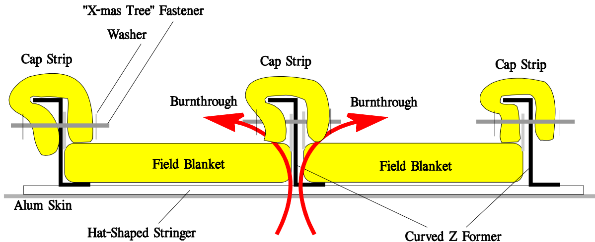
FIGURE 32. OEM STYLE OF BLANKET ATTACHMENT TO THE TEST RIG
