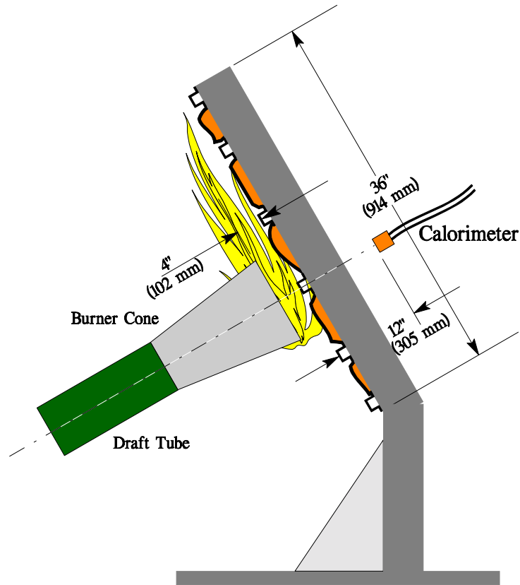
FIGURE B-6. POSITION OF BACKFACE CALORIMETERS RELATIVE TO TEST SPECIMEN FRAME
