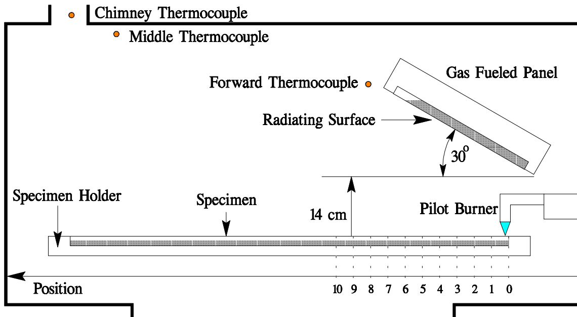
FIGURE 20. RADIANT PANEL TEST APPARATUS
