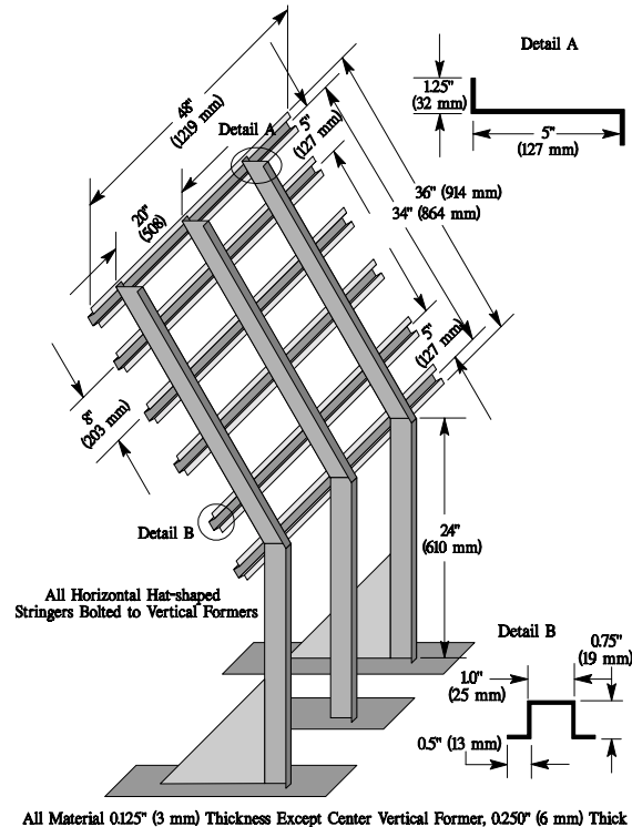
FIGURE B-1. BURNTHROUGH TEST APPARATUS SPECIMEN HOLDER
