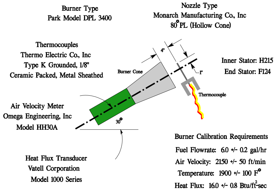
FIGURE B-8. BURNER INFORMATION AND CALIBRATION SETTINGS
