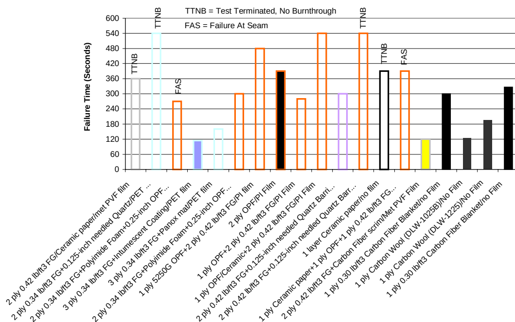
FIGURE 39. BURNTHROUGH TEST COMPARISON USING A 6-GPH BURNER AT 4 INCHES FROM THE TEST RIG
