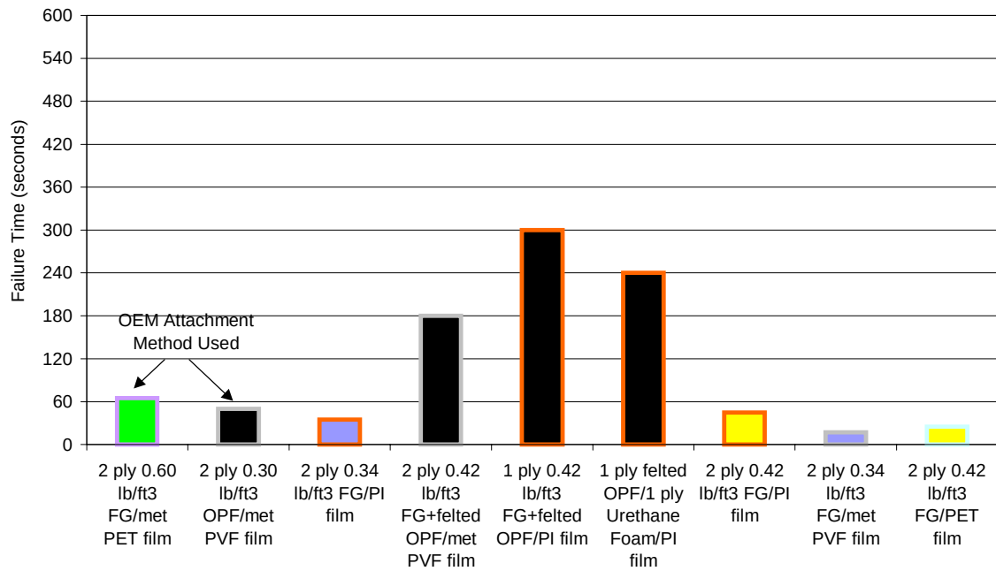
FIGURE 35. BURNTHROUGH TEST RESULTS USING THE TEST RIG WITH A 24- BY 24-INCH VOID IN LOWER SECTION
