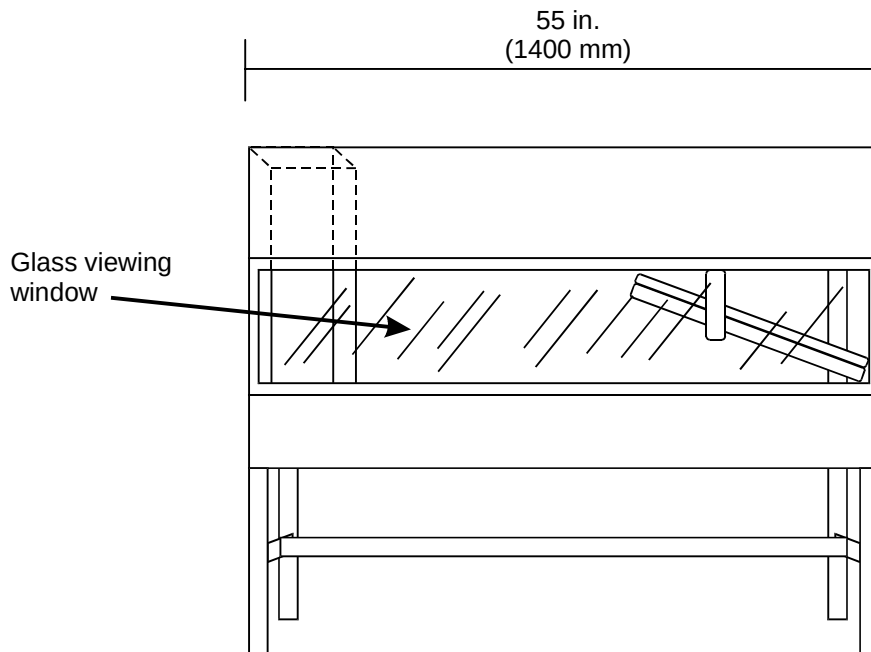
FIGURE A-1. RADIANT PANEL TEST CHAMBER
