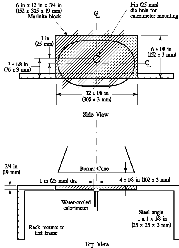
FIGURE B-4. CALORIMETER POSITION RELATIVE TO BURNER CONE
