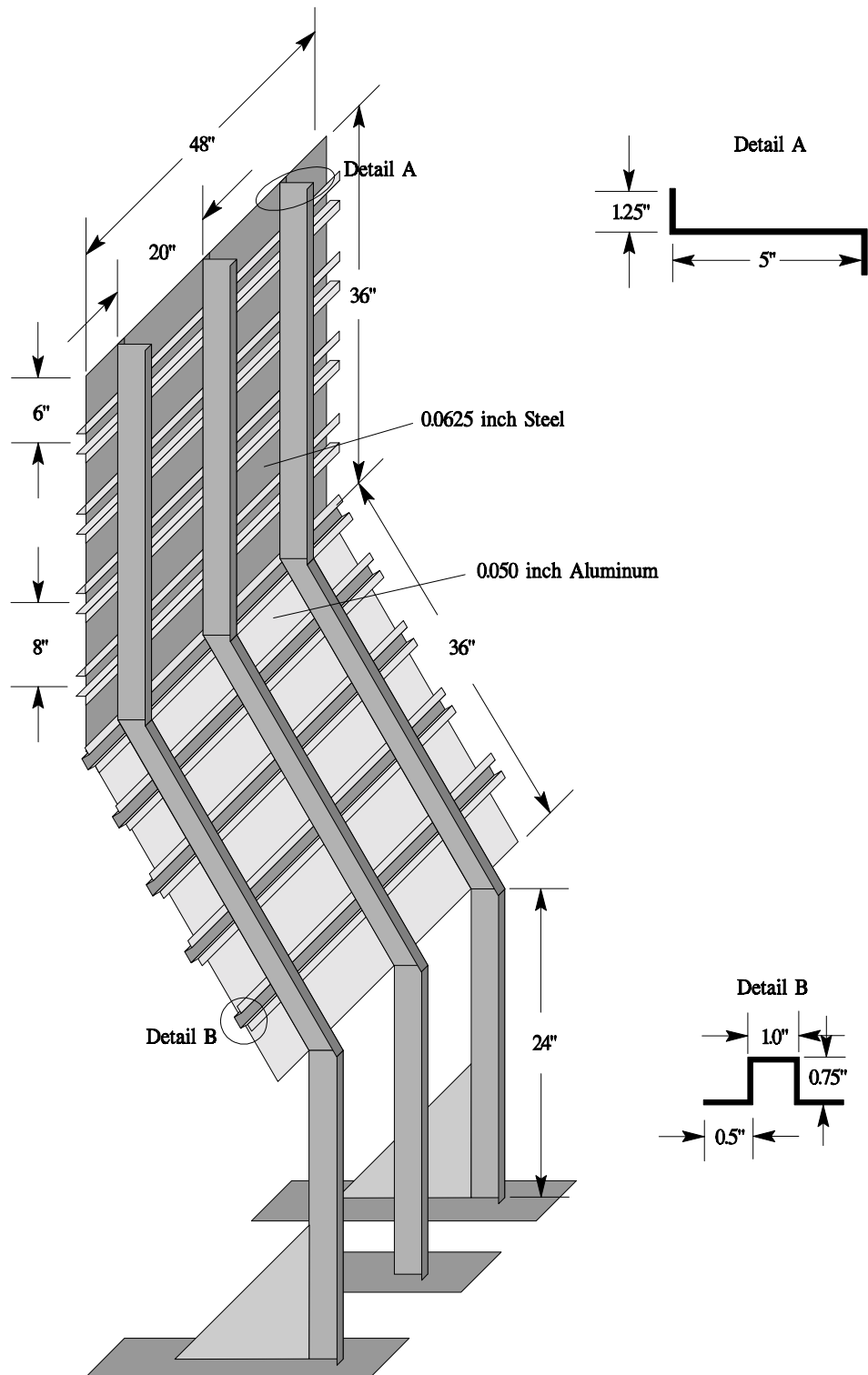
FIGURE 33. IMPROVED LABORATORY-SCALE BURNTHROUGH RIG USING FLAT SURFACES
