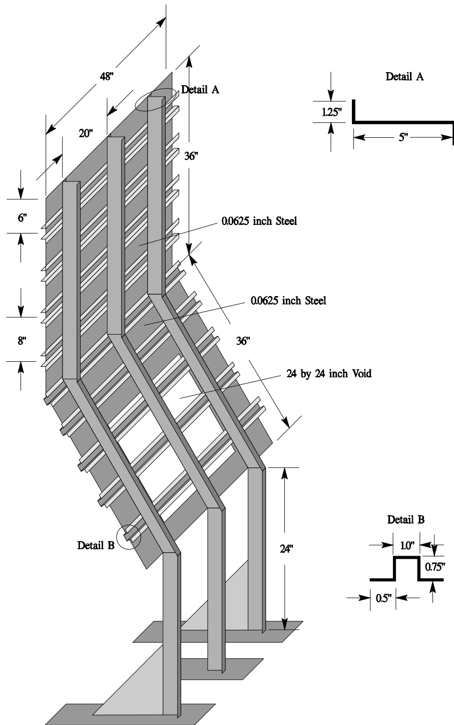
FIGURE 34. IMPROVED TEST RIG WITH 24- BY 24-INCH VOID MODIFICATION TO THE LOWER SECTION
