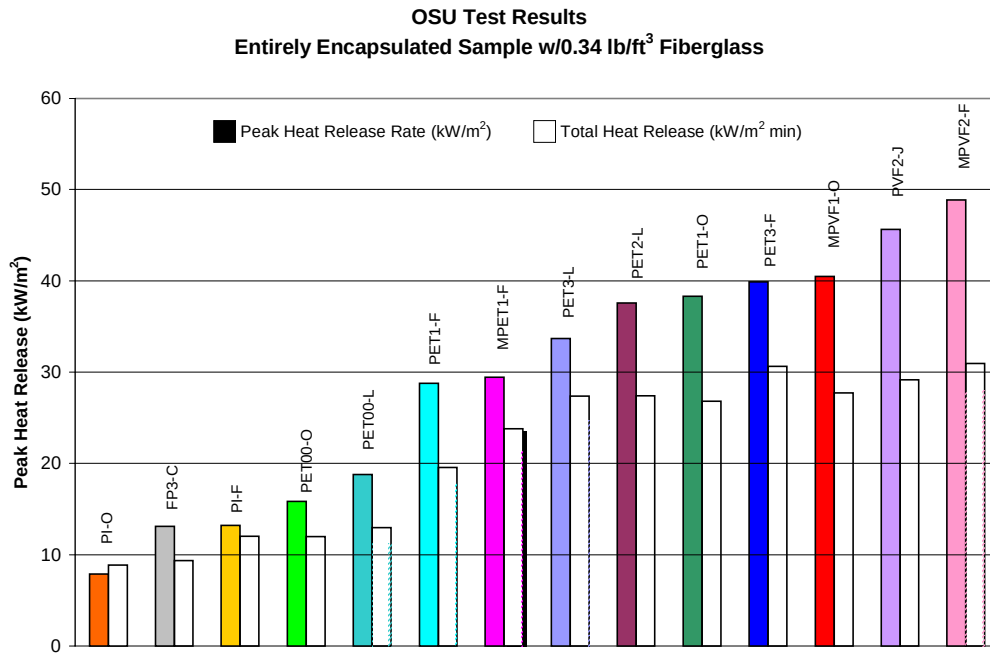
FIGURE 24. OSU TEST RESULTS USING THE ENTIRELY ENCAPSULATED METHOD OF SAMPLE PREPARATION
