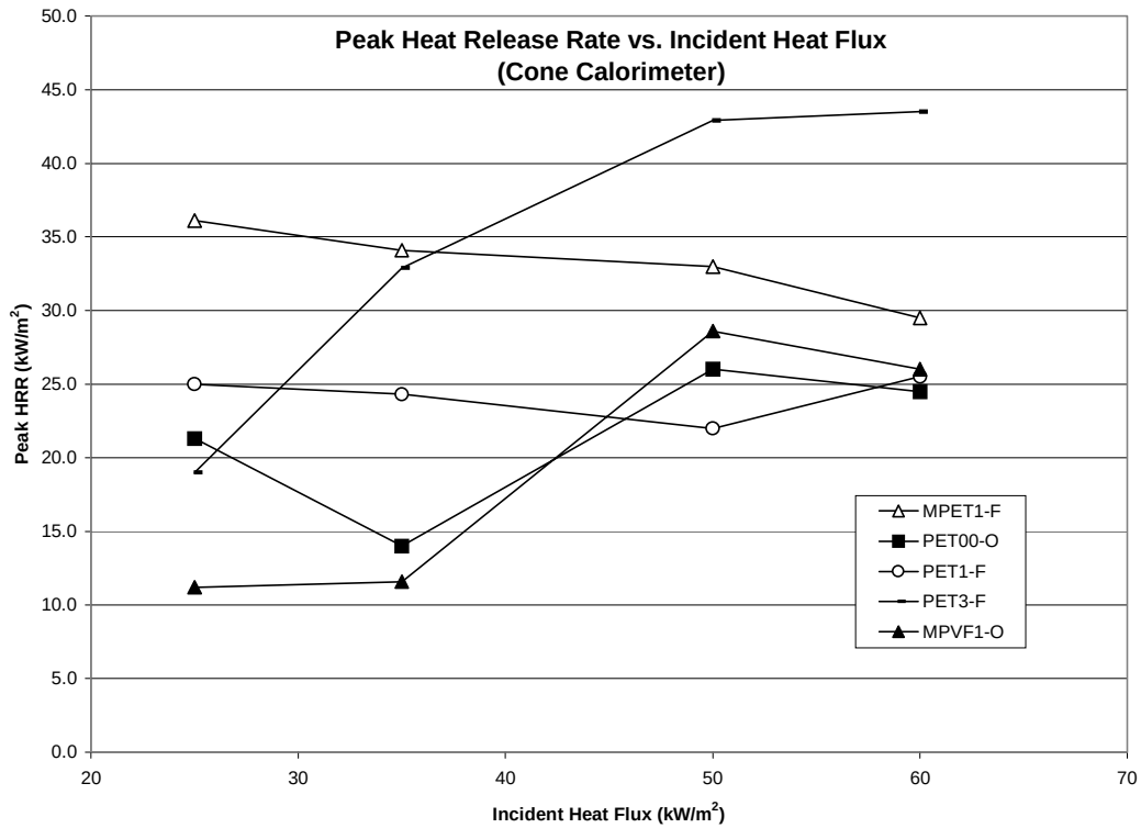
FIGURE 4. PEAK HEAT RELEASE RATE RESULTS USING CONE CALORIMETER
