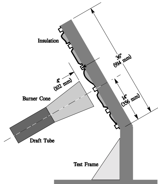
FIGURE B-2. BURNTHROUGH TEST APPARATUS
