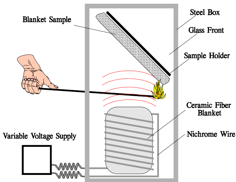
FIGURE 7. CABINET PREHEATING CONFIGURATION
