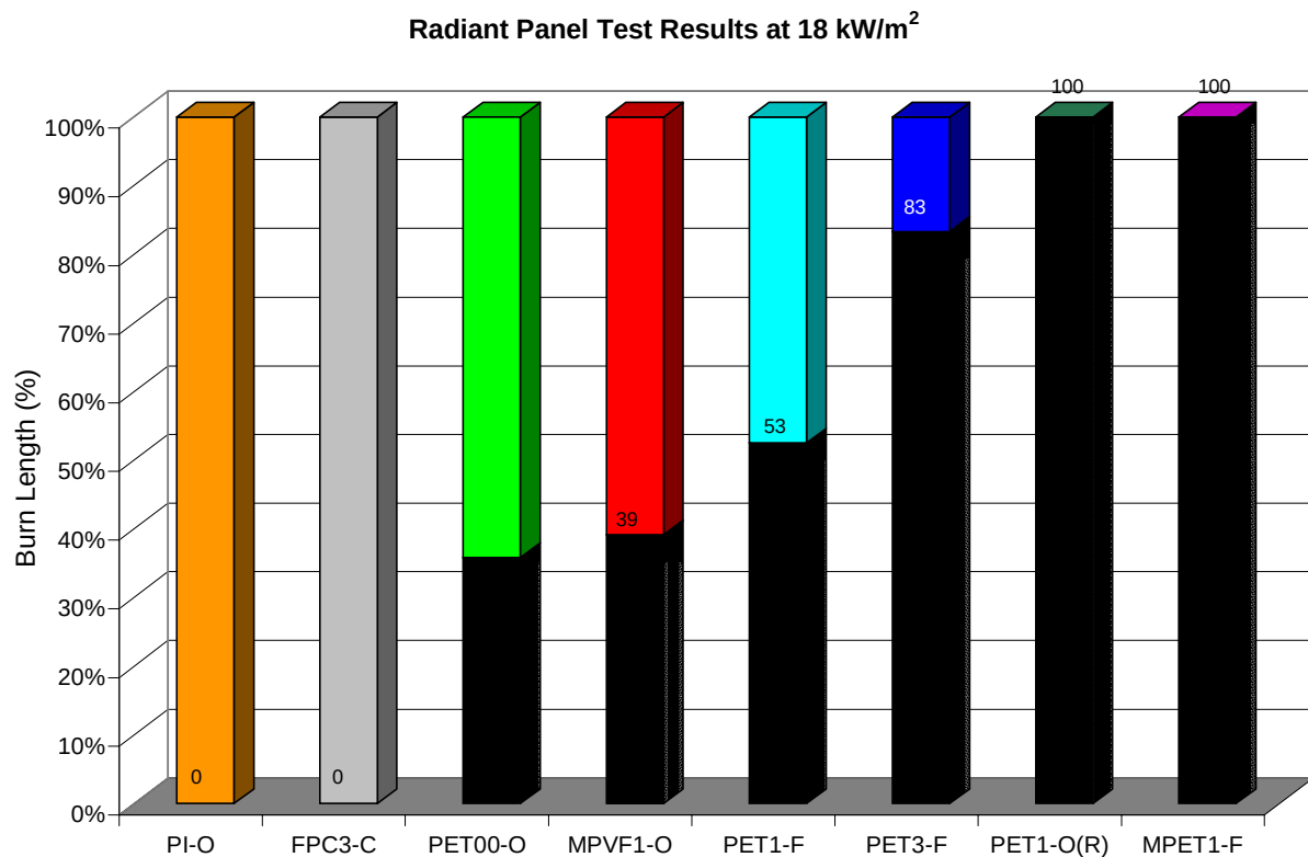
FIGURE 28. RADIANT PANEL TEST DATA FOR MATERIALS COMMON TO MOCK-UP AND FULL-SCALE TESTS
