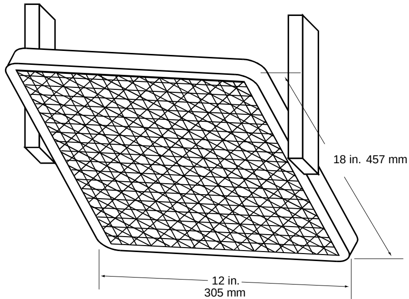
FIGURE A-3a. AIR-PROPANE RADIANT PANEL
