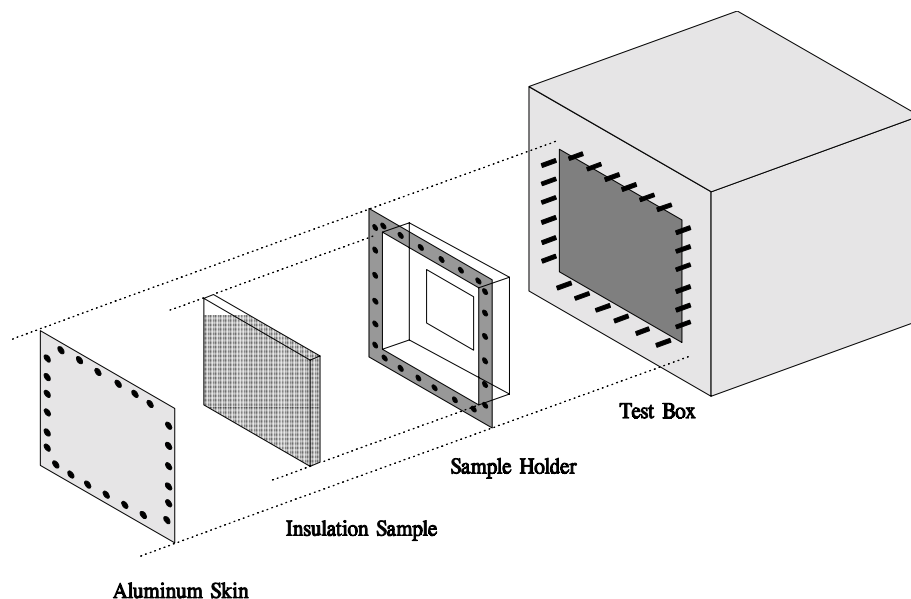
FIGURE 30. BURNTHROUGH BOX SAMPLE HOLDER
