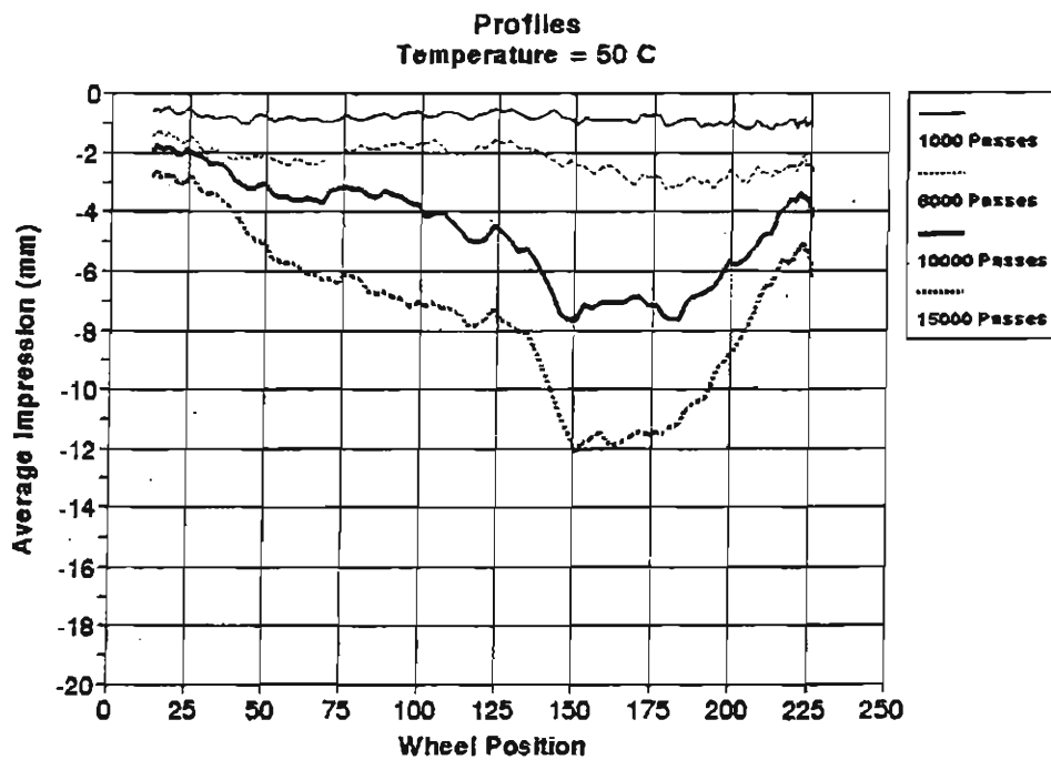
Fig. 25. Results of Field Produced HMA in the Hamburg Wheel-Tracking Device on 6th Avenue.
