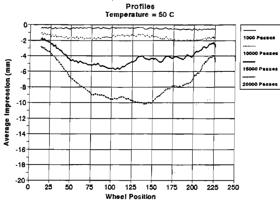
Fig. 24. Results of Lab Produced HMA in the Hamburg Wheel-Tracking Device on 6th Avenue.
