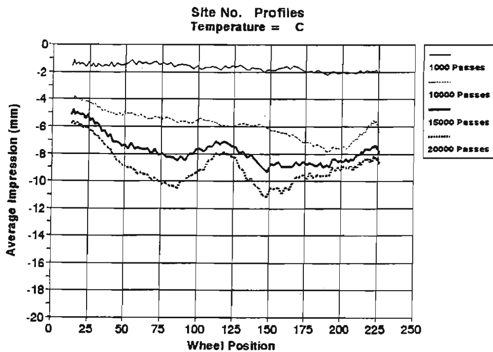
Fig. 17. Results of Field Produced HMA in the Hamburg Wheel-Tracking Device for the First 16,000 Tons on Arapahoe Road.
