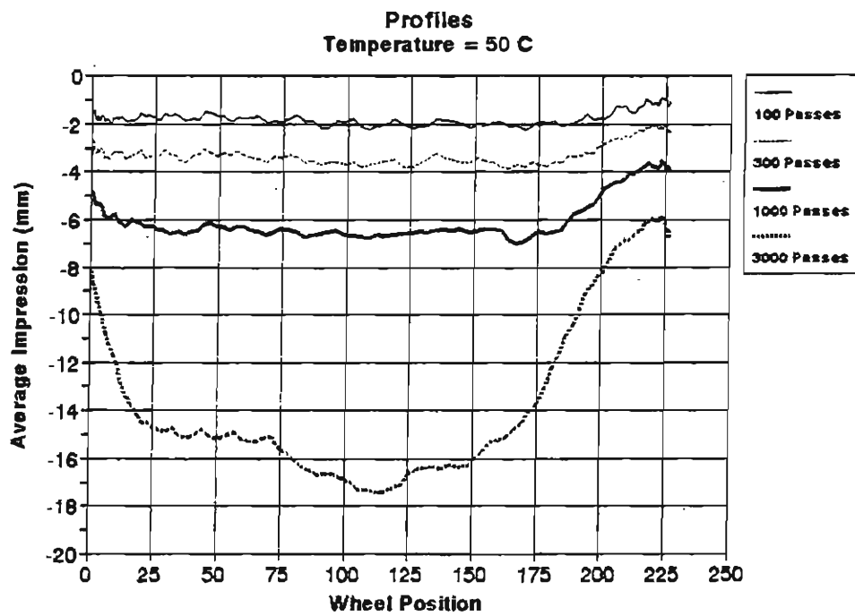
Fig. 10. Results of Field Produced HMA in the Hamburg Wheel-Tracking Device on I-70.
