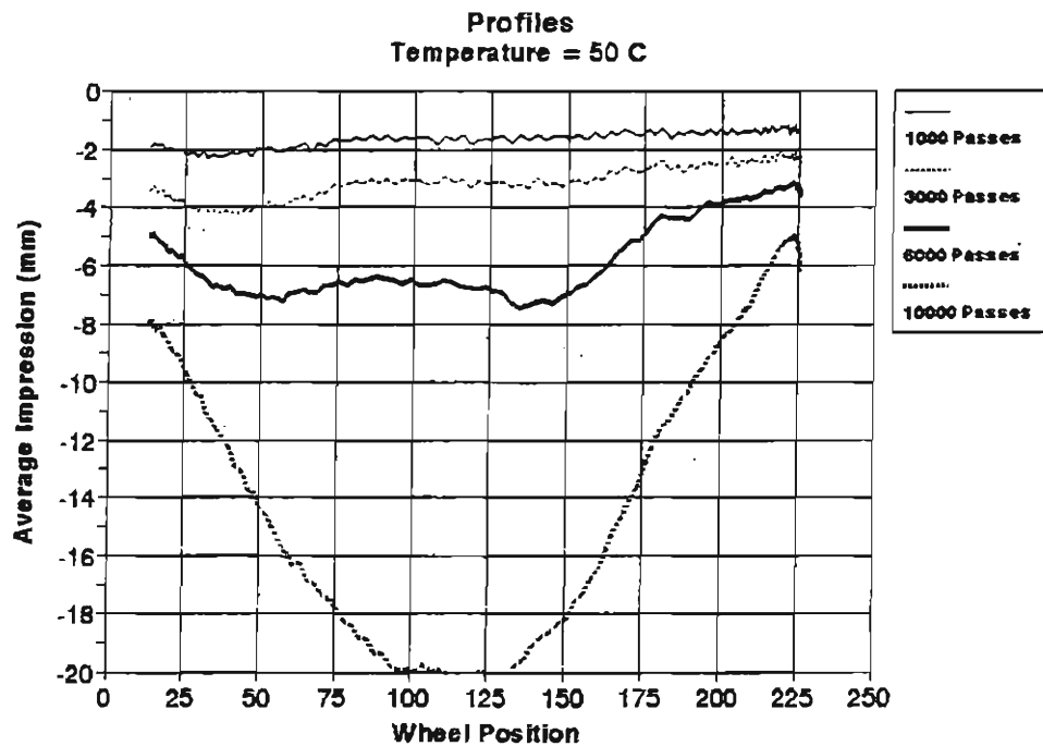
Fig. 18. Results of Field Produced HMA in the Hamburg Wheel-Tracking Device for the Final 10,000 Tons on Arapahoe Road.
