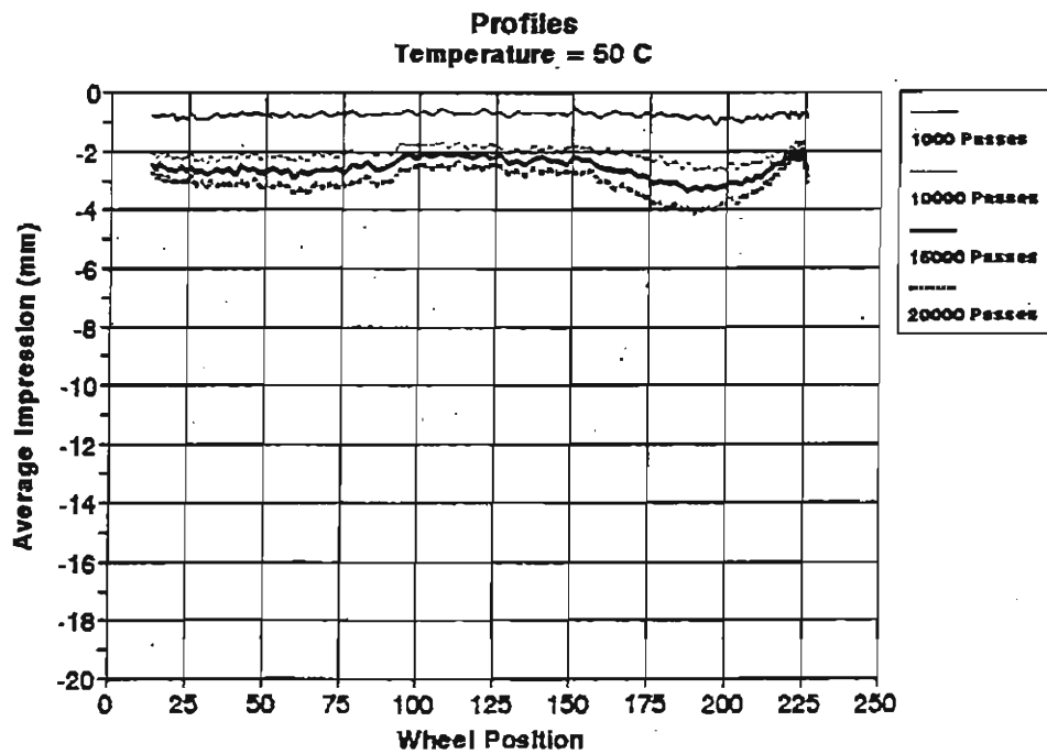
Fig. 16. Results of Lab Produced HMA in the Hamburg Wheel-Tracking Device on Arapahoe Road.
