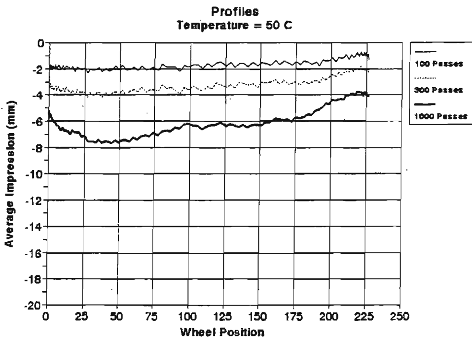
Fig. 9. Results of the Lab Produced HMA in the Hamburg Wheel-Tracking Device on I-70.
