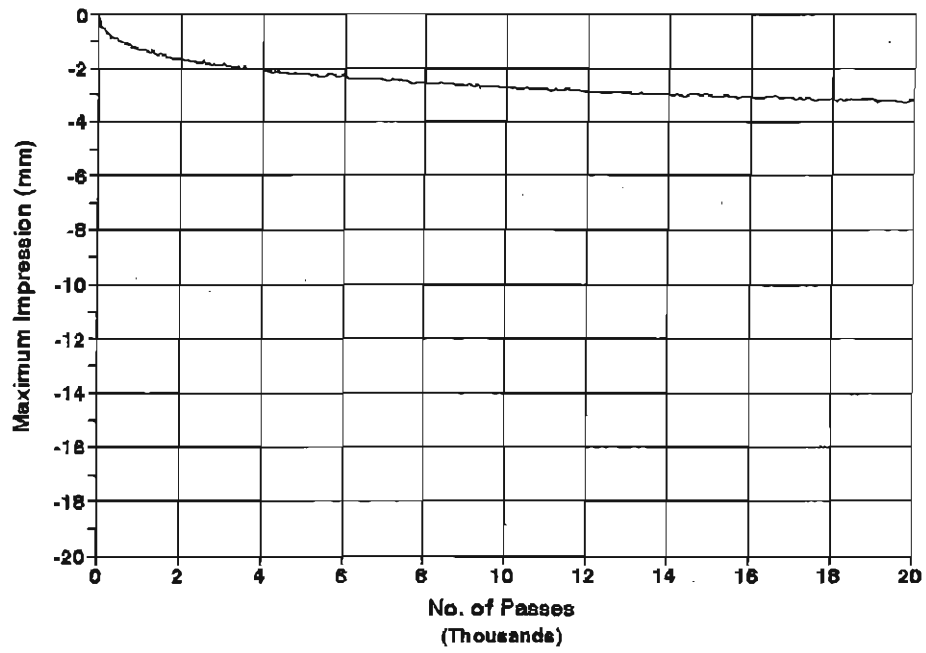
Site 5, 40-mm Thick Linear Kneading No Additional Aging
