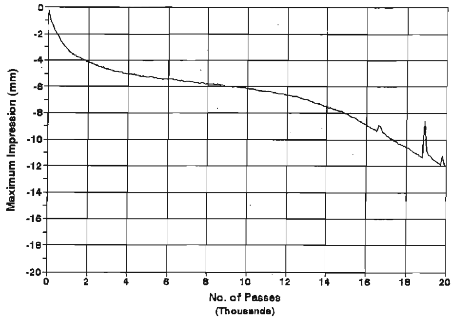
Site 6, Field Sample Temperature = 40 C
