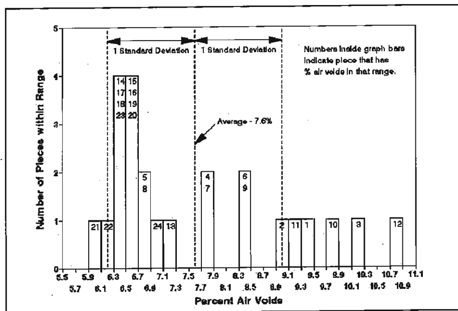
Figure 11. Typical Distribution of Air Voids in a 100-mm Thick French Compacted Sample for Site 1.
