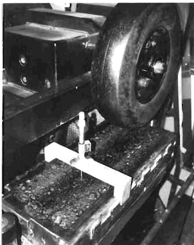
Figure 1. French Rutting Tester.
