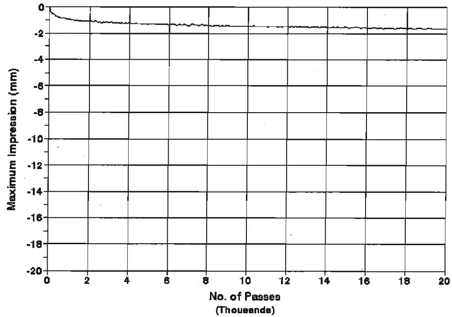
Site 7, 40-mm Thick Linear Kneading Temperature = 50 C
