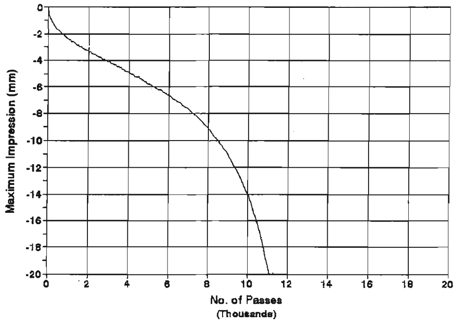
Site 5, Field Samples Temperature = 35 C
