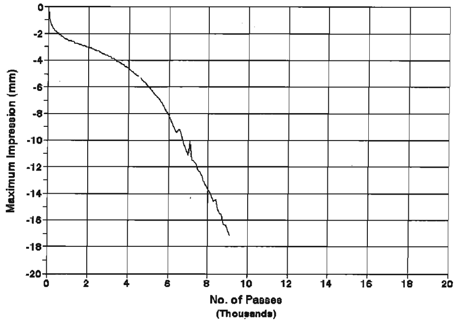
Site 1, 50-mm Thick French Samples Temperature = 50 C
