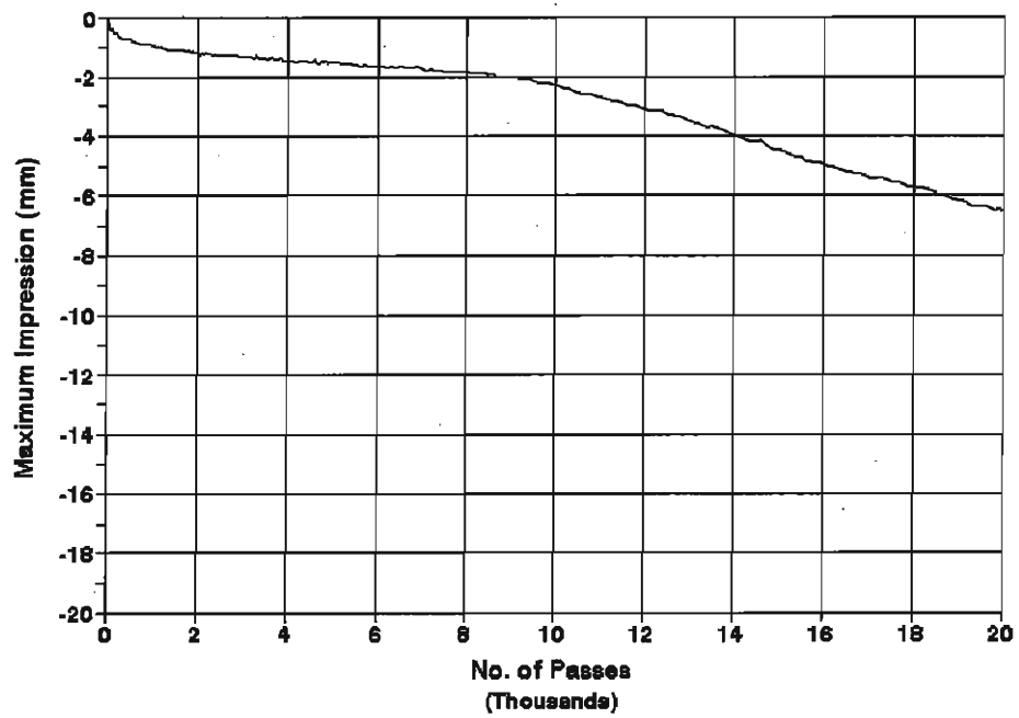
Site 4, 40-mm Thick Linear Kneading Temperature = 45 C
