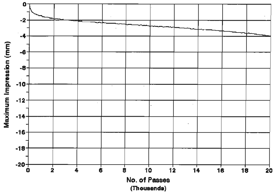
Site 7, 50-mm Thick French Sample Temperature = 50 C
