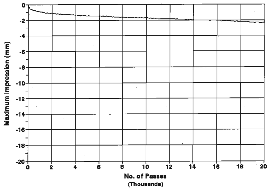
Site 3, 40-mm Thick Linear Kneading Temperature = 50 C
