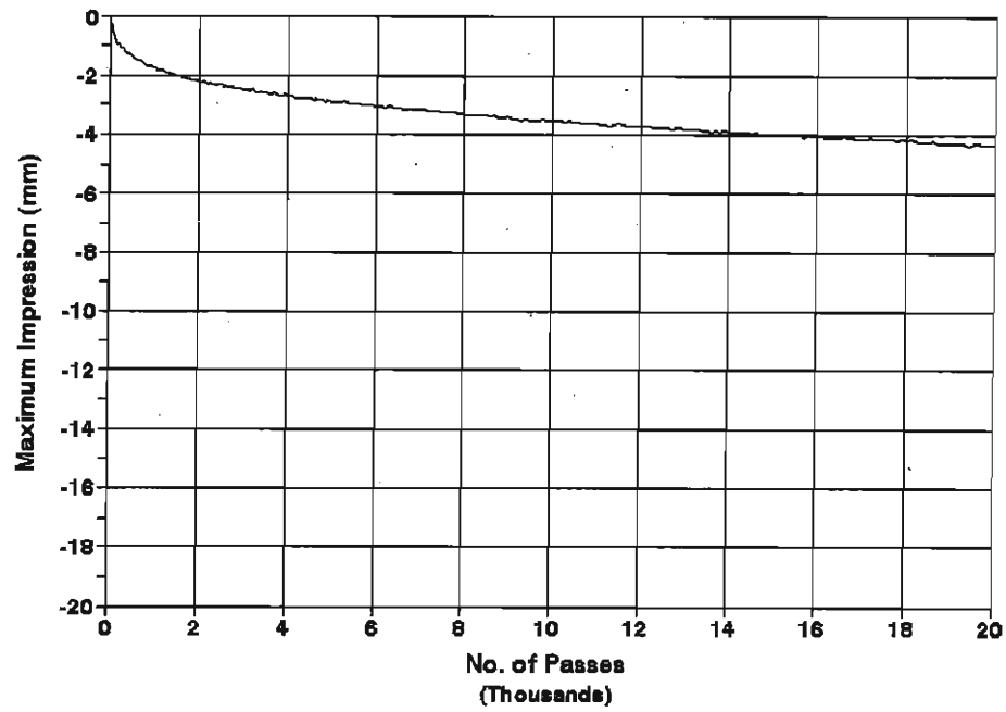
Site 5, 50-mm Thick French sample Temperature = 35 C
