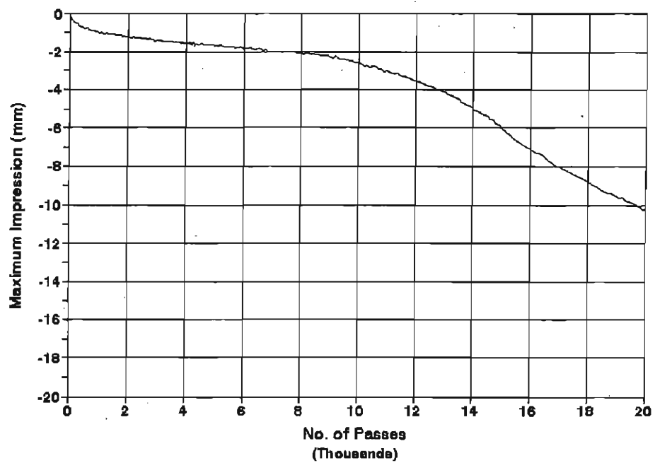
Site 4, 40-mm Thick Linear Kneading No Additional Aging
