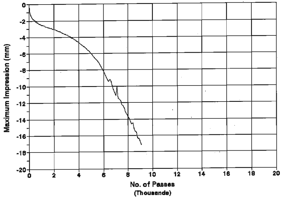
Site 3, Field Sample Temperature = 50 C
