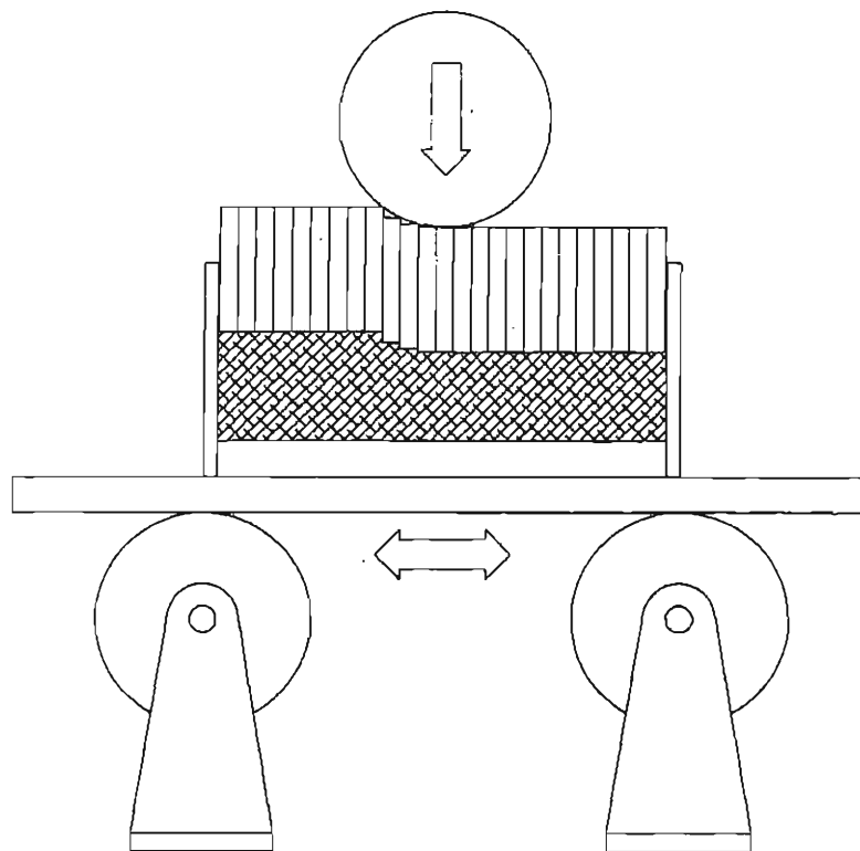
Figure 7. Schematic of the Linear Kneading Compactor.
