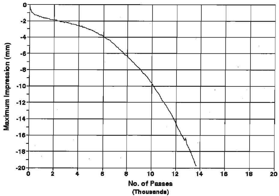
Site 1, 40-mm Thick Linear Kneading Temperature = 50 C
