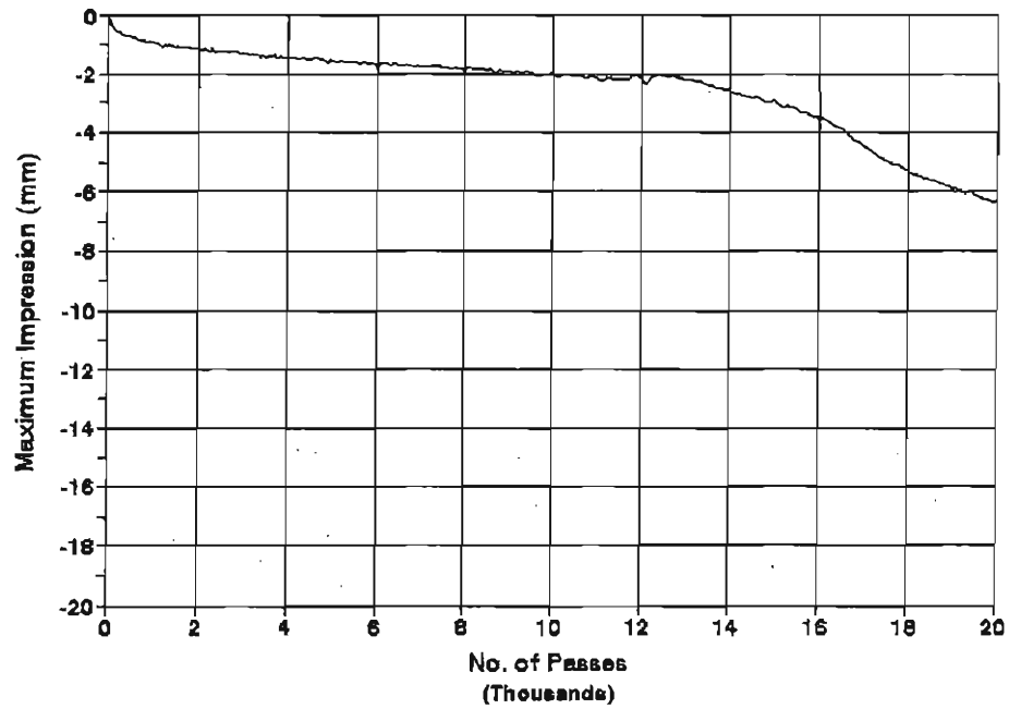
Site 7, 40-mm Thick Linear Kneading No Additional Aging
