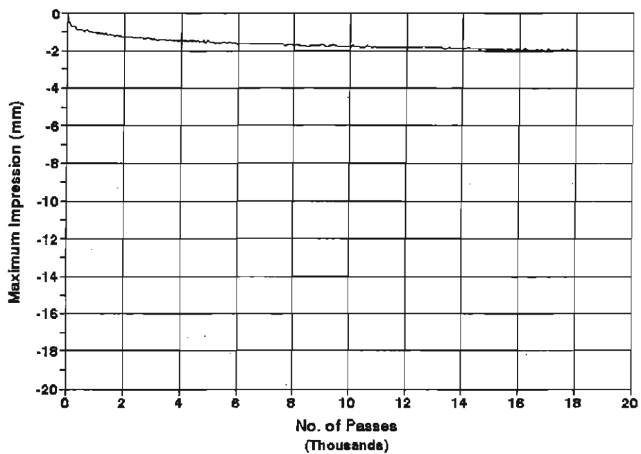
Site 6, 50-mm Thick French Sample Temperature = 40 C
