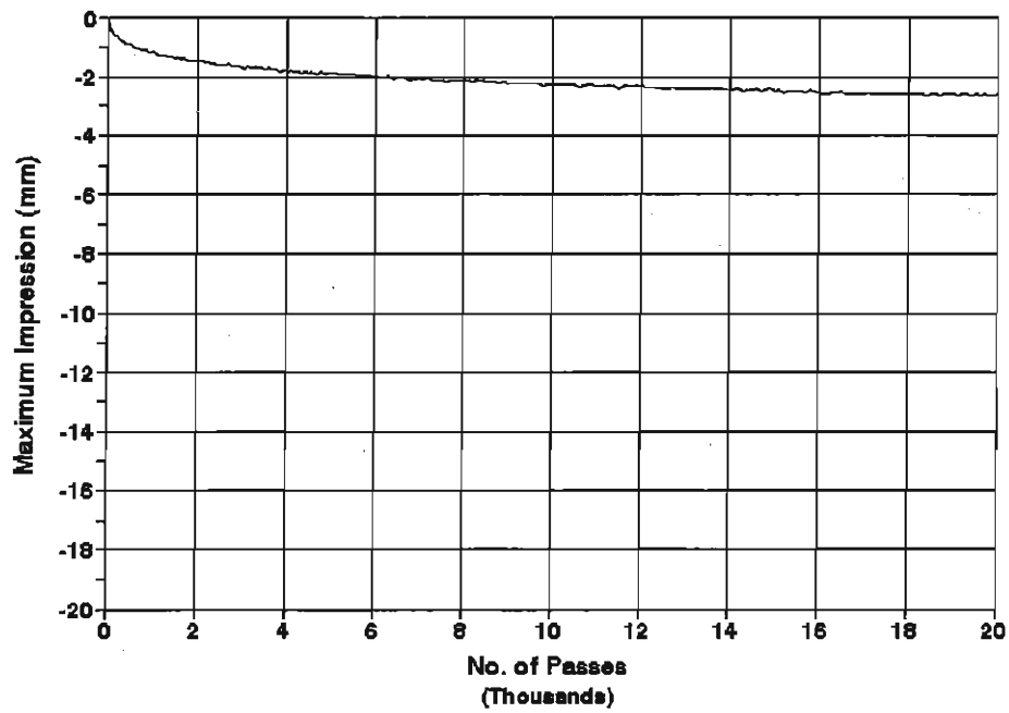
Site 5, 40-mm Thick Linear Kneading Temperature = 35 C
