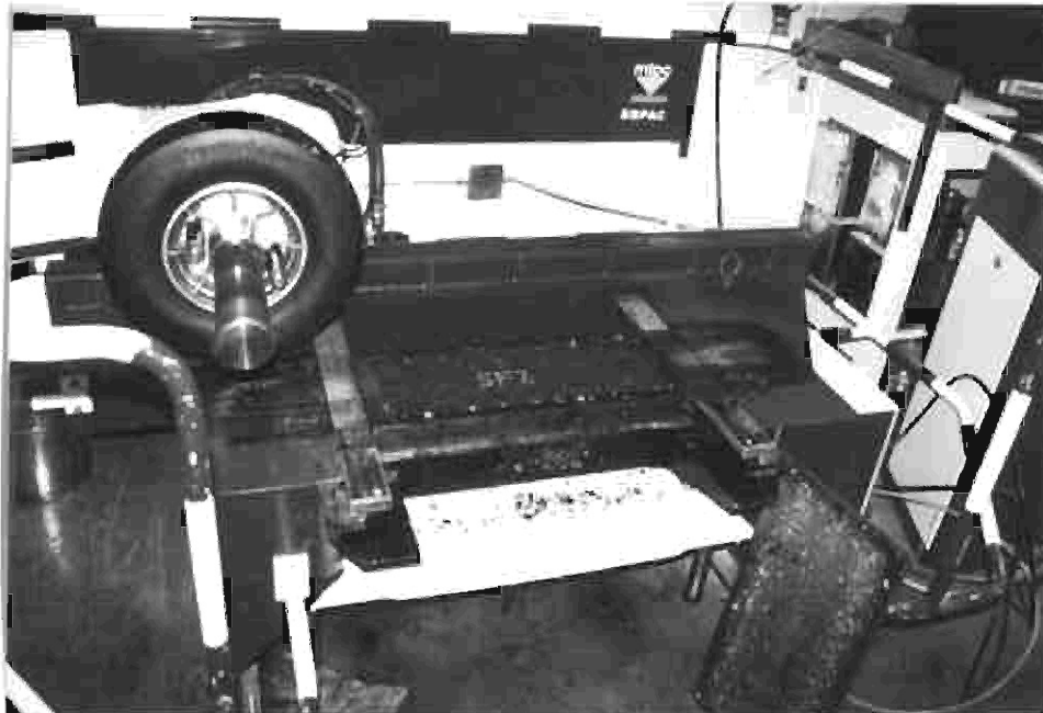
Figure 8. French Plate Compactor.
