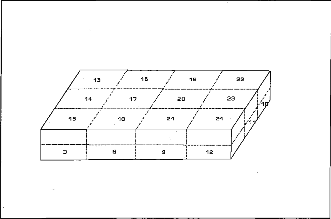
Figure 10. Layout of How 100-mm Thick French Compacted Samples Were Cut and Numbered.
