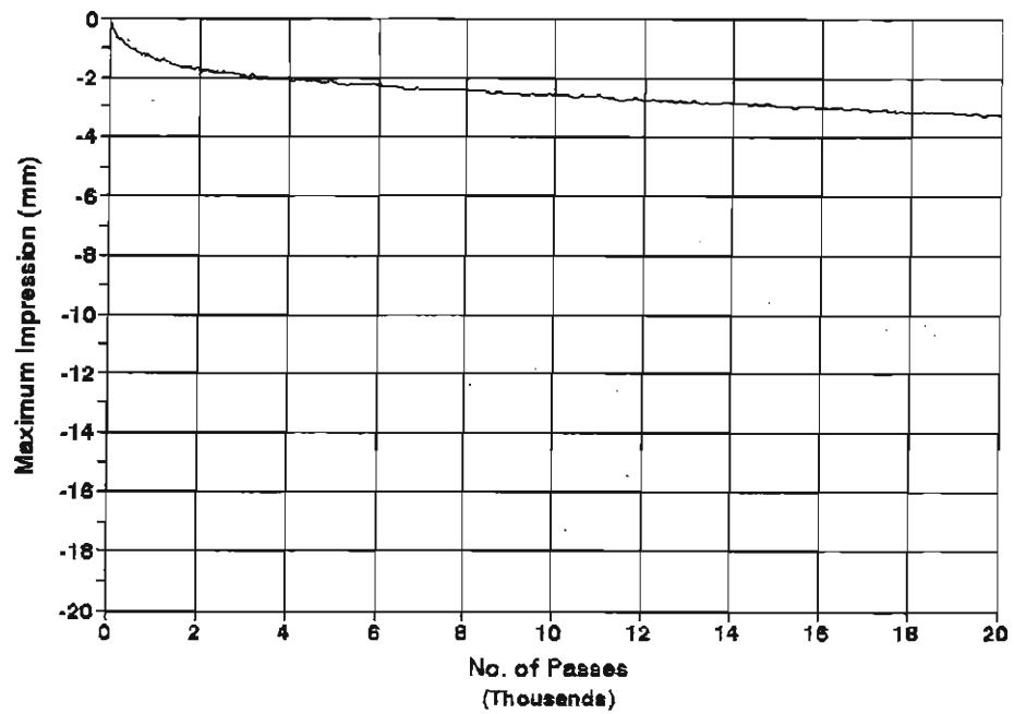
Site 2, 40-mm Thick Linear Kneading Temperature = 50 C
