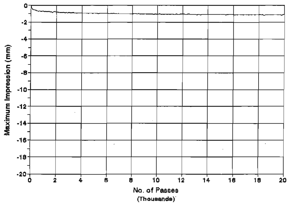
Site 6, 40-mm Thick Linear Kneading Temperature = 40 C
