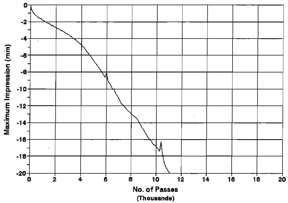
Site 2, Field Sample Temperature = 50 C
