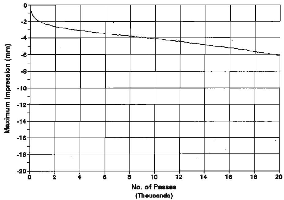
Site 3, 50-mm Thick French Sample Temperature = 50 C
