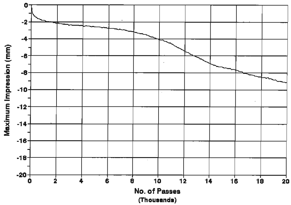
Site 4, 50-mm Thick French Sample Temperature = 45 C
