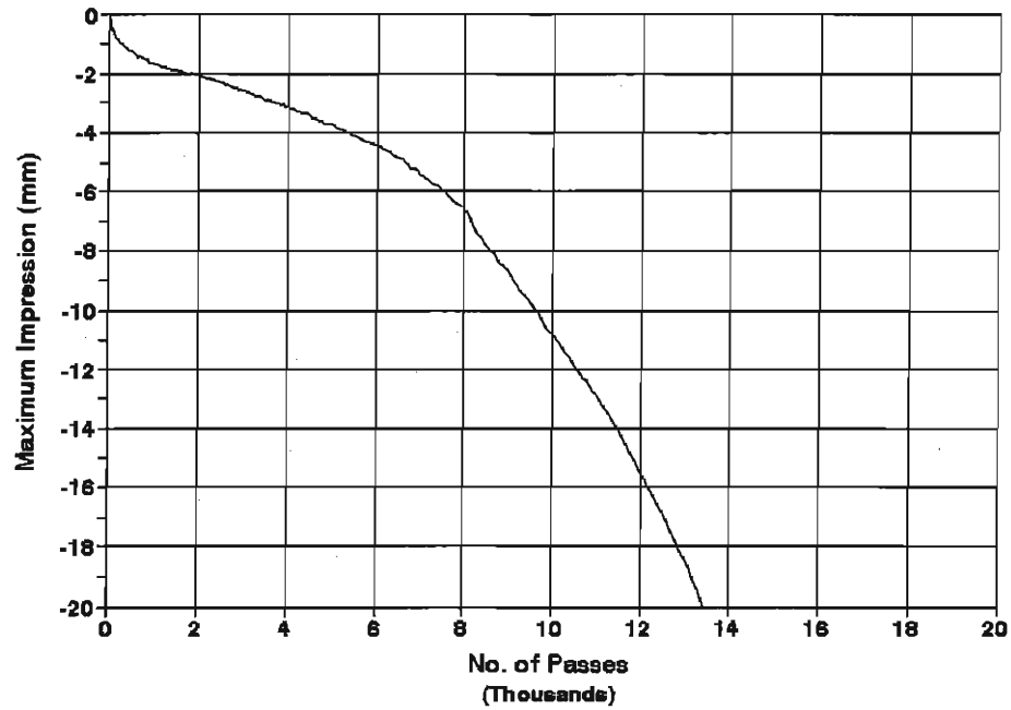
Site 3, 40-mm Thick Linear Kneading No Additional Aging
