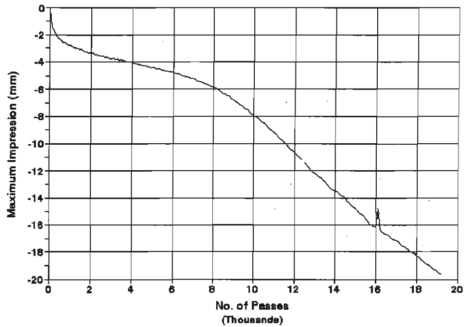
Site 2, 50-mm Thick French Sample Temperature = 50 C
