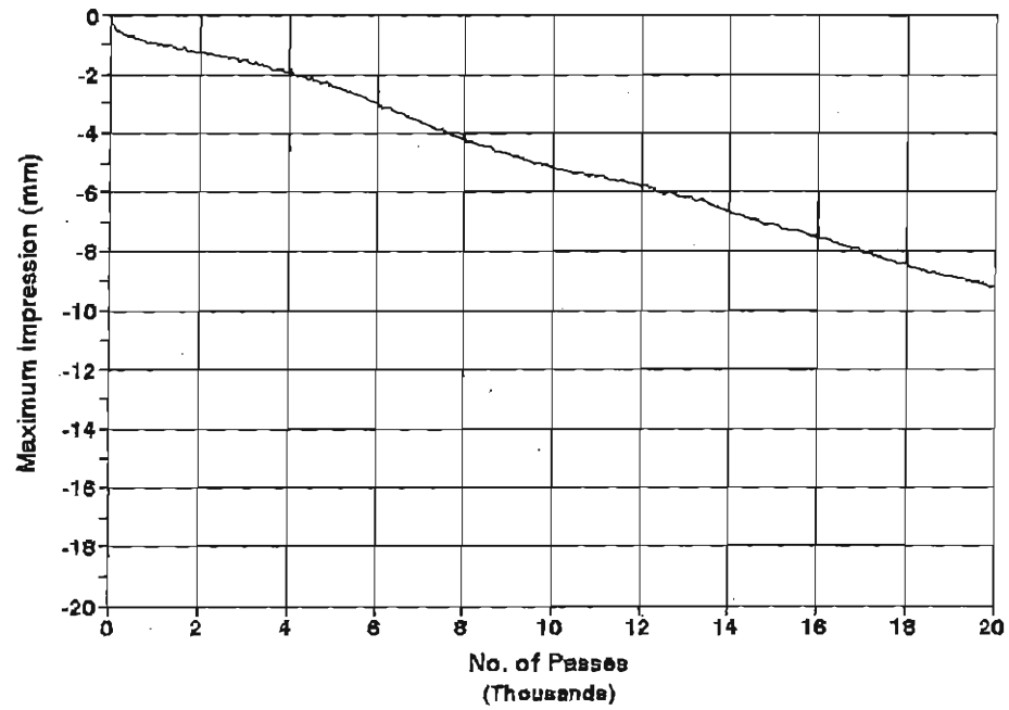
Mix3, 121 C compaction Test Temperature = 45 C
