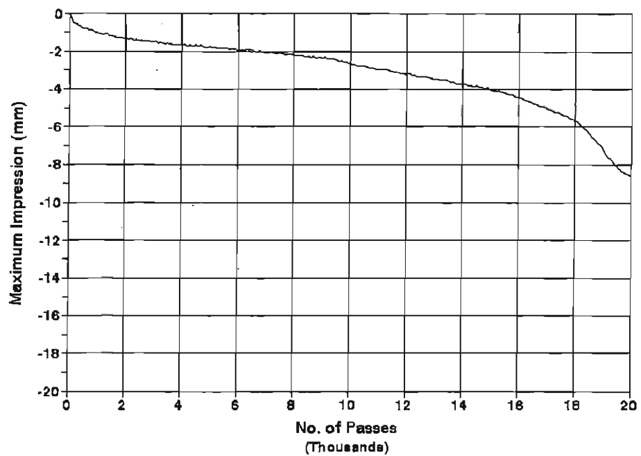
Mix4, 93 C Compaction Test Temperature = 45 C
