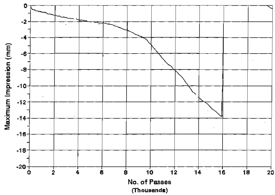
Mix3, Additive B, Type1 Test Temperature = 45 C
