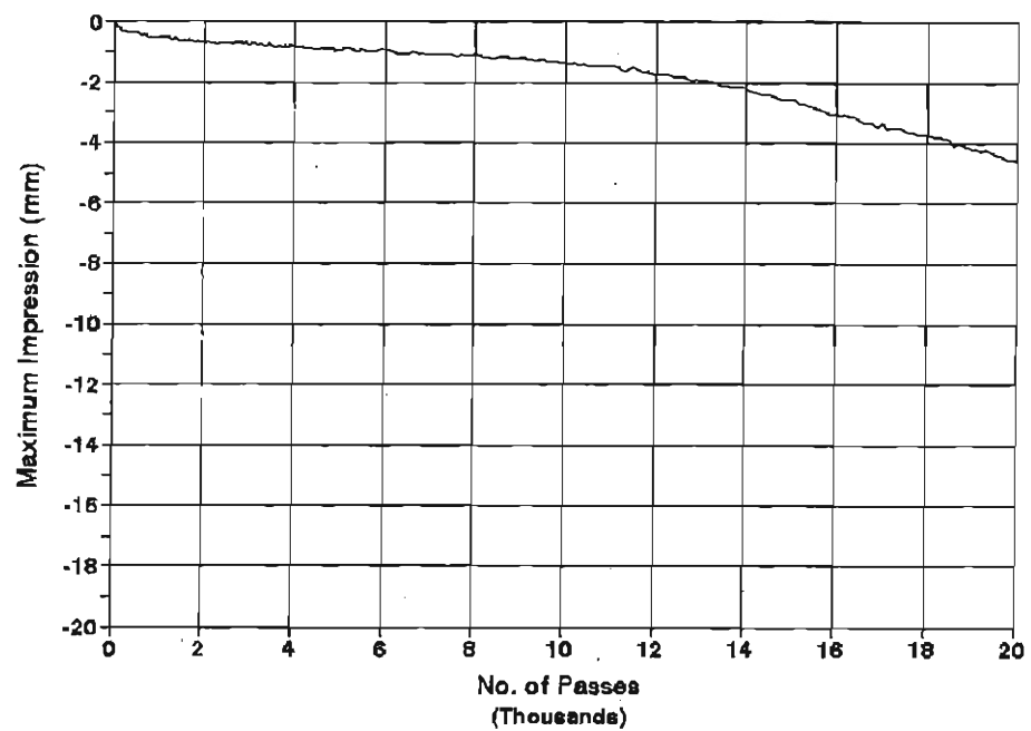
Mix4, Additive A, Type2 Test Temperature = 45 C
