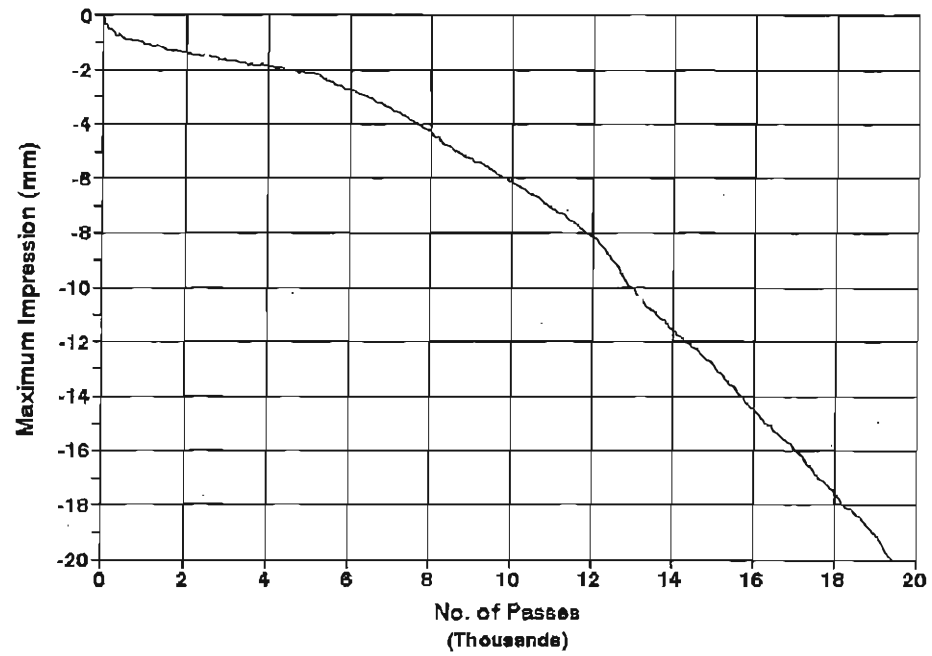
Mix3, 93 C Compaction Test Temperature = 45 C
