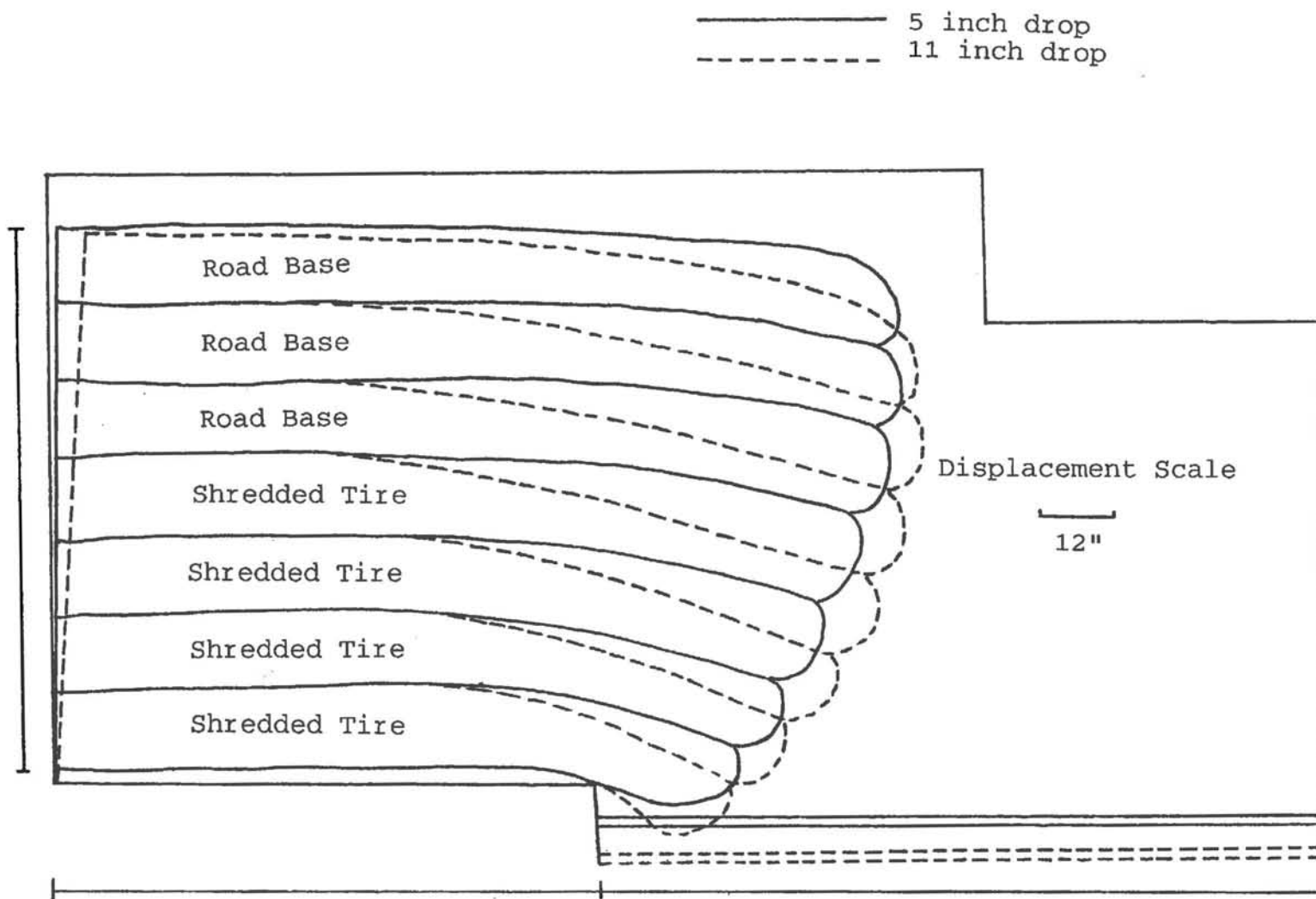
Figure 4.6 Displacement Field of the CTI Deep Patch Test with Shredded Tire Backfill
