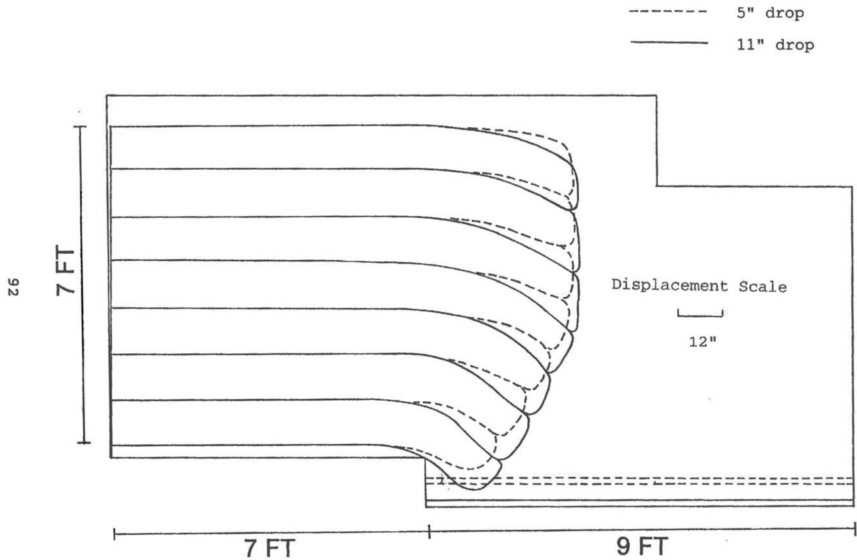
Figure 3.4 Displacement Field of the Backfill in the CTI Deep Patch Test with Road Base Backfill
