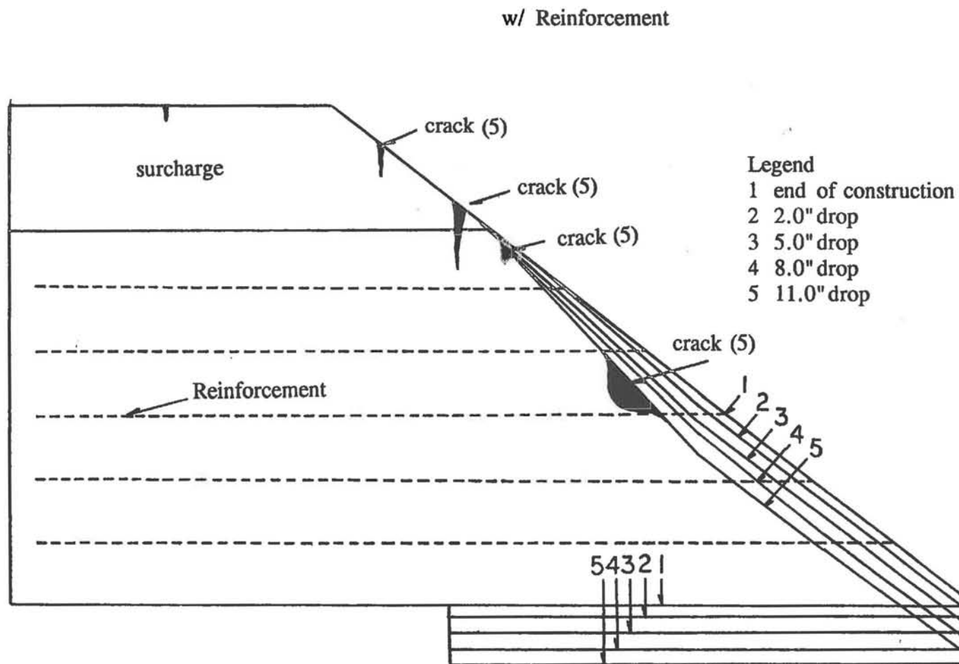
Figure 2.34 Displacement Field of the Backfill in the Reinforced USFS Deep Patch Test
