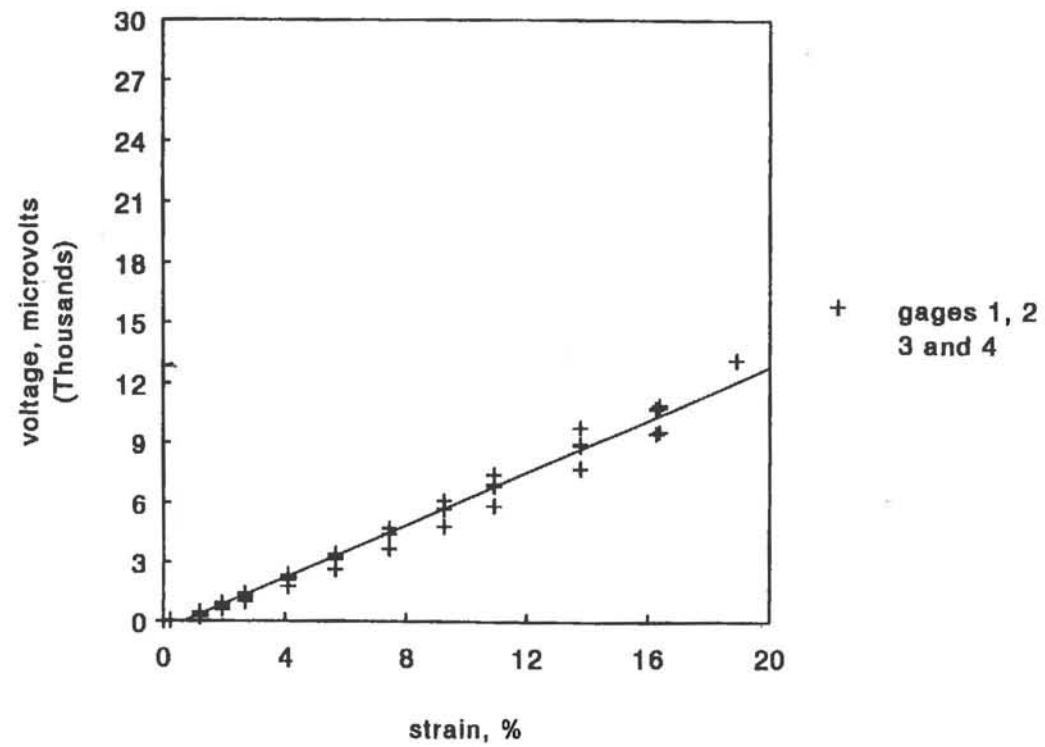
Figure 2.27 Calibration Curve for Strain Gage
