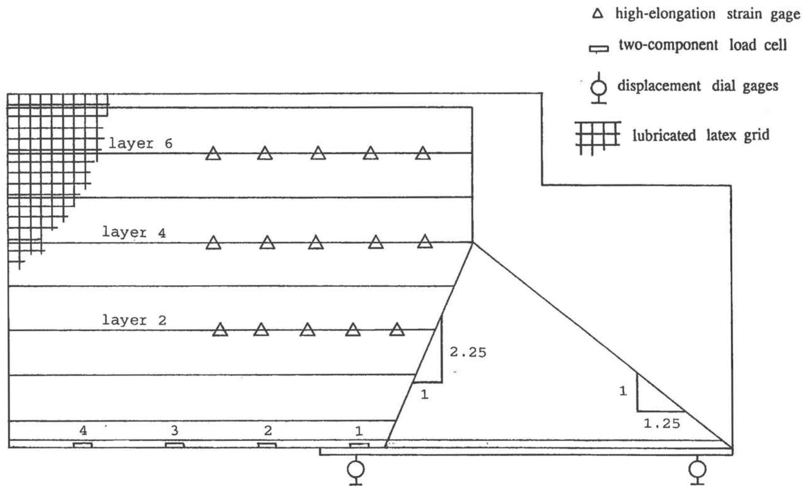
Figure 3.3 Instrumentation of the CTI Deep Patch Test
