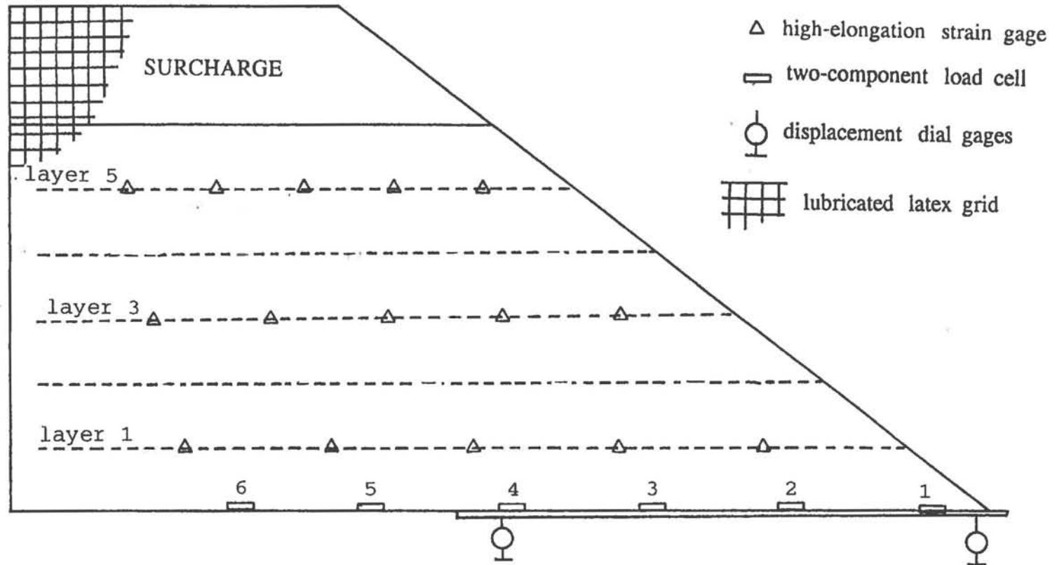
Figure 2.14 Instrumentation of the USFS Deep Patch Test
