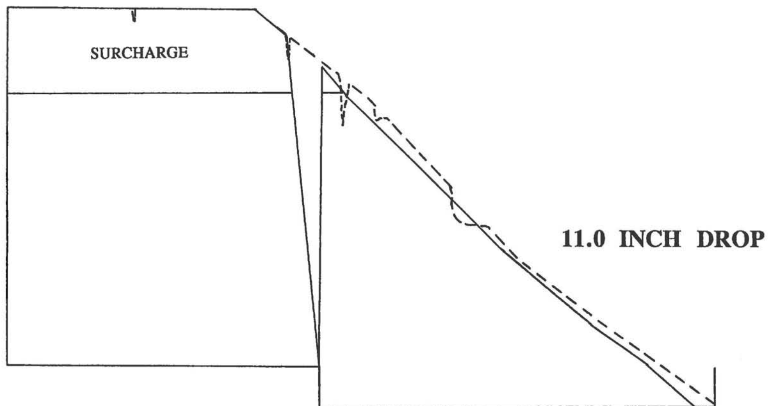
Figure 2.35(d) Comparison of Crack Propagation in the Two Tests at 11 inch-Drop
