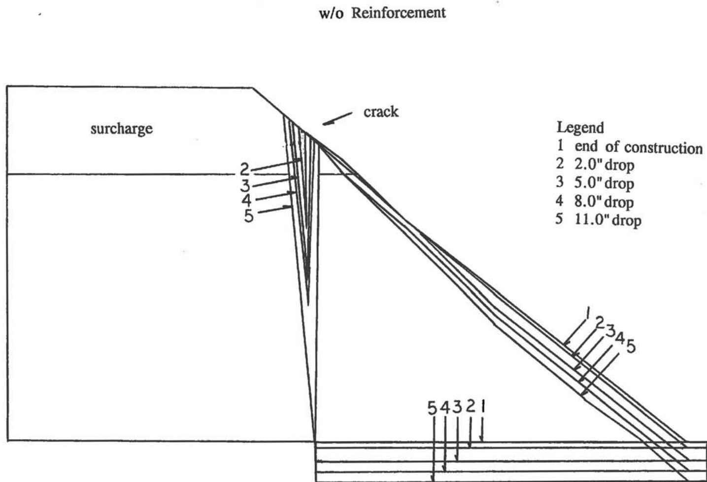
Figure 2.32 Displacement Field of the Backfill in the Unreinforced USFS Deep Patch Test
