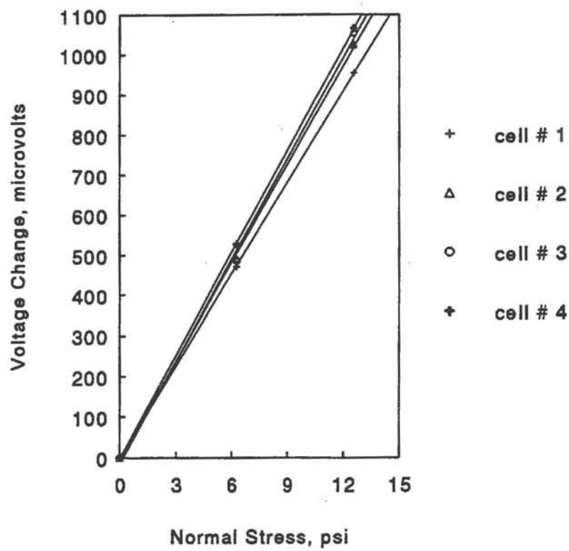
Figure 2.20 Normal Stress Calibration Curves for Load Cell
