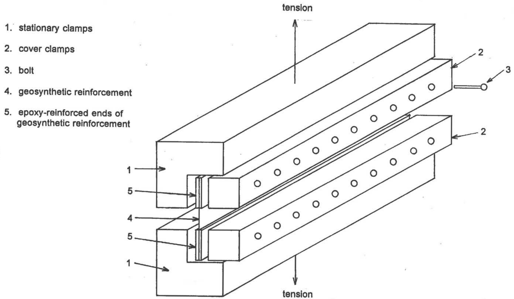
Figure 2.6 Schematic Diagram of the Uniaxial Load-Deformation Apparatus
