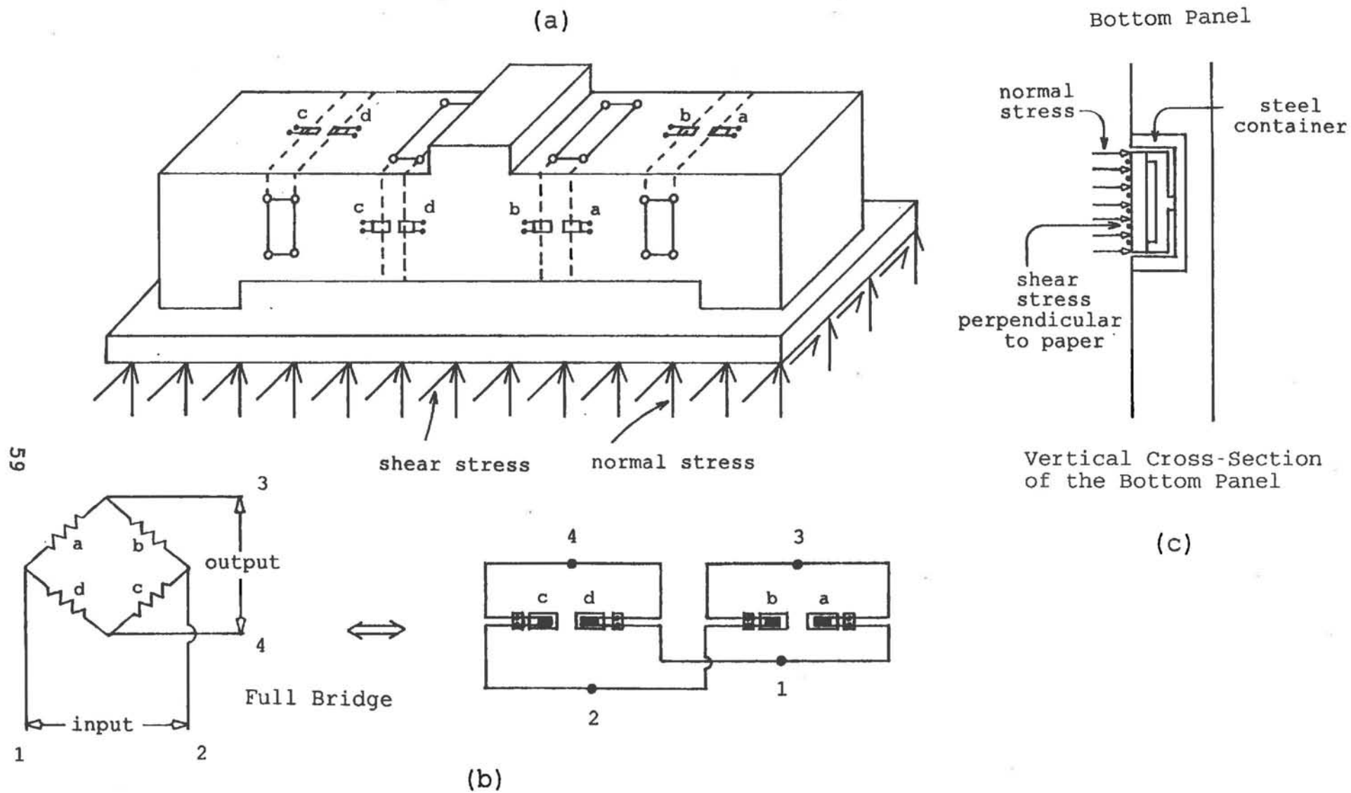
Figure 2.15 Schematic Diagram of the Two-Component Load Cell
