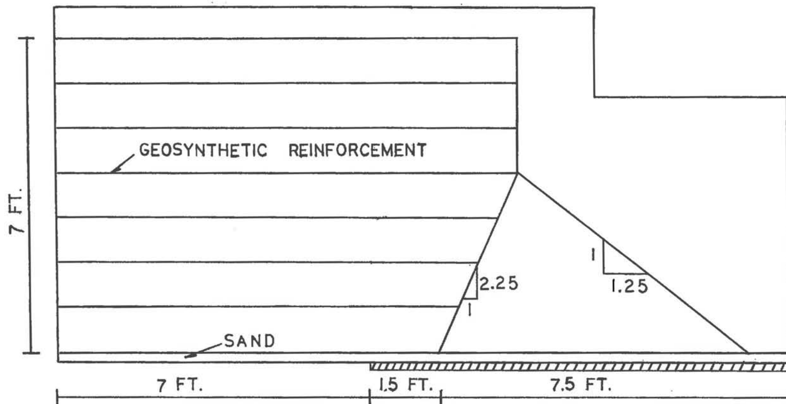
Figure 3.1 Schematic Diagram of the CTI Deep Patch Test
