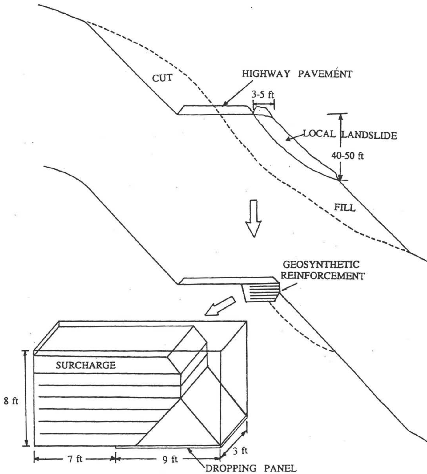
Figure 1.2 Schematic Diagram of the CTI Deep Patch Technique
