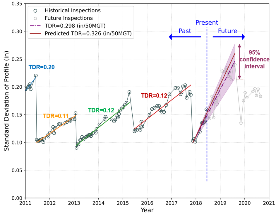
Figure 27. The application of the proposed ML model on a block as an example.
