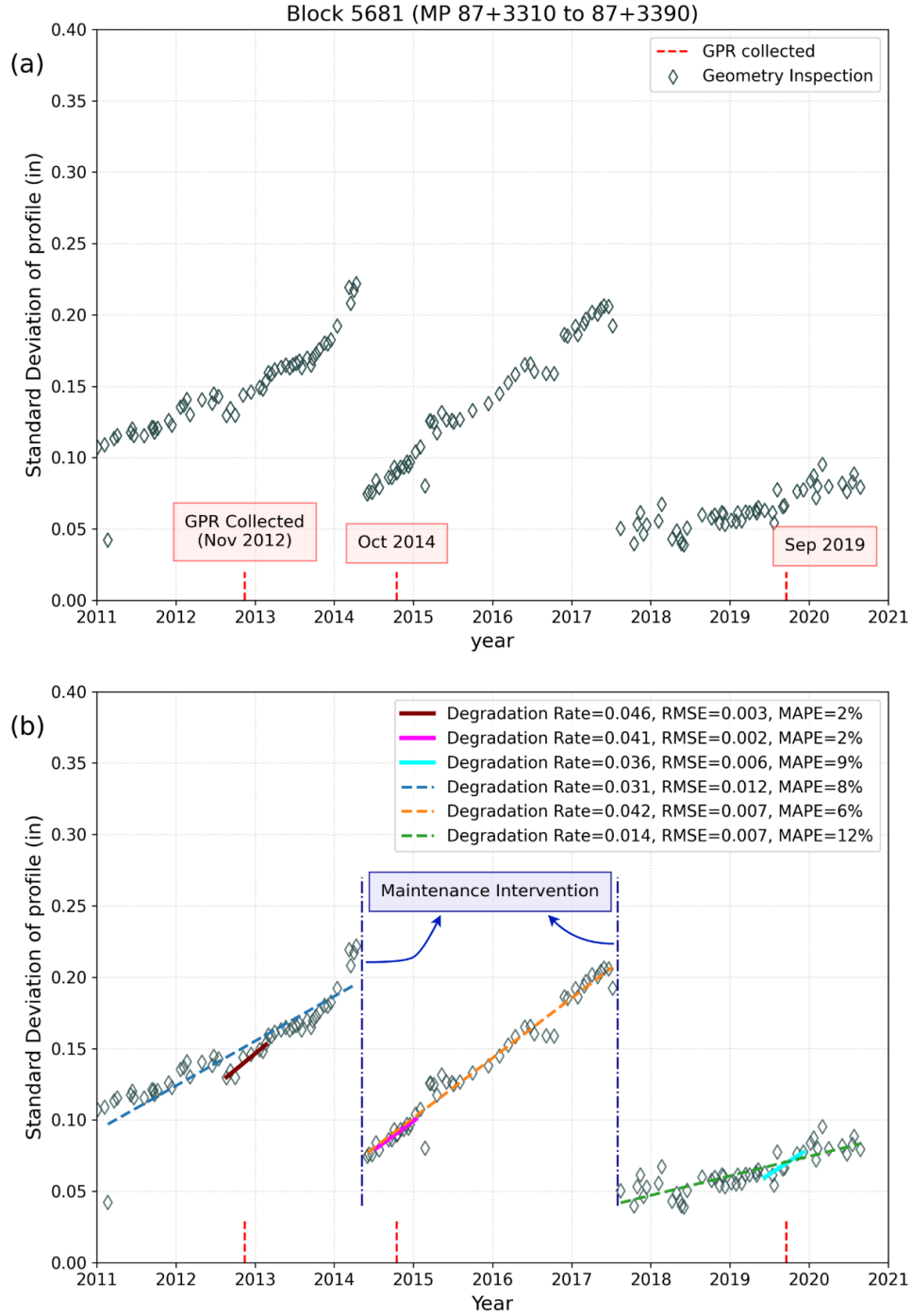
Figure 1. An example of studied profile geometry data of a block: (a) SD of profile for different geometry inspections vs. time and dates of collecting GPR, (b) fitted linear regression models to calculate track degradation rates.
