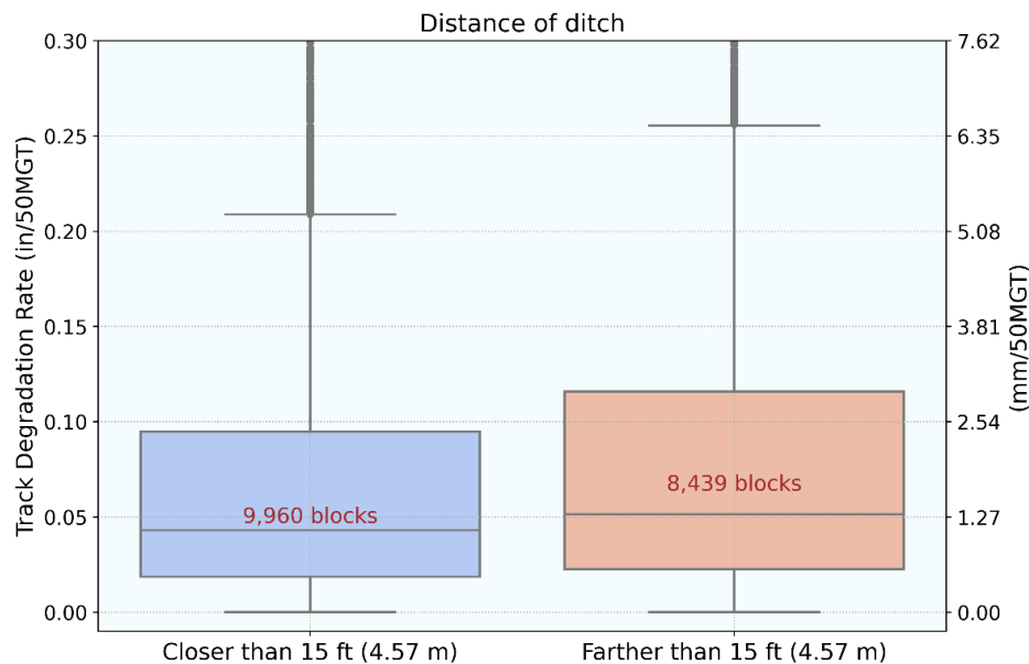
Figure 17. Effect of ditch distance from center of track on TDR.
