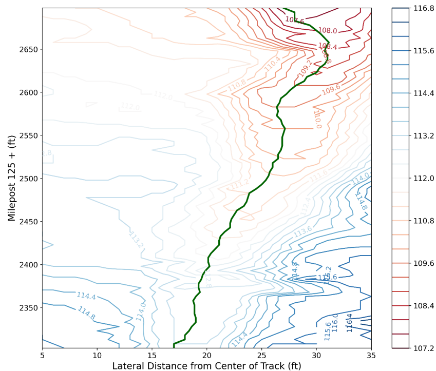
Figure 21. Topography contour lines at a milepost; the ditch location is automatically determined using LiDAR data and depicted by a green line. Note that this figure is not a geospatial map, but rather an indication of elevations at a distance from the centerline of track. It is also important that this figure is independent of the variations in alignment of the track.
