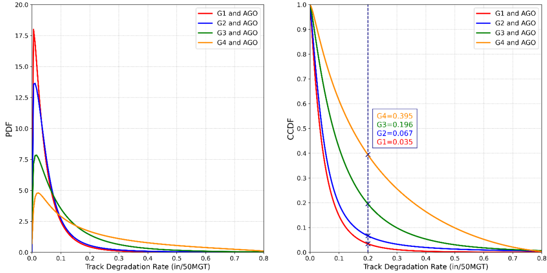
Figure 12. Effect of subsurface conditions on track degradation rates.
