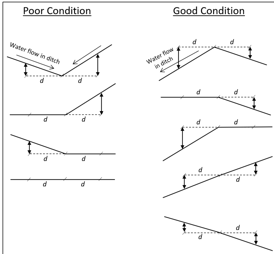
Figure 20. Schematic representation of longitudinal condition of ditch; in poor longitudinal drainage, water accumulates in the ditch, while in good longitudinal drainage, water flows freely.
