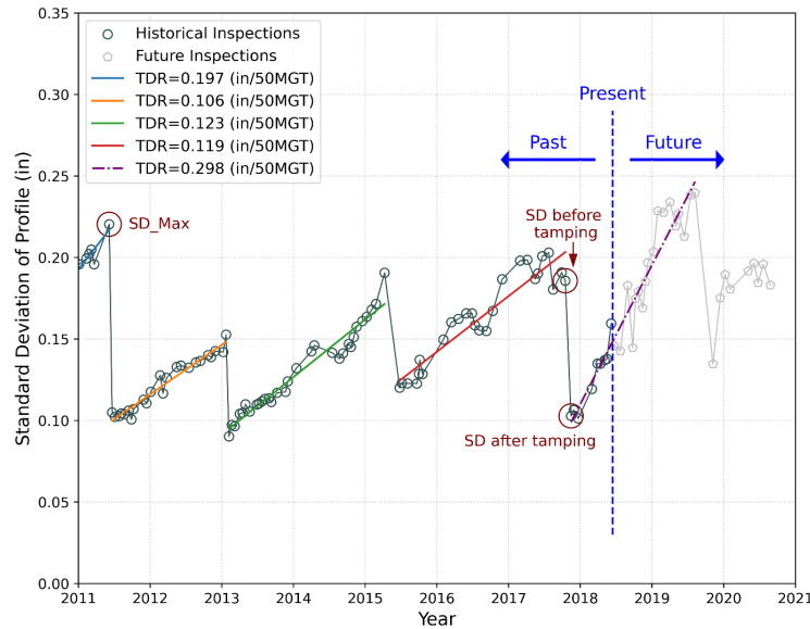
Figure 14. An example of SD vs time for a block. The goal of prediction models is to predict the TDR in current cycle, which is the slope of dotted purple line.
