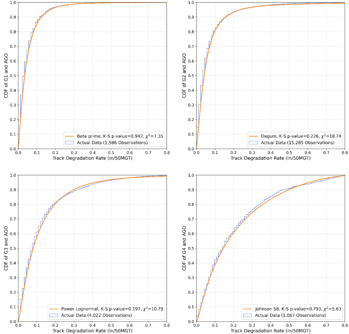
Figure 10. CDF of actual data and the best fitted distribution of categories from clean ballast (G1) to highly fouled ballast (G4) and AGO cross-section.
