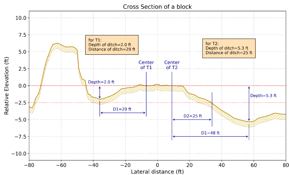
Figure 15. Cross section of a block as an example to show depth and distance of ditch; Distance of ditch is minimum value between D1 and D2.
