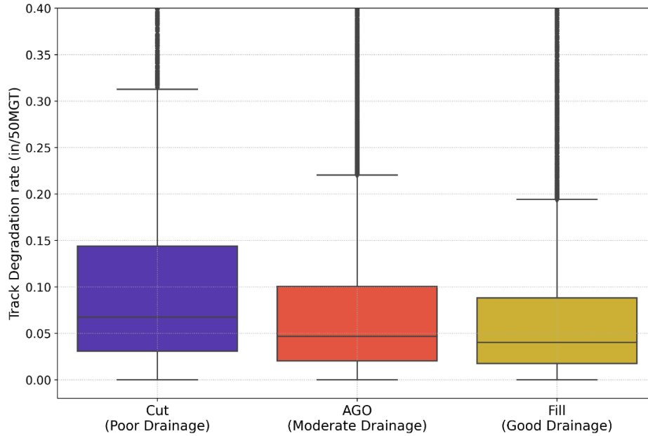
Figure 7. Box plot of track degradation rate with respect to drainage conditions.
