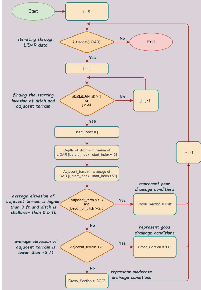
Figure 5. Flowchart for evaluating drainage and cross section condition from LiDAR data.
