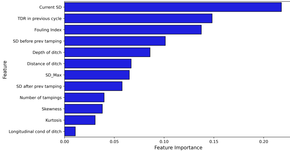
Figure 28. The importance of features for predicting TDR using the XGBoost model.
