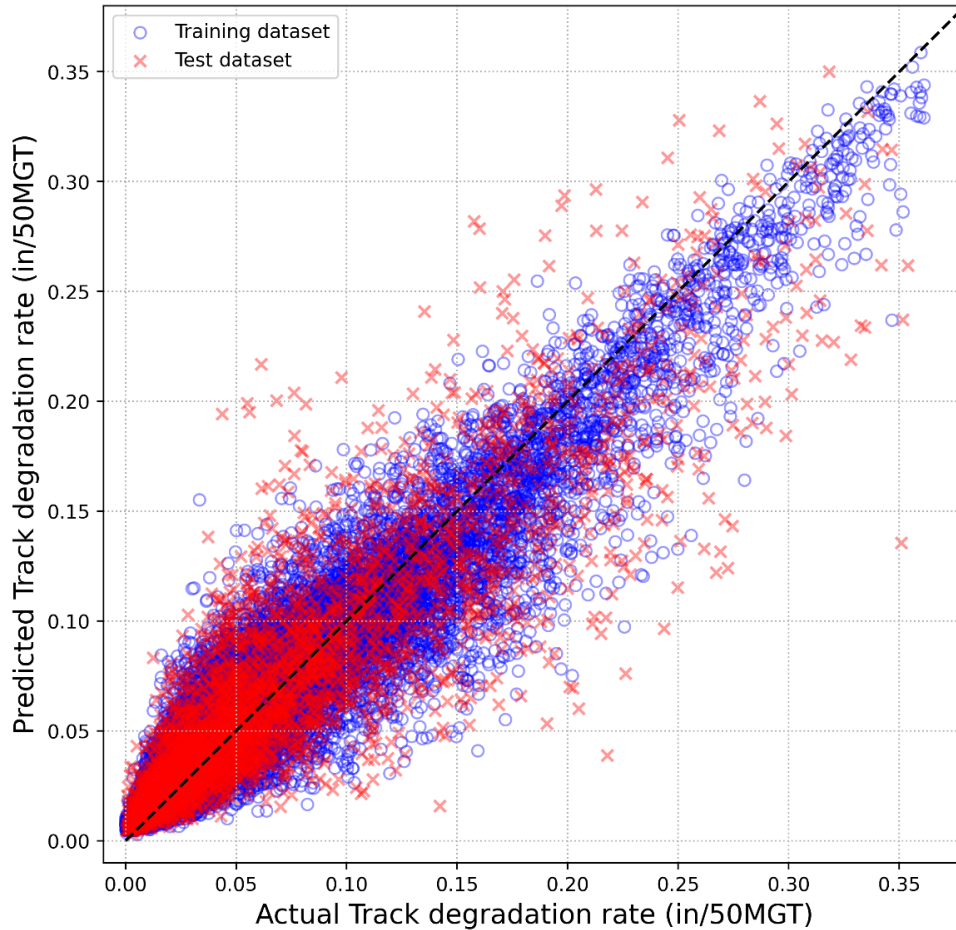
Figure 24. Scatter plot of predicted TDR vs. actual TDR values using XGBoost prediction model.
