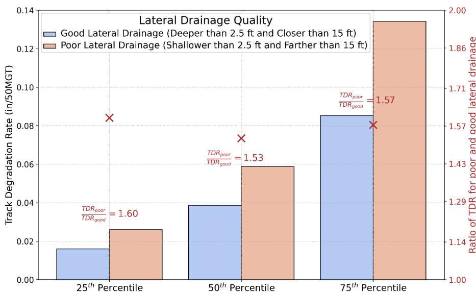
Figure 19. Comparing TDR for good and poor lateral drainage quality across different percentiles; the ratio of TDR for poor and good lateral drainage is shown by maroon “x” mark and is around 1.55 for different percentiles.
