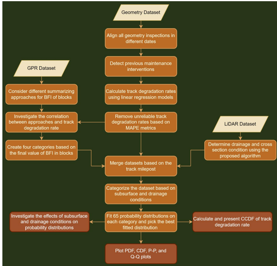
Figure 8. Flowchart diagram of approach for stochastic analysis of track degradation rate.
