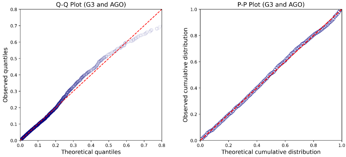
Figure 11. Q-Q and P-P plots of category “G3 and AGO,” which has the lowest K-S p-value among categories.
