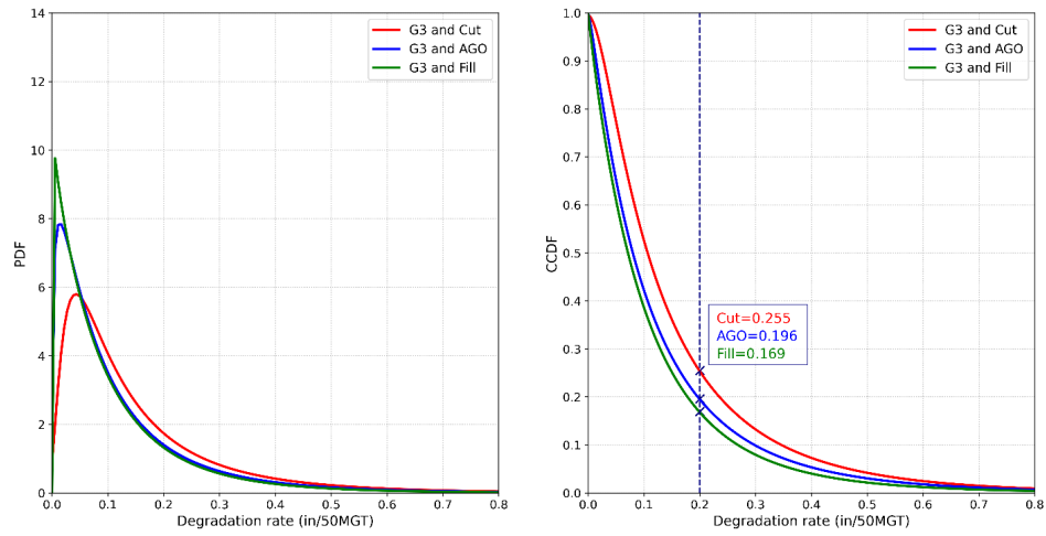
Figure 13. Effect of drainage and cross-section conditions on track degradation rates.
