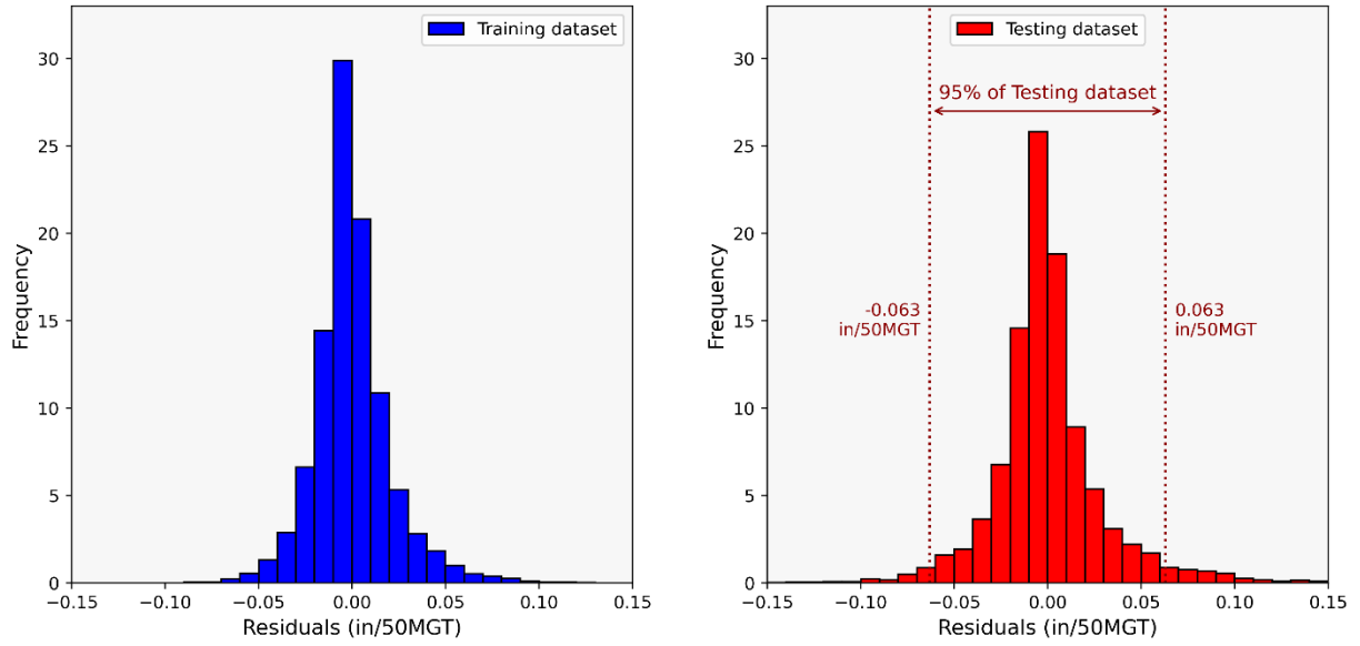
Figure 26. Histograms of residuals for both the training and testing datasets.
