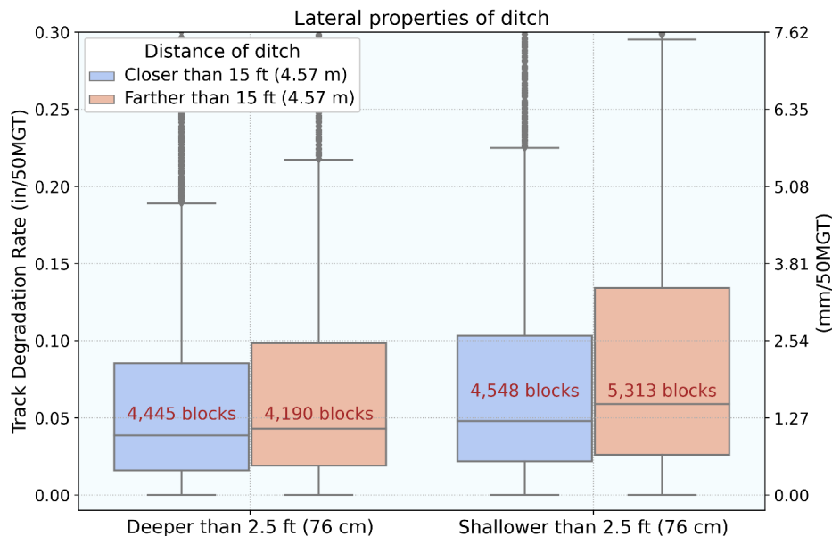
Figure 18. The boxplot of TDR considering both distance and depth of ditch; the effect of ditch distance is more significant when the ditch is shallow.
