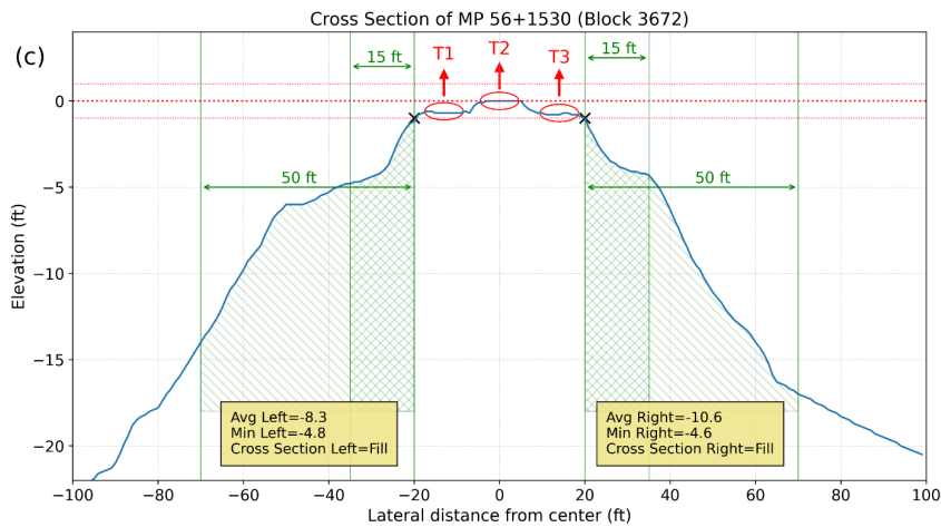
Figure 6. Applications of the proposed algorithm for determining cross-section and drainage condition of tracks; (a) typical cut cross-section (poor drainage condition) for all three tracks; (b) typical AGO cross section (moderate drainage condition); (c) typical fill cross section (good drainage condition); (d) cut cross-section for right terrain and AGO cross-section for left terrain due to existence of a good ditch.
