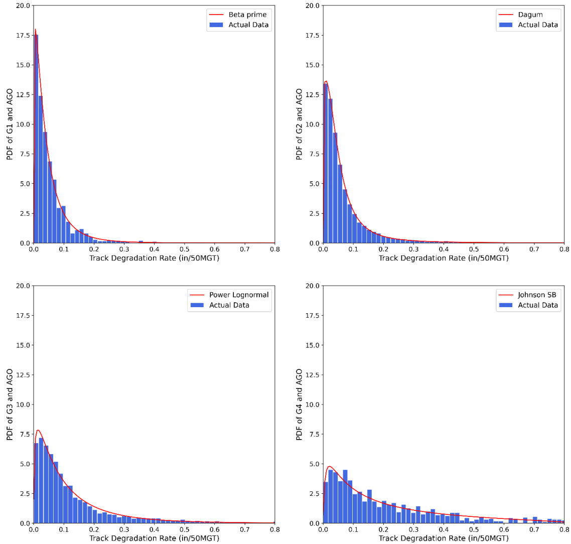
Figure 9. Histograms and the best fitted distributions of categories from clean ballast (G1) to highly fouled ballast (G4) and AGO cross-section.
