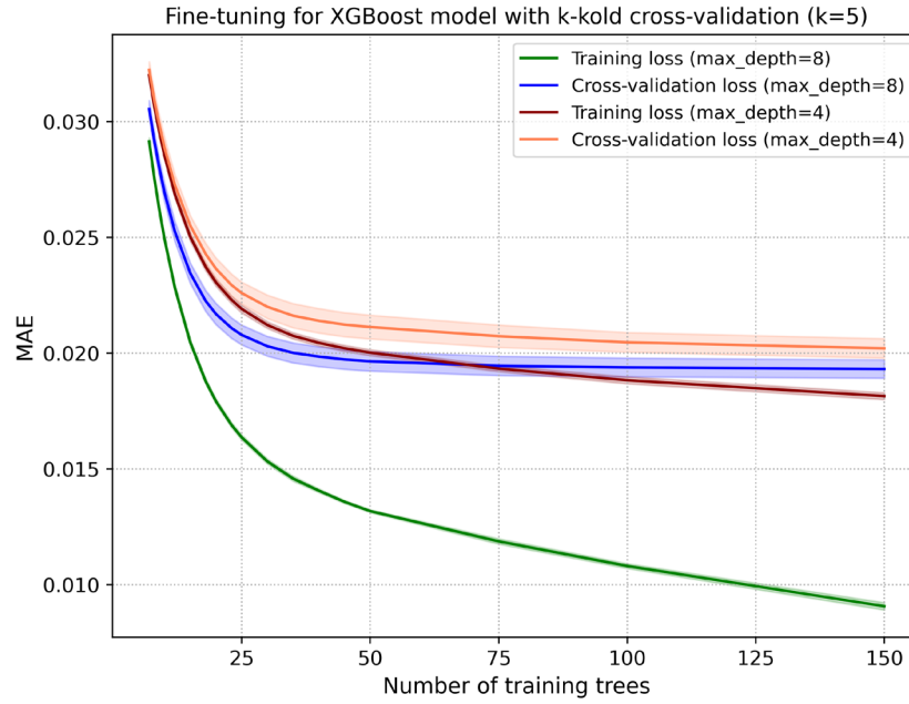
Figure 23. Fine-tuning the number of trees and maximum depth for the XGBoost model.
