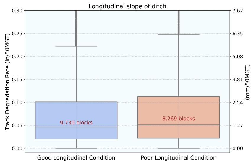
Figure 22. The effect of longitudinal drainage condition on TDR.
