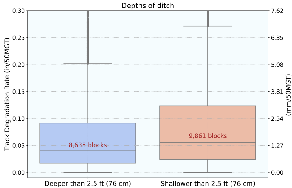
Figure 16. Effect of ditch depth on TDR.
