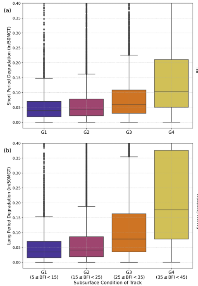
Figure 4. Box plot of track degradation rate with respect to subsurface conditions; (a) short period degradation; (b) long period degradation.
