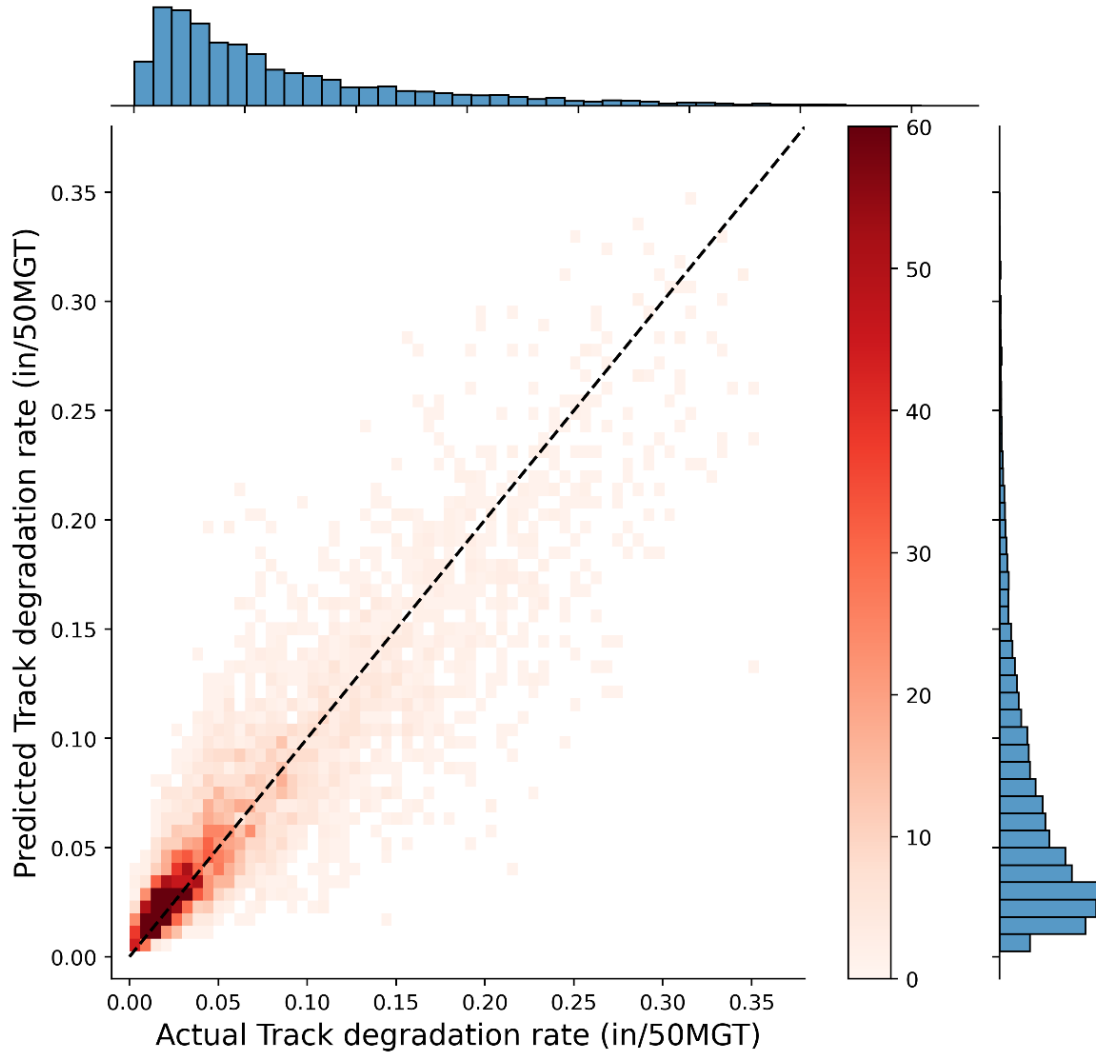
Figure 25. Concentration of data points for predicted TDR vs actual TDR in the test dataset, utilizing the XGBoost prediction model.
