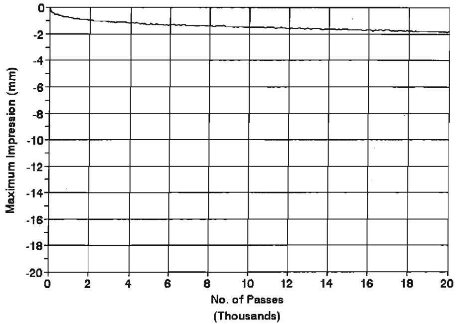
SITE6 L4 Temperature = 50 C
