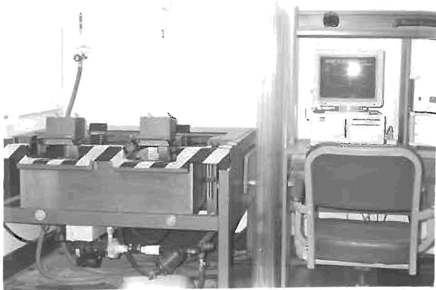
Figure 1. The Hamburg Wheel-Tracking Device
