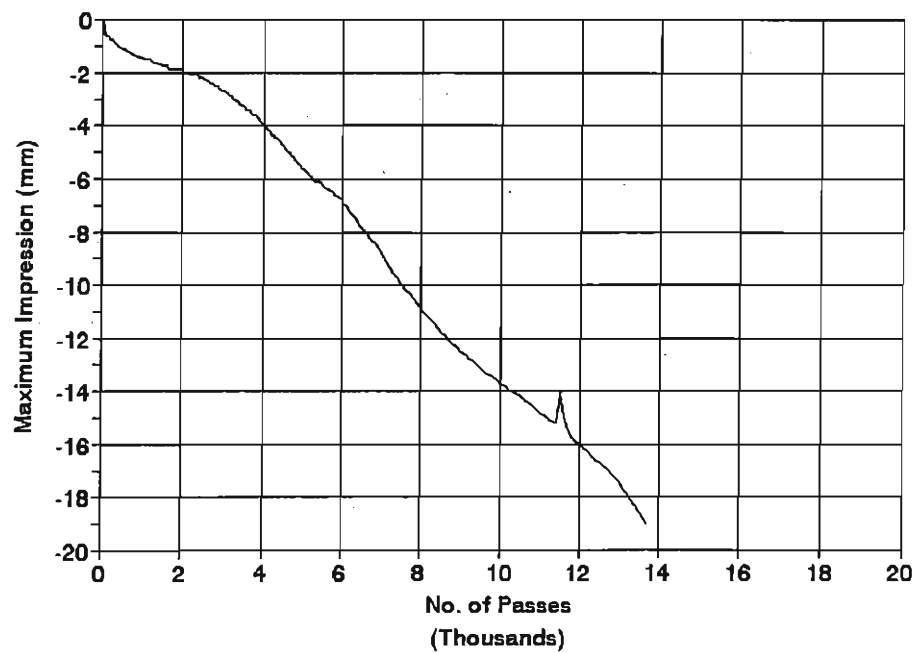
SITE3 FIELD Temperature = 45 C
