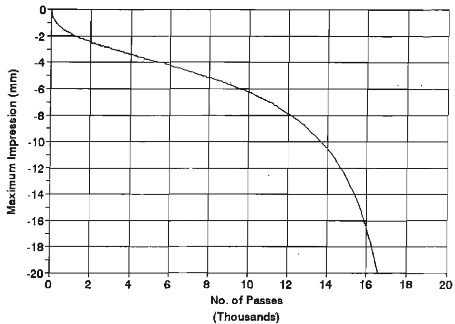
SITE4 L2 Temperature = 40 C
