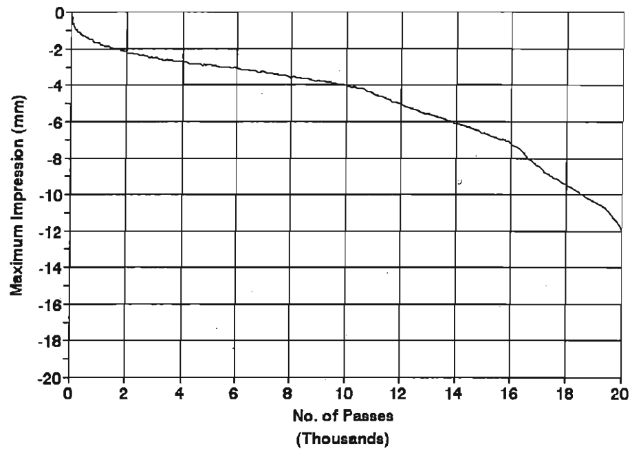
SITE1 L0 Temperature = 45 C
