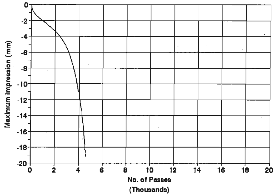
SITE5 L0 Temperature = 45 C
