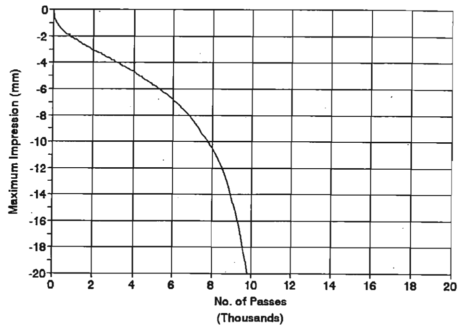
SITE8 FIELD Temp. 55 C
