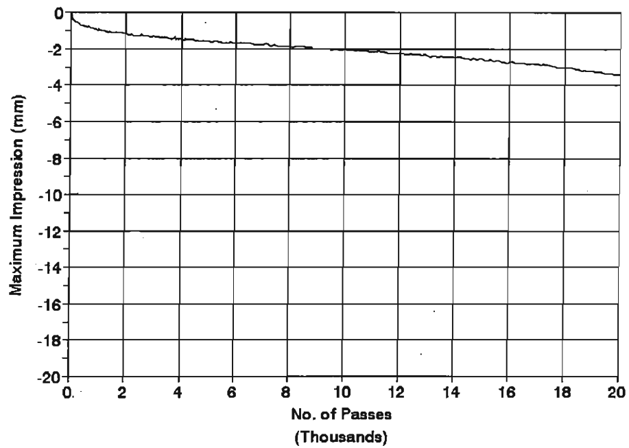
SITE7 L4 Temperature = 40 C
