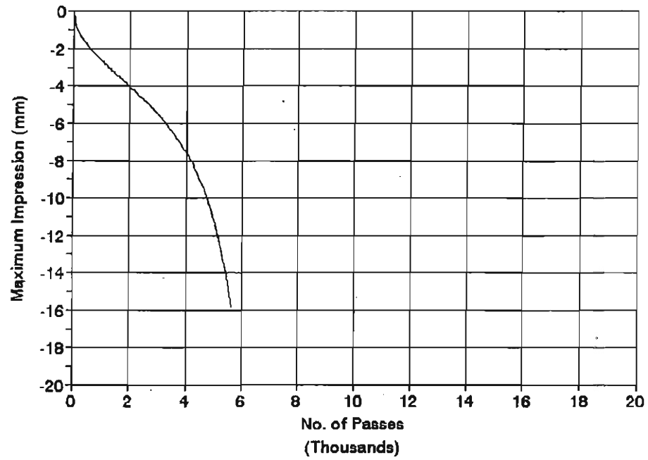
SITE4 L0 Temperature = 40 C
