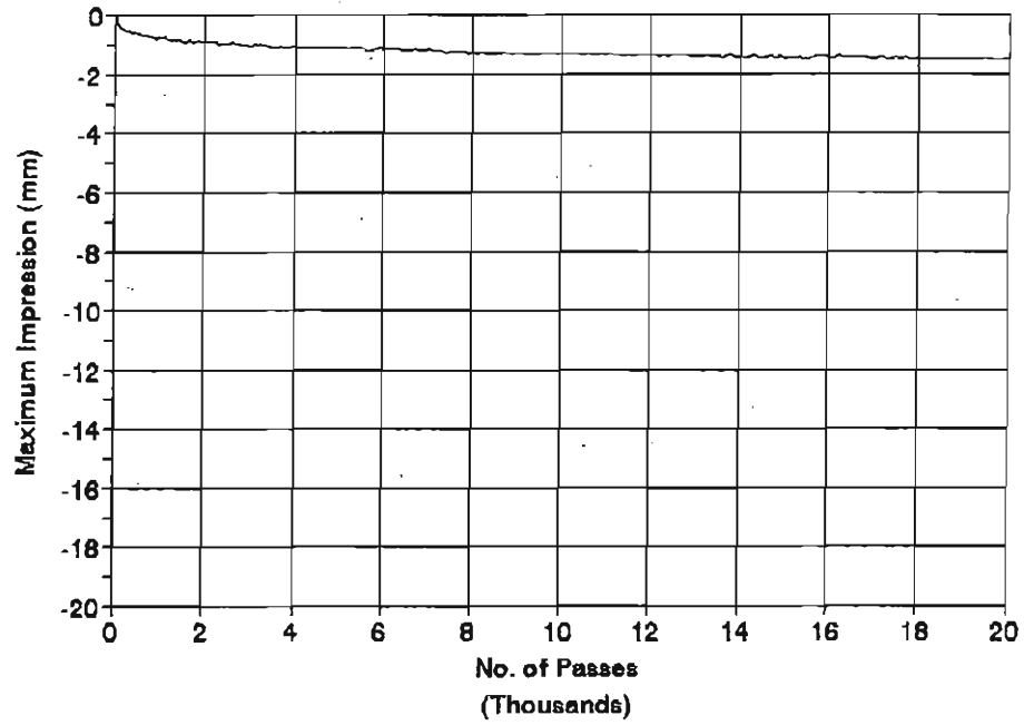
SITE2 L4 Temperature = 45 C
