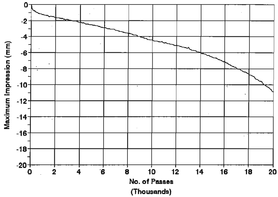
SITE4 FIELD Temperature = 40 C
