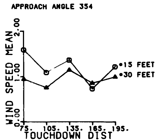
FIGURE D-4. MEAN CHANGES IN WIND SPEED TOUCHDOWN DISTANCE AND APPROACH AZIMUTH
