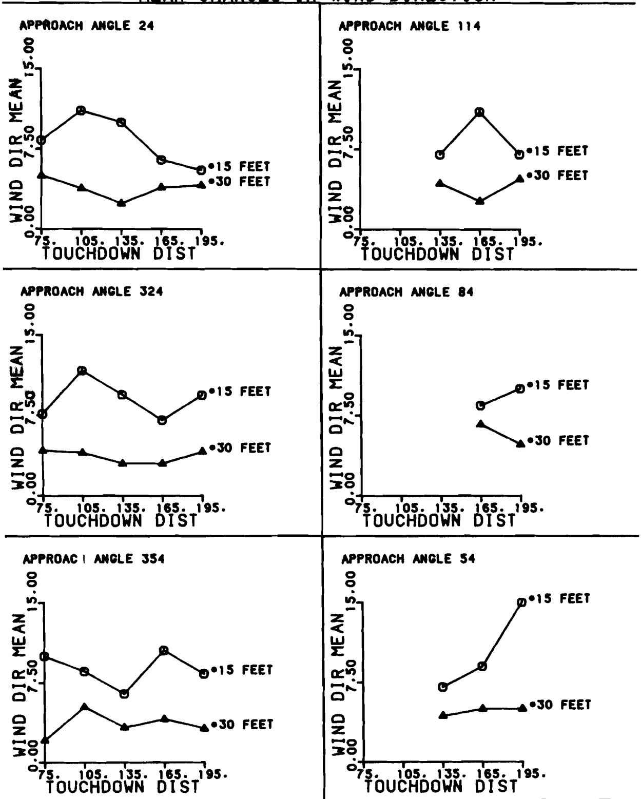
FIGURE D-1. MEAN CHANGES IN WIND DIRECTION TOUCHDOWN DISTANCE AND APPROACH AZIMUTH
