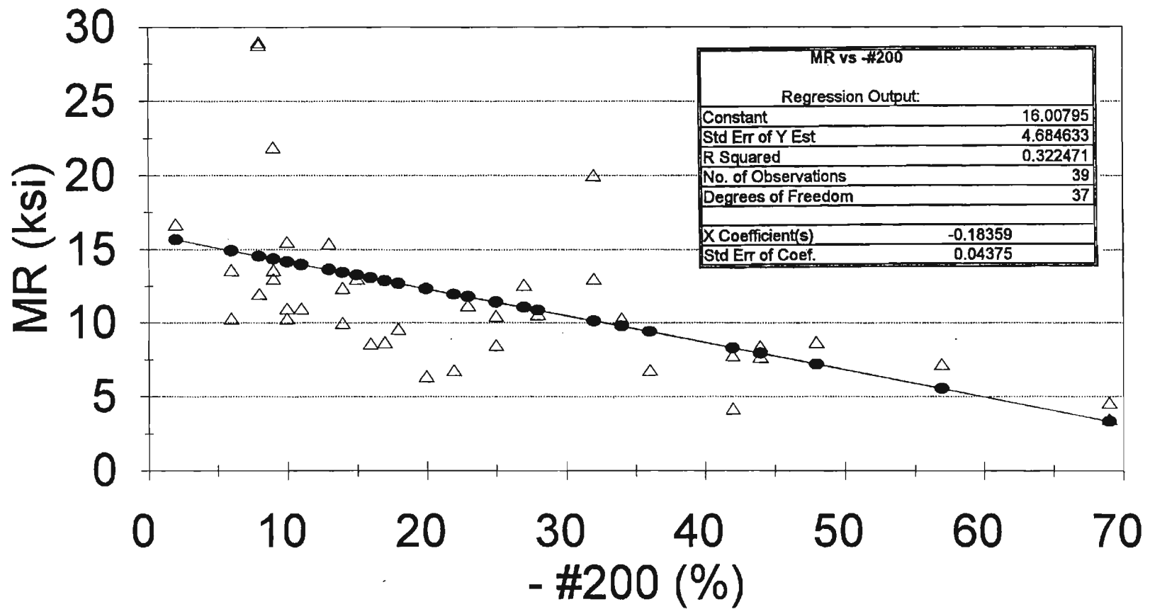
Figure V.4 Linear Regression Equation of M_r vs. Fines Content
