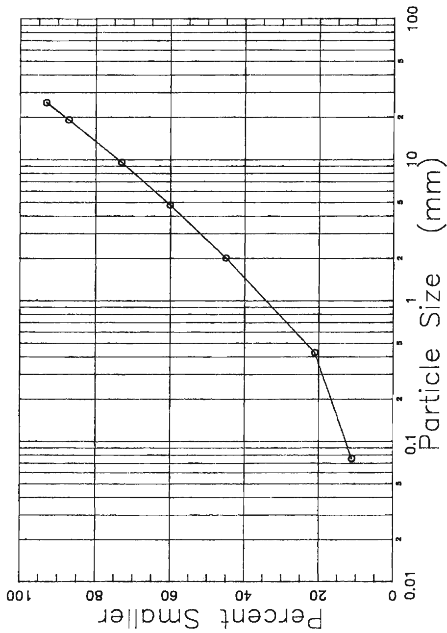
PARTICLE SIZE GRAPH Sample No. 18
