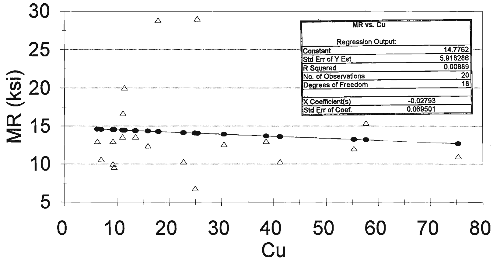
Figure V.6 Linear Regression Equation of M_r vs. C_u
