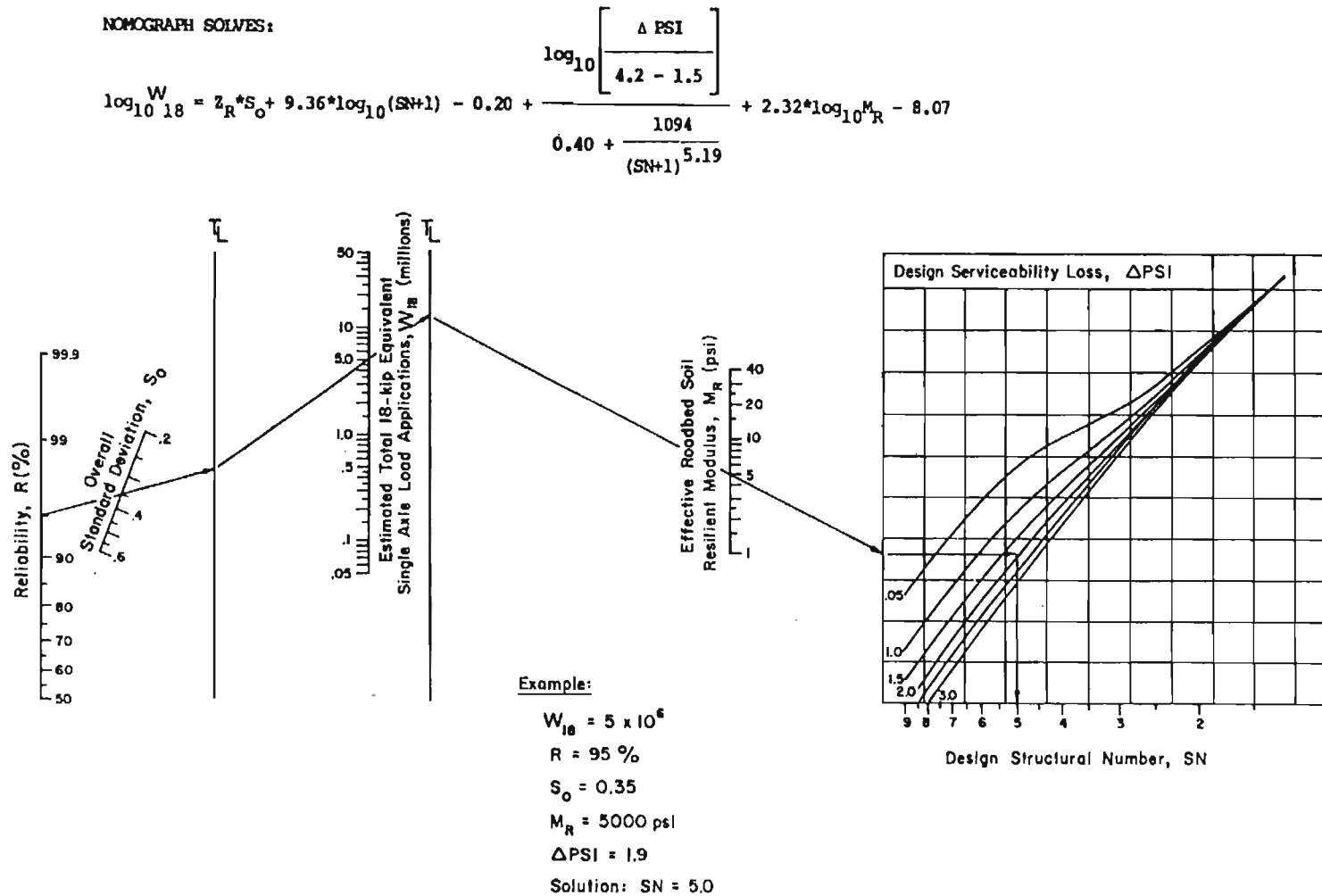
Figure III.1 Design chart for flexible pavements based on using mean values for each input (form AASHTO, 1986).
