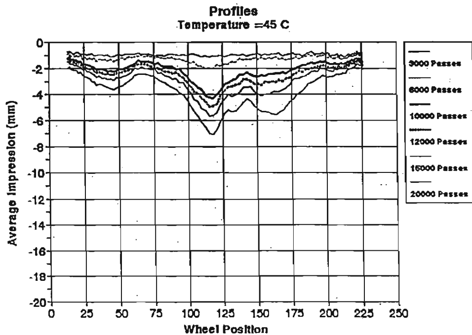
Figure 9. Results from the Hamburg Wheel-Tracking Device (Grading C) for the Colorado City Project
