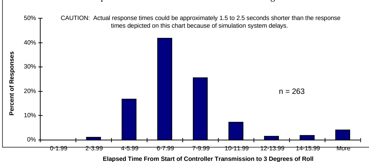
Figure 7. Roll response times - all flight simulator sites.
