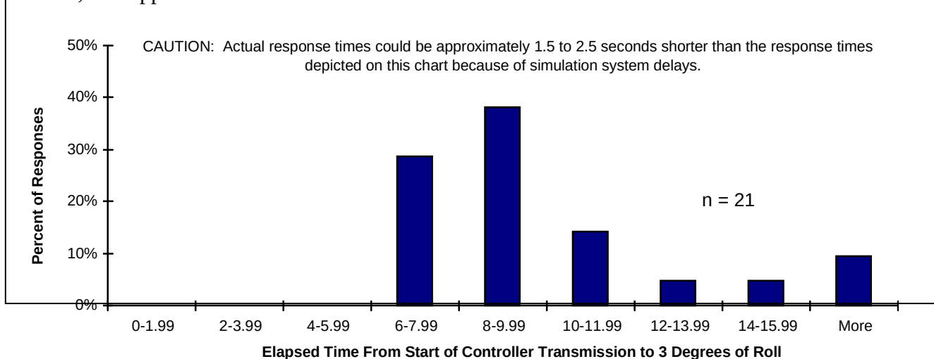
Figure 8. Roll response times for autopilot breakouts (MD90).
