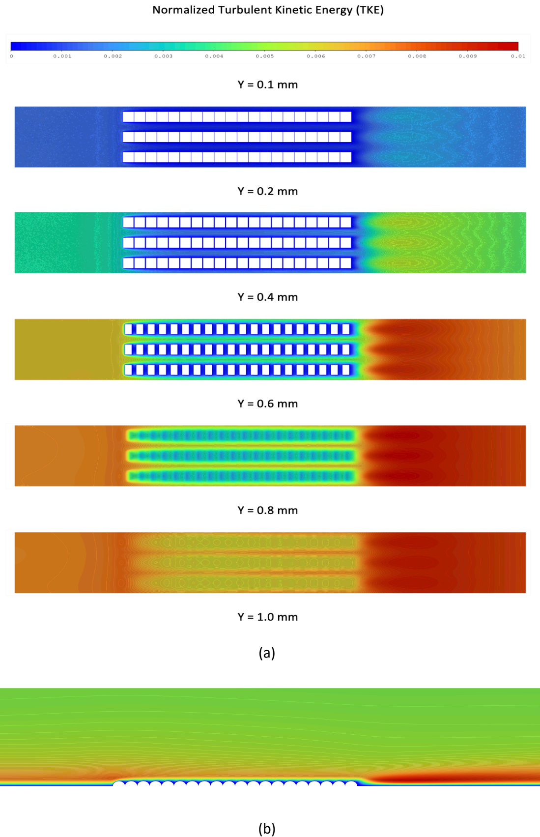
Figure 12. Contours of Normalized Turbulent Kinetic Energy Velocity from 10D Upstream to 15D Downstream of the Half-Stepped Cylinders, (a) X-Z Planes, (b) X-Y Plane at Mid-Section.
