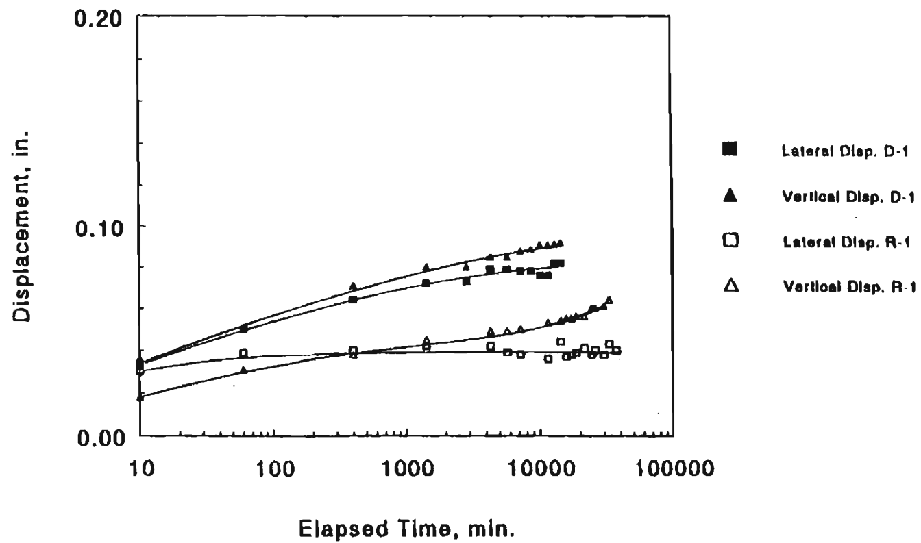
Figure 4.19 : Lateral and Vertical Displacements Versus Time Relationships of Tests D-1, R-1
