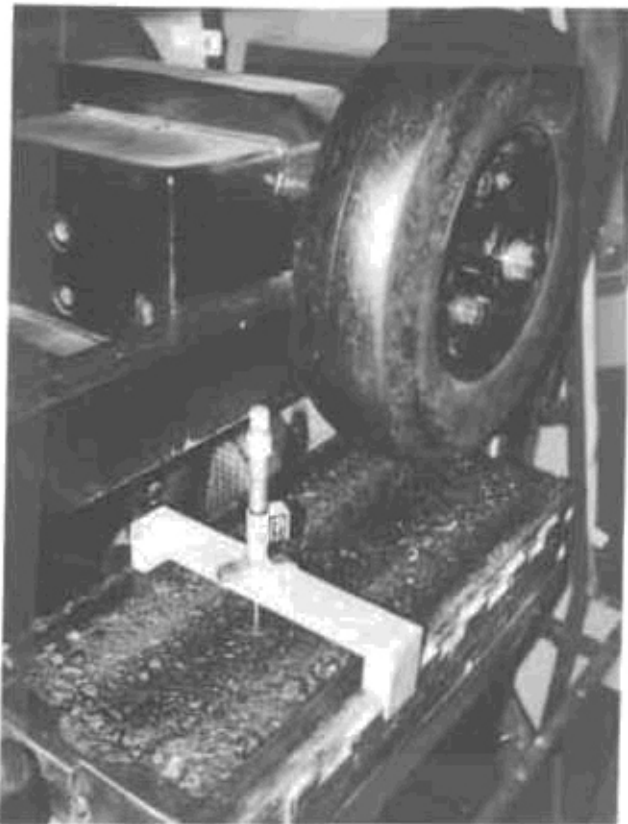
Figure 14. Close-Up of the French Rutting Tester.
