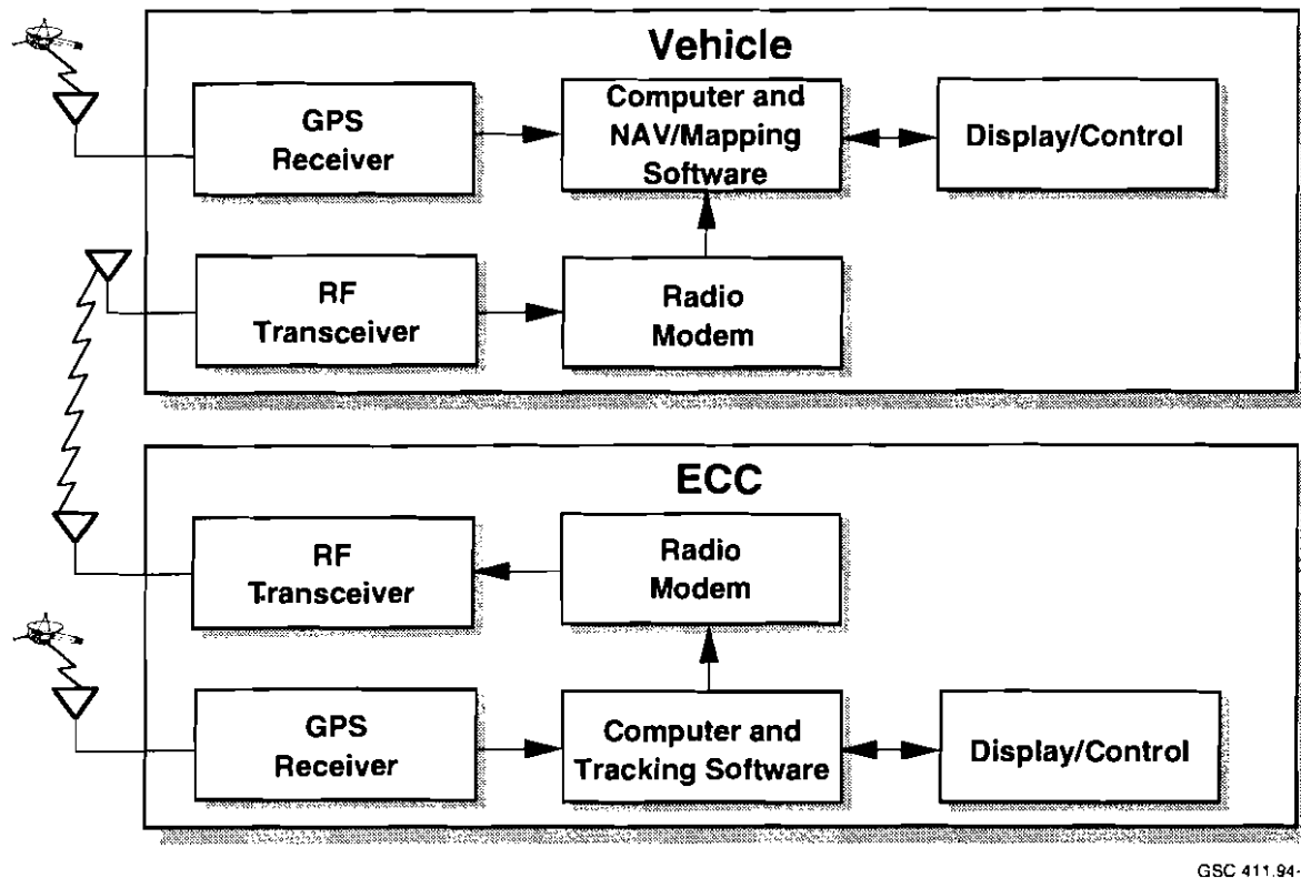
FIGURE 6. NAVIGATION SUBSYSTEM
