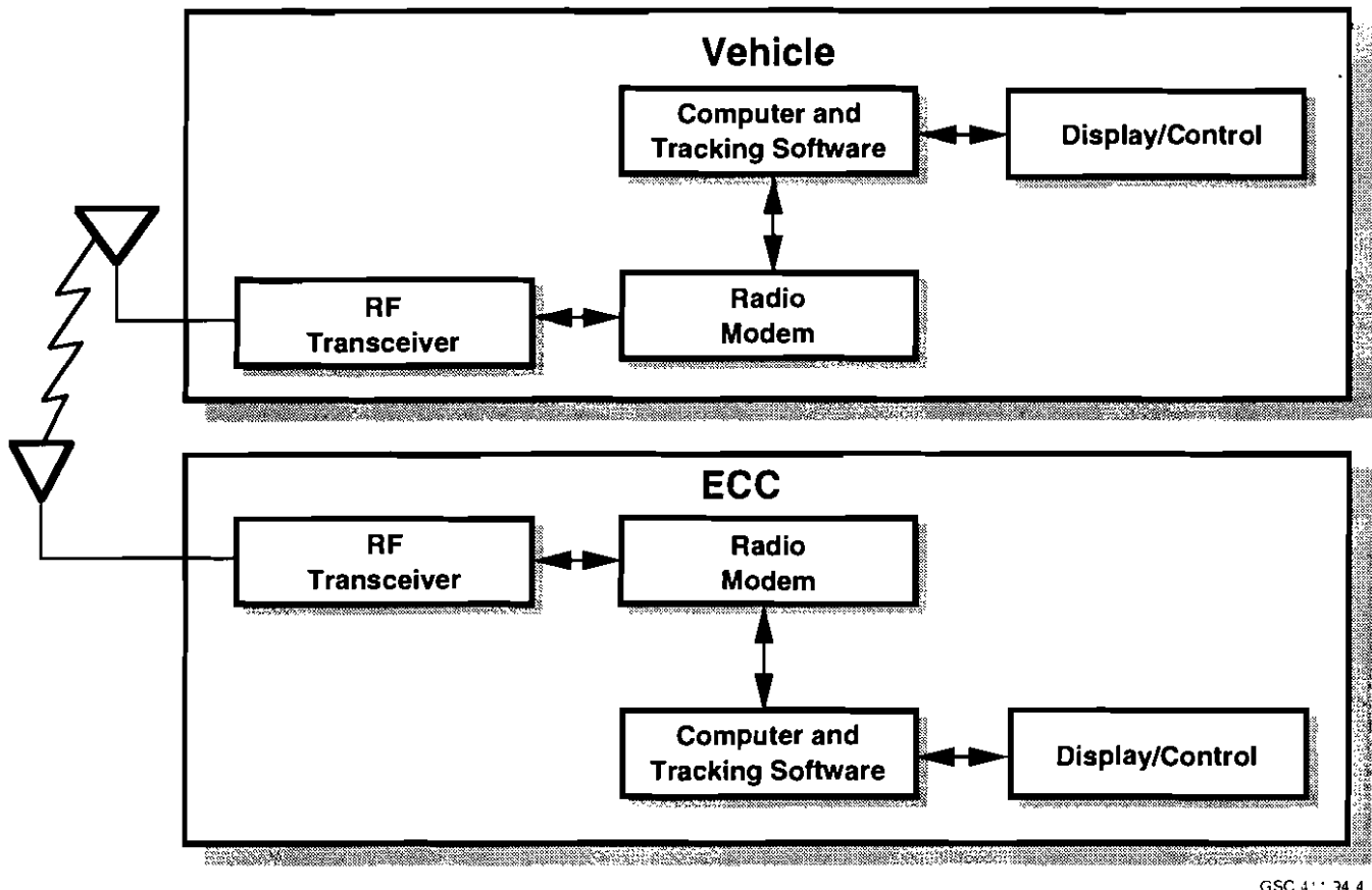
FIGURE 7. TRACKING SUBSYSTEM
