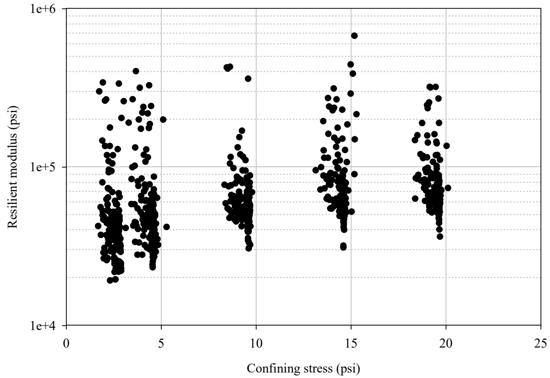
Figure 9-2 Resilient modulus of the LCC specimens as a function of confining stress
