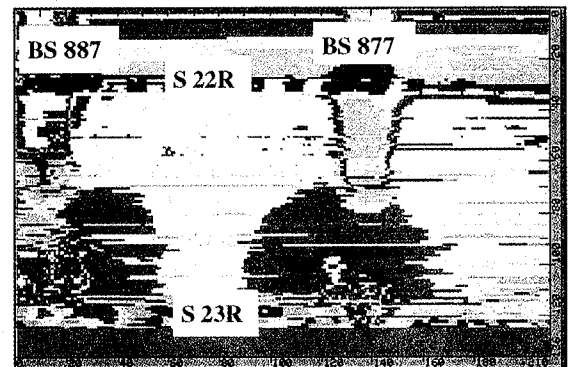
Corrosion is shown in dark blue around BS 877 and BS 887.
