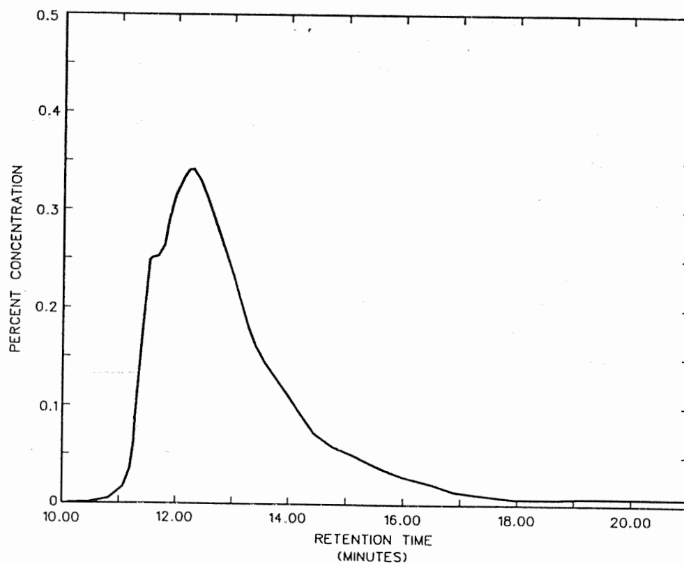
FIGURE B10. GPC CHROMATOGRAPH OF GILSONITE
