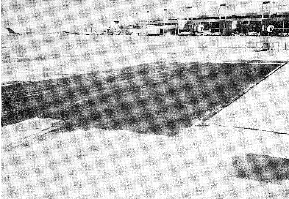
FIGURE 12. FUEL-RESISTANT SEALER TEST SECTION AT DFW AIRPORT
