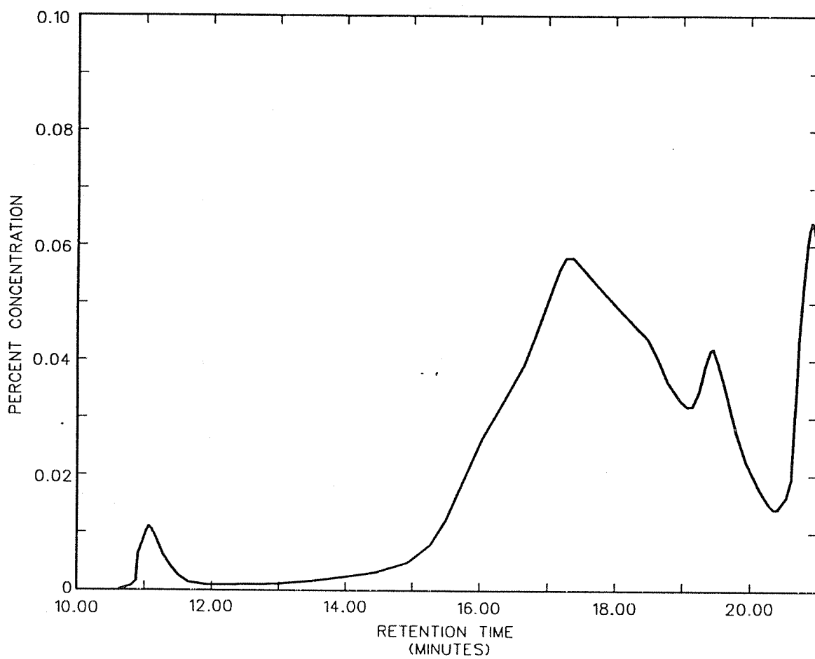
FIGURE B11. GPC CHROMATOGRAPH OF ROSPHALT 50
