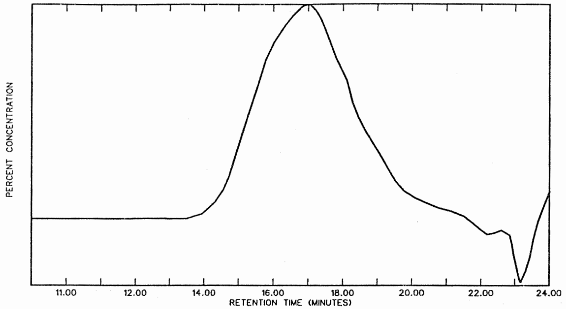
FIGURE B1. GPC CHROMATOGRAPH OF POLYBILT 103S
