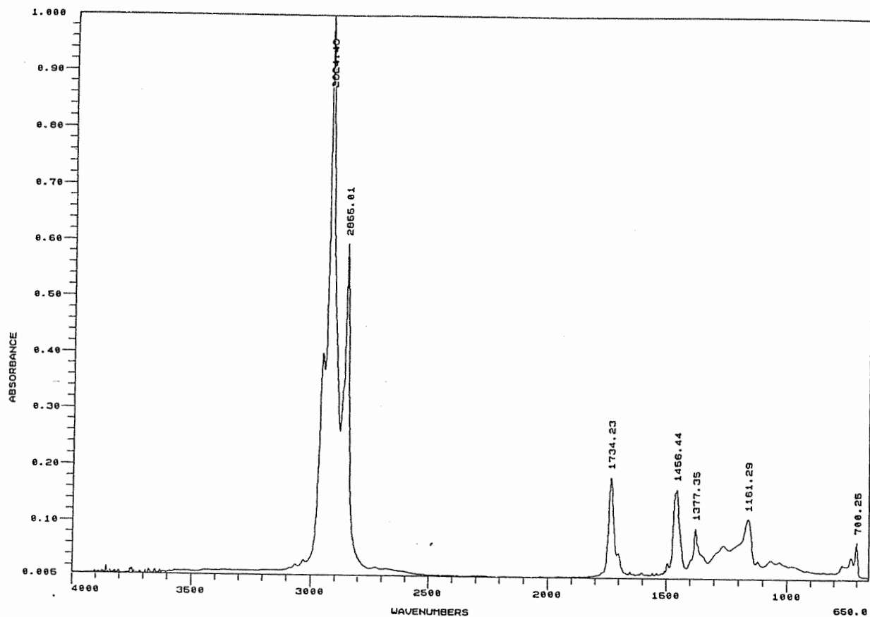
FIGURE A12. FTIR SPECTRUM OF DUCTILAD D1002
