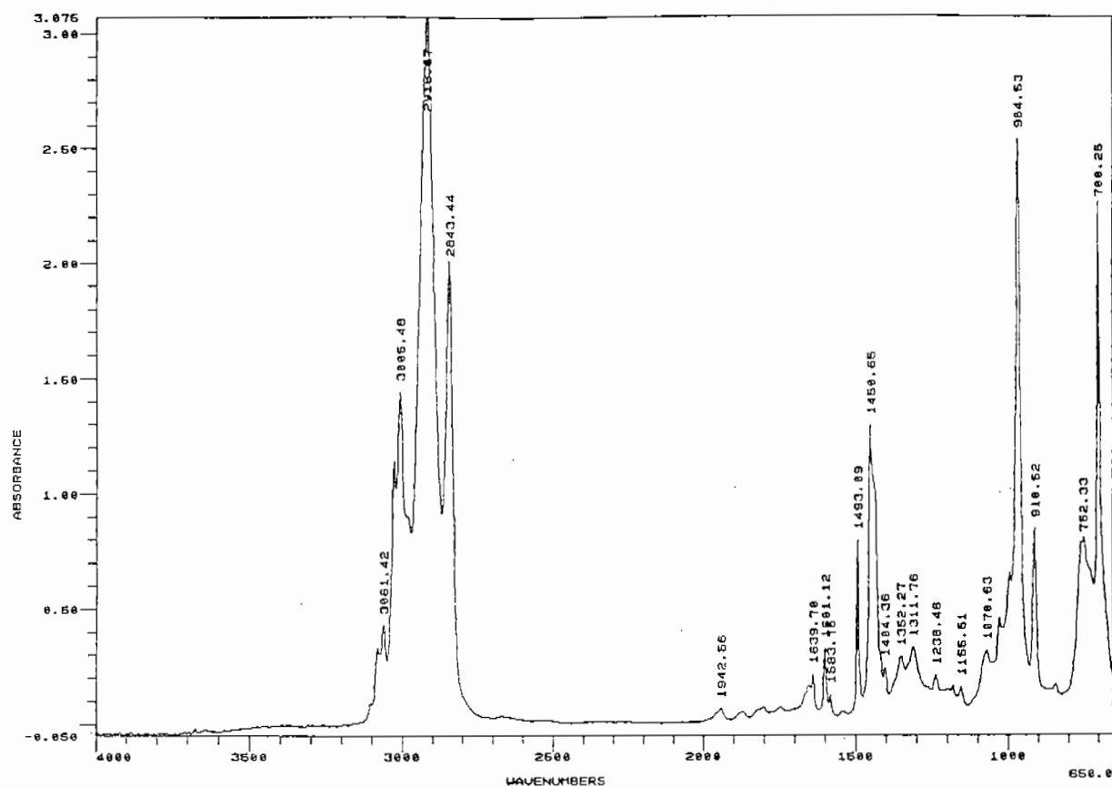
FIGURE A5. FTIR SPECTRUM OF KRATON D1101
