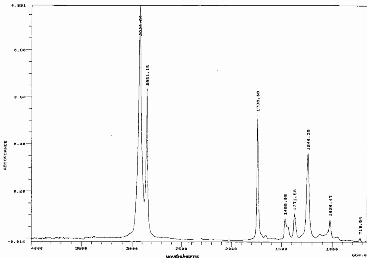
FIGURE A1. FTIR SPECTRUM OF POLYBILT 103S
