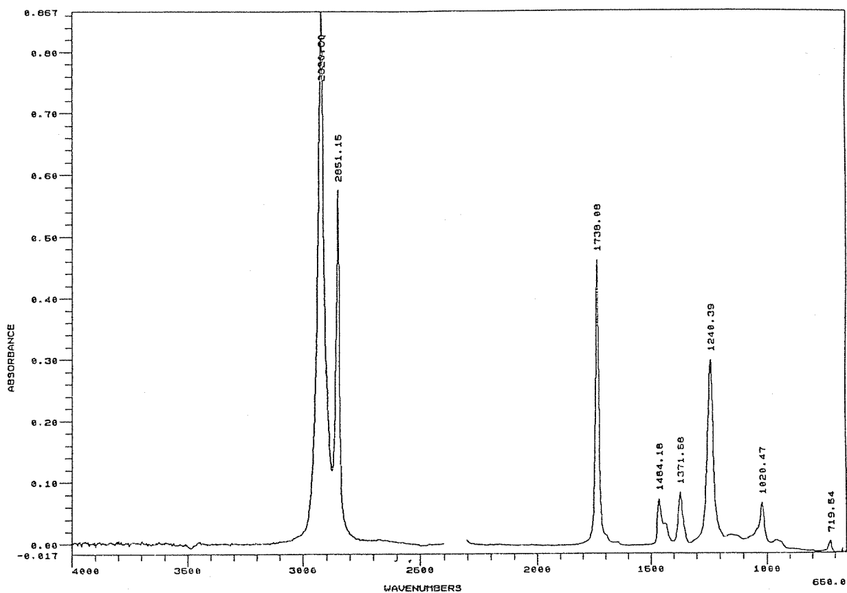
FIGURE A7. FTIR SPECTRUM OF ELVAX 150W
