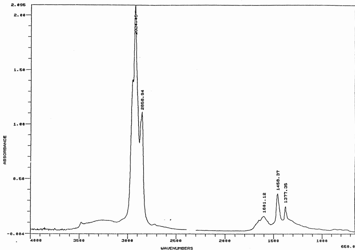
FIGURE A16. FTIR SPECTRUM OF GILSONITE
