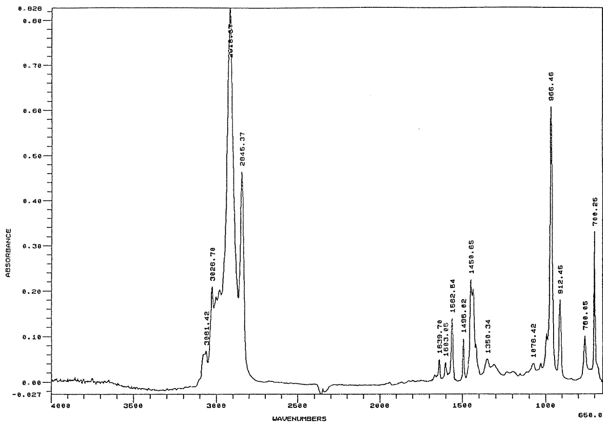
FIGURE A13. FTIR SPECTRUM OF RUB-R-ROAD
