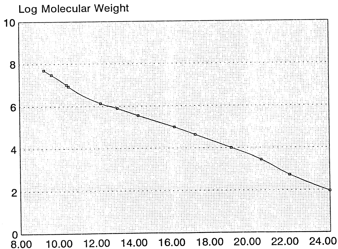
FIGURE 21. CALIBRATION CURVE FOR GPC SYSTEM NUMBER 1.
