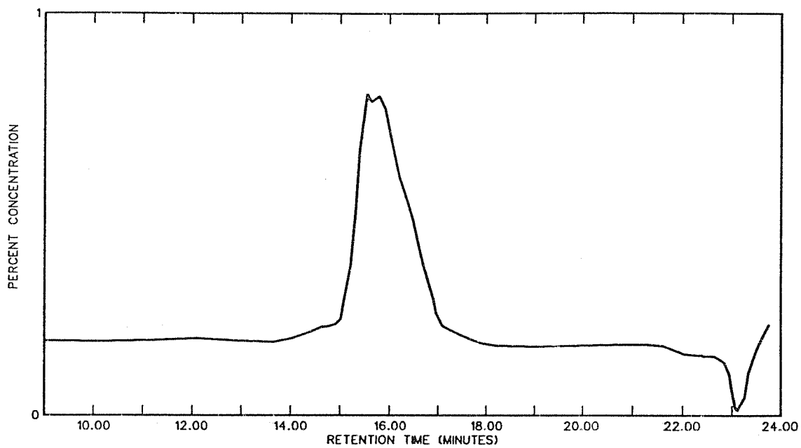
FIGURE B5. GPC CHROMATOGRAPH OF KRATON D1101
