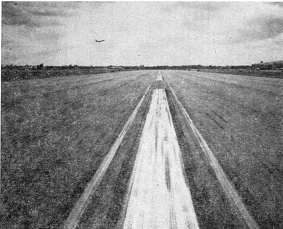
FIGURE 7. HOUSTON HOBBY RUNWAY 17-35 SURFACED WITH NOVAPHALT
