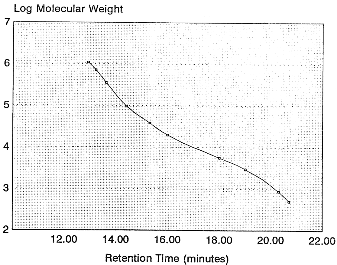
FIGURE 22. CALIBRATION CURVE FOR GPC SYSTEM NUMBER 2
