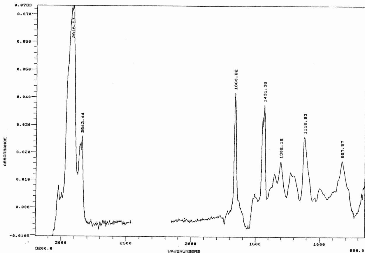
FIGURE A10. FTIR SPECTRUM OF NEOPRENE 654
