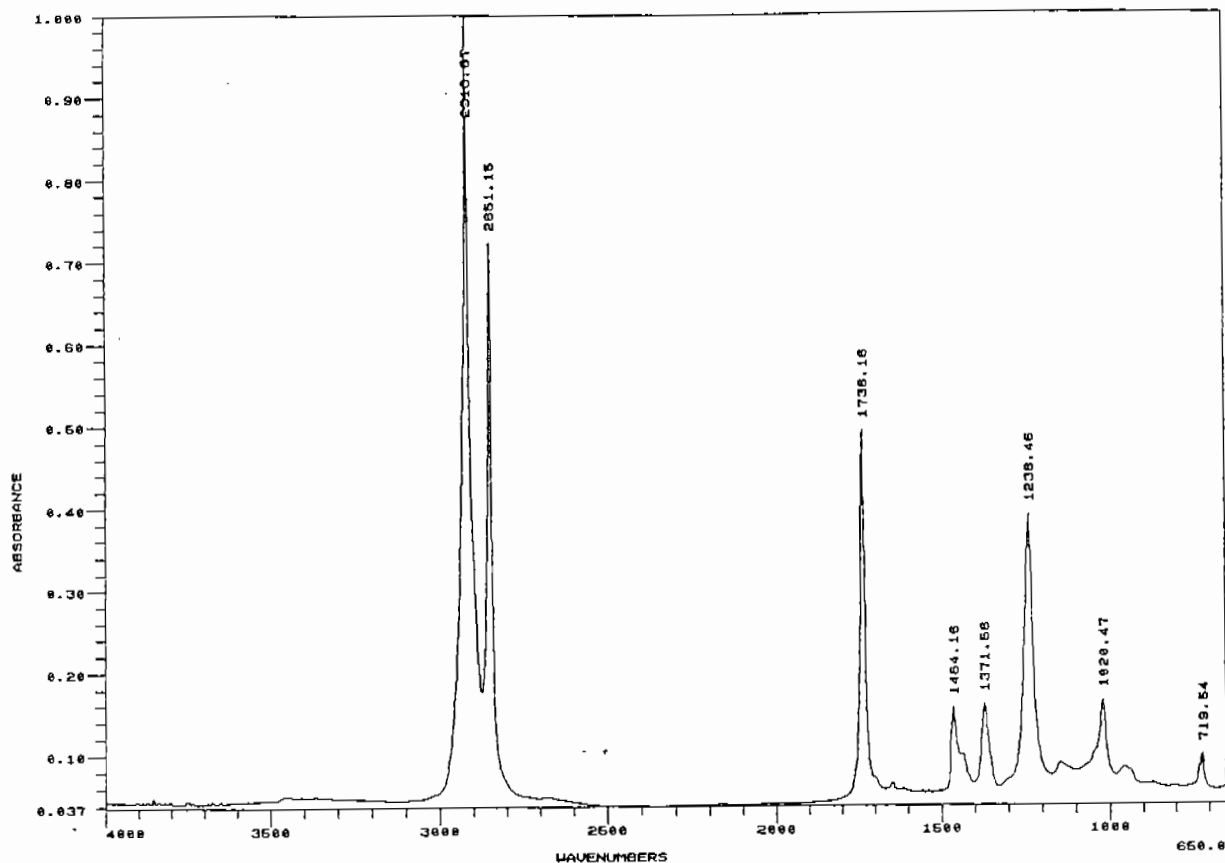
FIGURE A2. FTIR SPECTRUM OF POLYBILT 151
