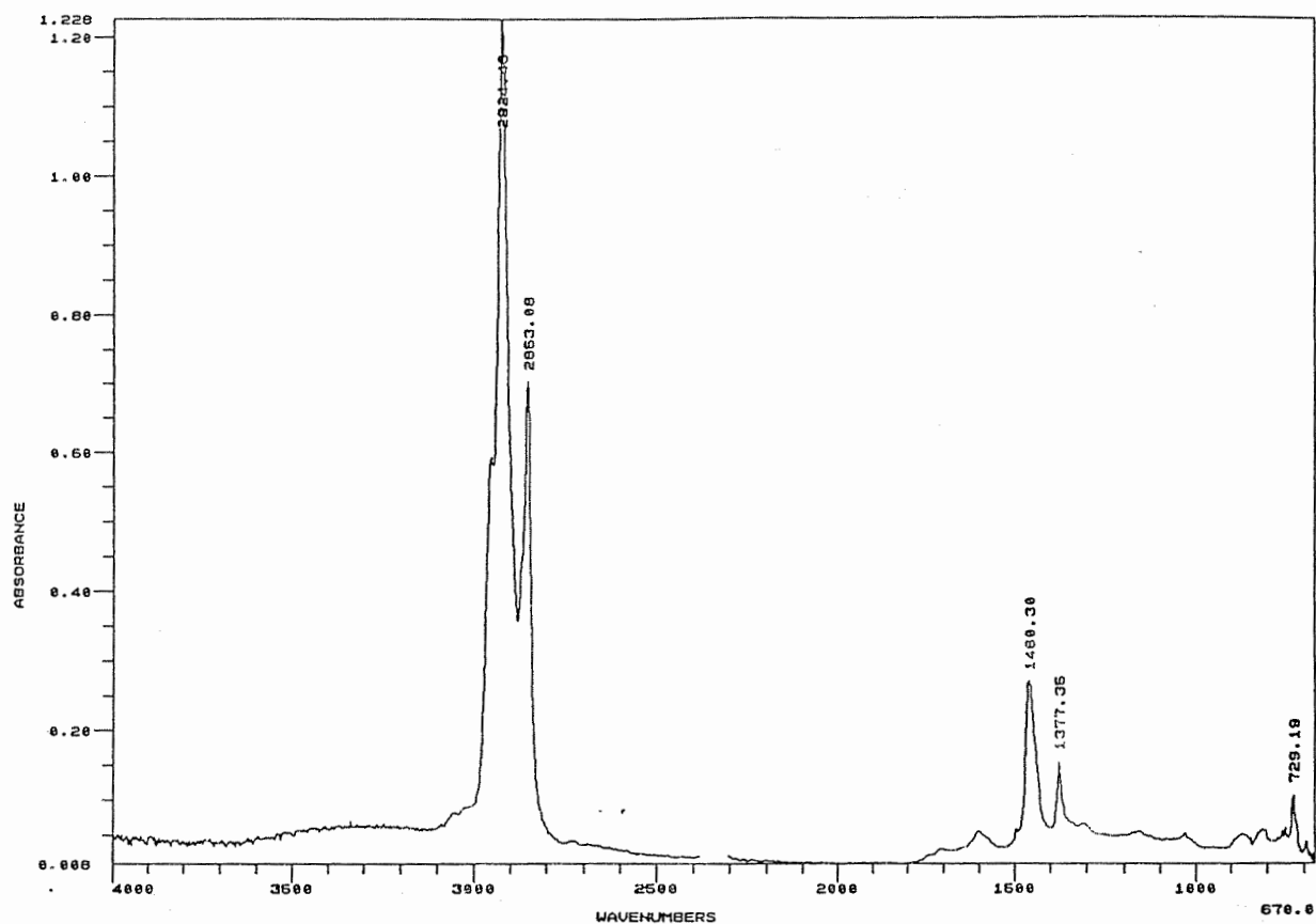
FIGURE A15. FTIR SPECTRUM OF NOVAPHALT
