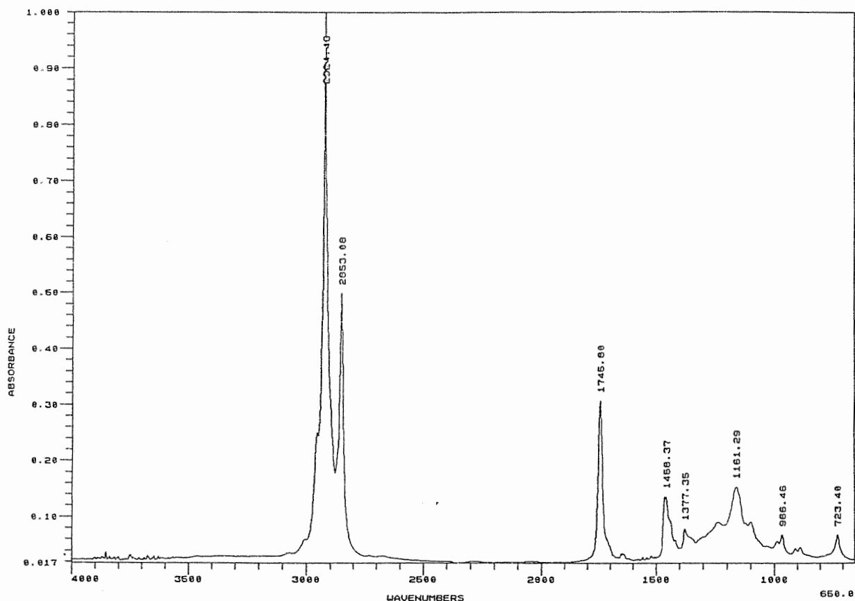
FIGURE A11. FTIR SPECTRUM OF DUCTILAD D1000
