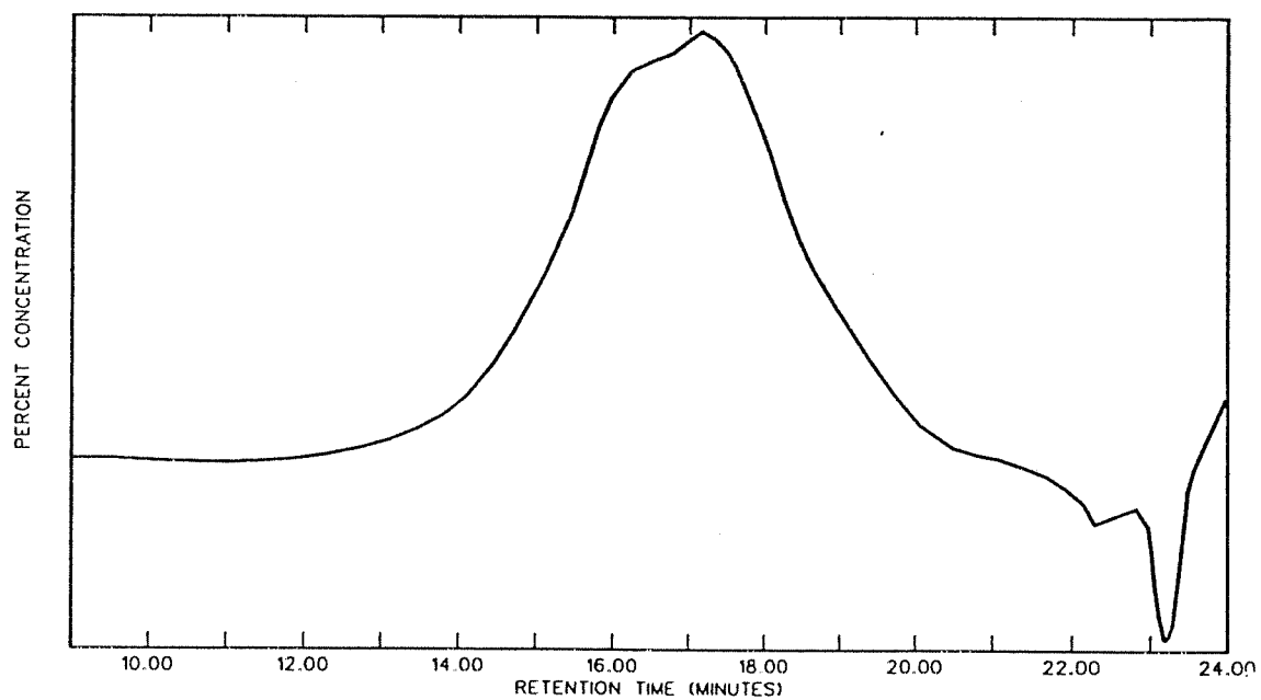
FIGURE B6. GPC CHROMATOGRAPH OF ELVAX 150W
