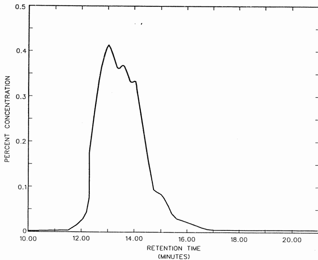
FIGURE B8. GPC CHROMATOGRAPH OF DUCTILAD D1000
