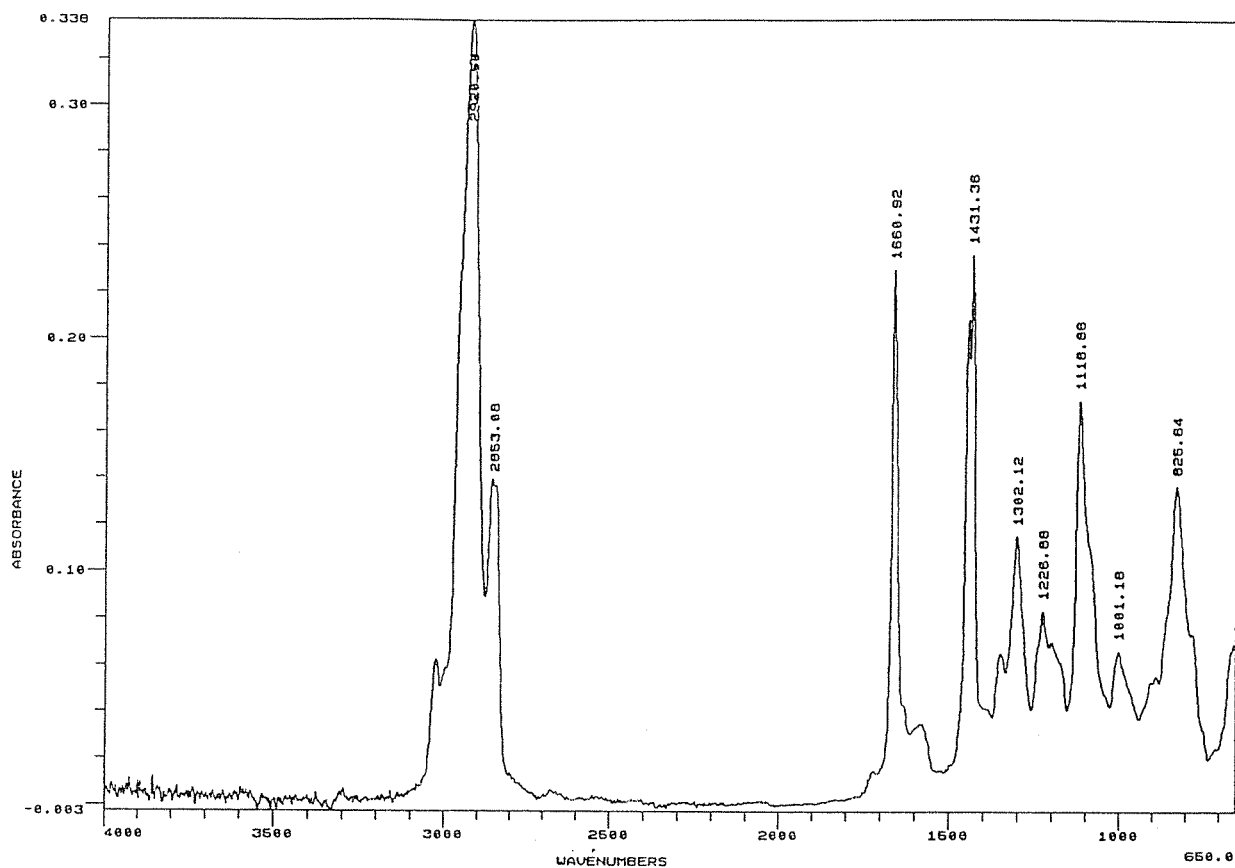
FIGURE A9. FTIR SPECTRUM OF NEOPRENE 735A
