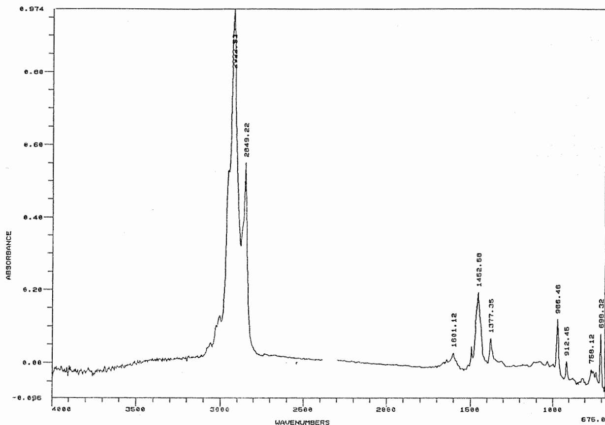
FIGURE A17. FTIR SPECTRUM OF ROSPHALT 50
