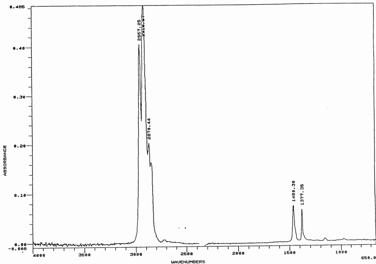
FIGURE A8. FTIR SPECTRUM OF VESTOPLAST-S
