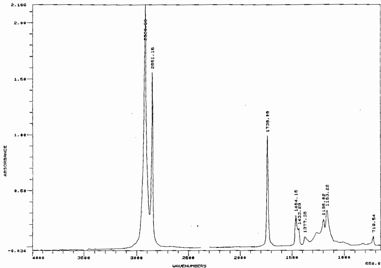
FIGURE A4. FTIR SPECTRUM OF POLYBILT 503
