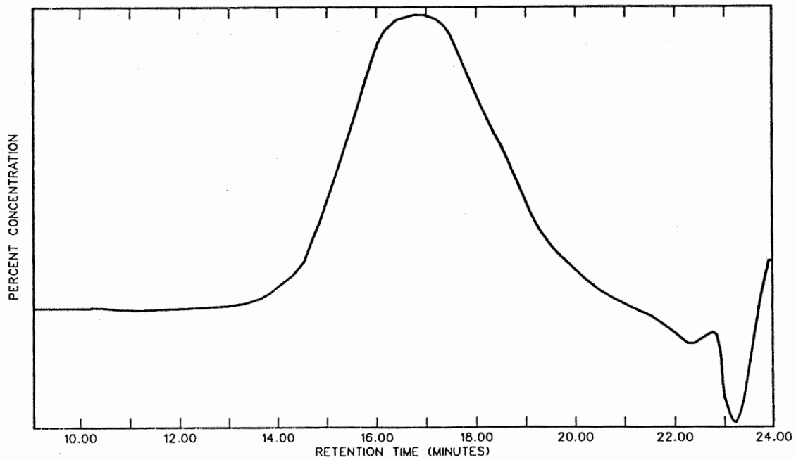
FIGURE B2. GPC CHROMATOGRAPH OF POLYBILT 151
