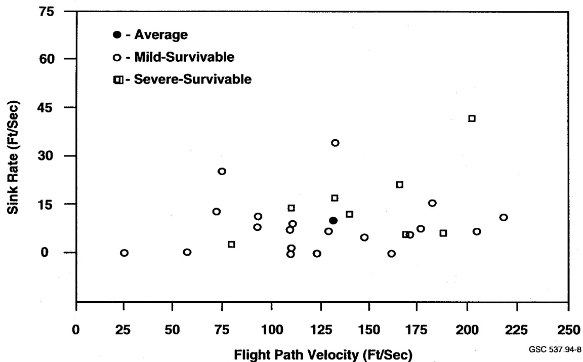
FIGURE 9. FLIGHT PATH VELOCITY VS. SINK RATE FOR SCENARIO 3
