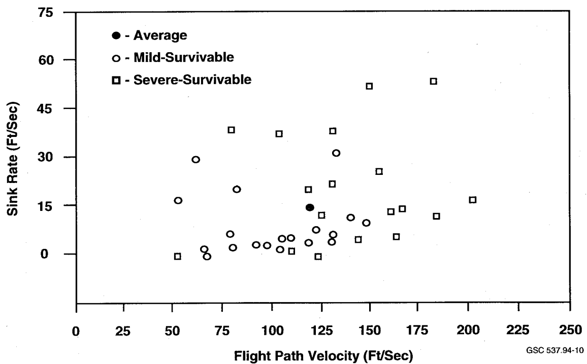
FIGURE 11. FLIGHT PATH VELOCITY VS. SINK RATE FOR SCENARIO 4
