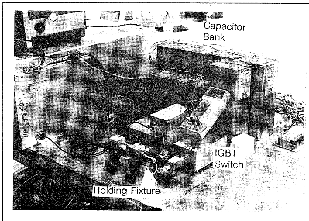
Generator and Fixture
