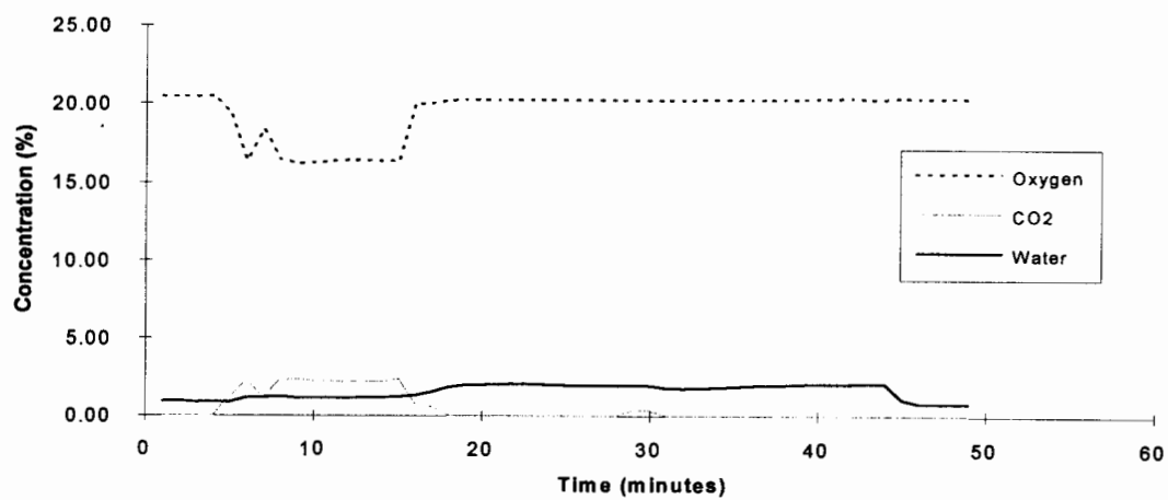
HCFC-123 - Test 2
