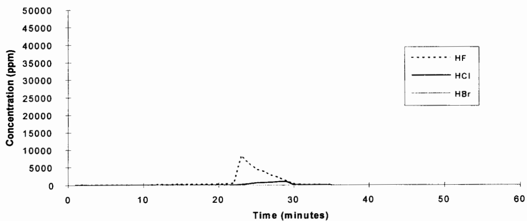
Halon 1211 - Test 2
