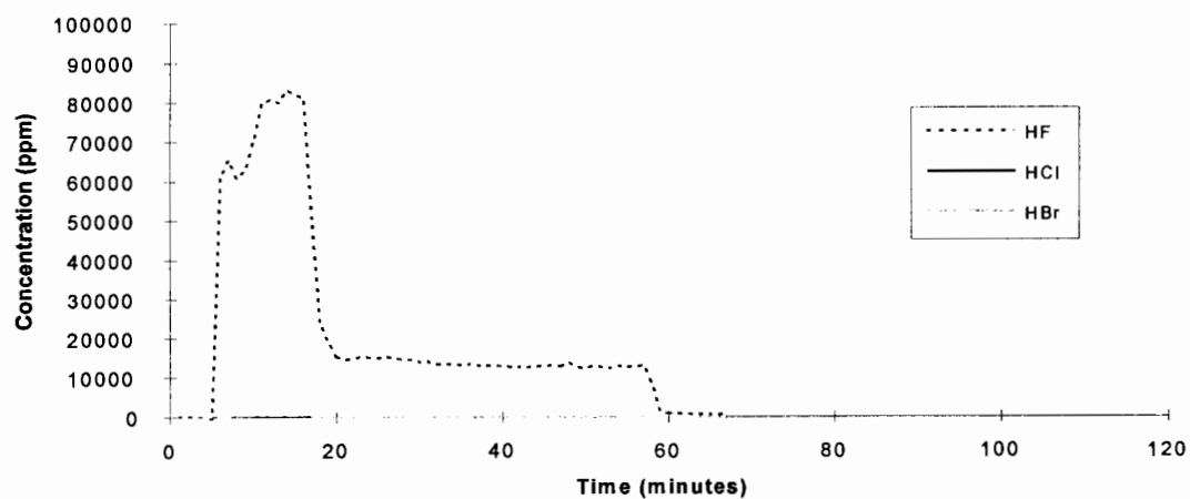
HFC 23 - Test 2
