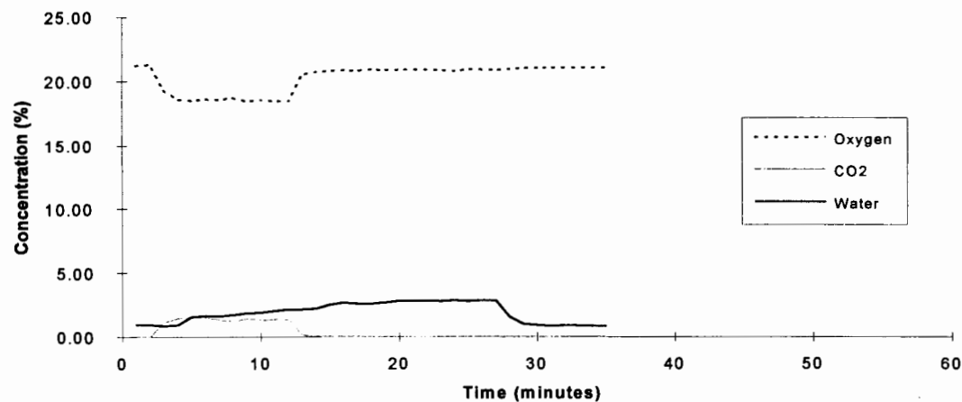
Perfluorobutane - Test 3
