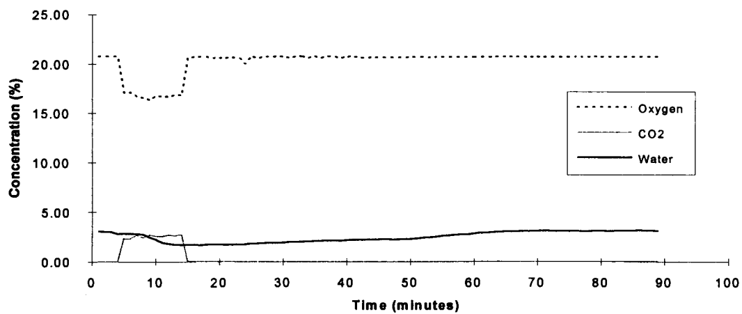
C3F7I - Test 2
