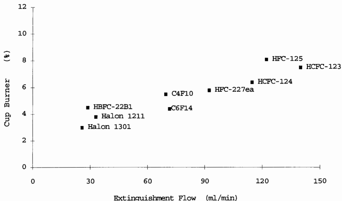
FIGURE 3. EXTINGUISHMENT FLOW VS CUP BURNER
