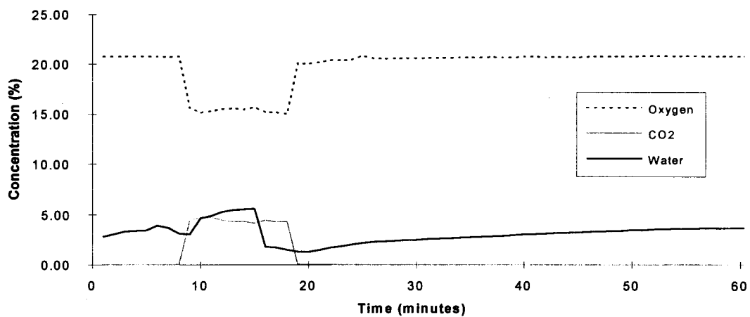
Perfluoropentane - Test 2
