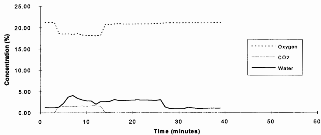
Perfluorobutane - Test 1
