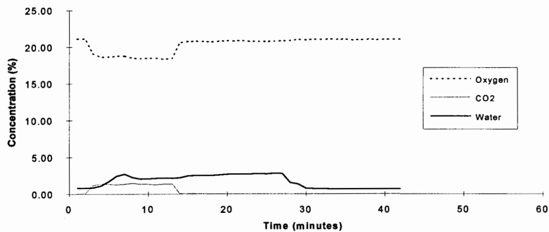
Perfluorobutane - Test 2
