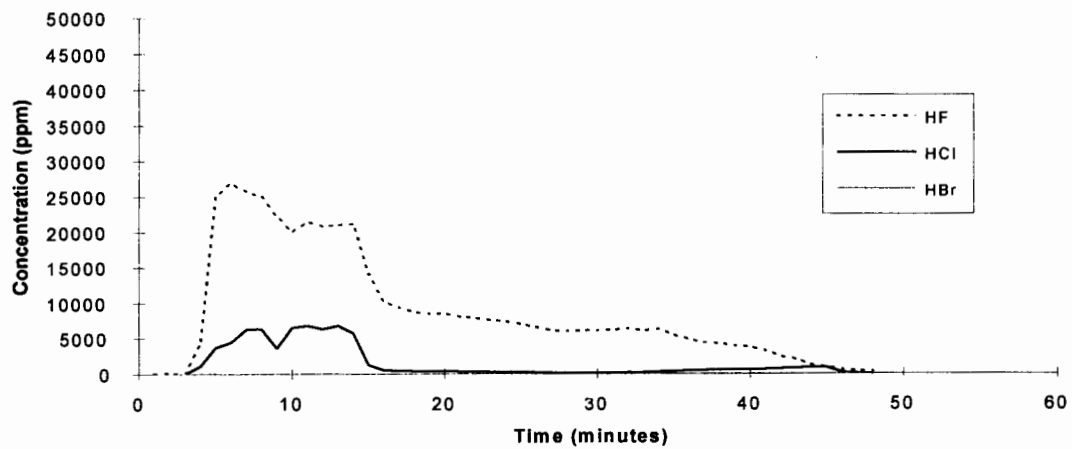
HCFC-123 - Test 1
