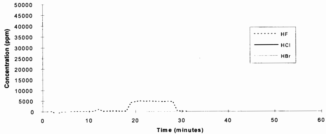
CF3I - Test 3
