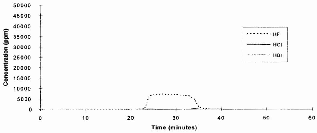
HFC-227EA - Test 2
