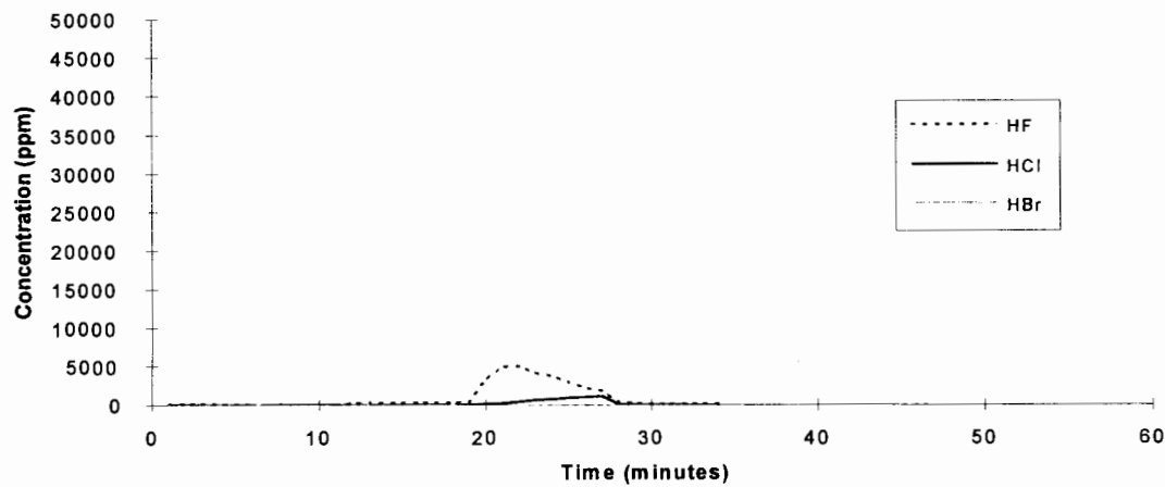
Halon 1211 - Test 3
