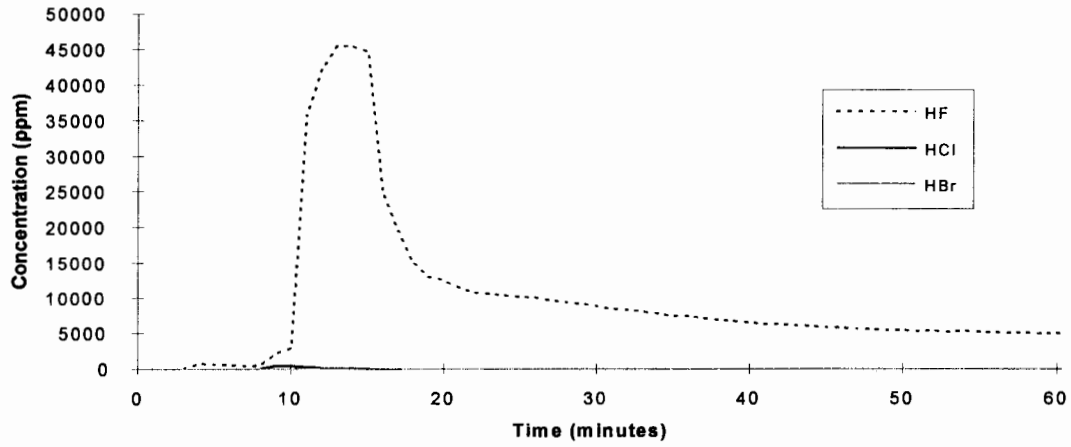
Perfluoropentane - Test 1
