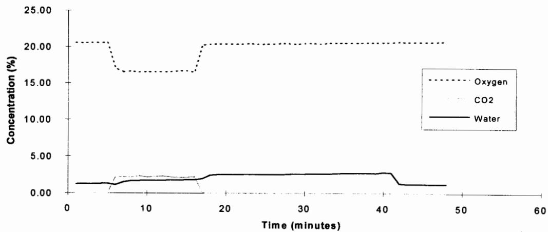
HCFC-123 - Test 3
