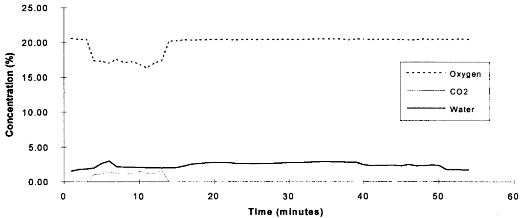
HCFC-124 - Test 3
