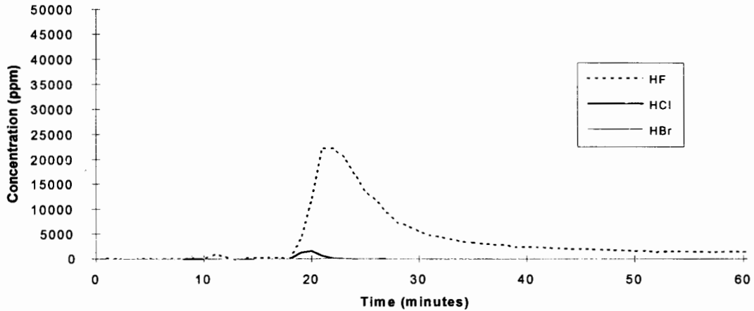
Perfluoropentane - Test 3
