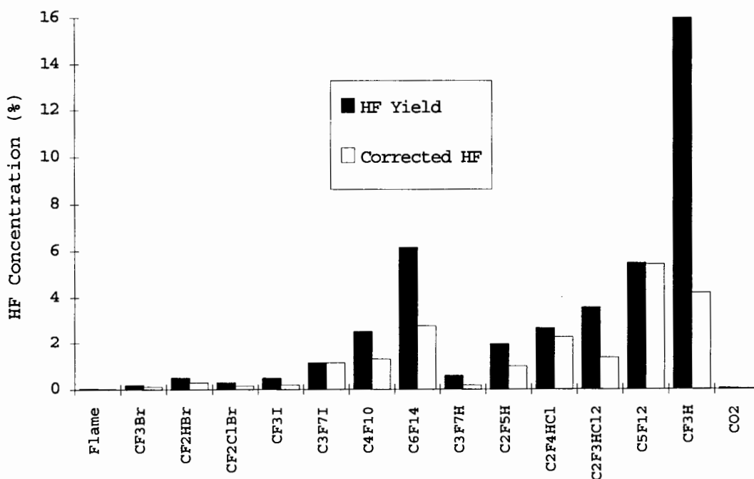
FIGURE 4. HYDROGEN FLUORIDE YIELD
