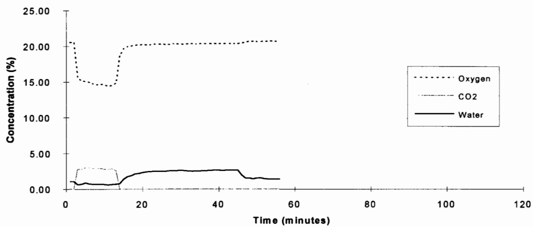
HFC 23 - Test 1
