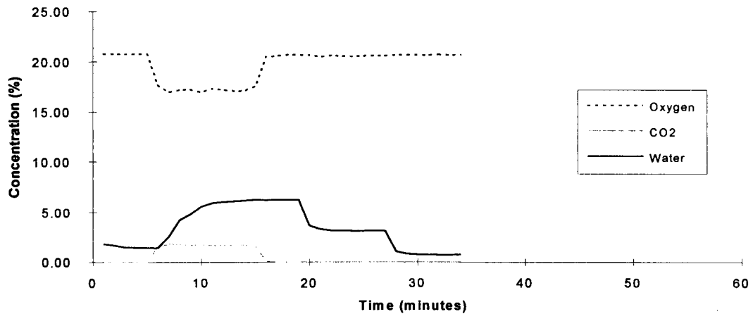
Halon 1211 - Test 3
