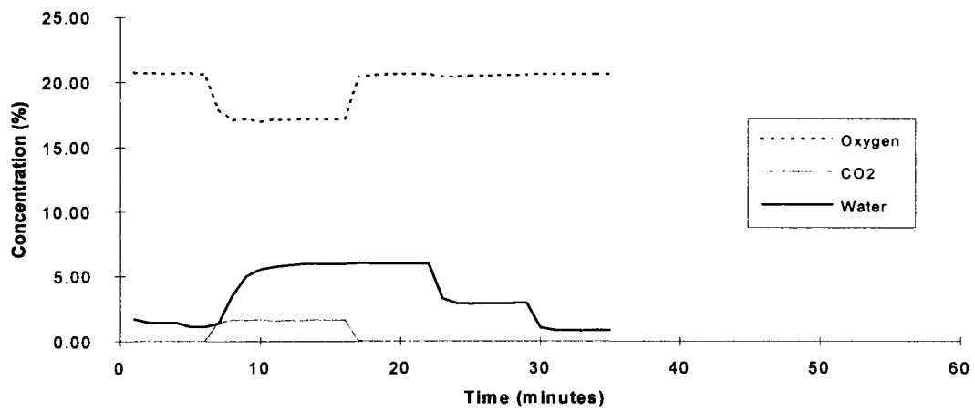
Halon 1211 - Test 2
