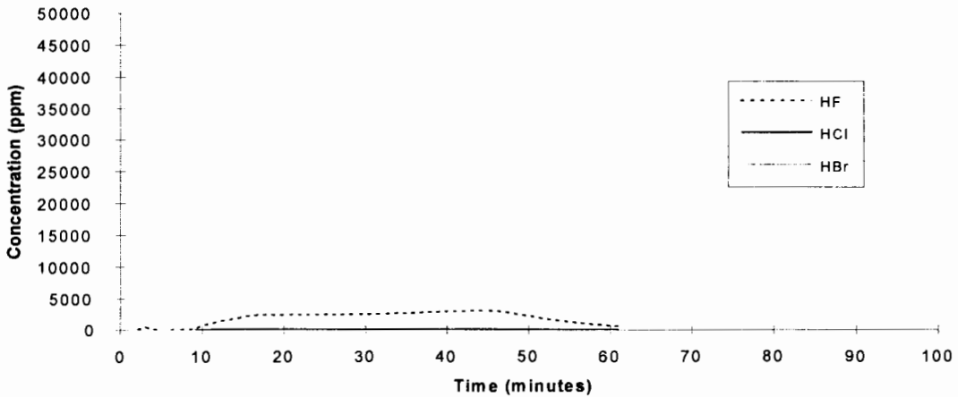
C3F7I - Test 3
