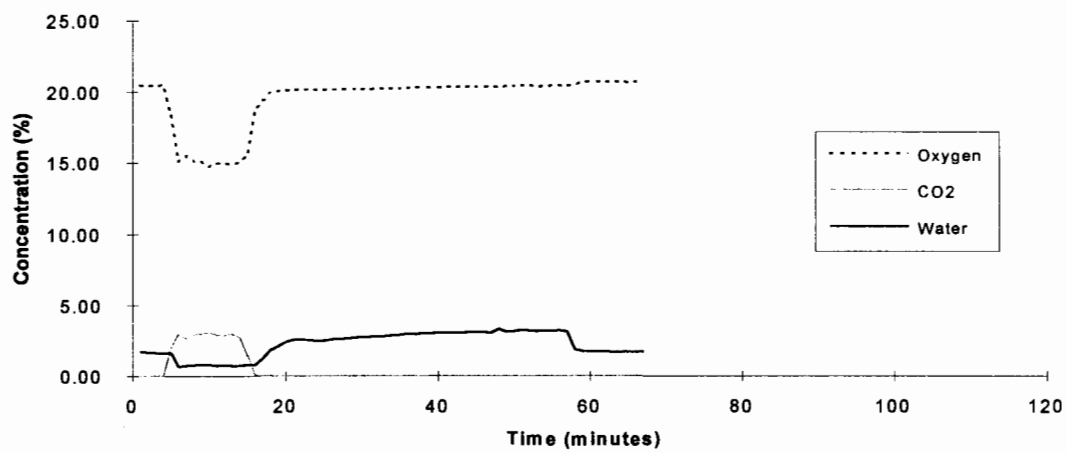
HFC 23 - Test 2
