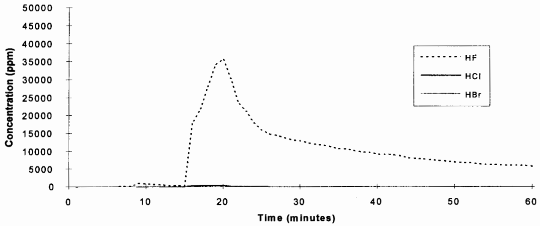
Perfluoropentane - Test 2
