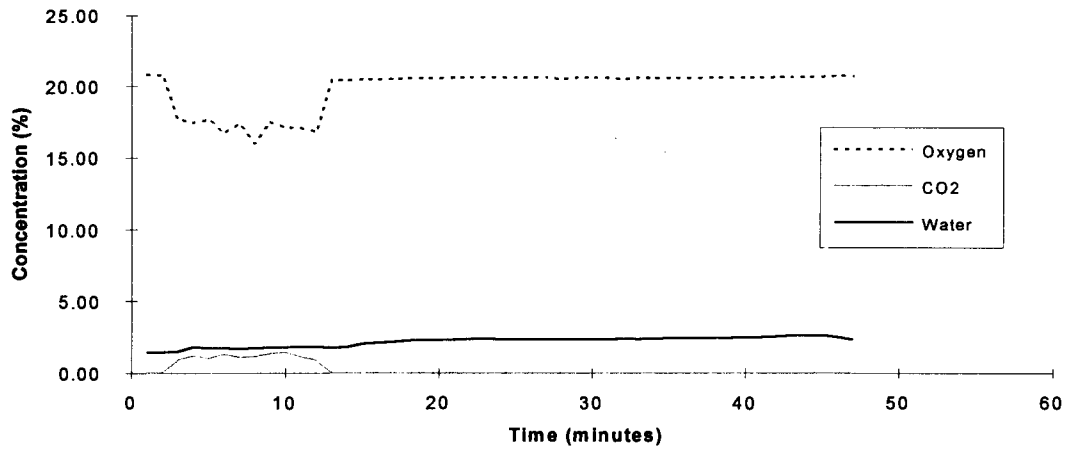
HCFC-124 - Test 1
