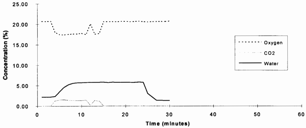
Halon 1301 - Test 1
