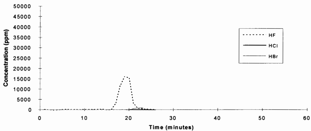
HBFC-22B1 - Test 2
