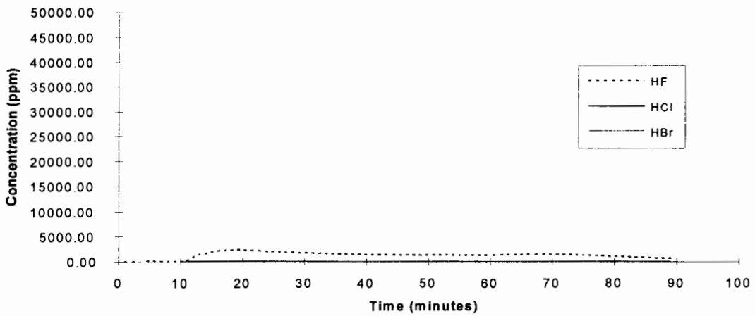
C3F7I - Test 2
