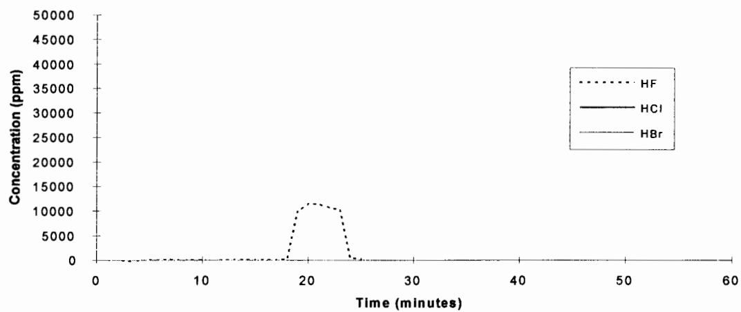
HBFC-22B1 - Test 1
