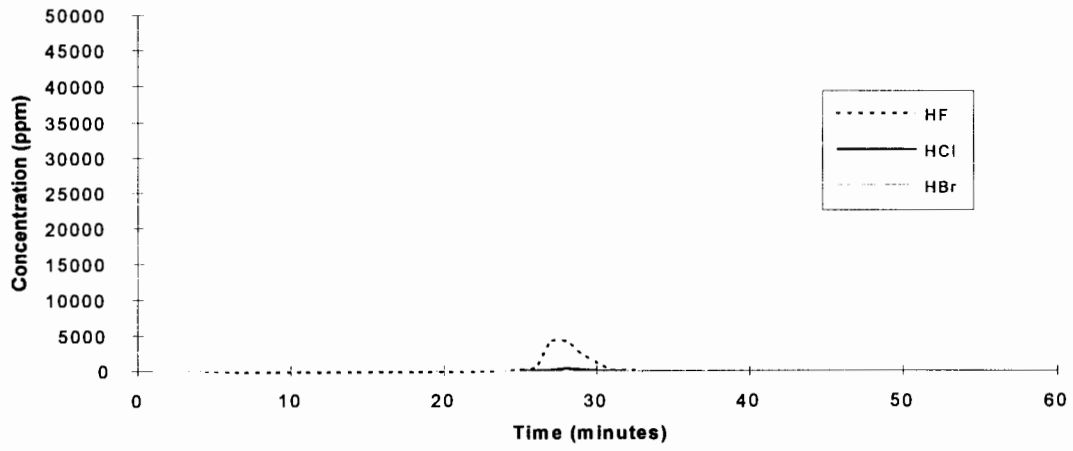
HFC-227EA - Test 1
