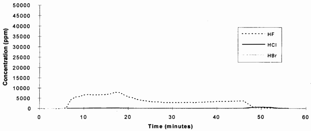
HFC-125 - Test 2
