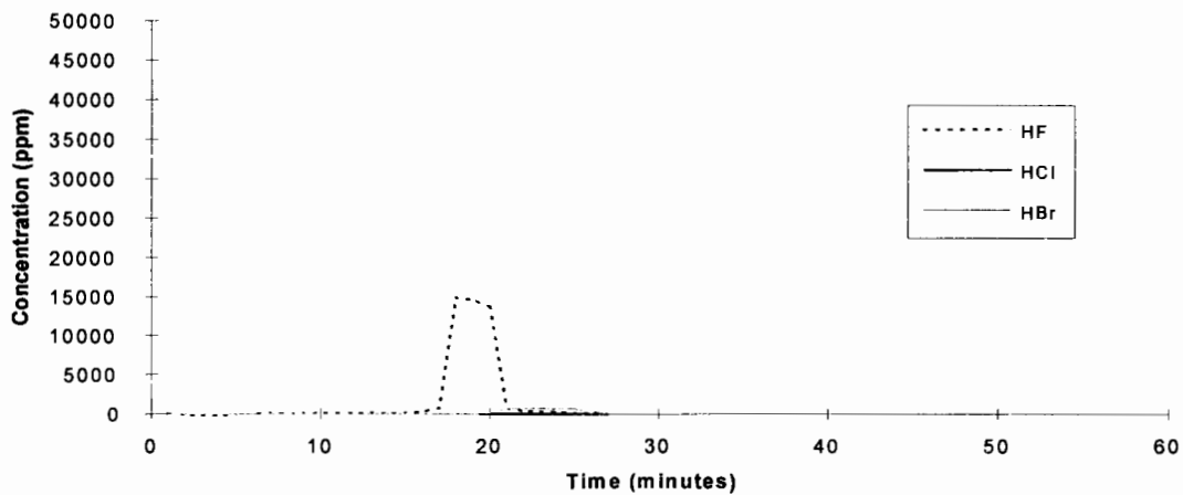
HBFC-22B1 - Test 3
