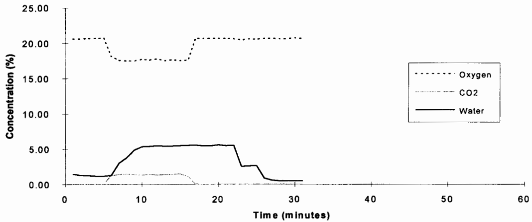
Halon 1301 - Test 2
