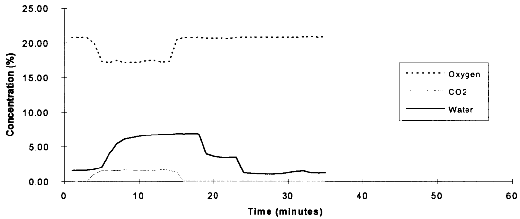
Halon 1211 - Test 1
