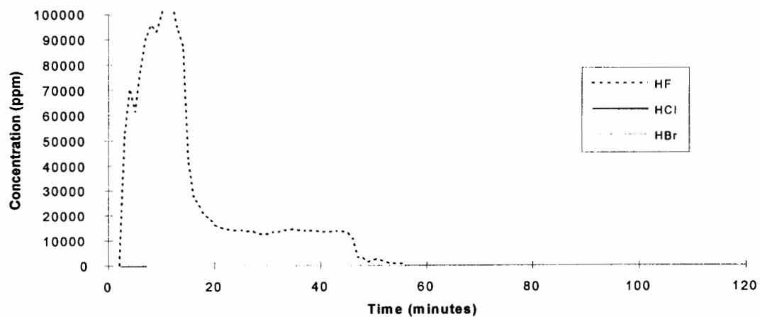
HFC 23 - Test 1
