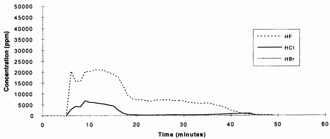
HCFC-123 - Test 2
