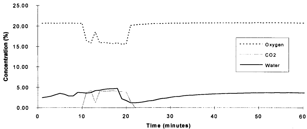
Perfluoropentane - Test 3
