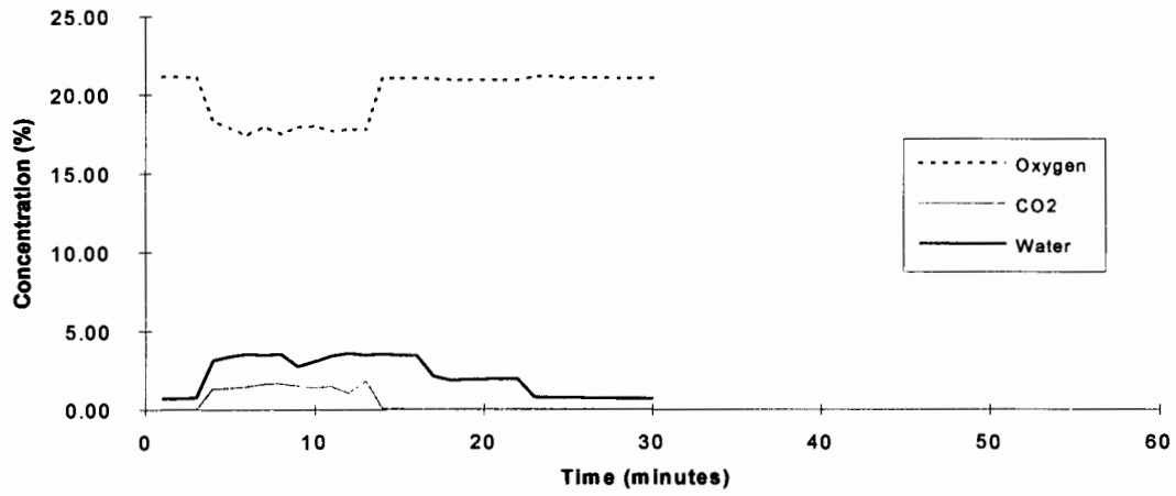
CF3I - Test 1
