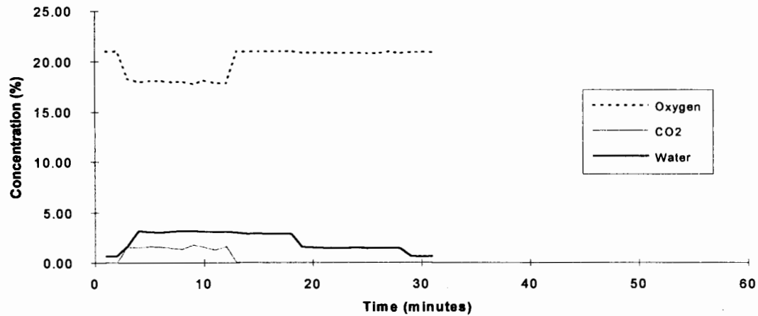
CF3I - Test 3
