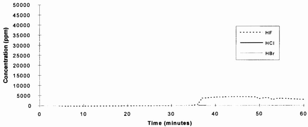
HFC-227EA - Test 3
