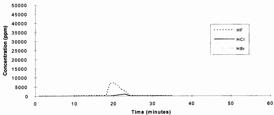
Halon 1211 - Test 1
