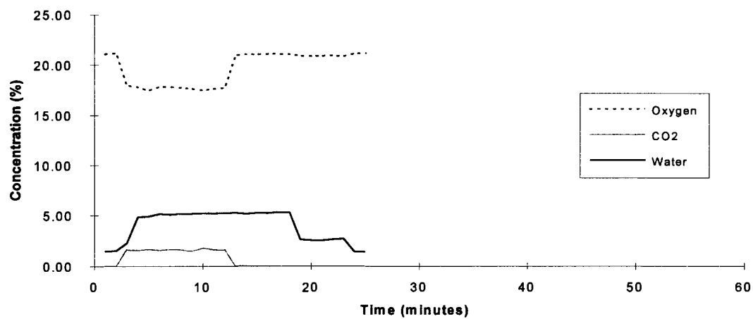
HBFC-22B1 - Test 1
