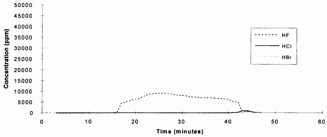
HFC-125 - Test 1
