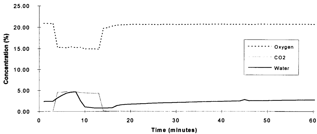
Perfluoropentane - Test 1
