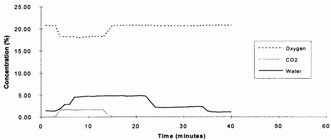
HFC-227EA - Test 2
