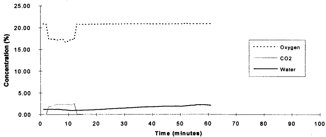
C3F7I - Test 3
