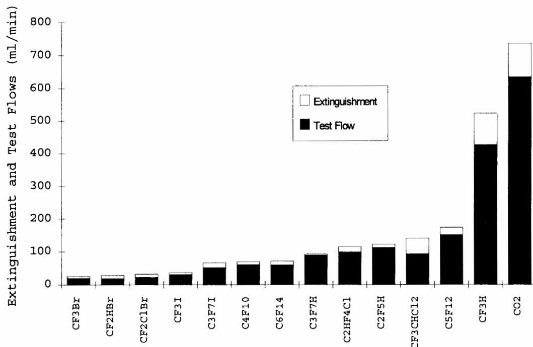
FIGURE 2. AGENT COMPARISON
