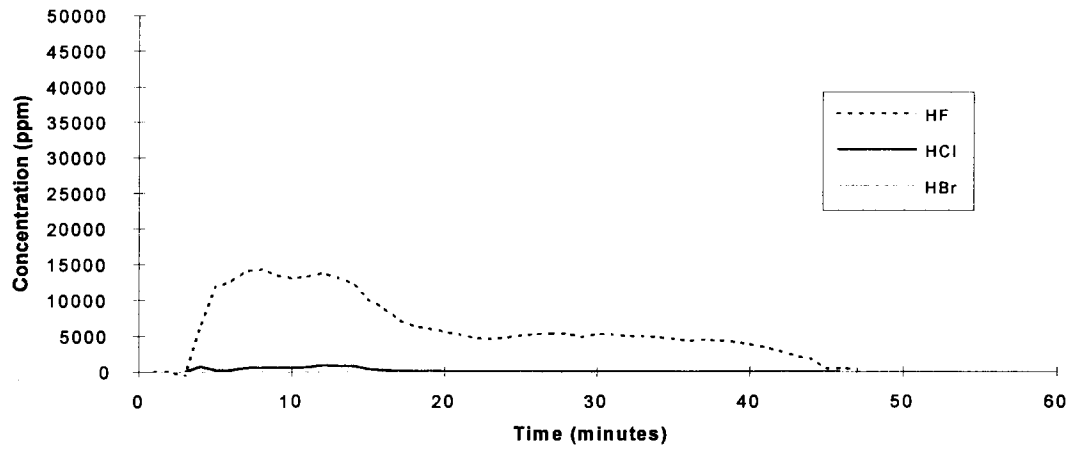
HCFC-124 - Test 1
