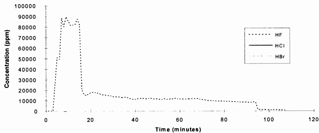
HFC 23 - Test 3
