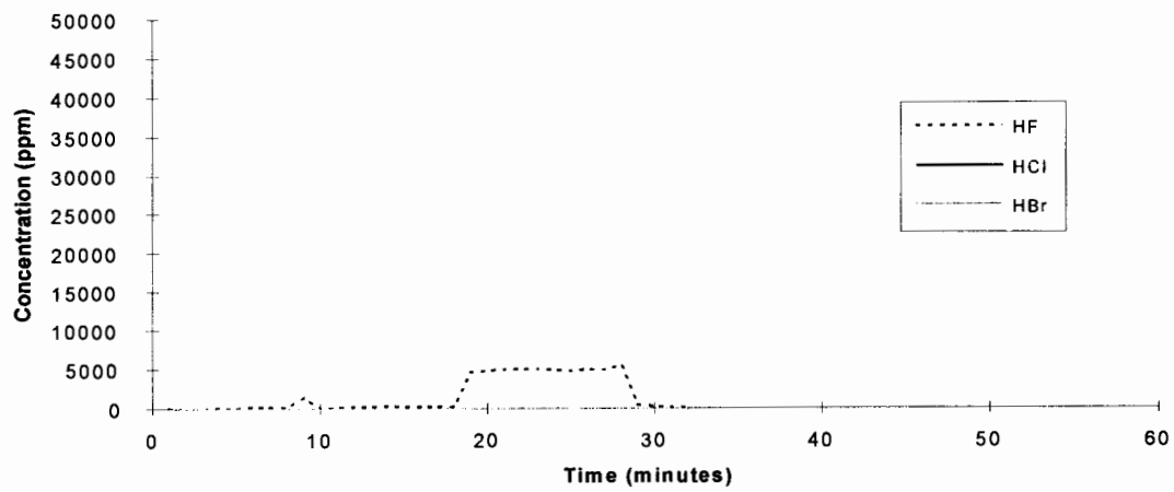
CF3I - Test 2
