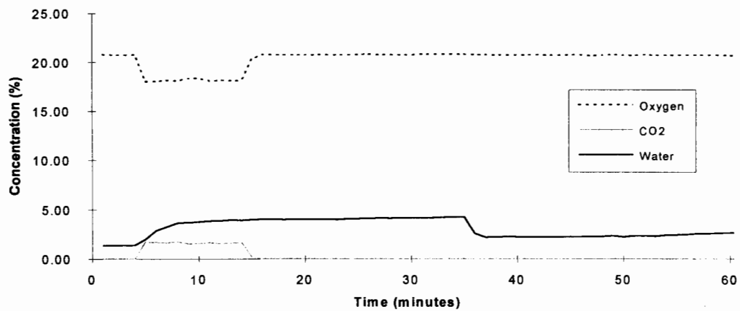
HFC-227EA - Test 3
