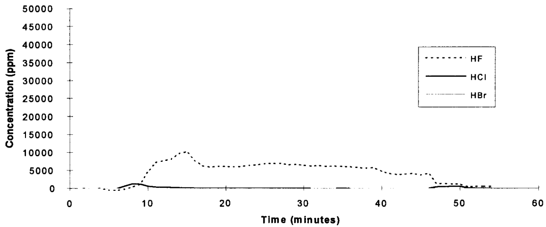
HCFC-124 - Test 3
