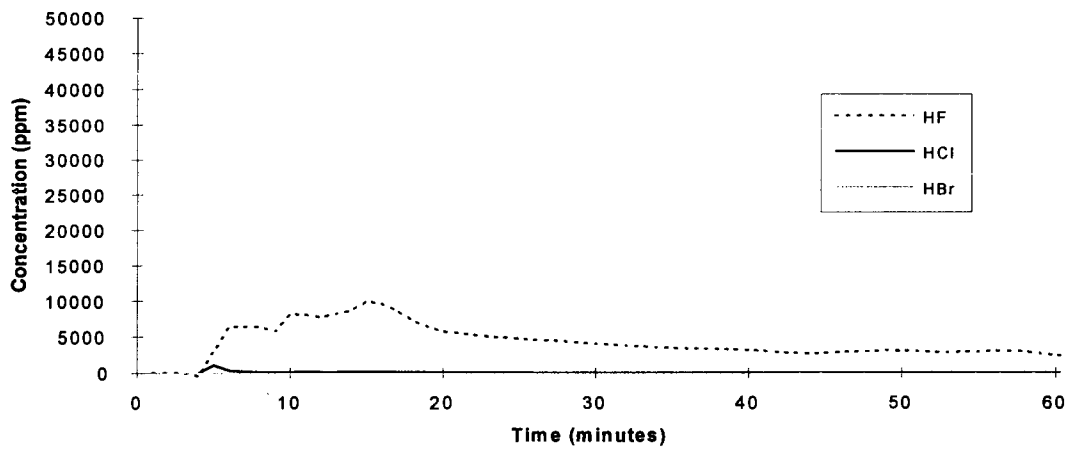
HCFC-124 - Test 2
