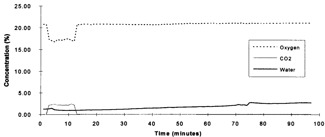
C3F7I - Test 1
