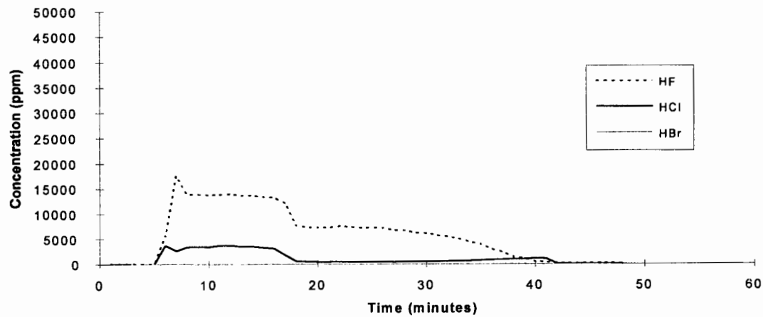
HCFC-123 - Test 3
