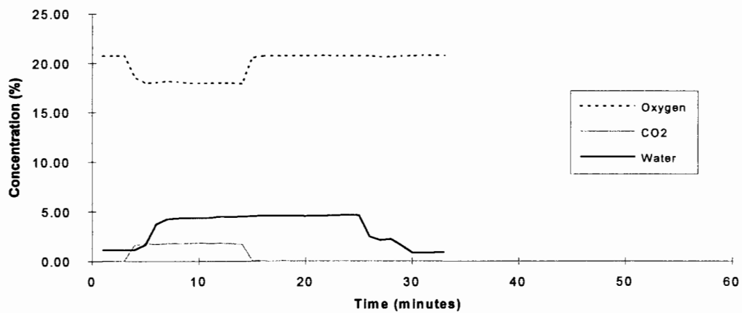
HFC-227EA - Test 1
