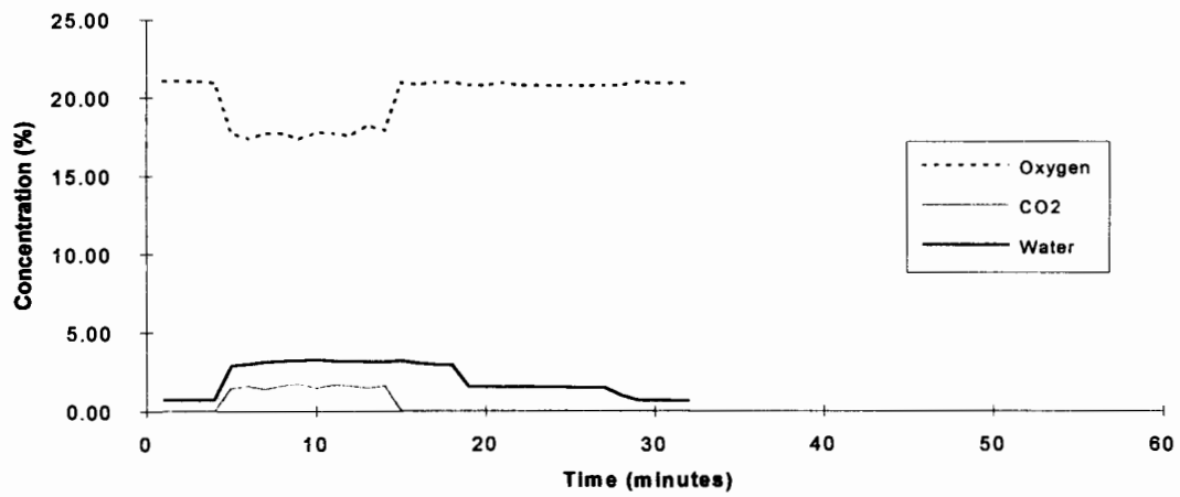
CF3I - Test 2
