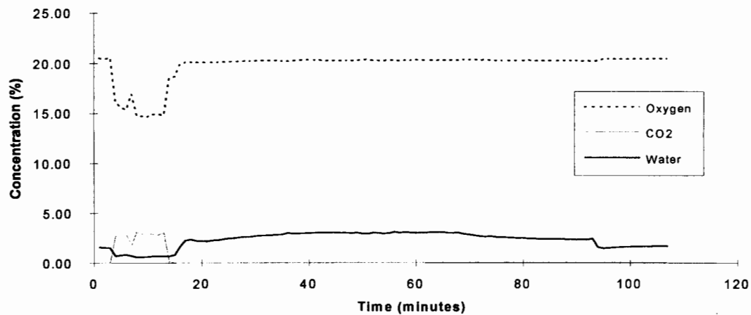
HFC 23 - Test 3
