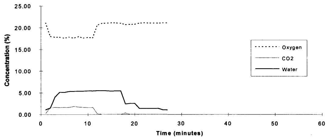
HBFC-22B1 - Test 3
