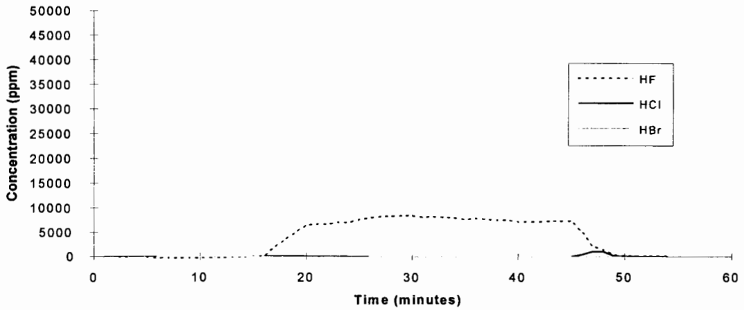
HFC-125 - Test 3
