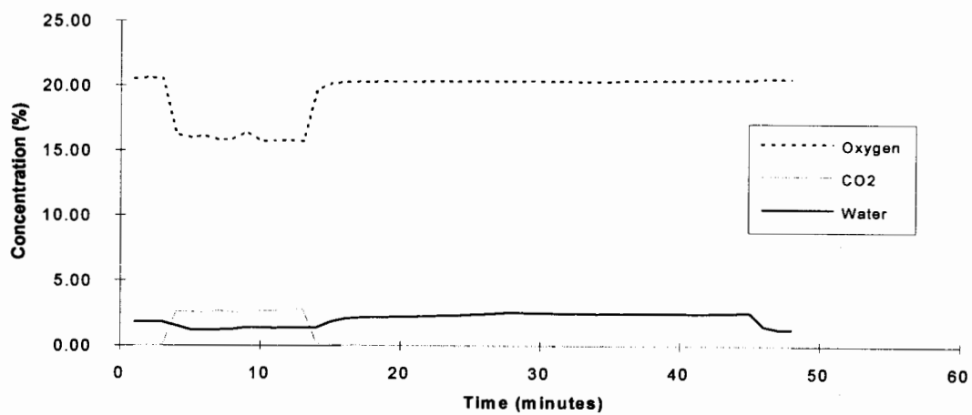
HCFC-123 - Test 1
