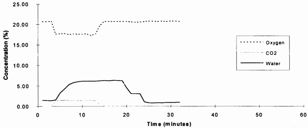
Halon 1301 - Test 3
