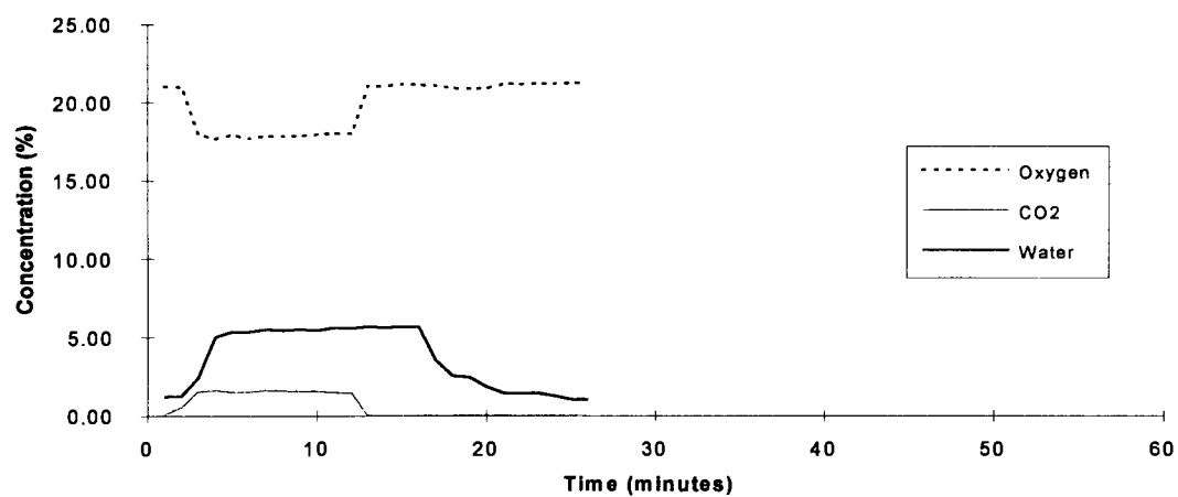
HBFC-22B1 - Test 2
