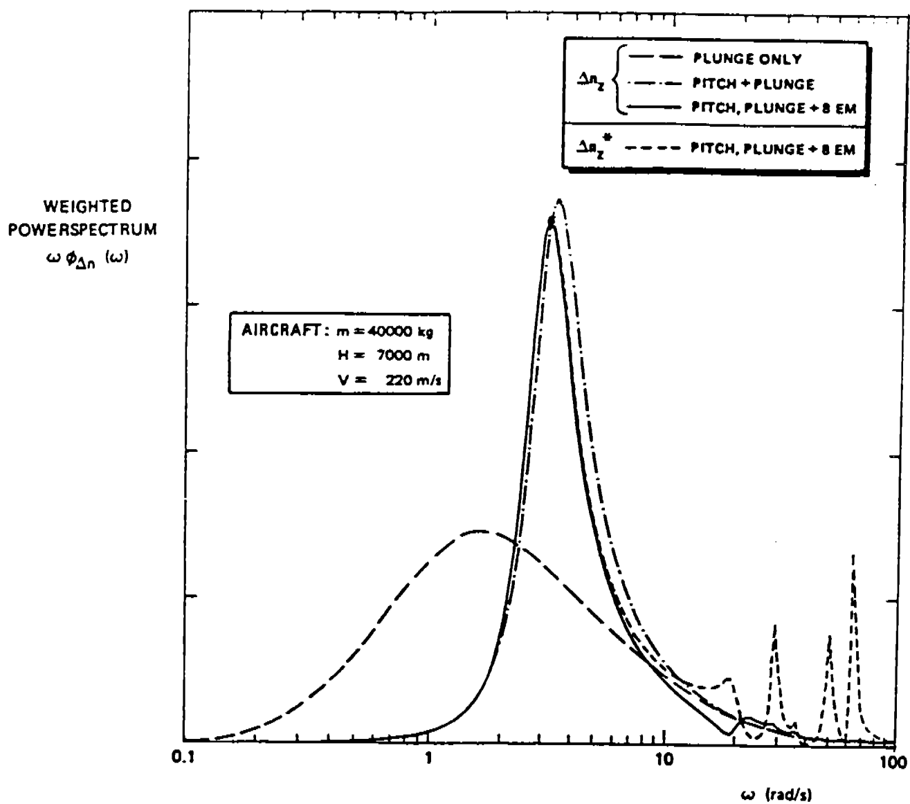
FIGURE A1. WEIGHTED POWERSPECTRUM OF DUE TO TURBULENCE FOR TWIN-ENGINE SHORT HAUL TRANSPORT AIRCRAFT
