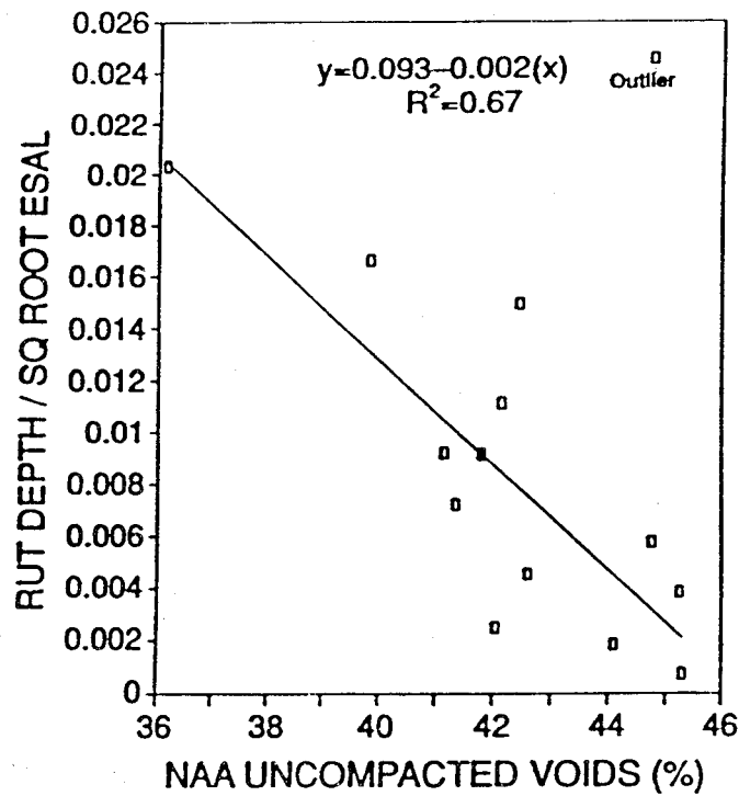
Figure 7. Relationship between NAA uncompact voids and rate of rutting 36
