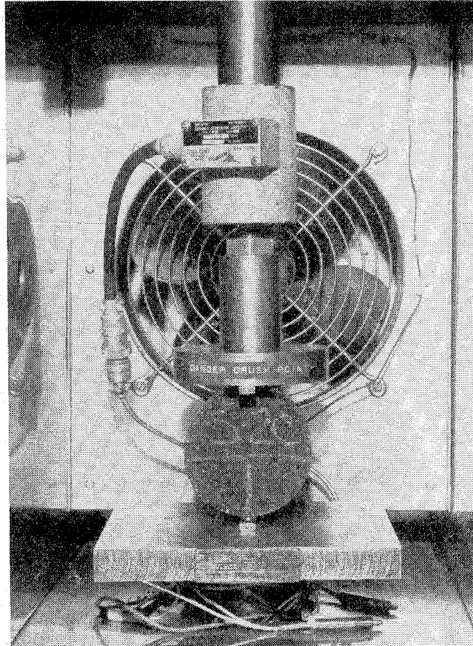
Figure 18. Indirect Tensile Test
