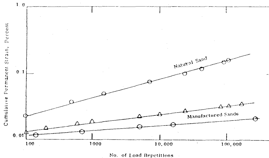
Figure 1. Typical relationship between permanent deformation and type of sand 19
