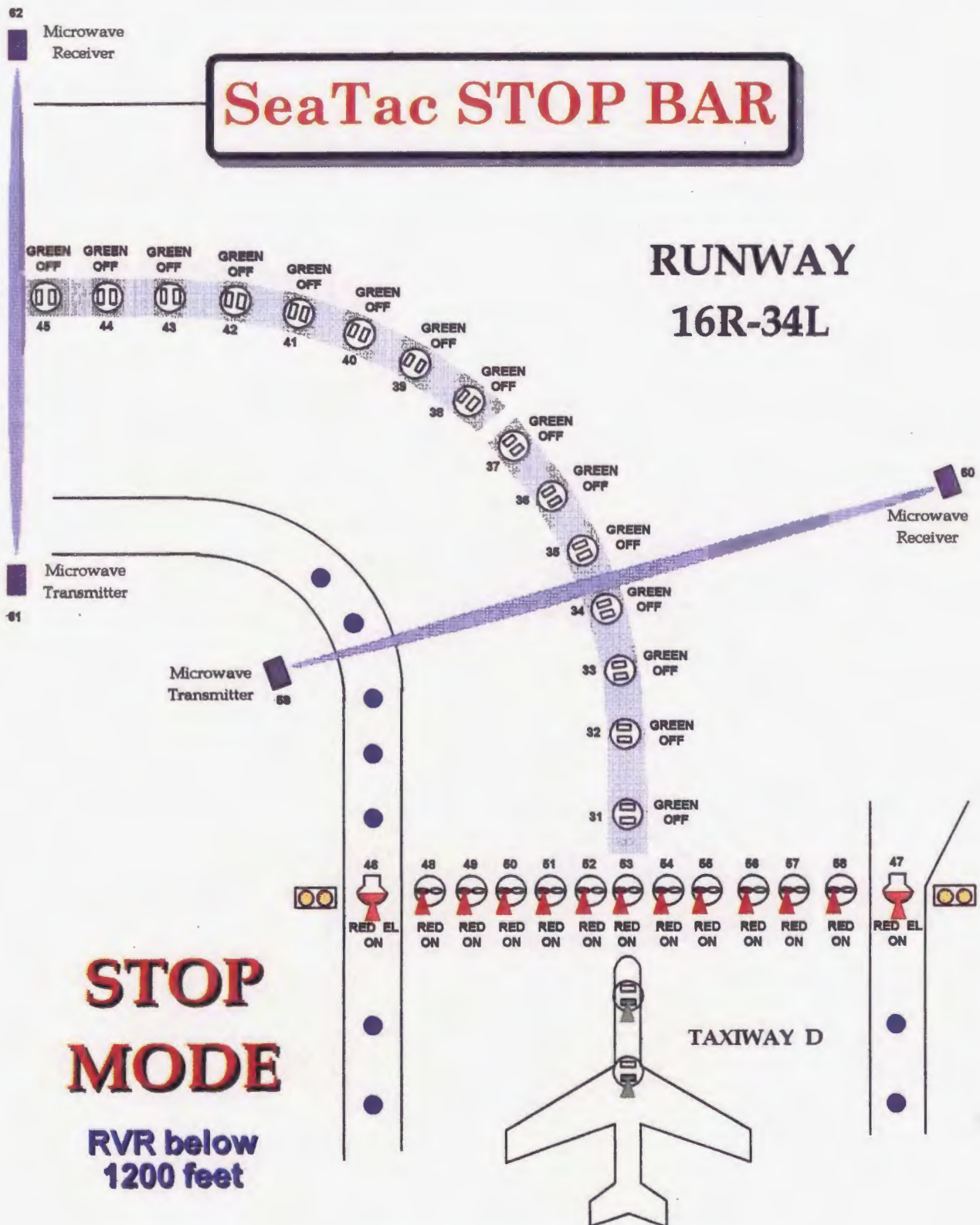
FIGURE 8. TAXIWAY D STOP MODE CONFIGURATION
