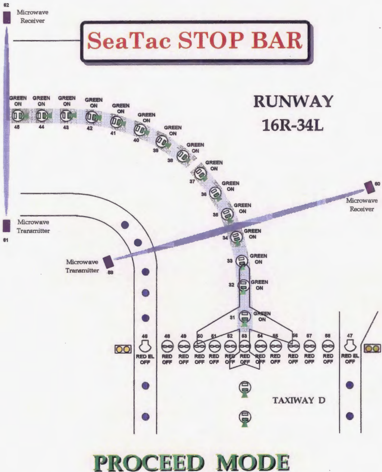
FIGURE 9. TAXIWAY D PROCEED (CLEARED) MODE CONFIGURATION
