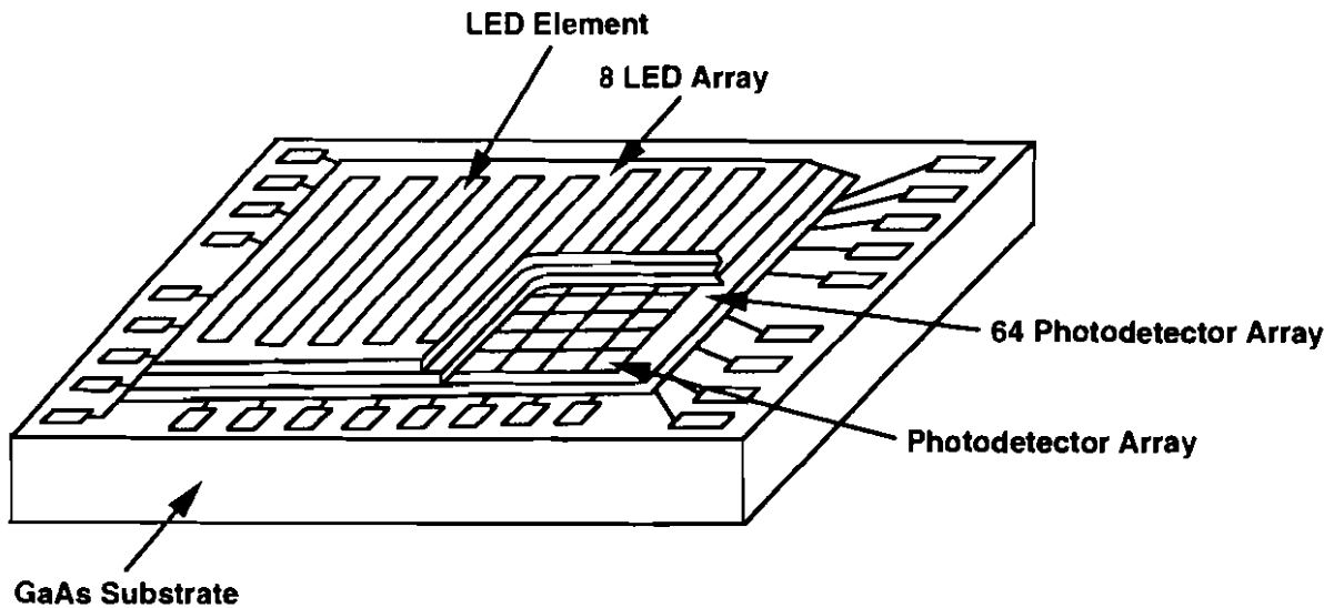
FIGURE 3.2-2. OPTICAL NEURAL COMPUTING INTEGRATED CIRCUIT (Mitsubishi 1992)
