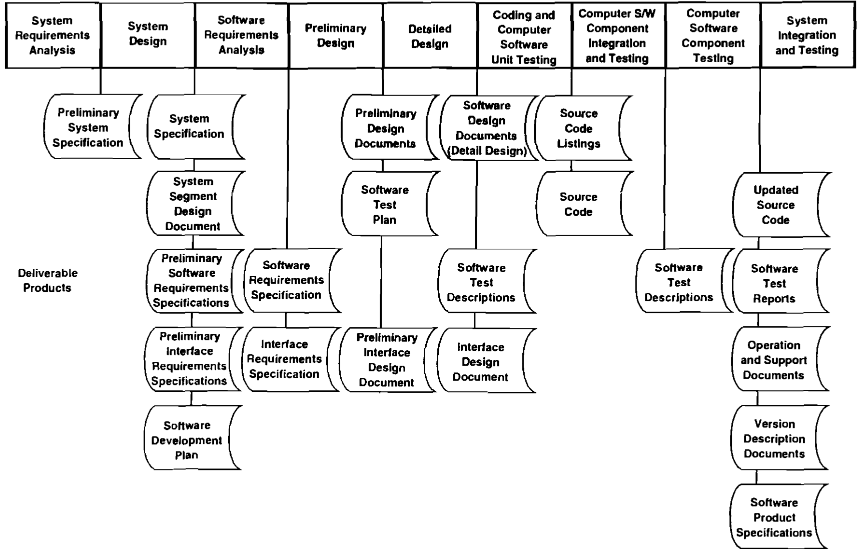
FIGURE 5.4-1. SYSTEM DEVELOPMENT CYCLE (DOD-STD-2167A)
