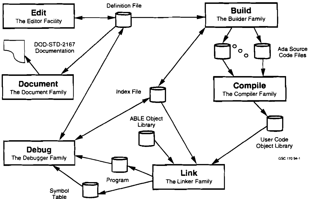
FIGURE 3.1-1. ELEMENTS OF THE BABBAGE TOOL AND THEIR RELATIONSHIPS (Leeper 1990)
