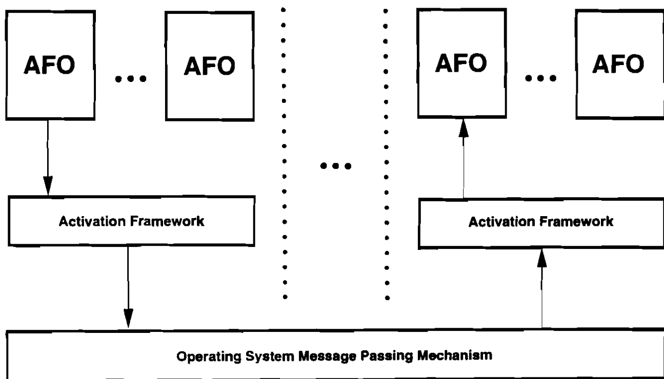
FIGURE 4.1-1. FTPP ARCHITECTURE (Masotto, Babikyan, and Harper 1990)
