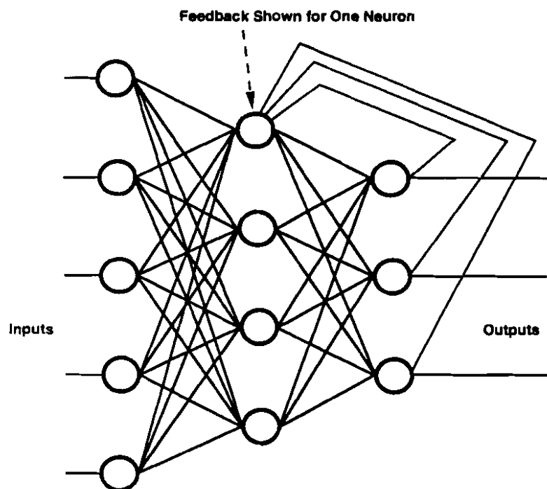
FIGURE 2.4-4. A FEEDBACK NEURAL NETWORK
