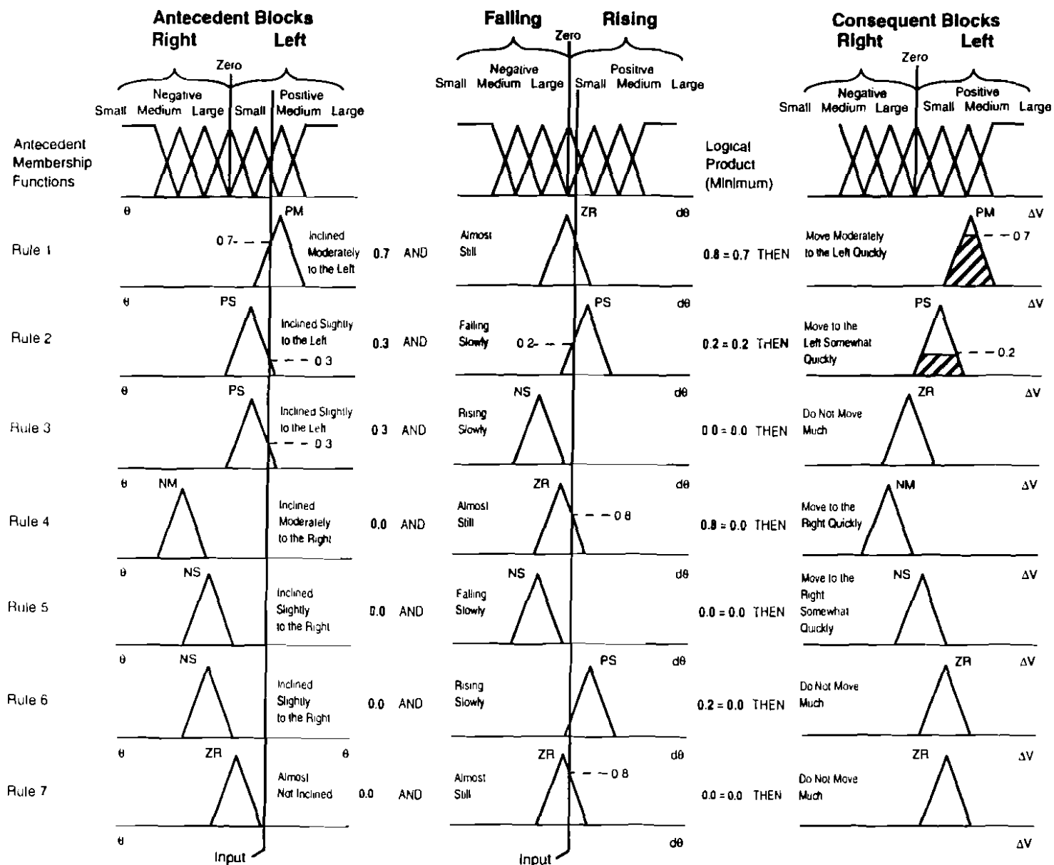
FIGURE 2.3-3. OBTAINING THE LOGICAL PRODUCT
