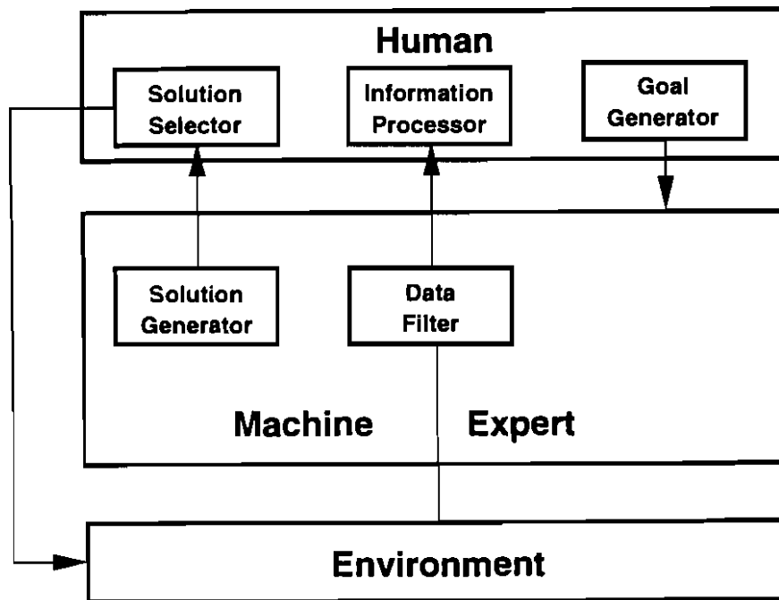
FIGURE 6.4-2. IMPROVED HUMAN PERFORMANCE GENERATOR (Wiener and Nagel 1988)
