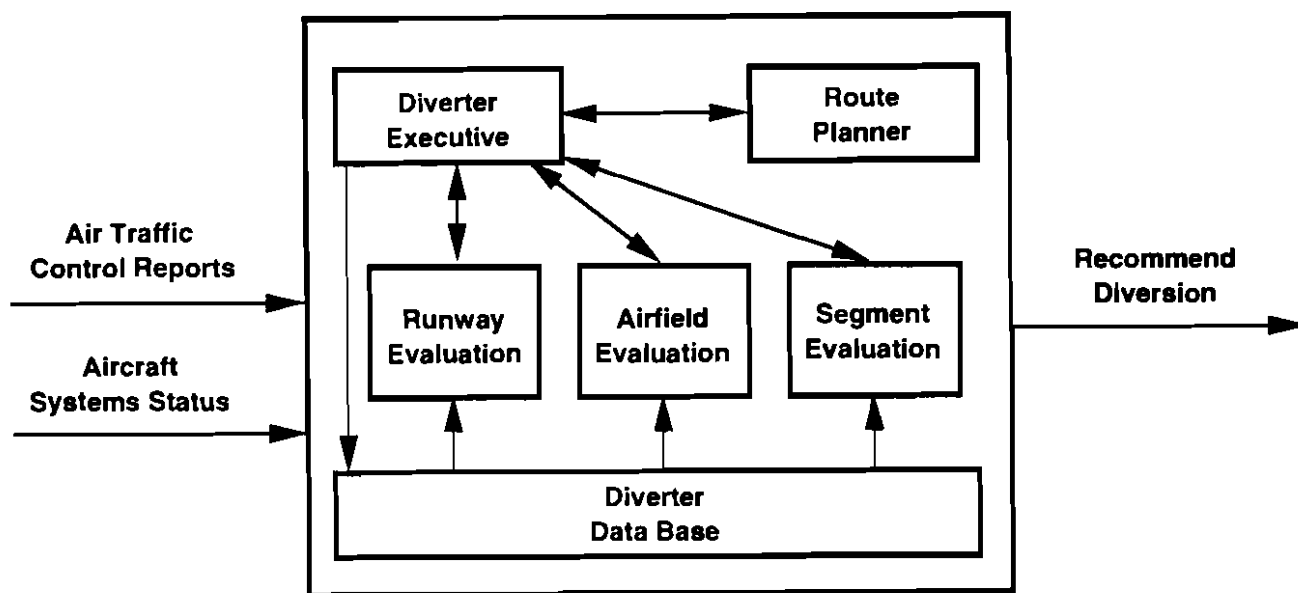
FIGURE 4.4-1. DIVERTER SOFTWARE ARCHITECTURE (Rudolph, Homoki, and Sexton 1990)
