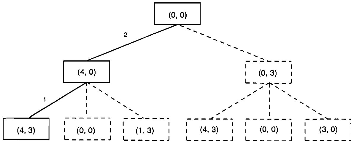
FIGURE 2.2-6. DEPTH FIRST SEARCH TREE (Rich and Knight 1991)
