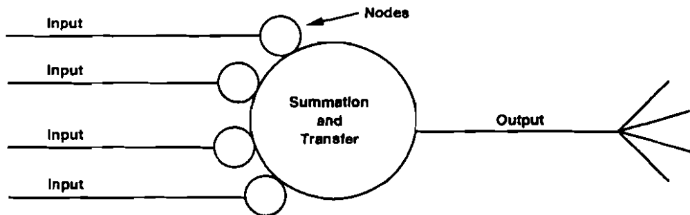
Artificial Neuron
