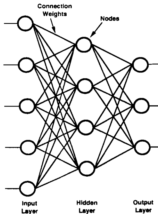
FIGURE 2.4-1. NEURAL NETWORK
