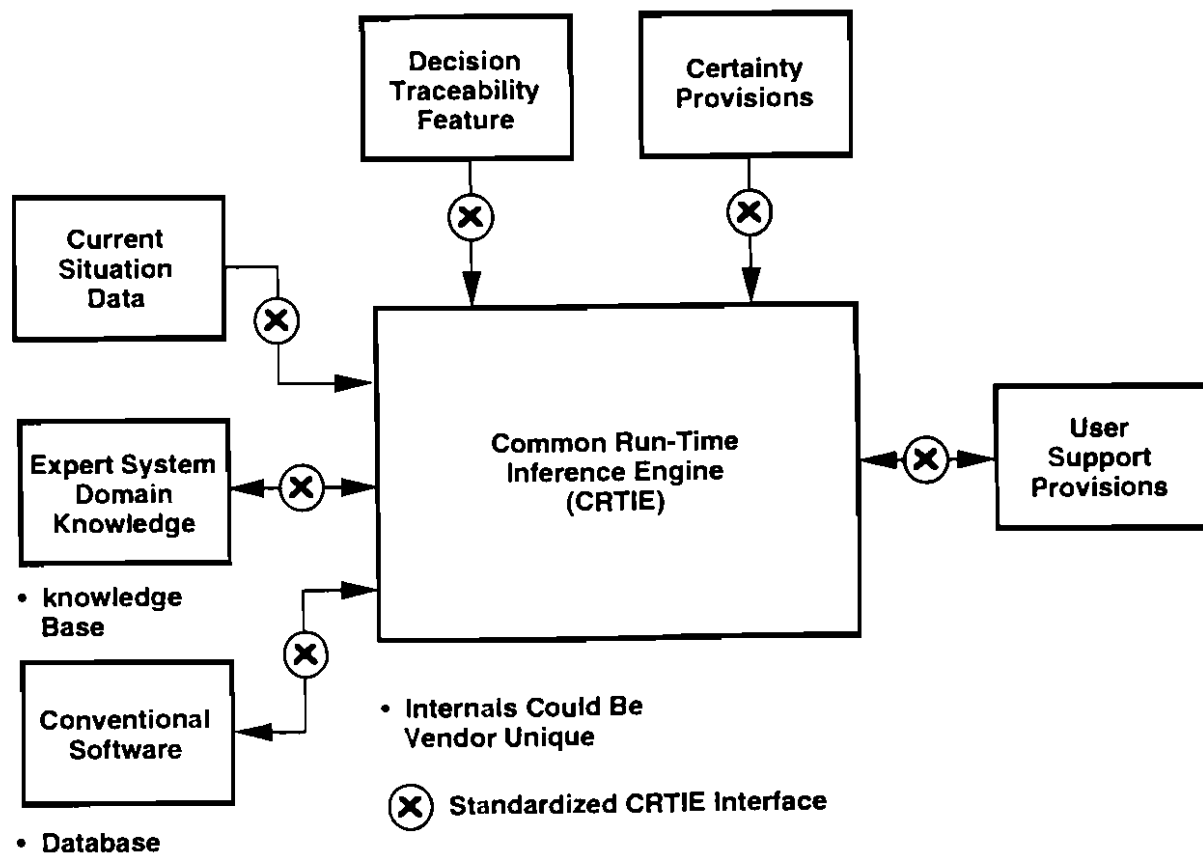
FIGURE 5.3-1. COMMON RUN-TIME INFERENCE ENGINE (Warn 1987)
