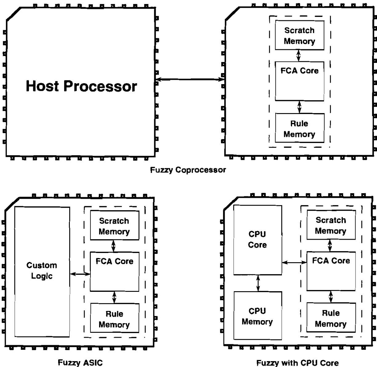
FIGURE 3.2-3. BASIC IMPLEMENTATIONS OF ASIC CORE USING FUZZY LOGIC (The Fuzzy Source 1992)
