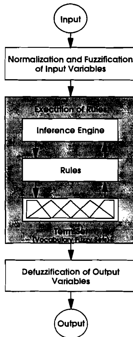
FIGURE 2.3-5. FUZZY CONTROLLER
