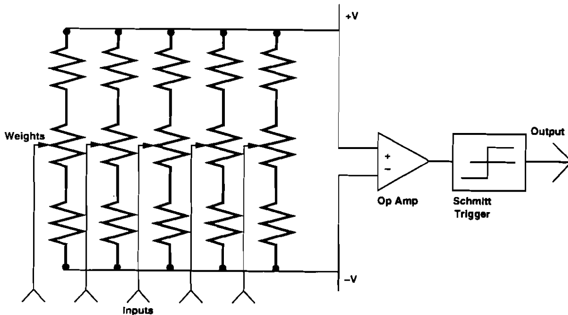
FIGURE 2.4-5. CONSTRUCTION OF A NEURAL NETWORK
