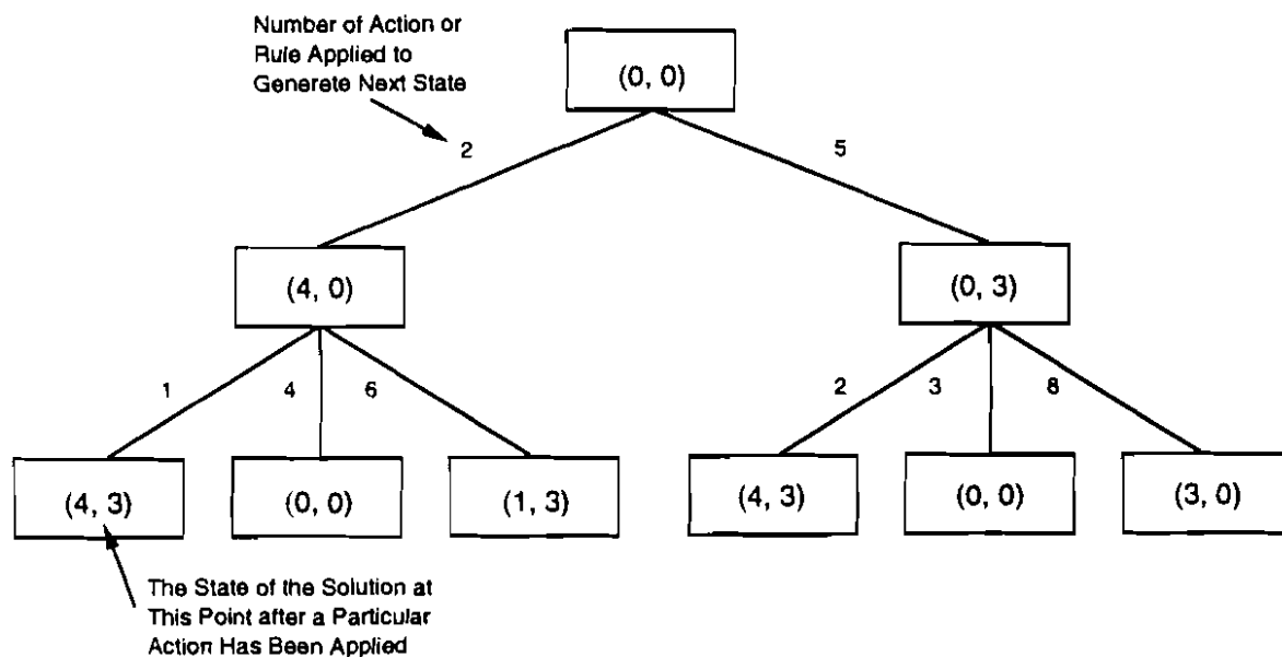
FIGURE 2.2-5. BREADTH FIRST SEARCH TREE (Rich and Knight 1991)
