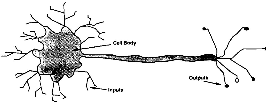
Biological Neuron
