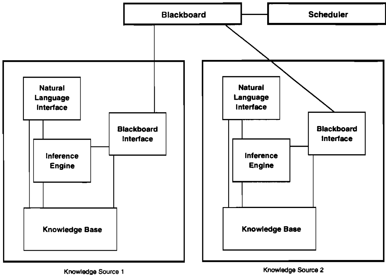
FIGURE 2.2-7. BLACKBOARD SYSTEM ARCHITECTURE
