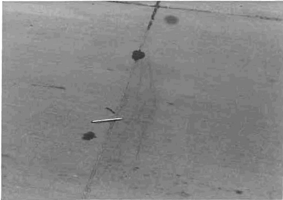
Photo 3: Shrinkage Cracking
