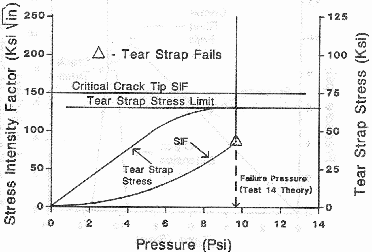
Figure 6-11. Analytic Predictions for 24-in. Crack
