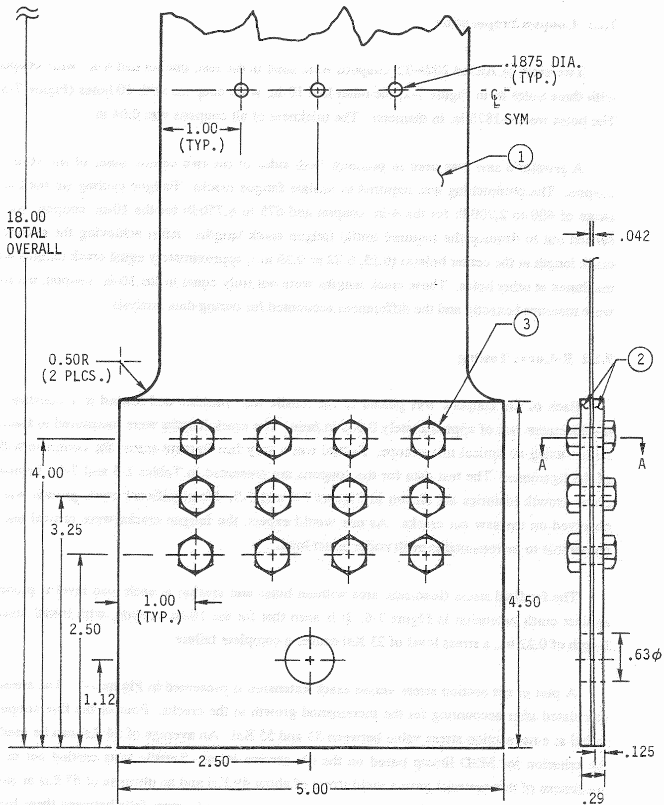
Figure 7-2. Four-Inch Coupon Configuration
