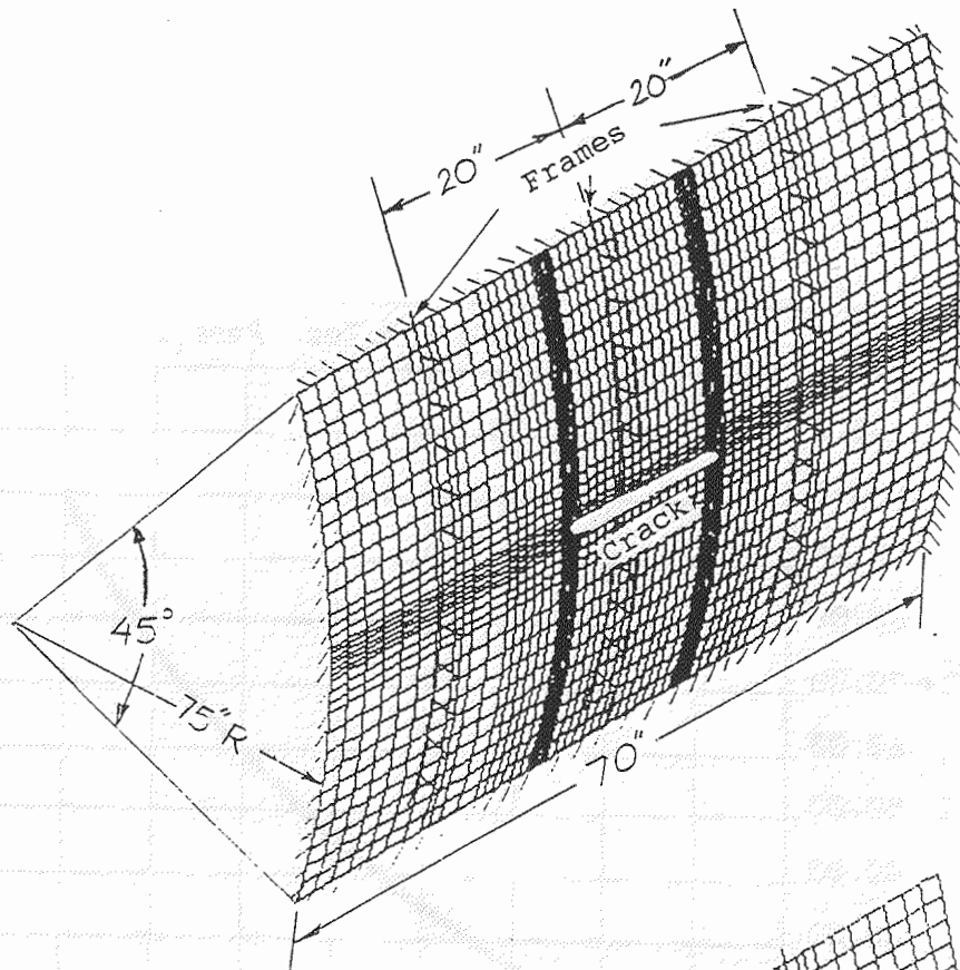
(a) STIFFENED SHELL MODEL WITH 16 INCH CRACK
