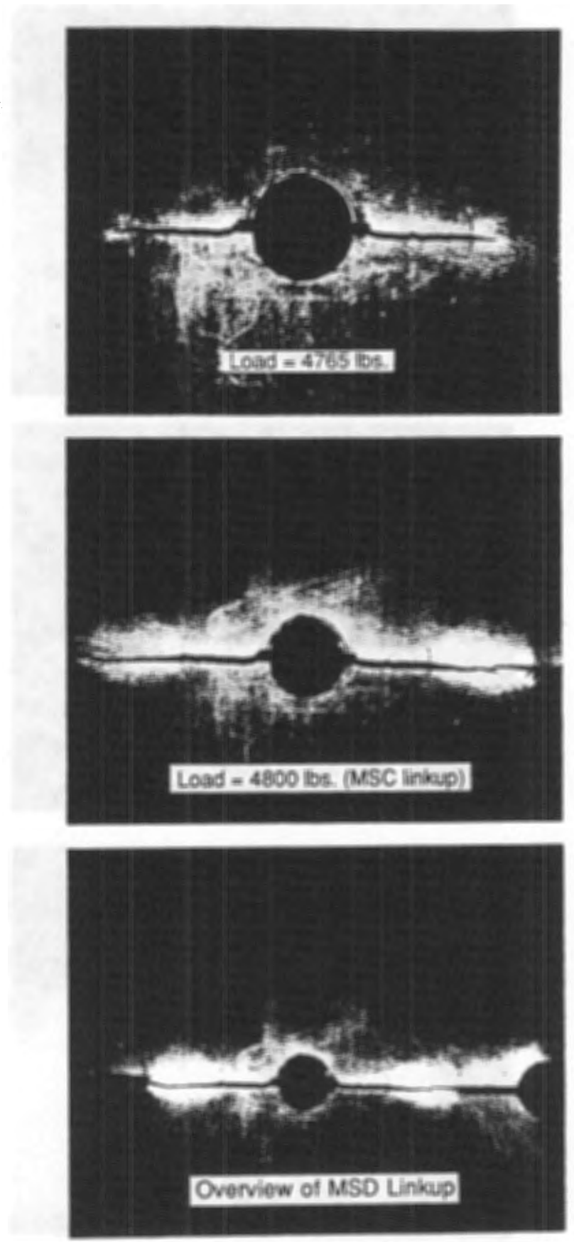
Figure 7-5. R-Curve Test Final Crack Growth
