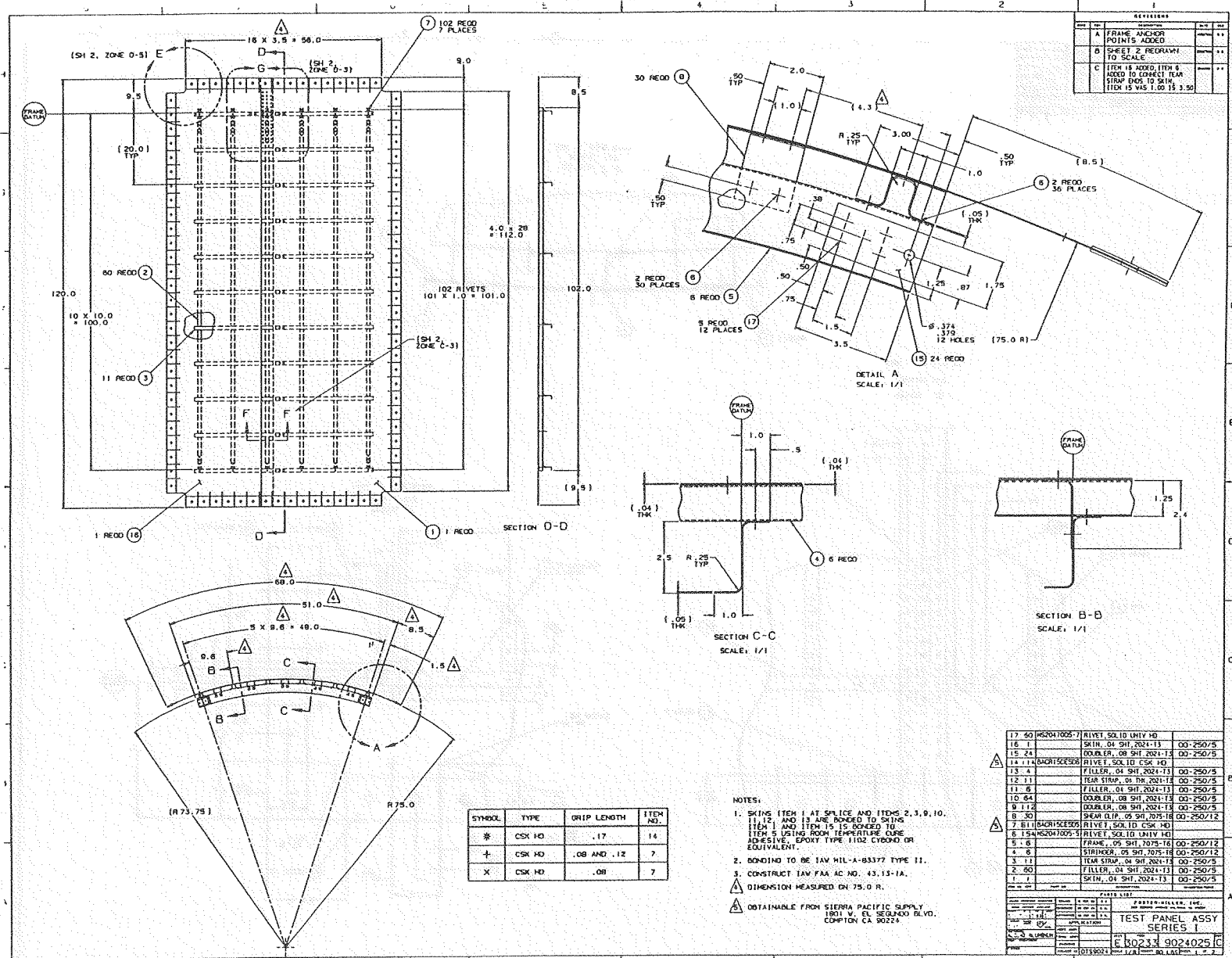
Figure 4-3. Test Panel 2
