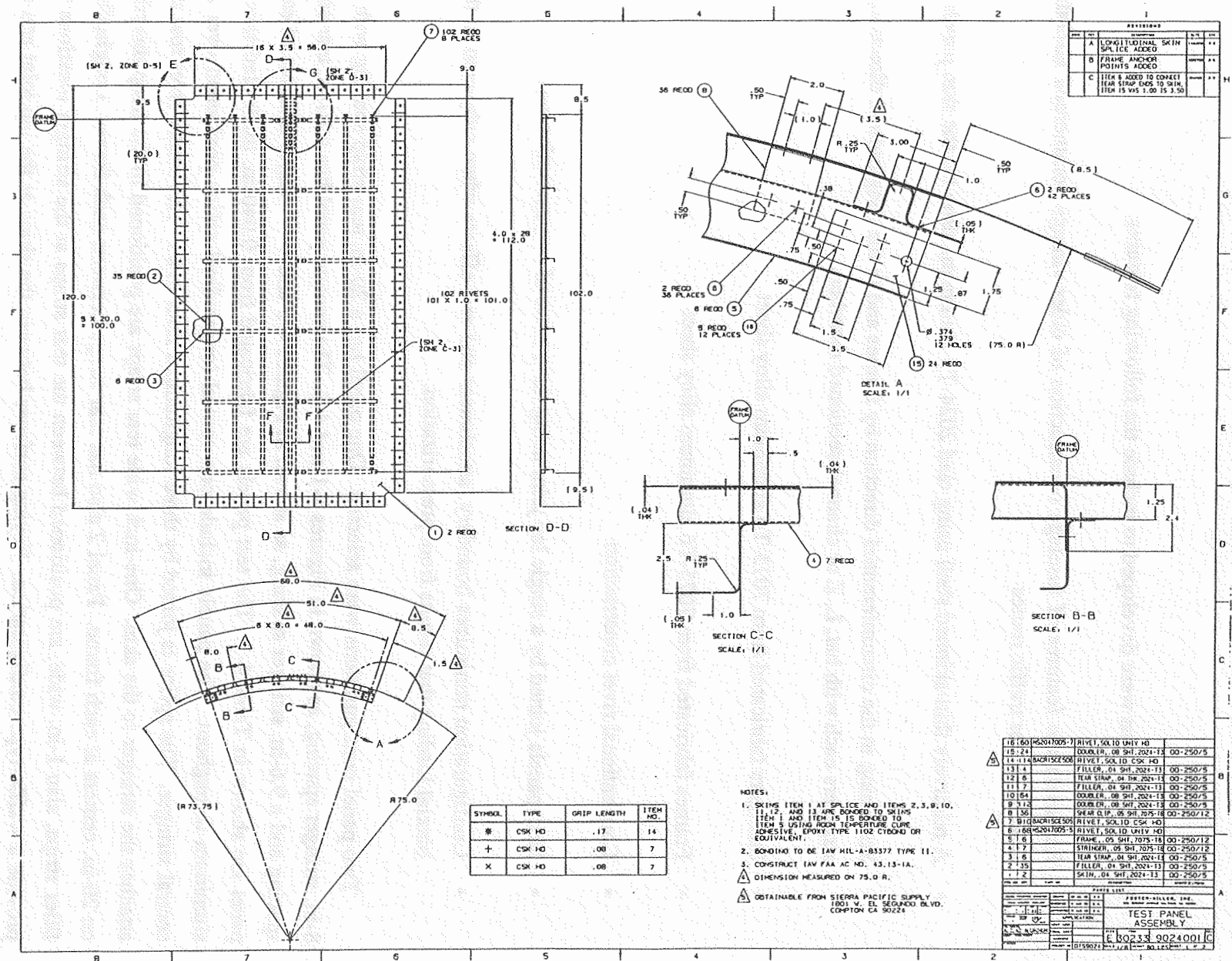
Figure 4-1. Test Panel 1
