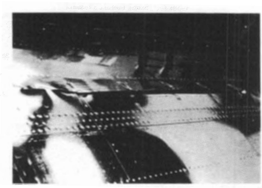
Figure 6-13. Fractured Panel with Initial 36-in. Crack
