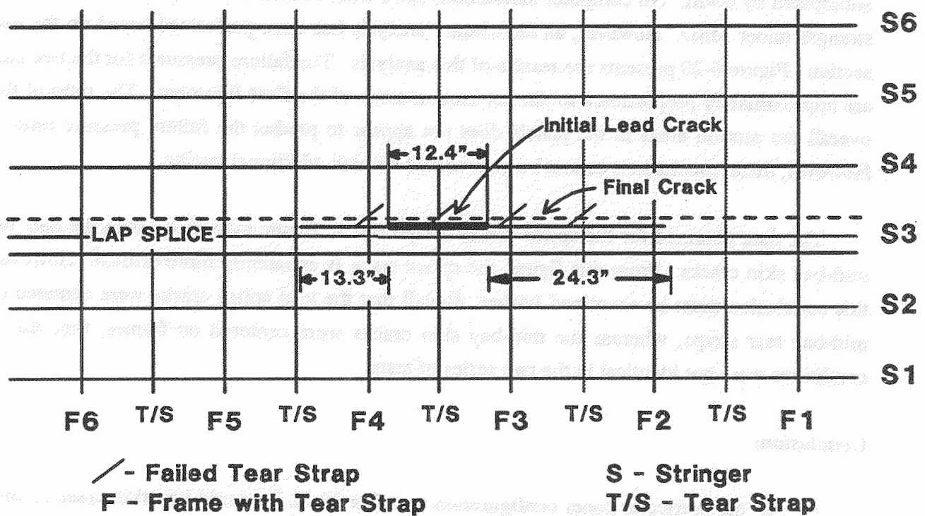
b) INITIAL AND FINAL DAMAGE
