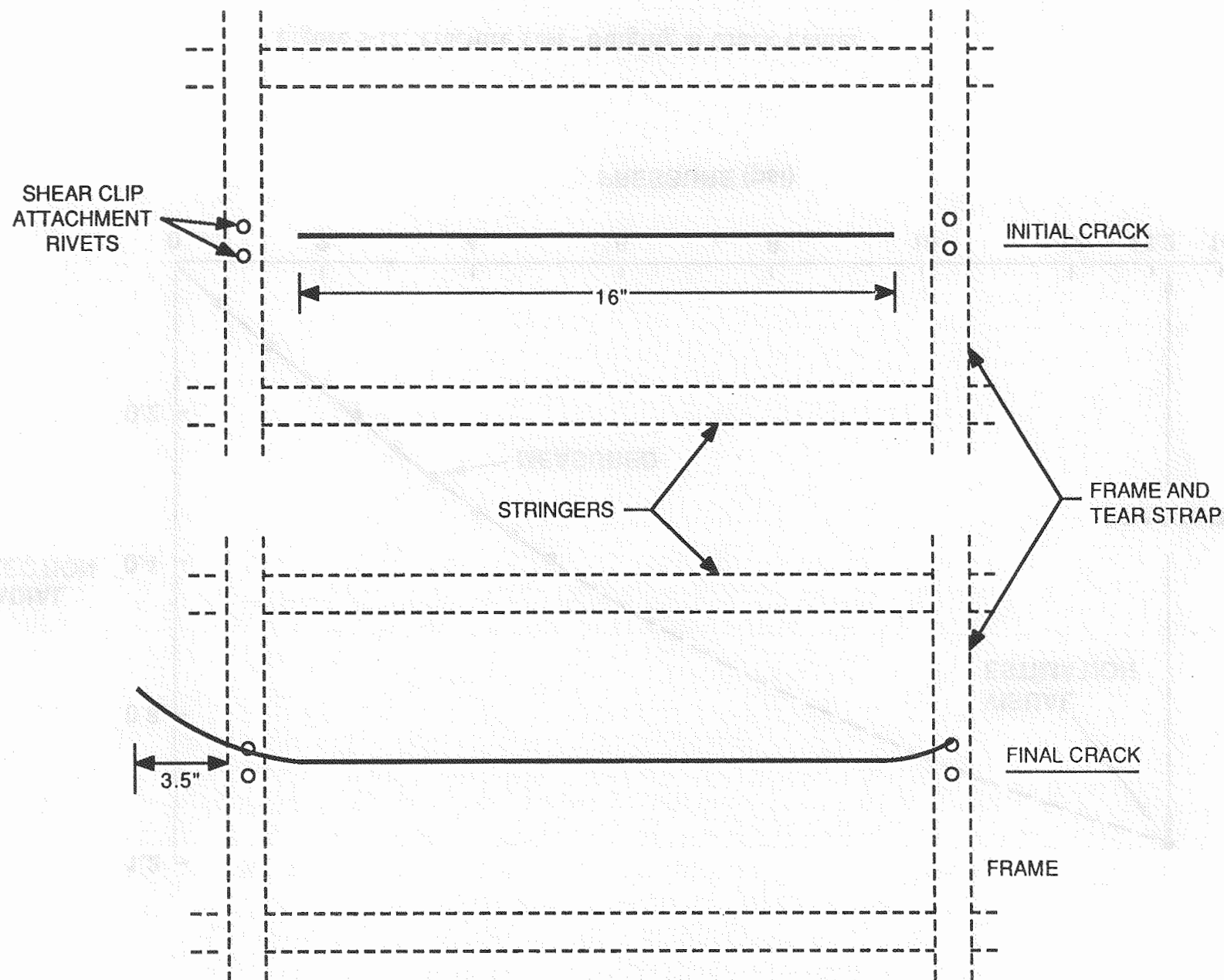
Figure 5-11. Panel Fracture
