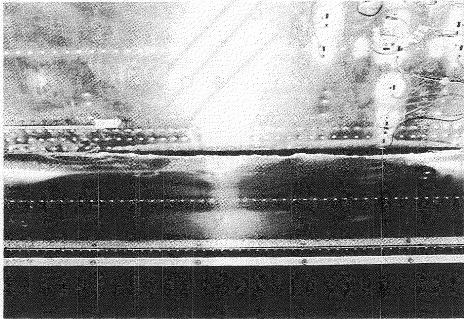
Figure 5-16. Catastrophic Panel Failure
