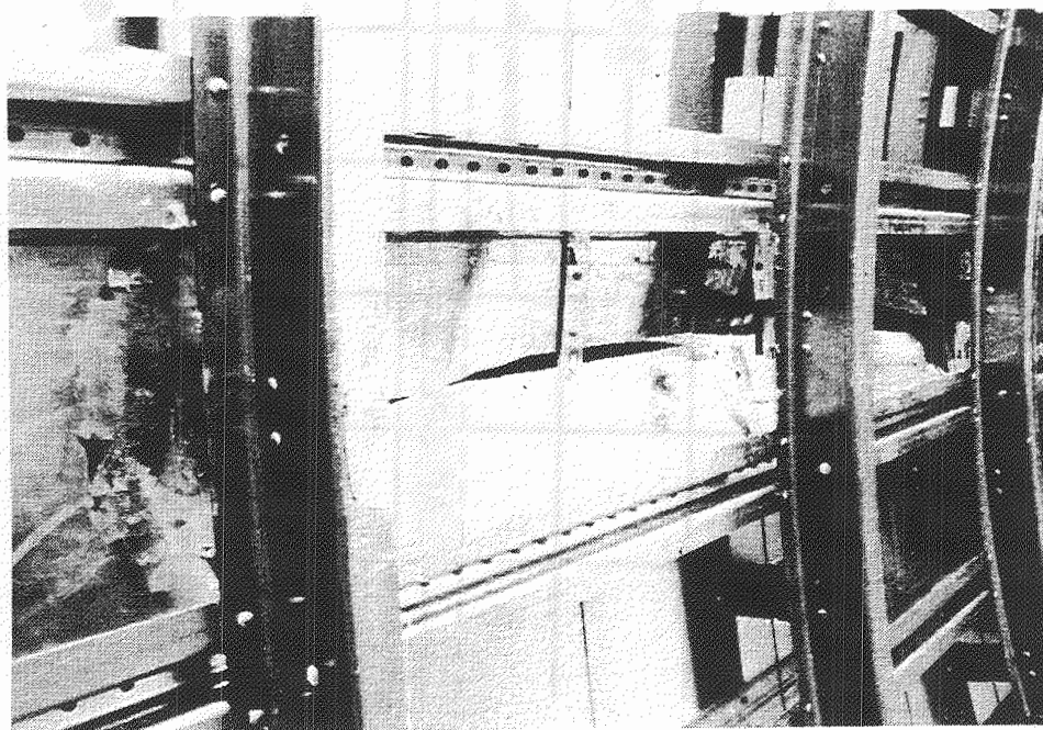
Figure 6-8. Underside View of Damaged Panel with 24-in. Initial Crack
