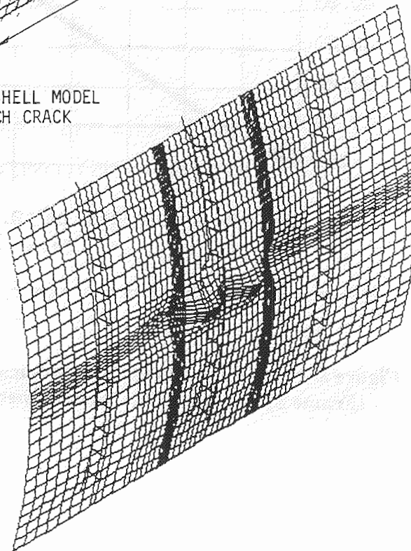
(b) BULGING DEFORMATION UNDER INTERNAL PRESSURE
