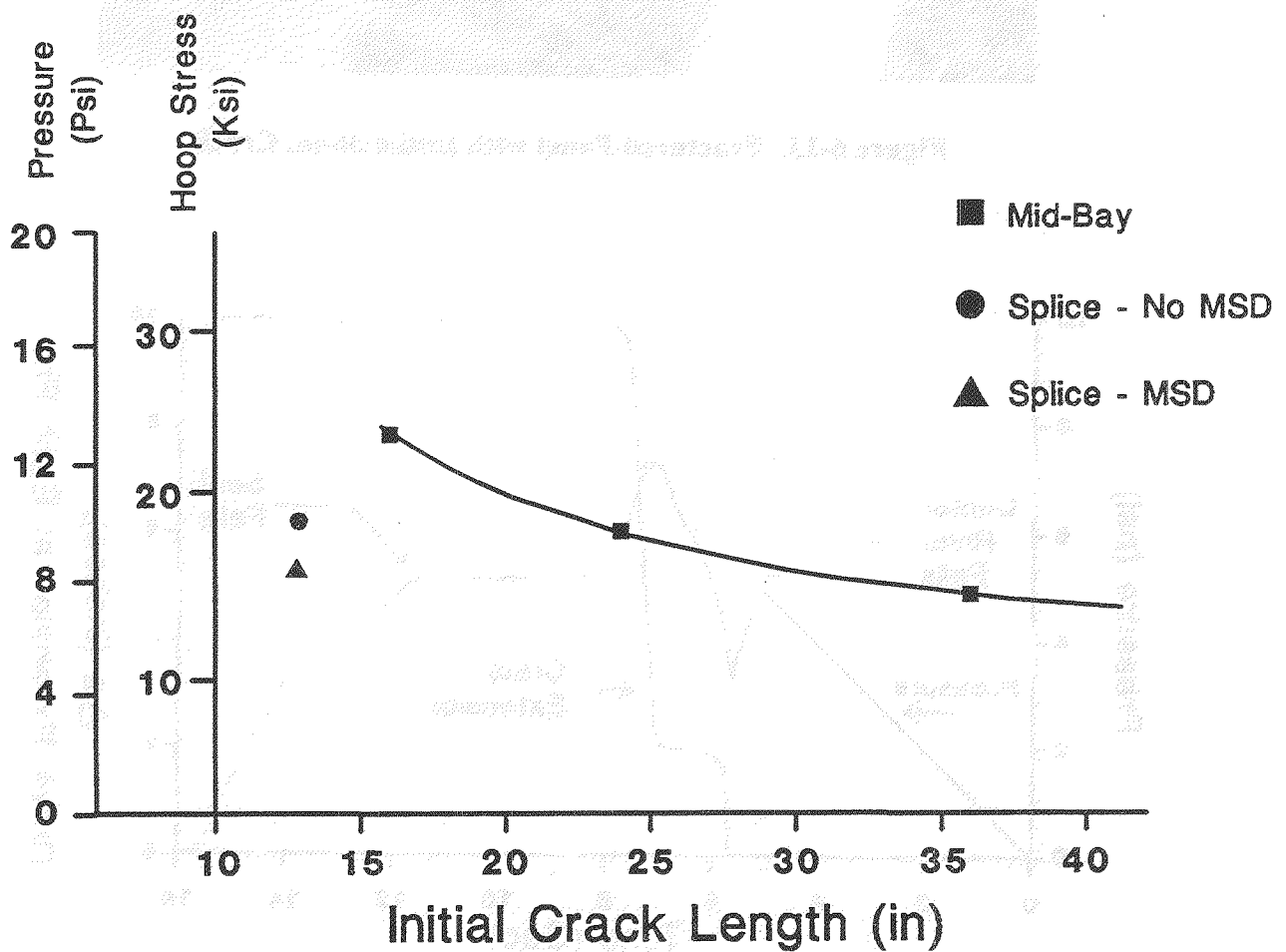
Figure 6-15. Test Results on Failure Pressures/Residual Strength
