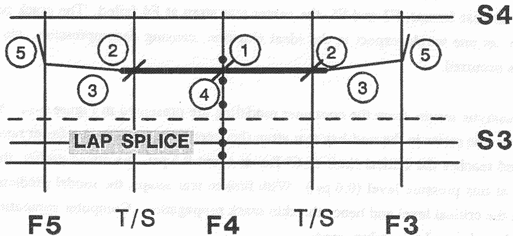
Figure 6-10. Failure Event Sequence for Panel with Initial 24-in. Crack
