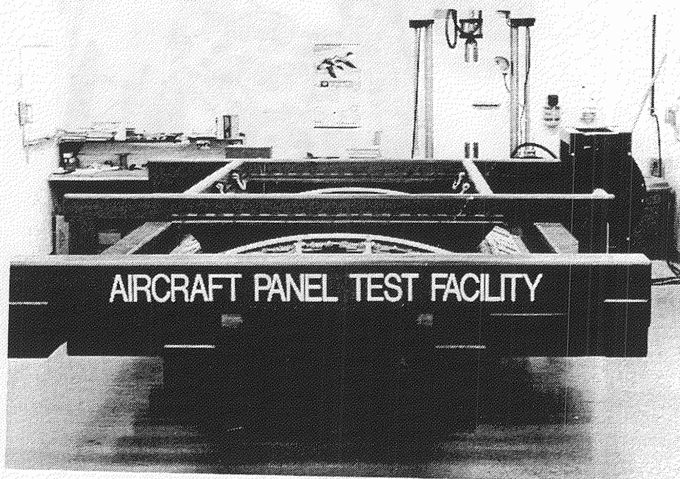
Figure 3-14. Test Fixture Structure
