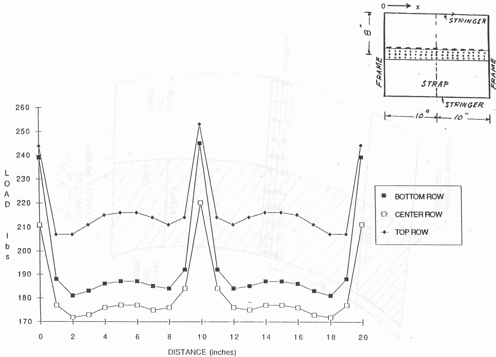
Figure 8-9. Rivet Load Distribution
