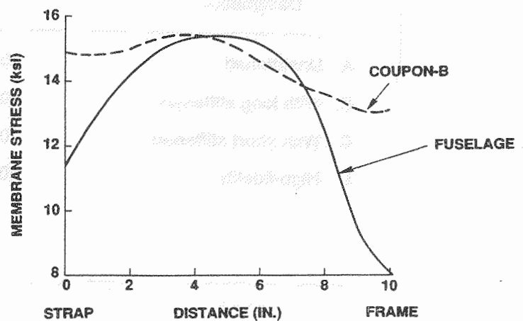
Figure 8-6b. Comparison of Stress Distribution in the Fuselage and Coupon with Staff Stiffeners
