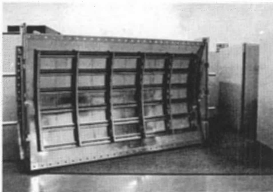
Figure 4-6. Interior of Test Panel
