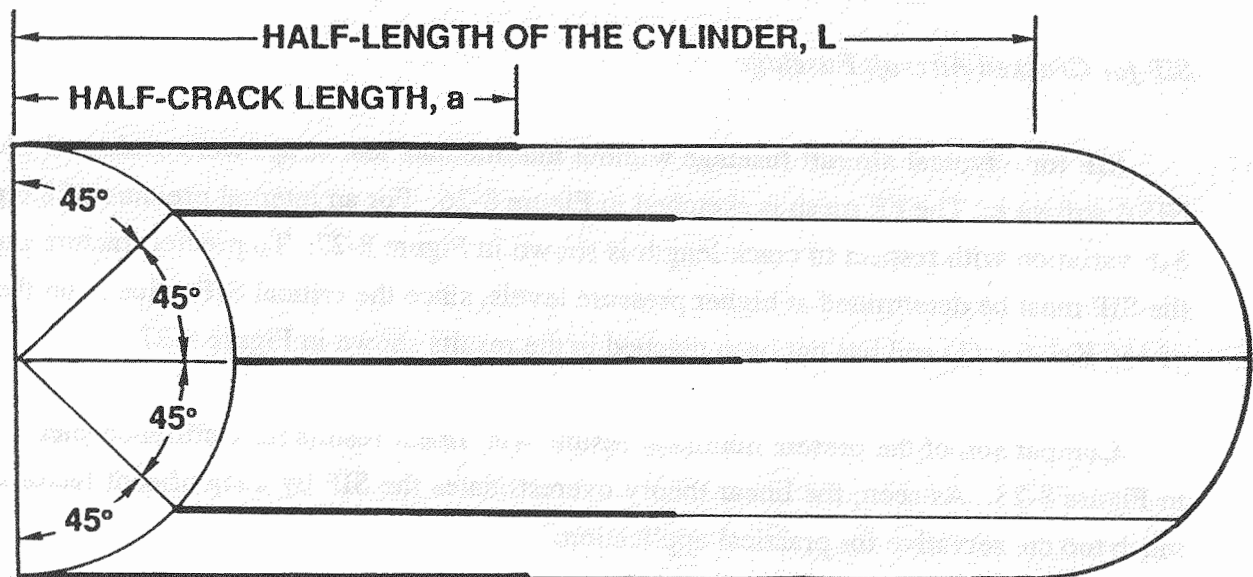
Figure 8-23. Method for SIF Calculation
