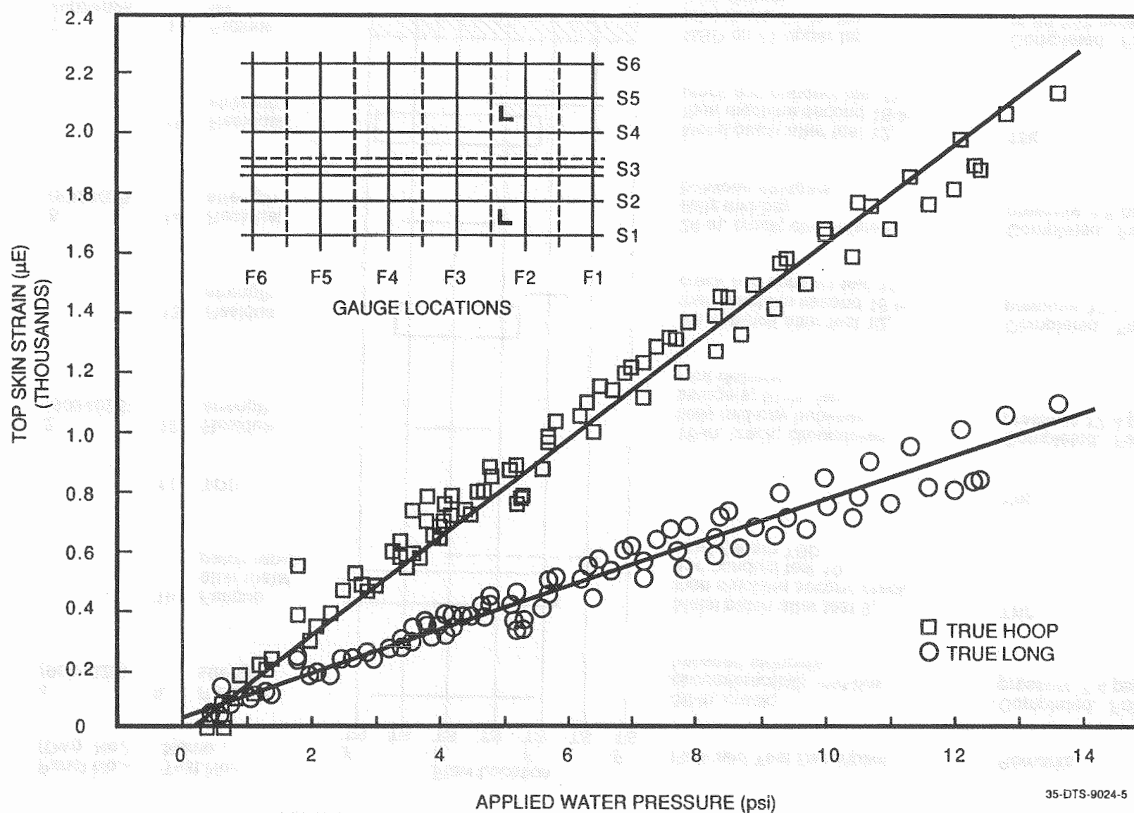
Figure 6-1. True Hoop and Longitudinal Top Skin Strains
