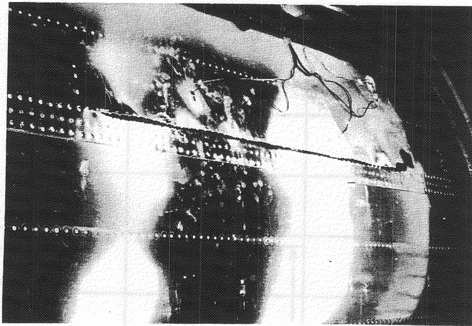
a) FRACTURED PANEL
