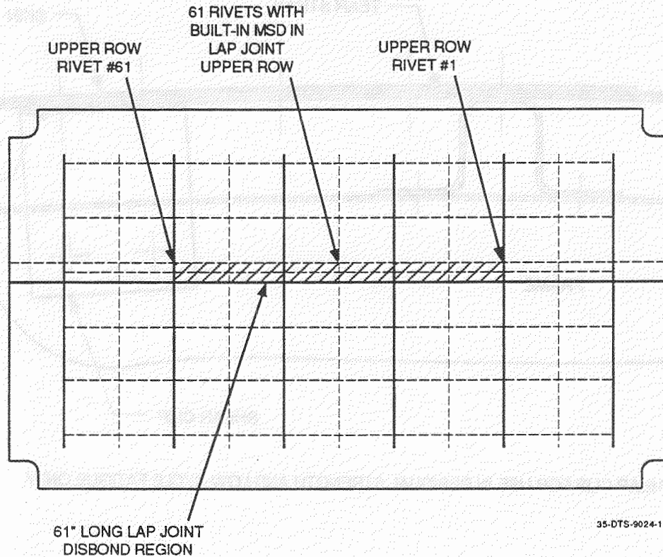
Figure 5-14. Panel Configuration and Initial Damage
