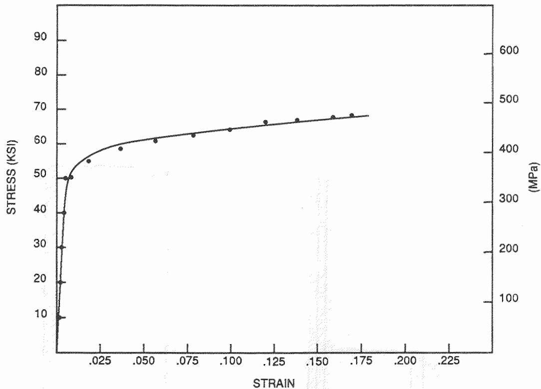
Figure 7-8. Stress-Strain Curve for R-Curve Test Specimen Material (2024-T3)
