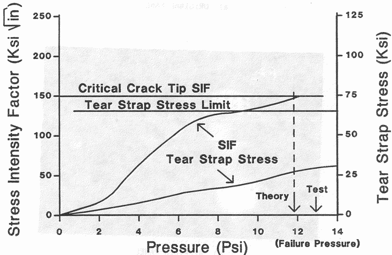
Figure 6-5. Analytic Predictions for 16-in. Crack
