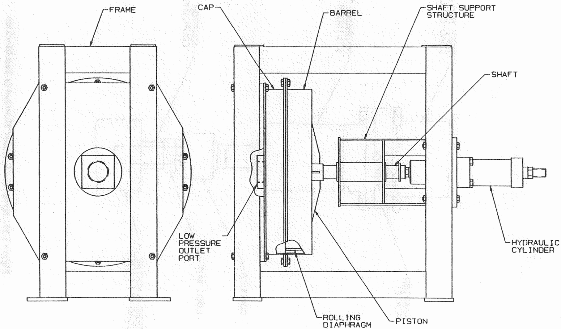
Figure 3-10. Pressure Reducer Assembly
