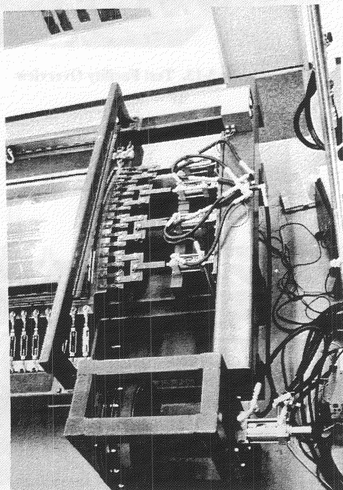
Figure 3-16. Panel End Loading Arrangement and Pressure Reducer
