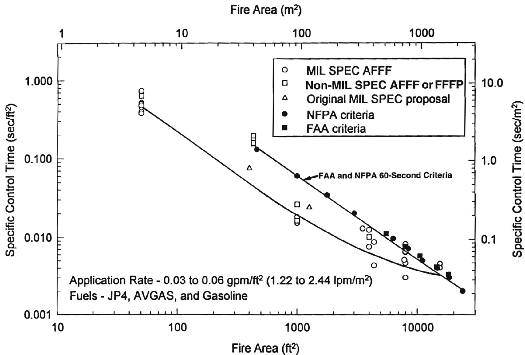
FIGURE 11. SPECIFIC CONTROL TIMES FOR AFFF AT LOW APPLICATION RATES
