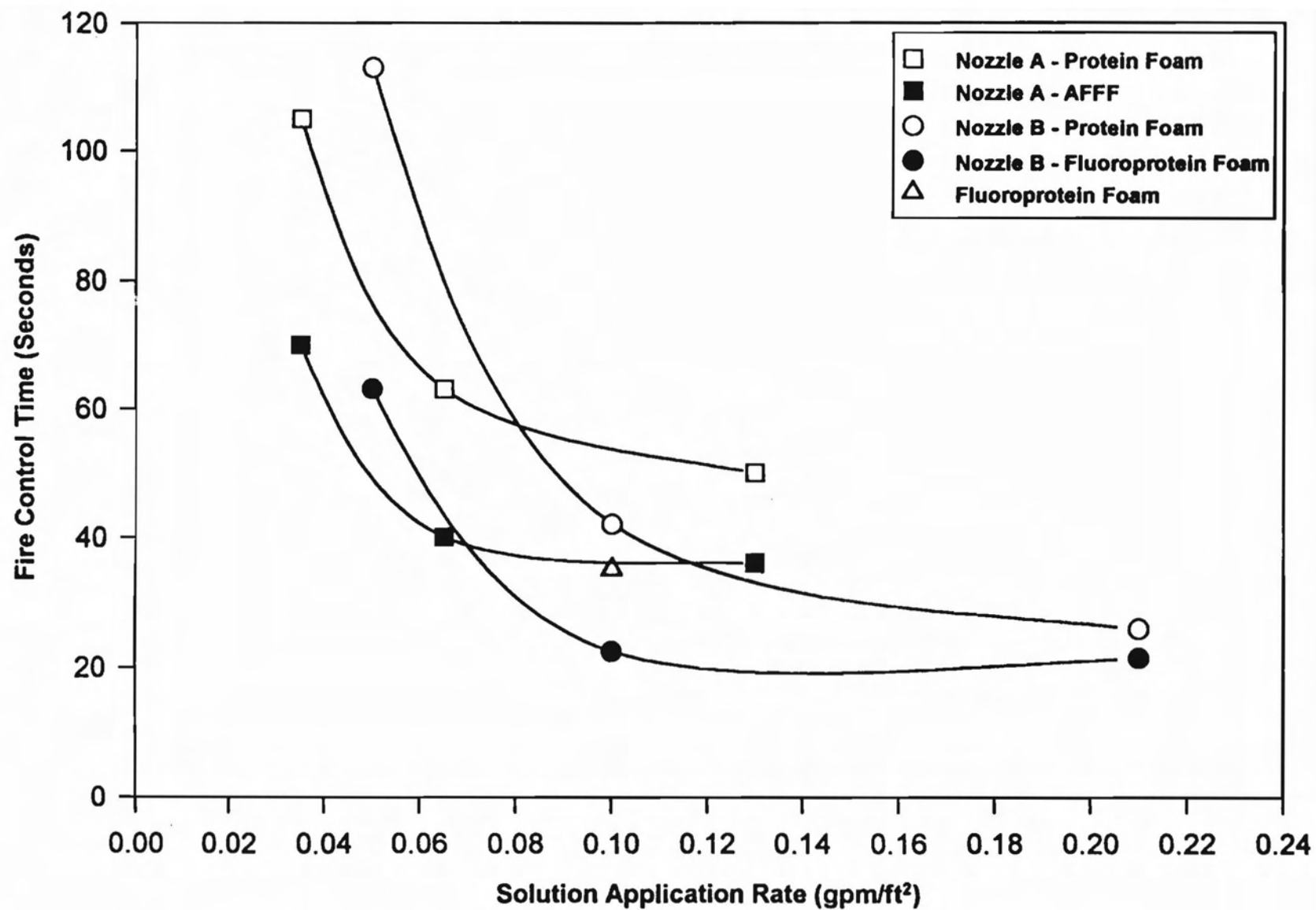
FIGURE 1. FIRE CONTROL TIME AS A FUNCTION OF SOLUTION APPLICATION RATE USING PROTEIN FOAM AND AFFF
