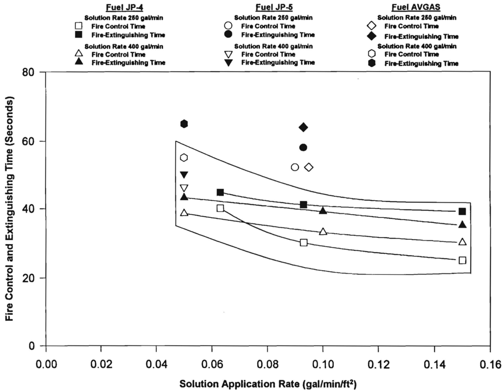
FIGURE 2. FIRE CONTROL AND EXTINGUISHING TIMES AS FUNCTIONS OF THE FOAM SOLUTION APPLICATION RATE USING MANUFACTURER A'S AFFF AGENT AT 250 AND 400 GAL/MIN ON JP-4, JP-5, AND AVGAS FIRES
