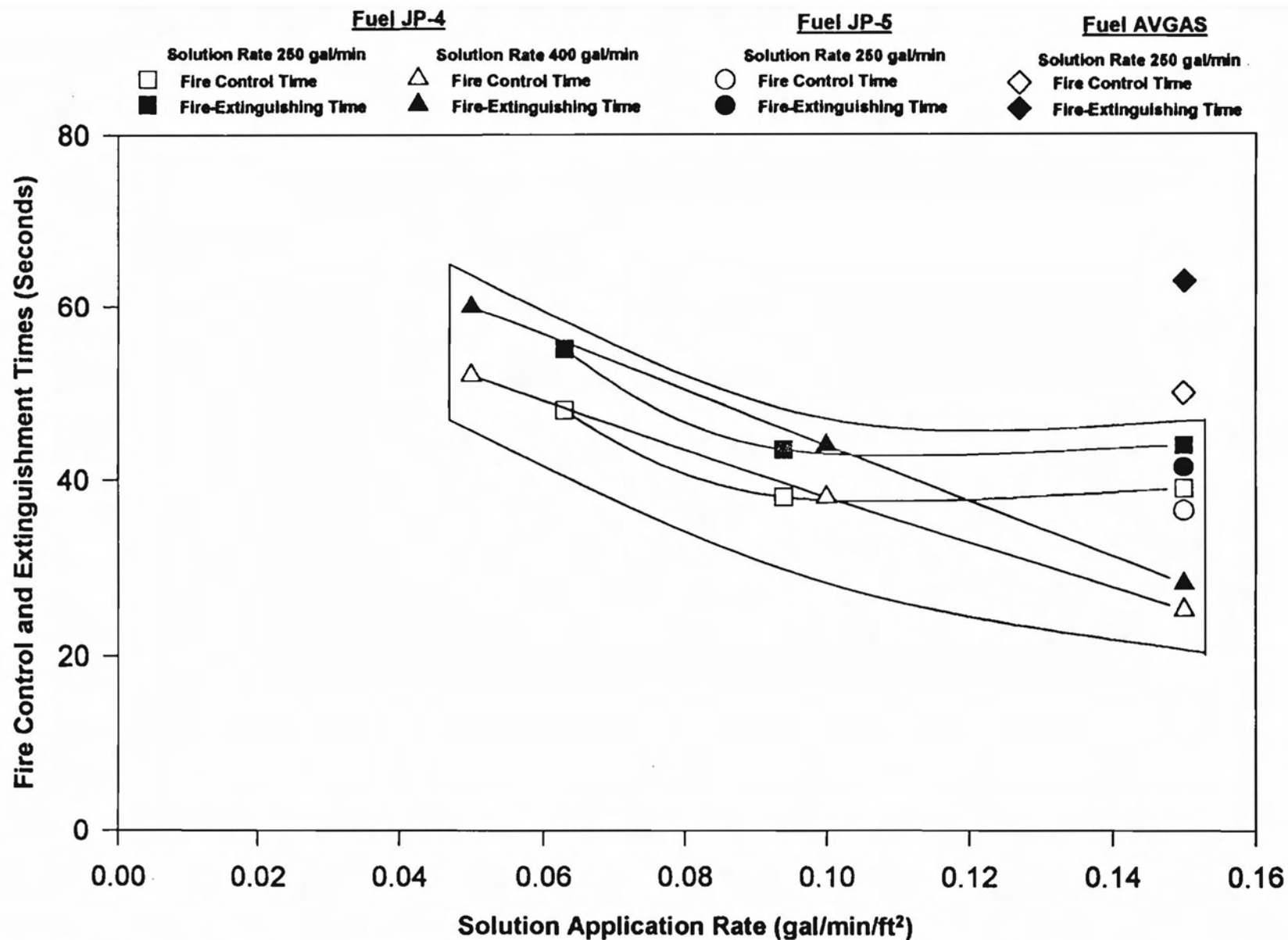
FIGURE 3. FIRE CONTROL AND EXTINGUISHING TIMES AS FUNCTIONS OF THE FOAM SOLUTION APPLICATION RATE USING MANUFACTURER B'S AFFF AGENT AT 250 AND 400 GAL/MIN ON JP-4, JP-5, AND AVGAS FIRES
