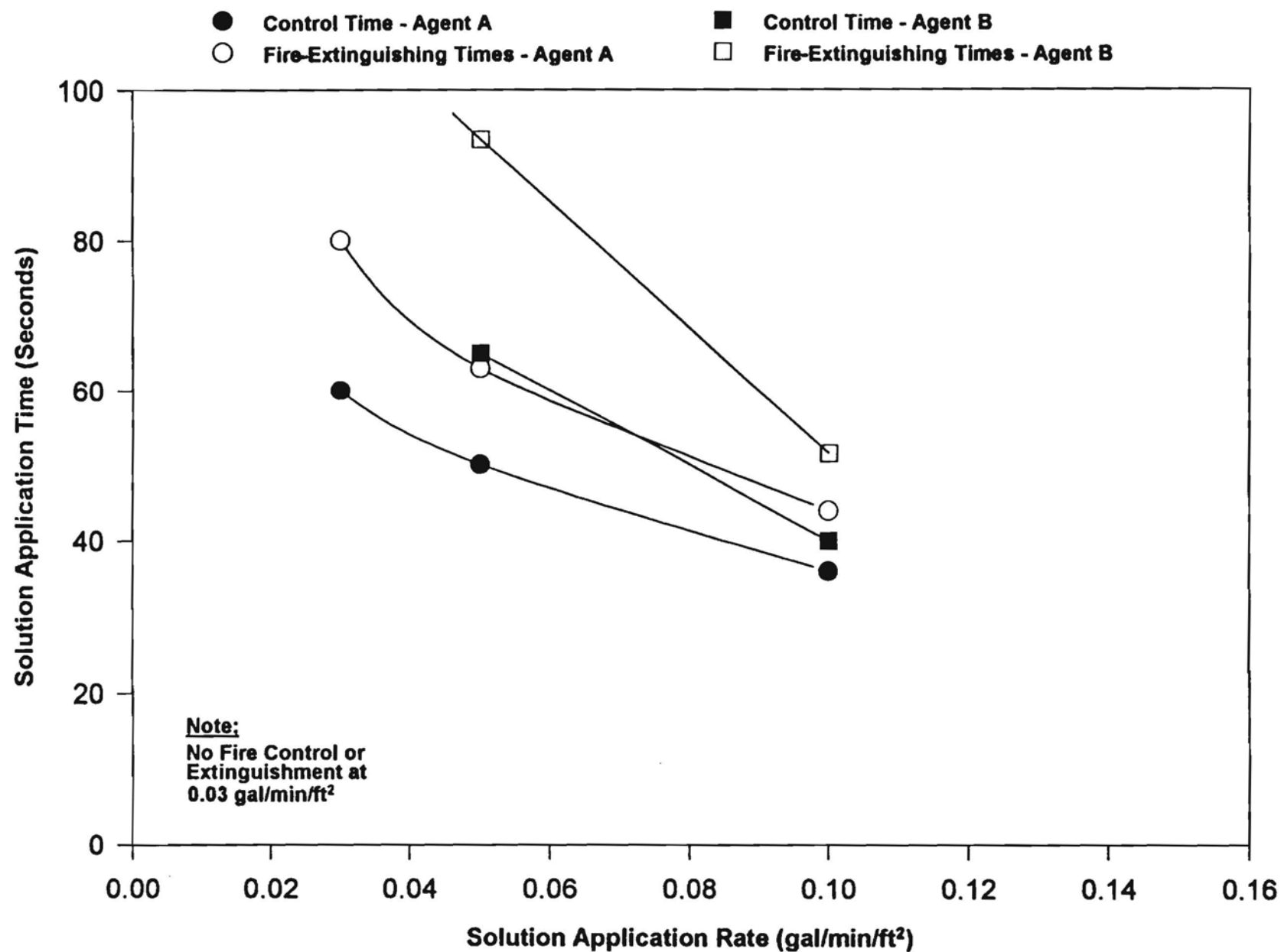
FIGURE 4. FIRE CONTROL AND EXTINGUISHING TIMES AS A FUNCTION OF SOLUTION APPLICATION RATE USING AFFF AT 250, 400, AND 800 GAL/MIN ON 8000 FT² JP-4 FUEL FIRES
