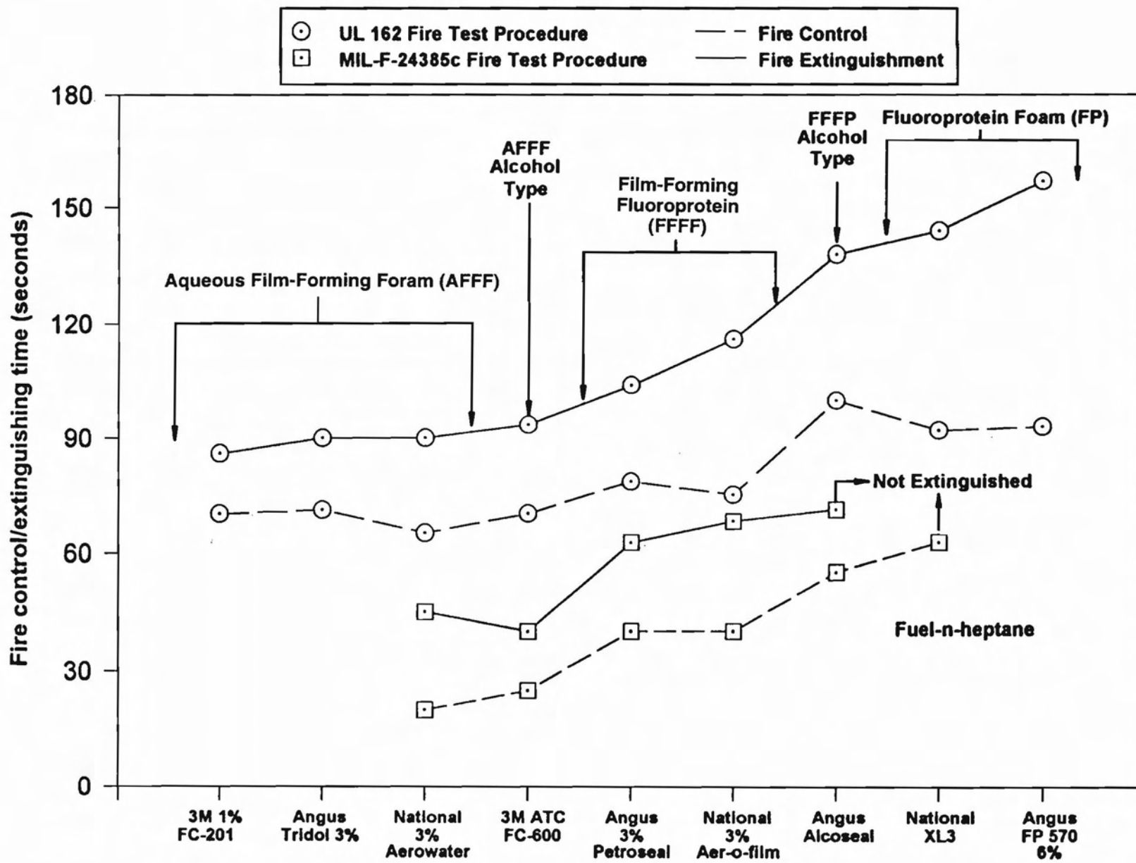
FIGURE 8. SUMMARY OF 50 FT 2 (4.6 M 2 ) FIRE TESTS, FROM FAA TESTS 28
