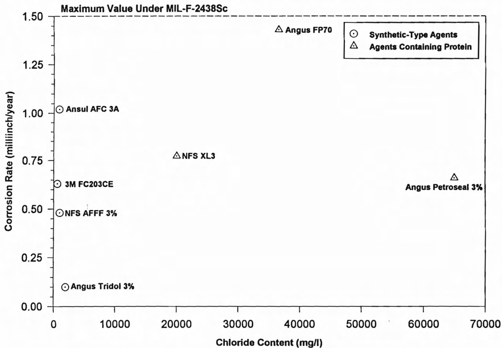
FIGURE A-1. CORROSION RATE OF FOAM FIREFIGHTING AGENTS AGAINST STEEL (UNS G10100) VS. THEIR CHLORIDE CONTENT
