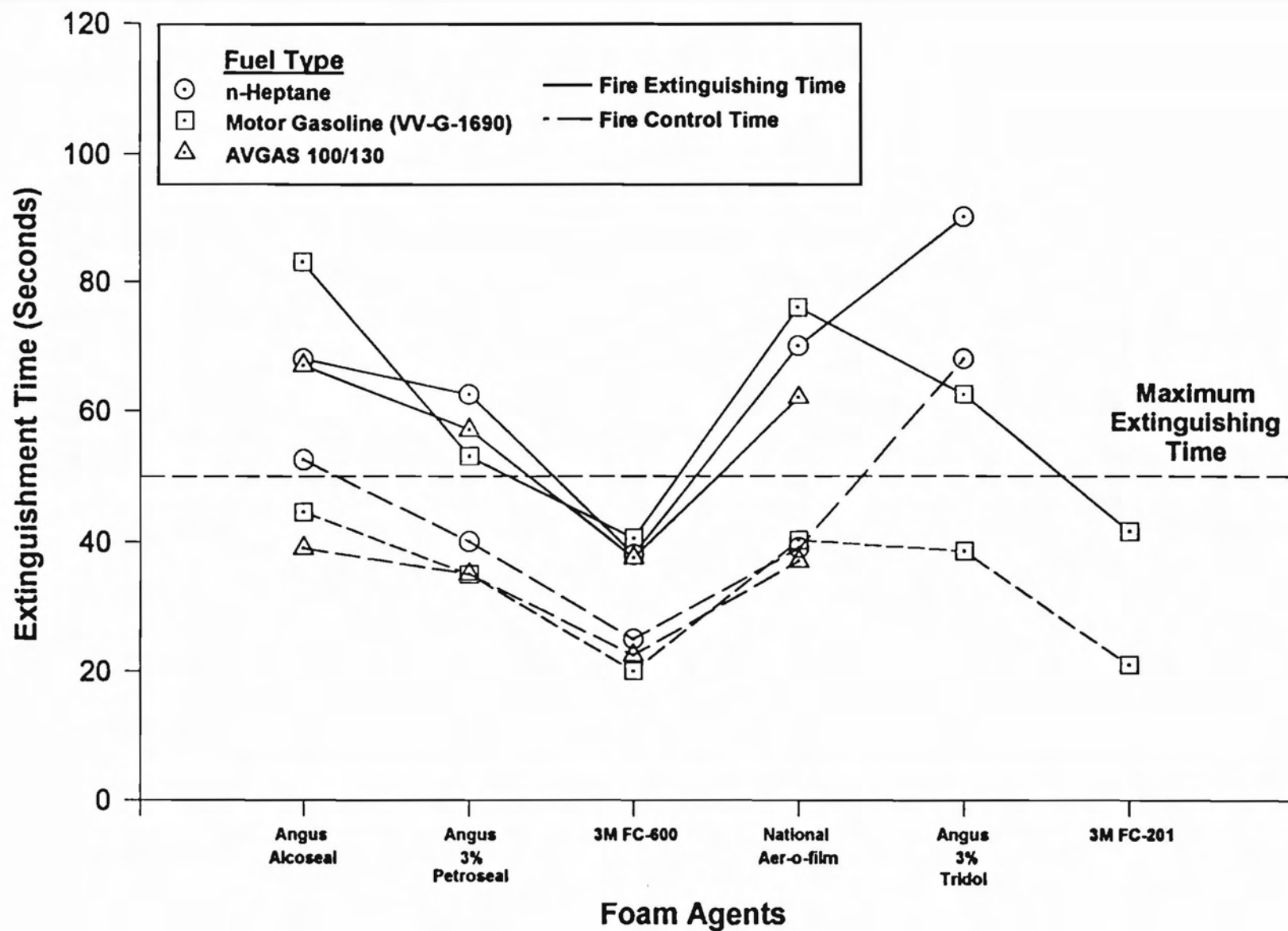
FIGURE A-3. EFFECT OF FUEL TYPE OF FIRE PERFORMANCE USING THE MIL-F-24385C 50 SQUARE FOOT FIRE TEST
