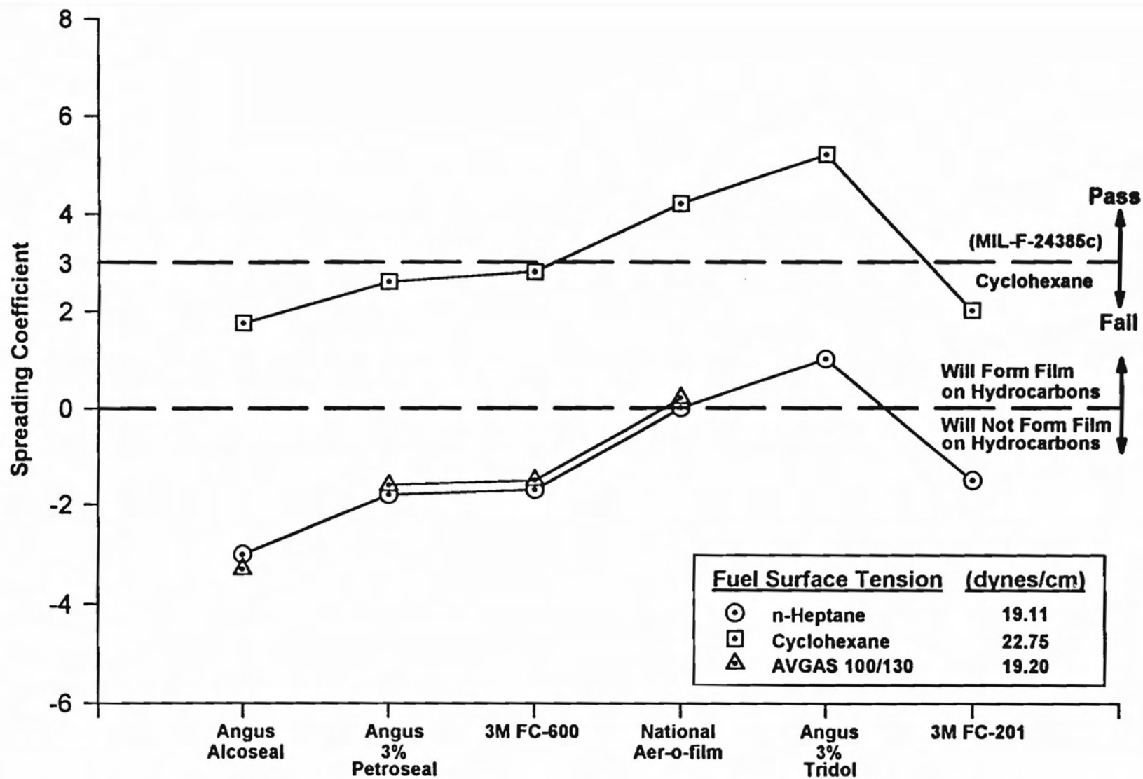
FIGURE A-2. SPREADING COEFFICIENTS FOR FILM-FORMING FOAM AGENTS ON THREE TEST FUELS
