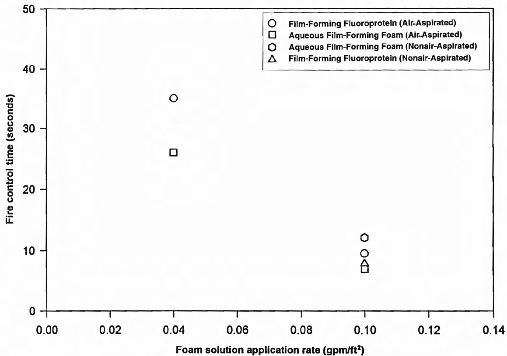
FIGURE 9. FIRE CONTROL FOR LARGE-SCALE FIRE TESTS OF FFFP AND AFFF
