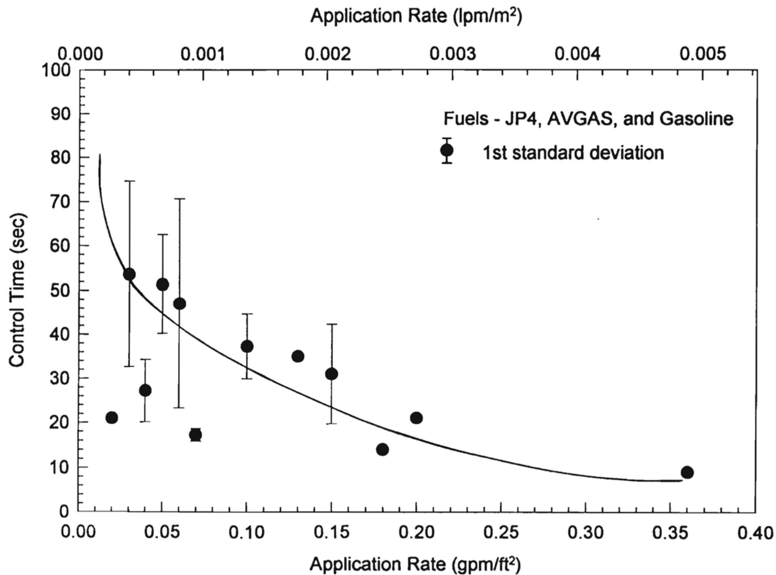
FIGURE 10. AFFF CONTROL TIME AS A FUNCTION OF APPLICATION RATE
