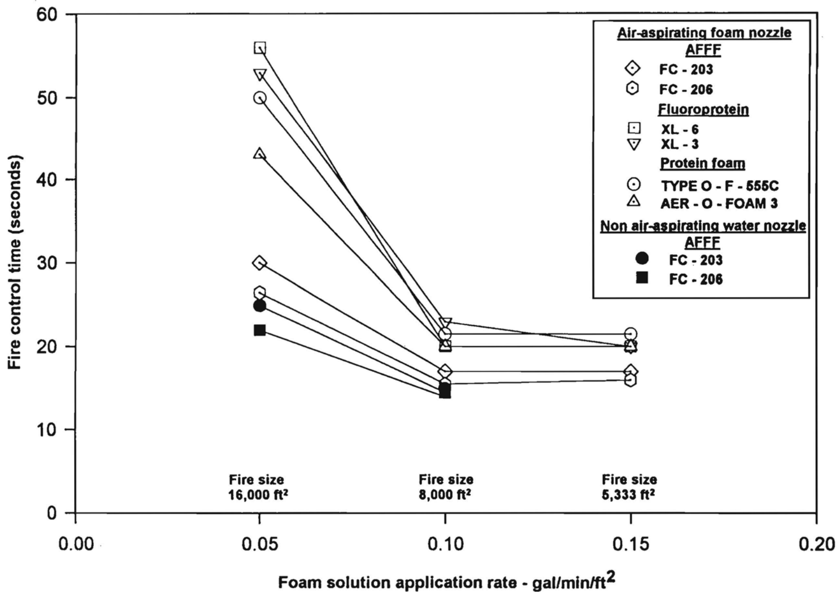
FIGURE 5. FIRE CONTROL TIME AS A FUNCTION OF SOLUTION APPLICATION RATE FOR AFFF, FLUOROPROTEIN, AND PROTEIN FOAMS FOR JET A FUEL FIRES
