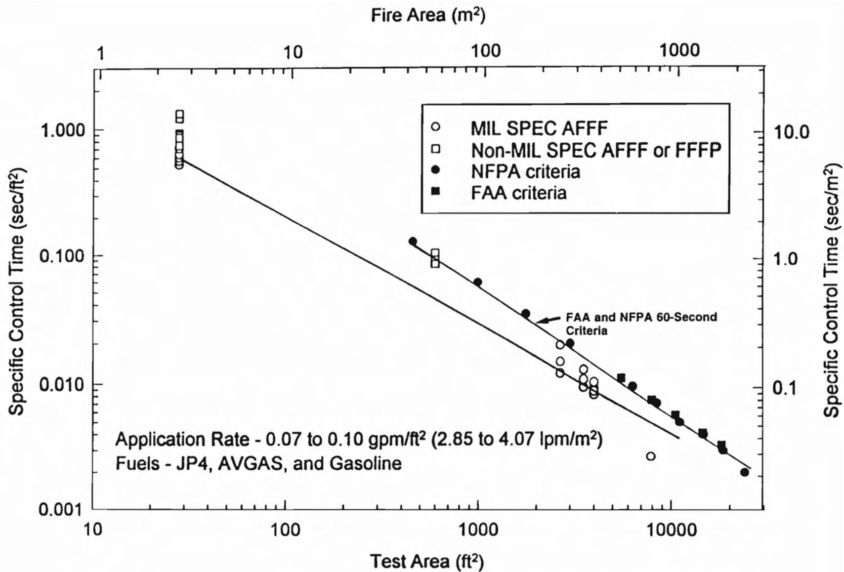
FIGURE 12. SPECIFIC CONTROL TIMES FOR AFFF AT INTERMEDIATE APPLICATION RATES
