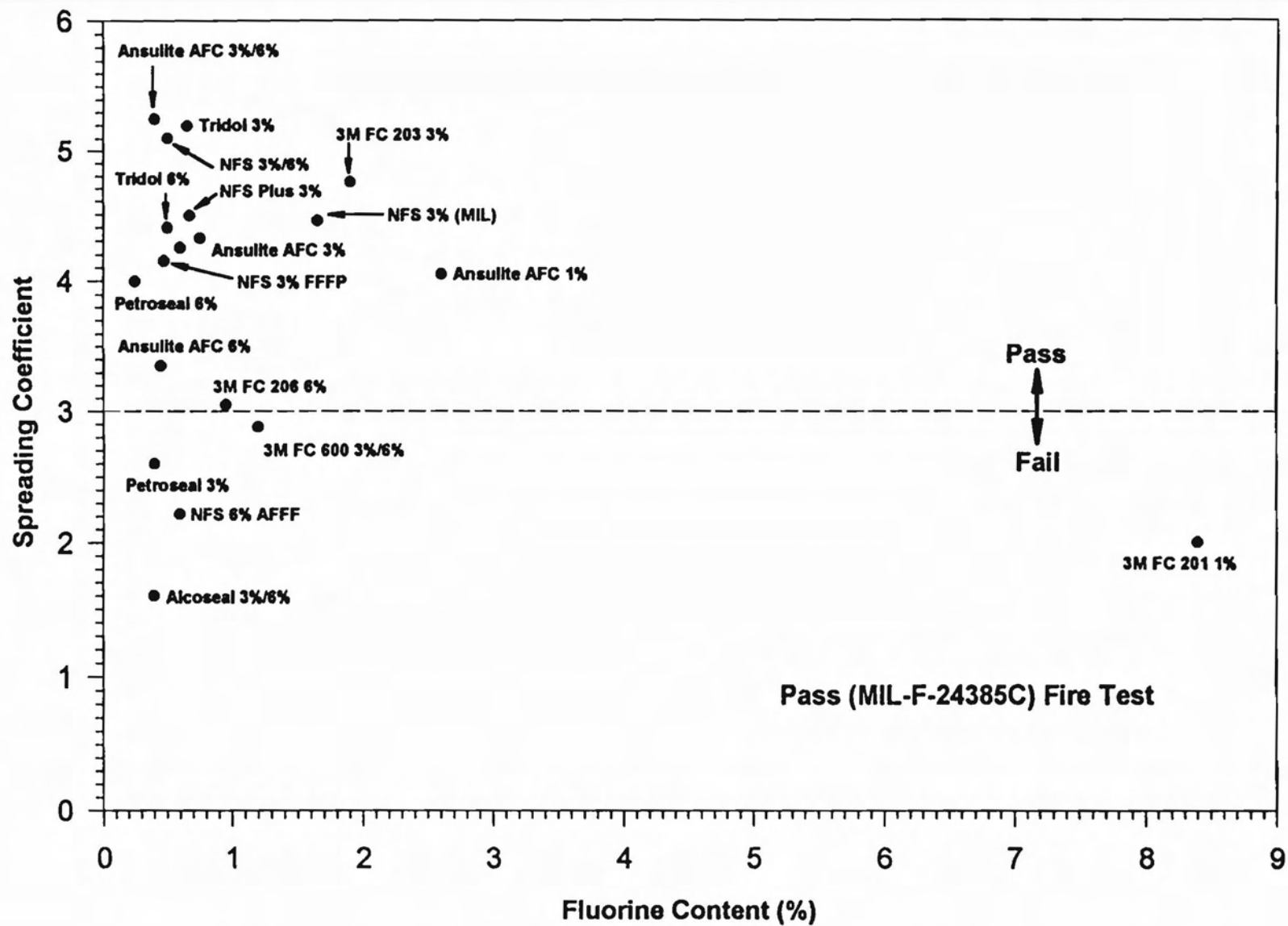
FIGURE A-4. SPREADING COEFFICIENT AS A FUNCTION OF FLUORINE CONTENT
