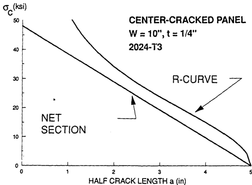
Figure 2-36. Illustration of the width effect on thin sheet strength.
