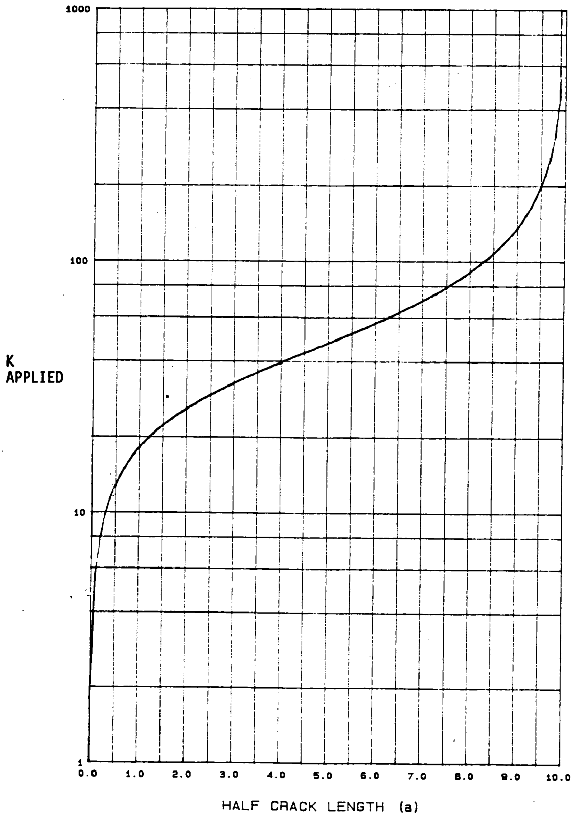
Figure 2-29. K applied versus crack length
