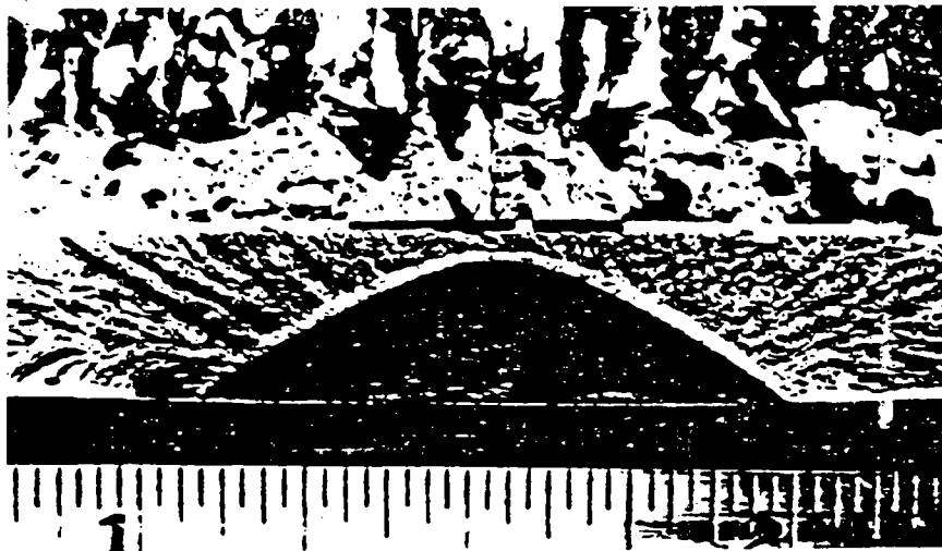
(c) Crack in left wing pivot forging of F-111 aircraft.
