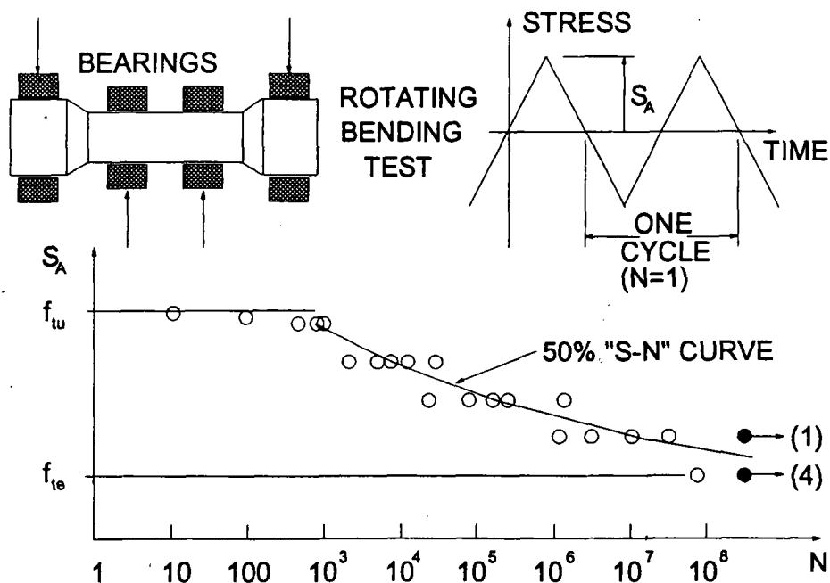
Figure 1-9. Results of a typical fatigue experiment.
