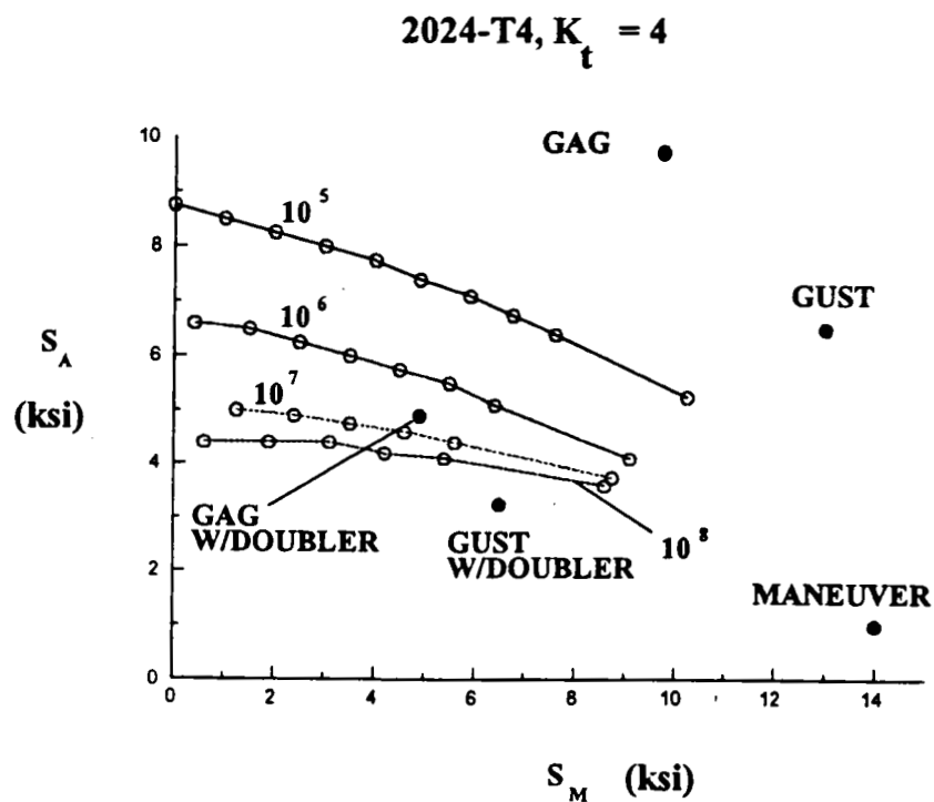
Figure 1-12. Goodman diagram for 2024-T4 aluminum.
