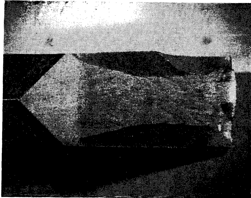
Figure 2-18. Typical fracture surfaces.
