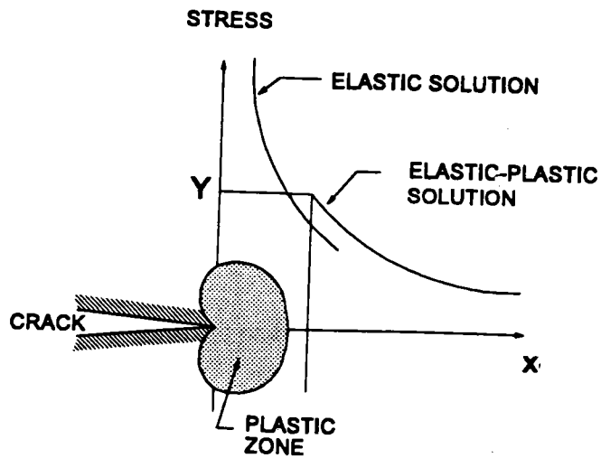
Figure 2-10. Refined estimate of plastic zone formation ahead of crack tip.
