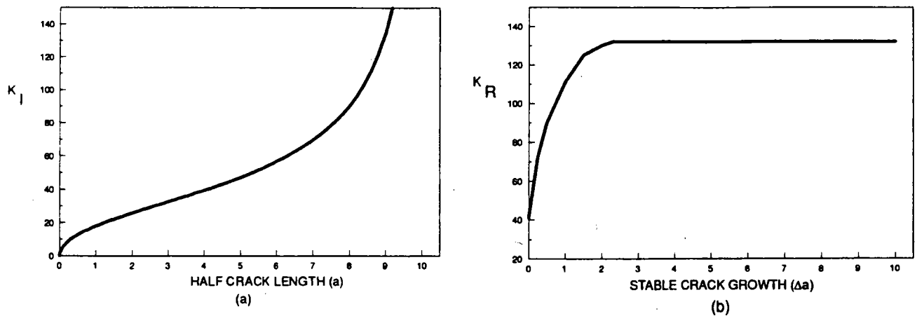
Figure 2-25. K_I and K_R curves
