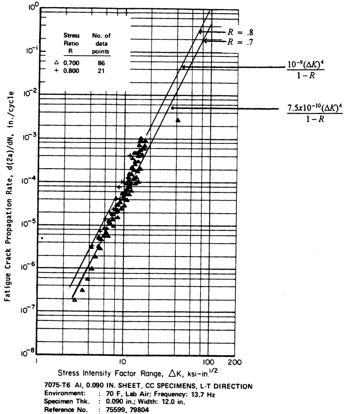
(c) Results for R = 0.7 and R = 0.8 .
