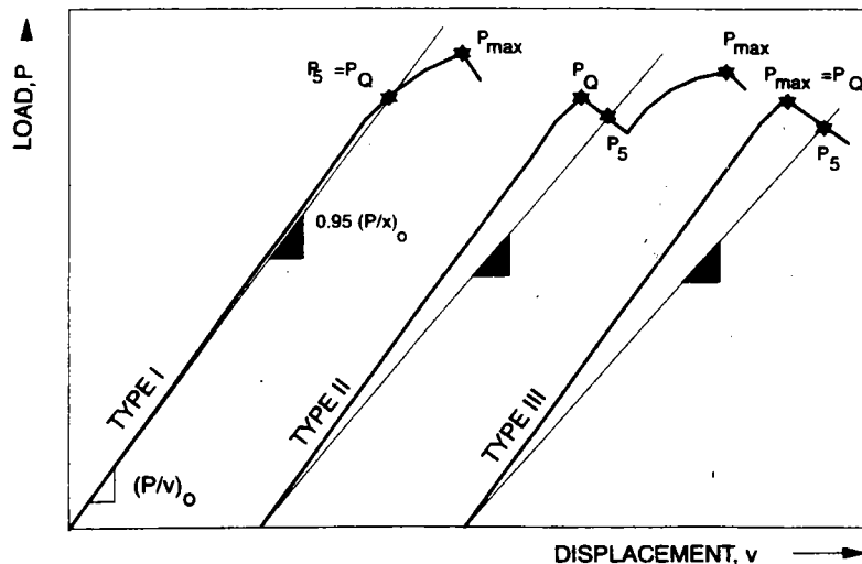
Figure 2-15. Load-displacement plot
