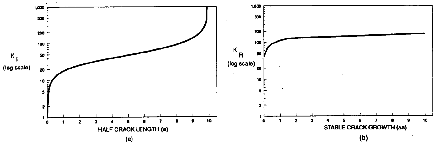
Figure 2-26. K_I and K_R curves (logarithmic scale)
