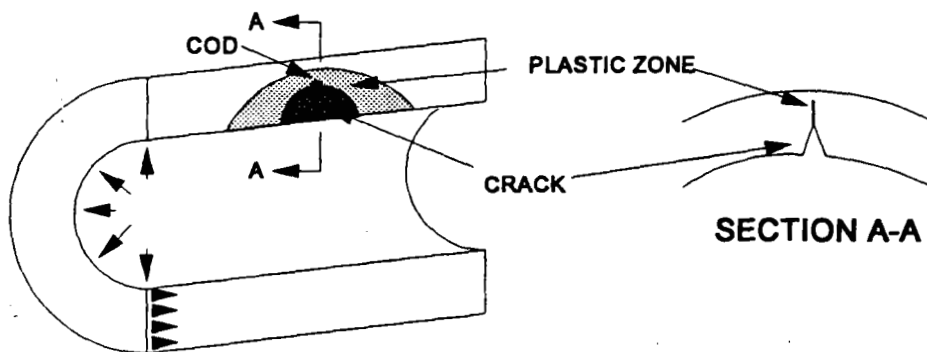
Figure 2-41. Erdogan's plastic zone model.
