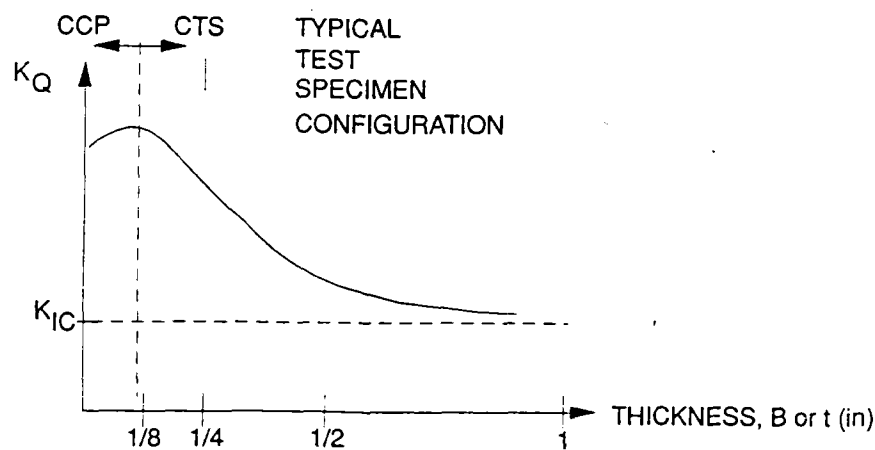
Figure 2-16. Thickness effect on fracture strength.
