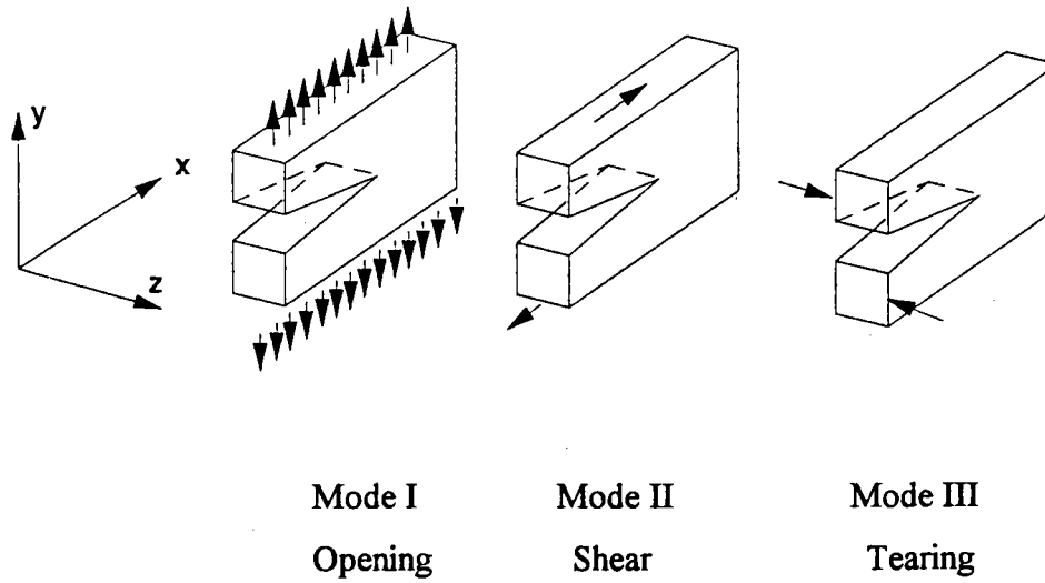
Figure 2-8. Fracture modes
