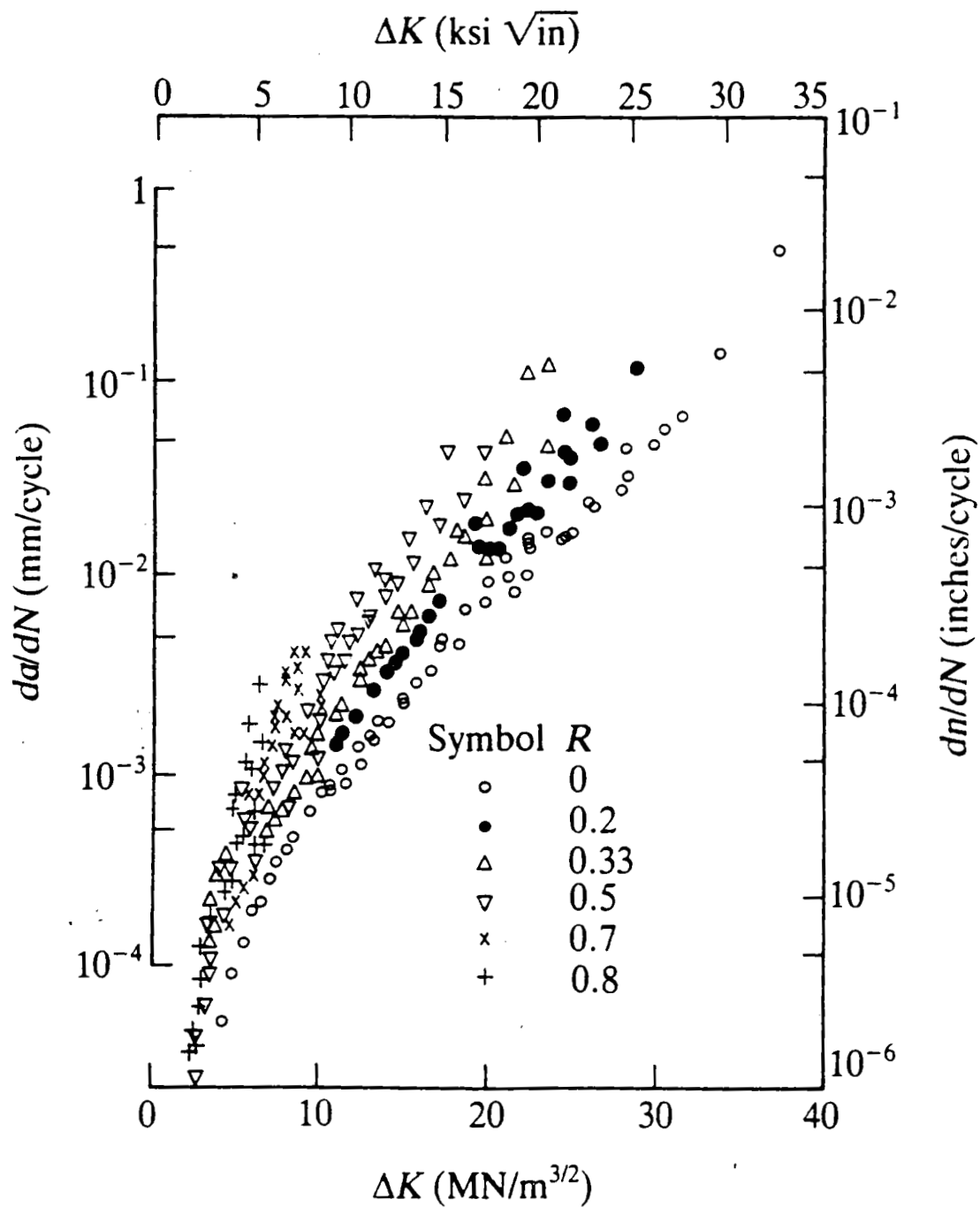
Figure 3-5. Effect of stress ratio on 7075-T6 aluminum crack growth rate.
