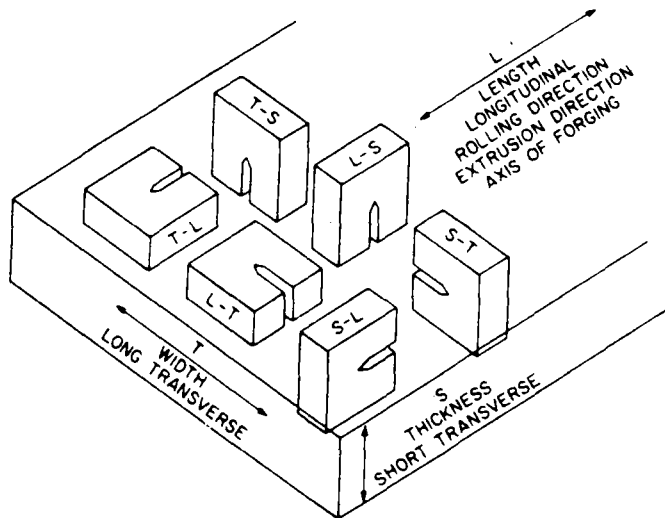
Figure 2-14. CTS orientation.
