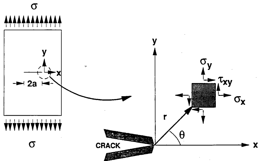
Figure 2-6. Stress components in Irwin's analysis.
