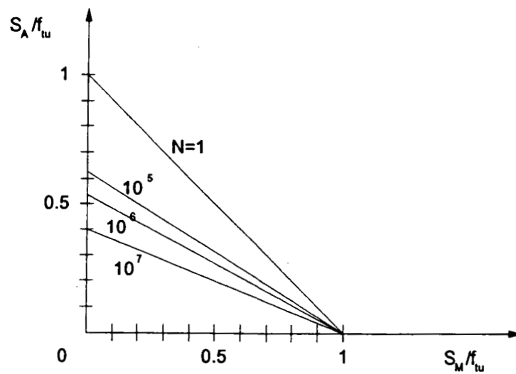
Figure 1-11. Modified Goodman diagram.
