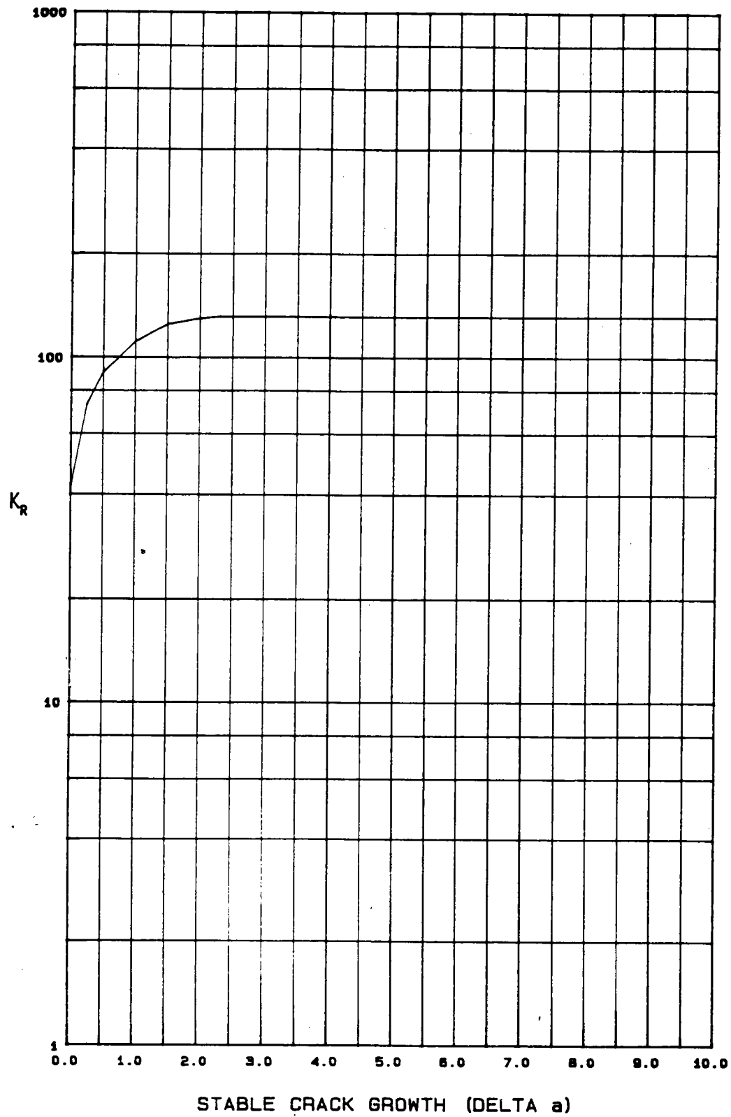
Figure 2-28. R-Curve for 2024-T3
