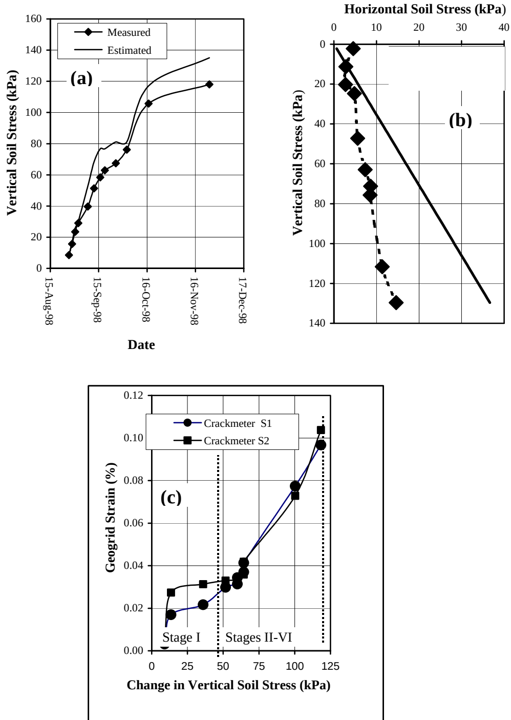
Figure 10. Measured and estimated data on section 400 of the phase I structure: (a) Vertical Stresses, (b) Horizontal Stresses, and (c) Geogrid Strains.
