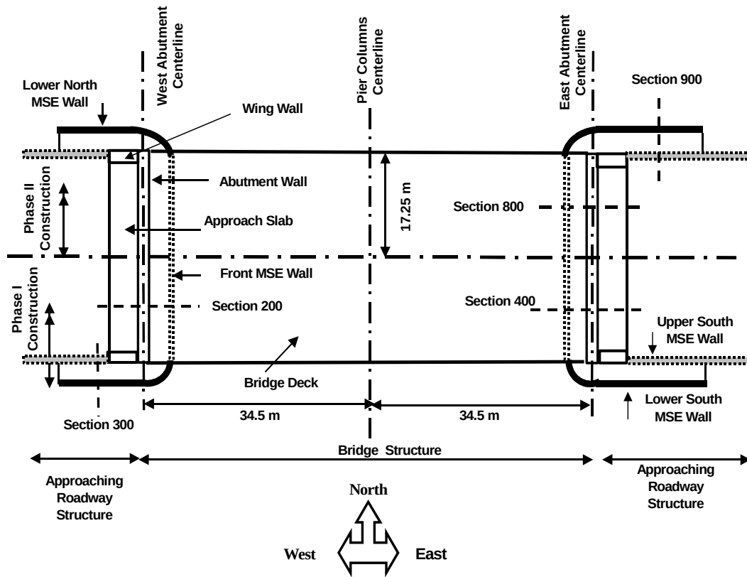
Figure 2. Top view of the Founders/Meadows Bridge.
