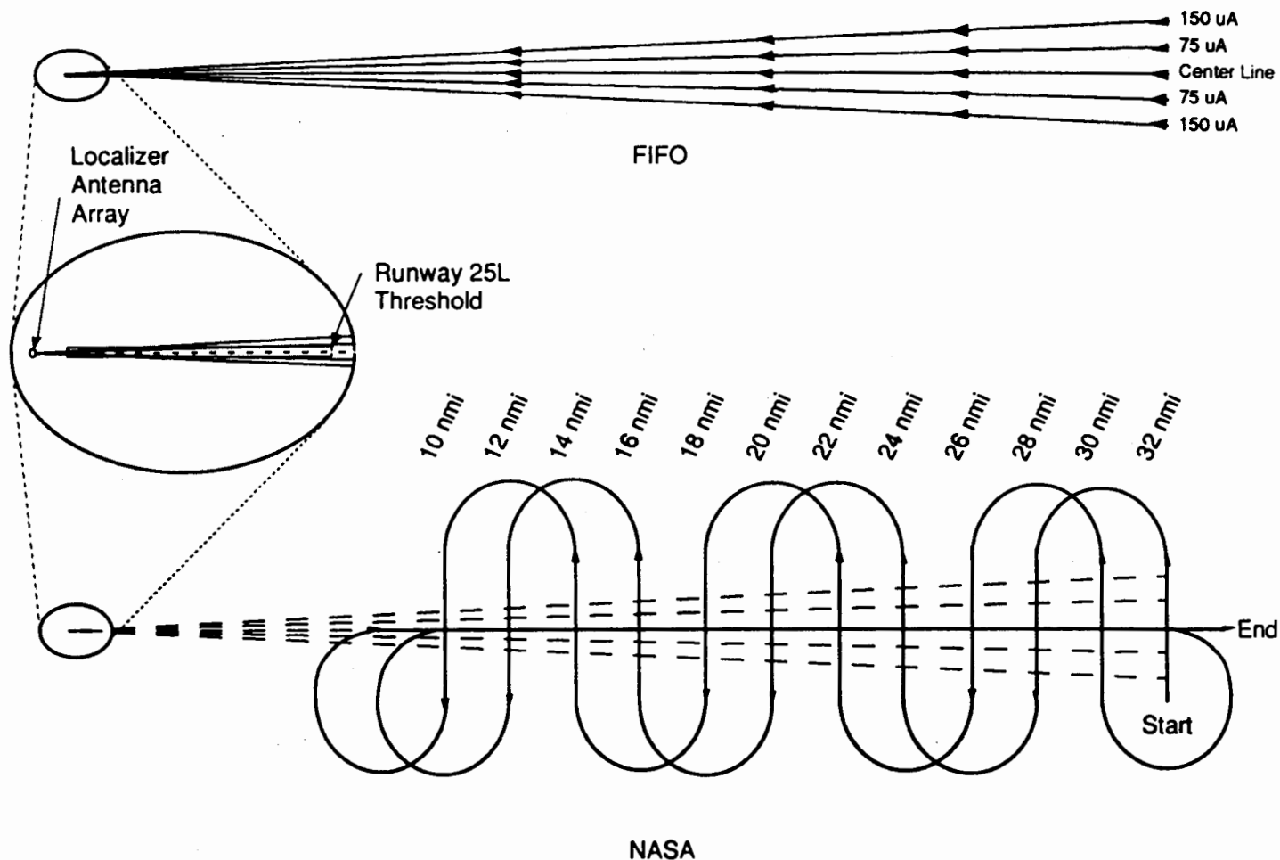
FIGURE 4. FLIGHT PATHS FLOWN BY THE FIFO AND NASA AIRCRAFT
