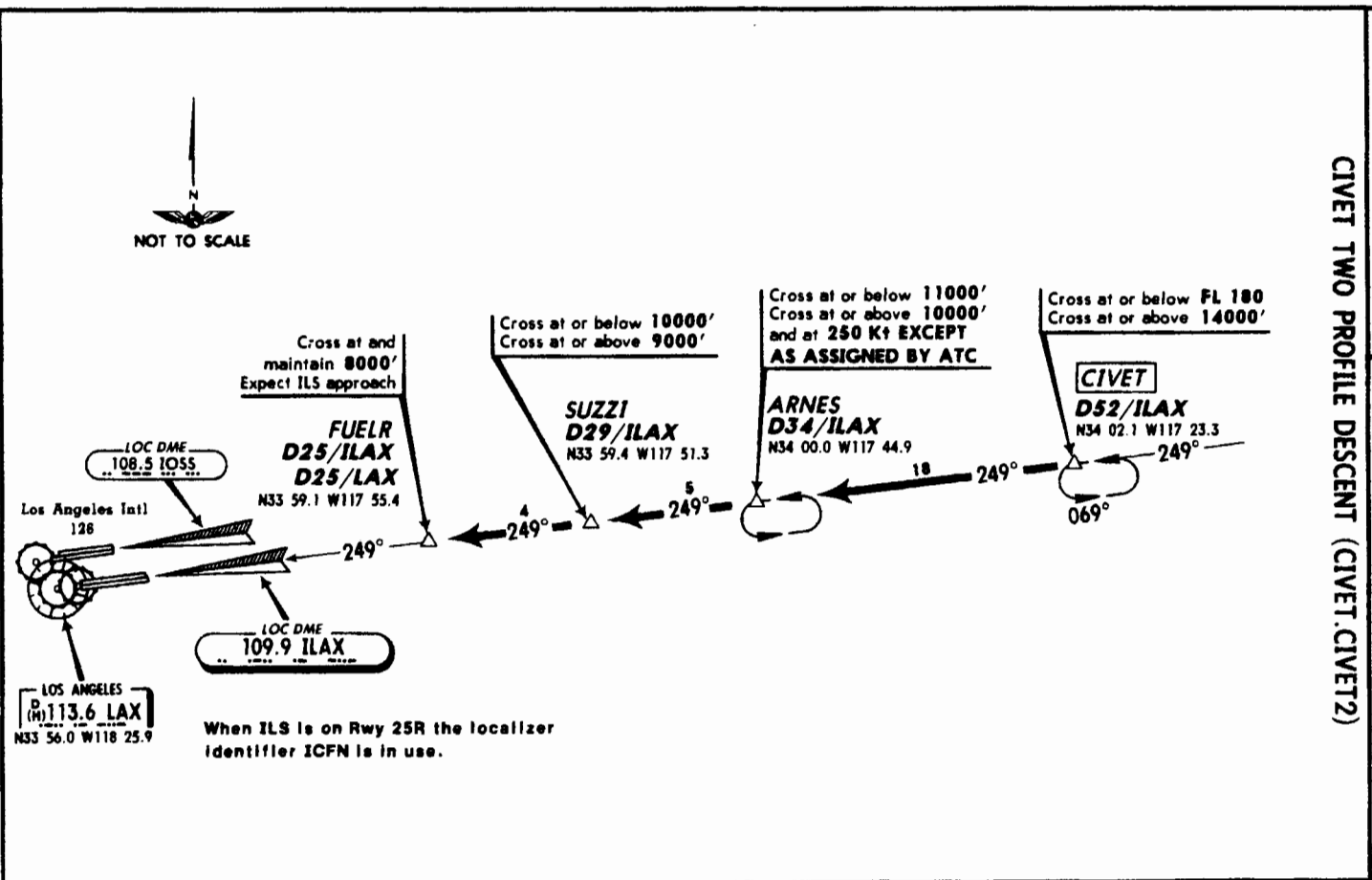
FIGURE 3. LAX CIVT ARRIVAL PROFILE
