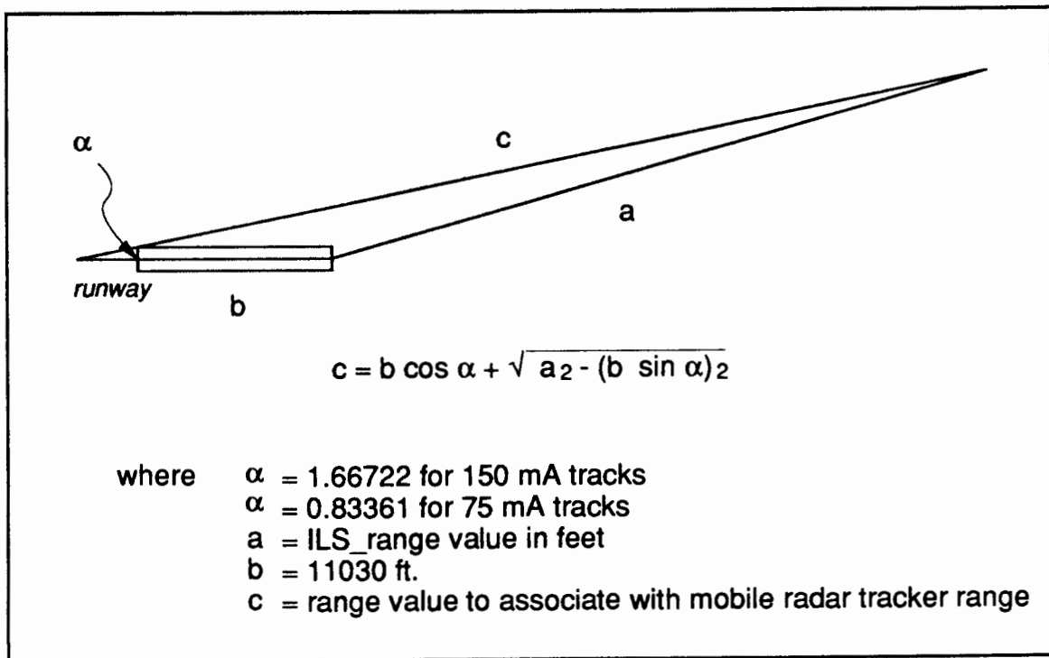
FIGURE 22. CALCULATION OF RANGE FROM LOCALIZER ANTENNA
