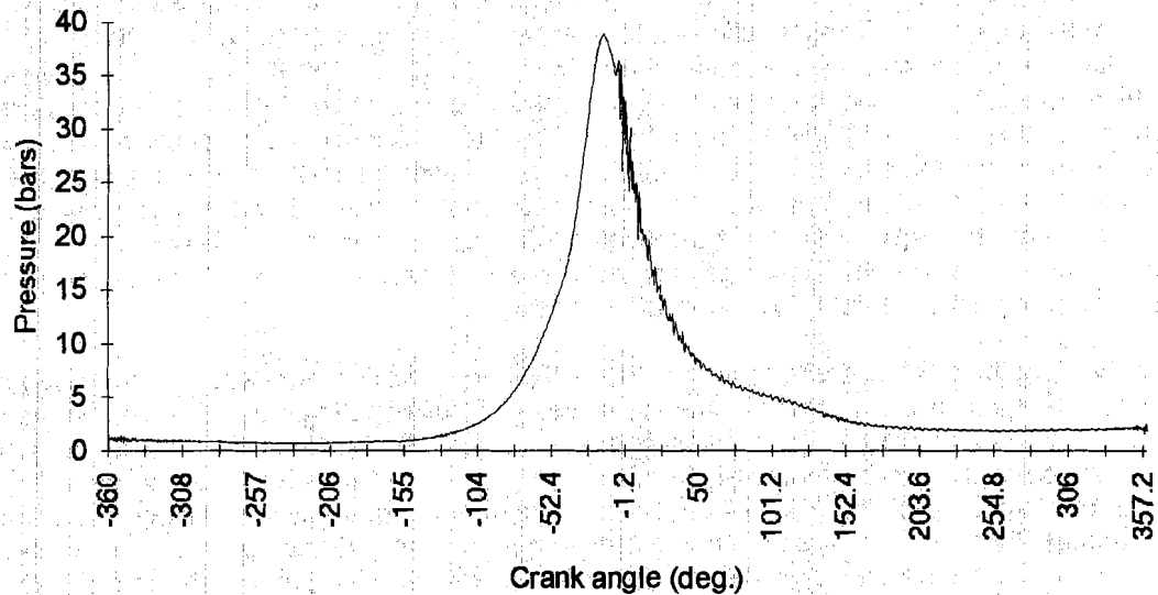
Figure 2.4.3. Pressure Trace Showing Incipient Detonation.
