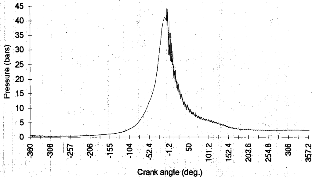
Figure 2.4.4. Pressure Trace Showing Detonation.
