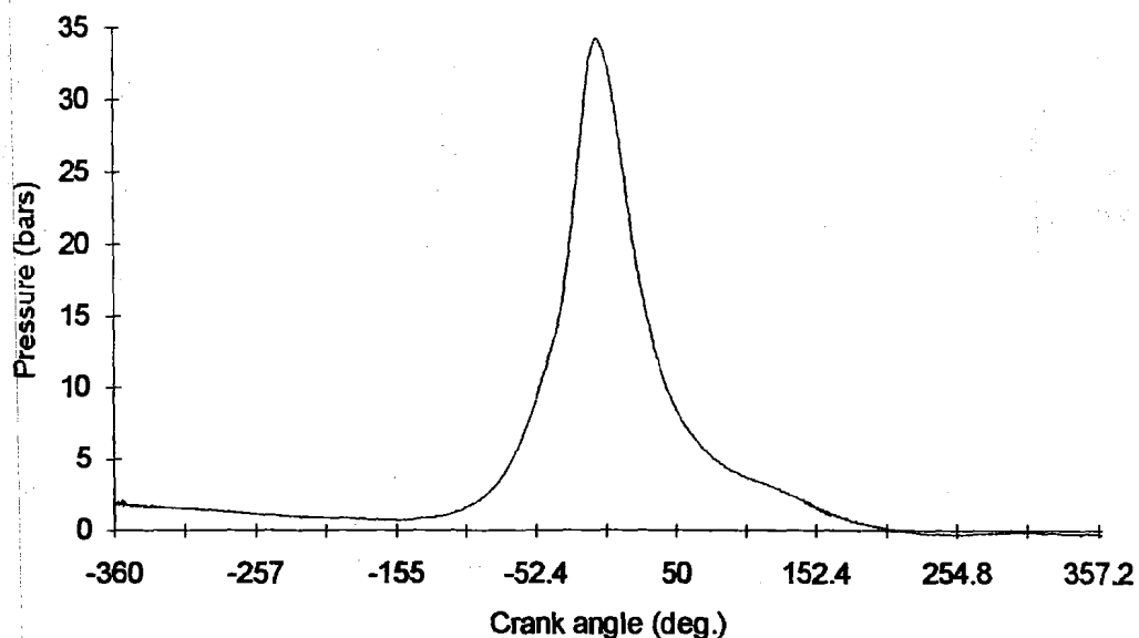
Figure 2.4.2. Pressure Trace Showing Normal Combustion.
