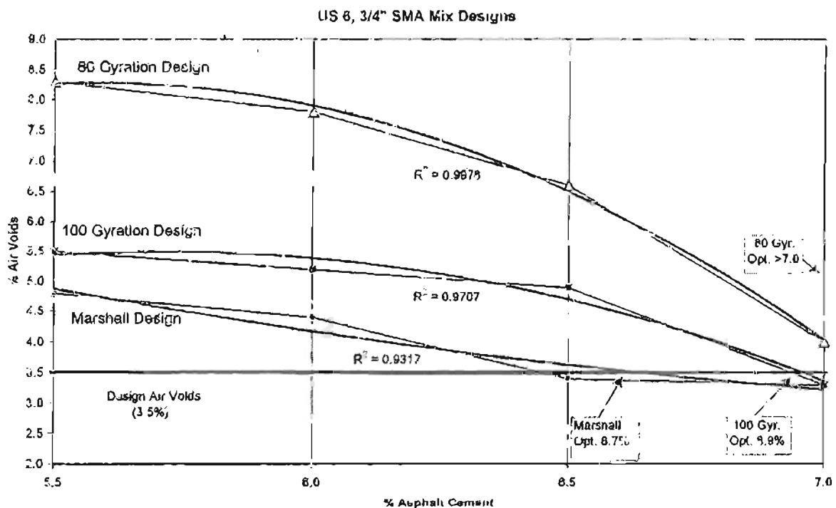
Figure 24. 3/4" SMA mix designs.
