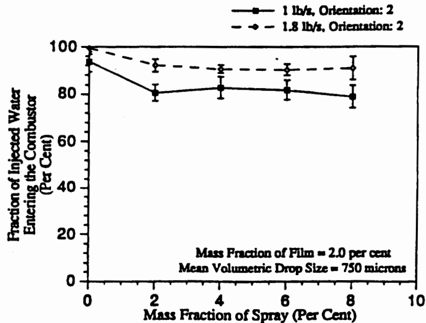
Figure 42. Case VIII: Effect of Mass Fraction of Injected Film and Spray of Large Droplet Size on Water Entry into the Combustor (Orientation 2)
