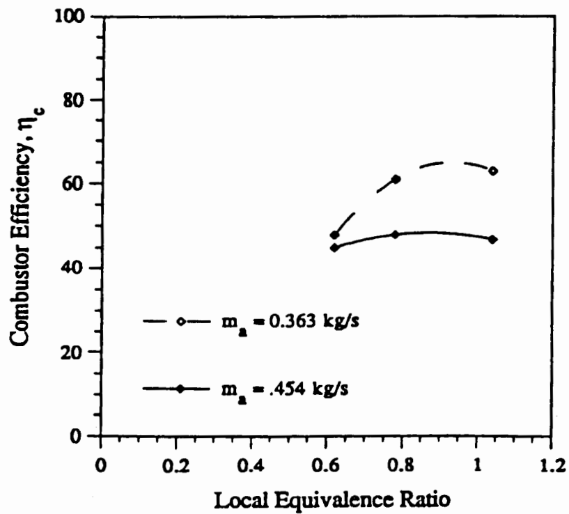
Figure 76. Overall Combustor Efficiency
