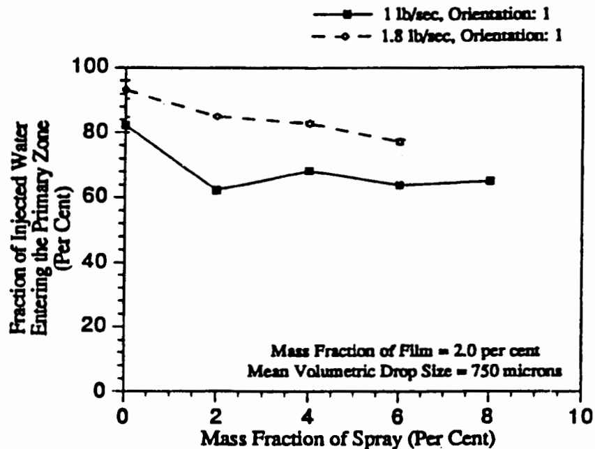
Figure 30. Case II: Effect of Mass Fraction of Injected Film and Spray of Large Droplet Size on Water Entry into the Primary Zone Through the Dome and Primary Jets (Orientation 1)
