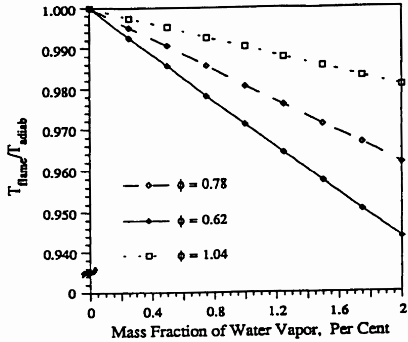
Figure 75. Effect of Vitiating on Flame Temperature
