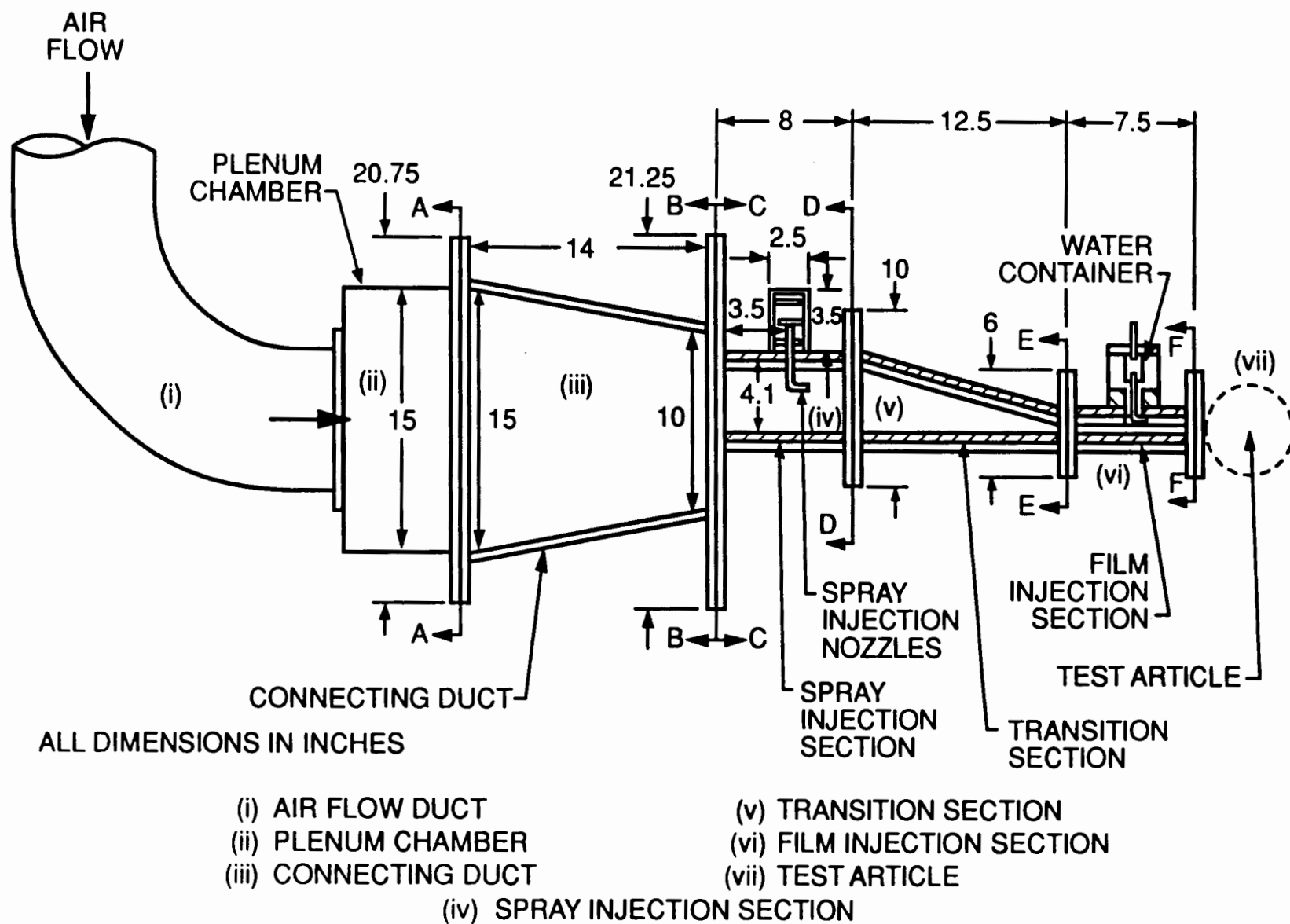
Figure 9. Side View of the Two-Phase Flow Tunnel
