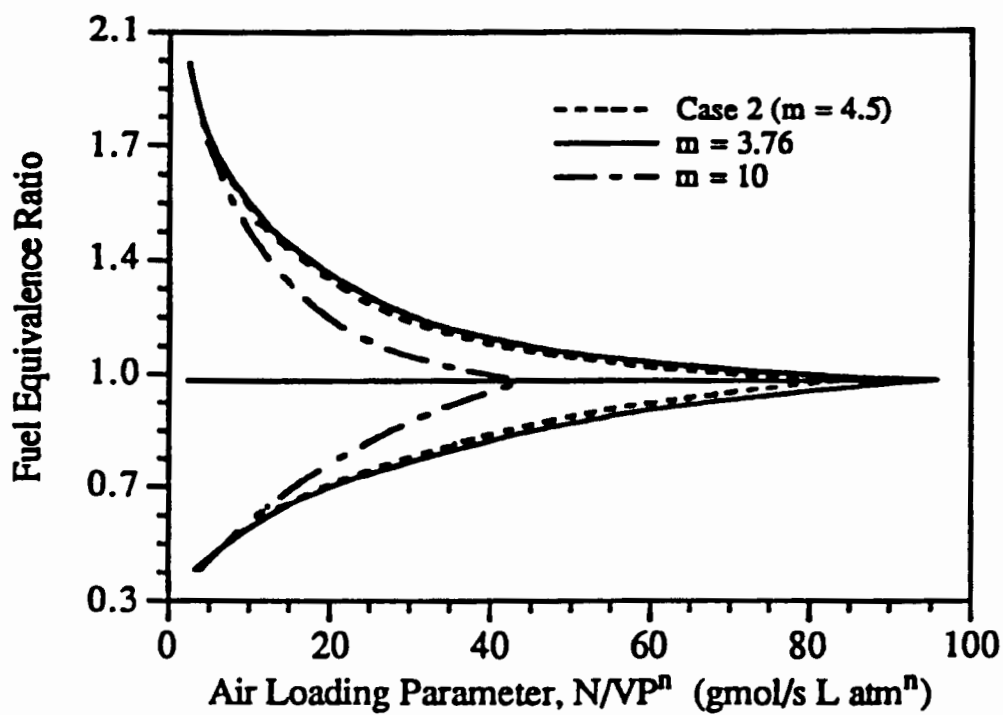
Figure 74. Effect of Vitiatio on Flameout Characteristics
