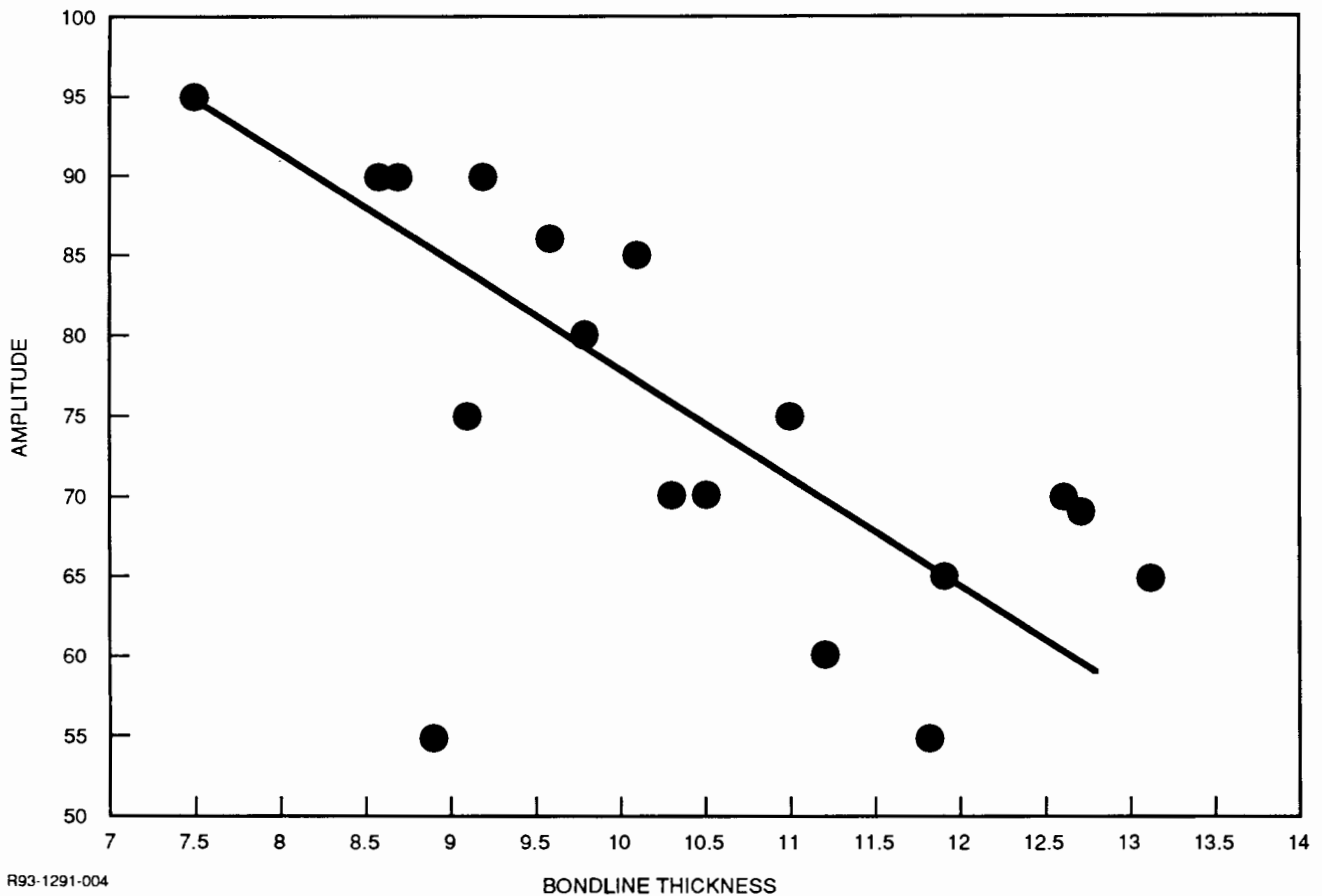
FIGURE 1. EFFECT OF BONDLIN THICKNESS
