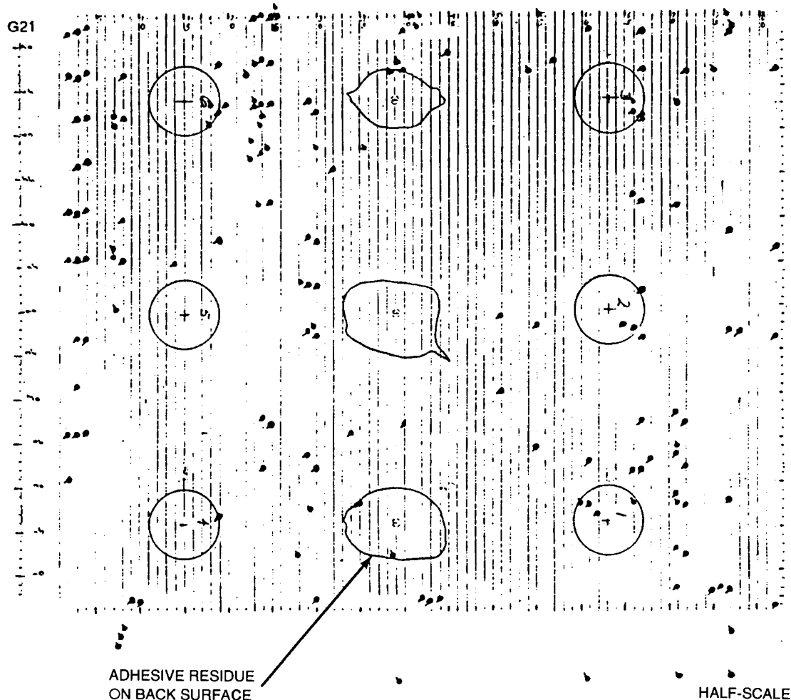
FIGURE 8. WEAK BOND INDICATIONS SENSED AND THEN GRAPHED ON A FACSIMILE OF SPECIMEN G21
