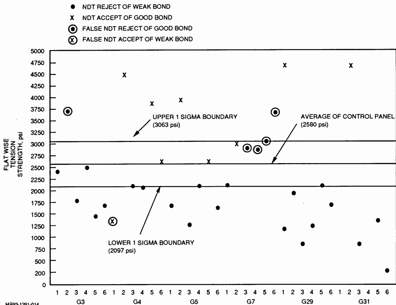
FIGURE 10. PLOT OF FLATWISE TENSION/NDT RESULTS
