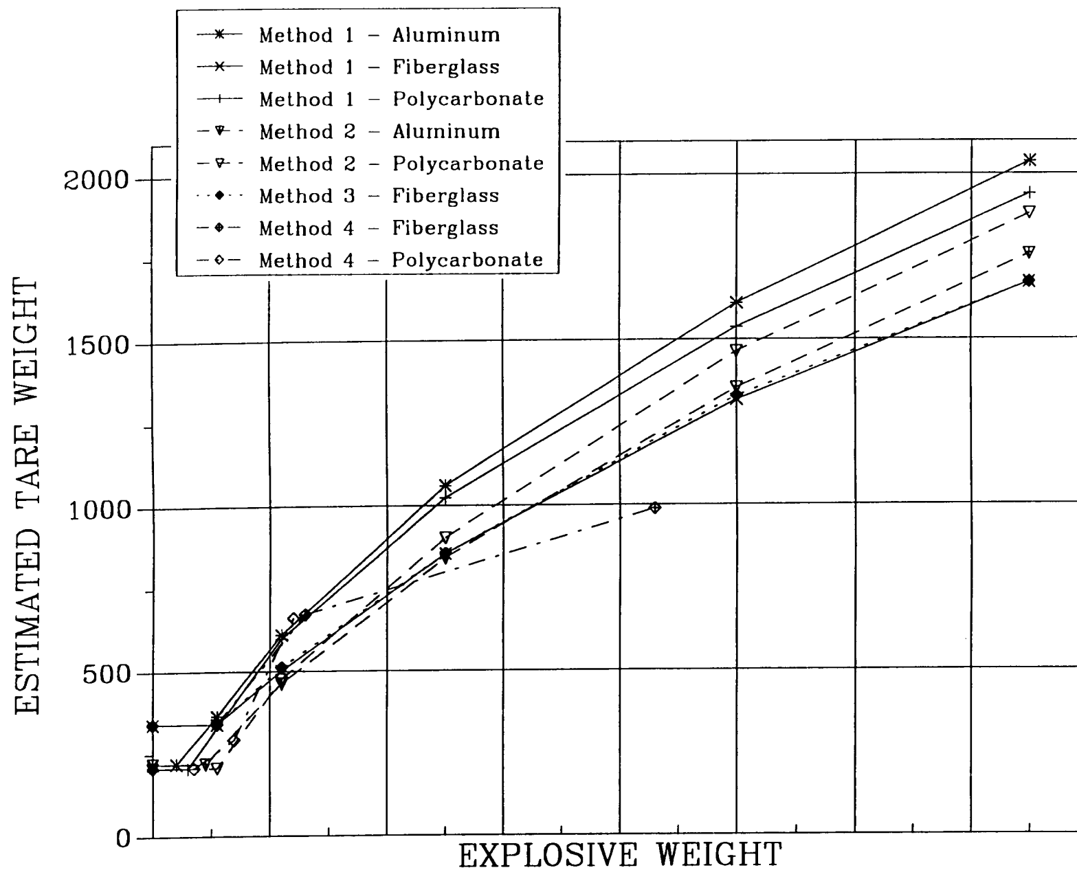
FIGURE 2.2-1 SUMMARY OF HARDENING COUNTERMEASURES 1 - 4
