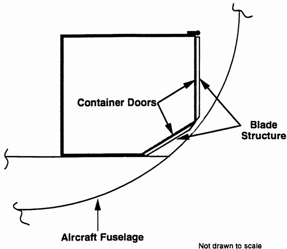
FIGURE 3.2-1 CONTAINER WITH BLADED DOORS
