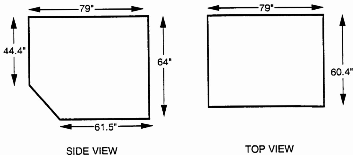
FIGURE 2-1 LD-3 UNIT LOAD DEVICE
