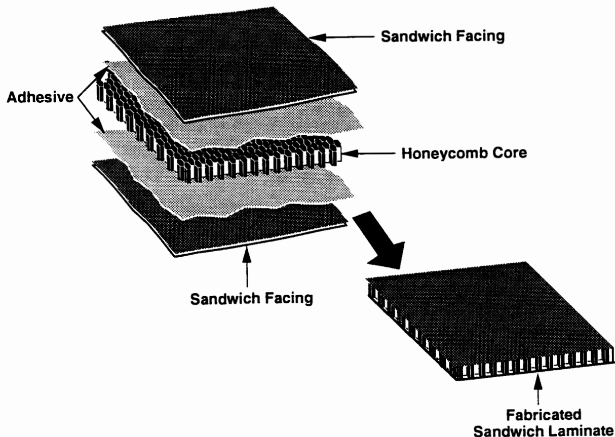
FIGURE 5.1-1 TYPICAL HONEYCOMB SANDWICH CONSTRUCTION
