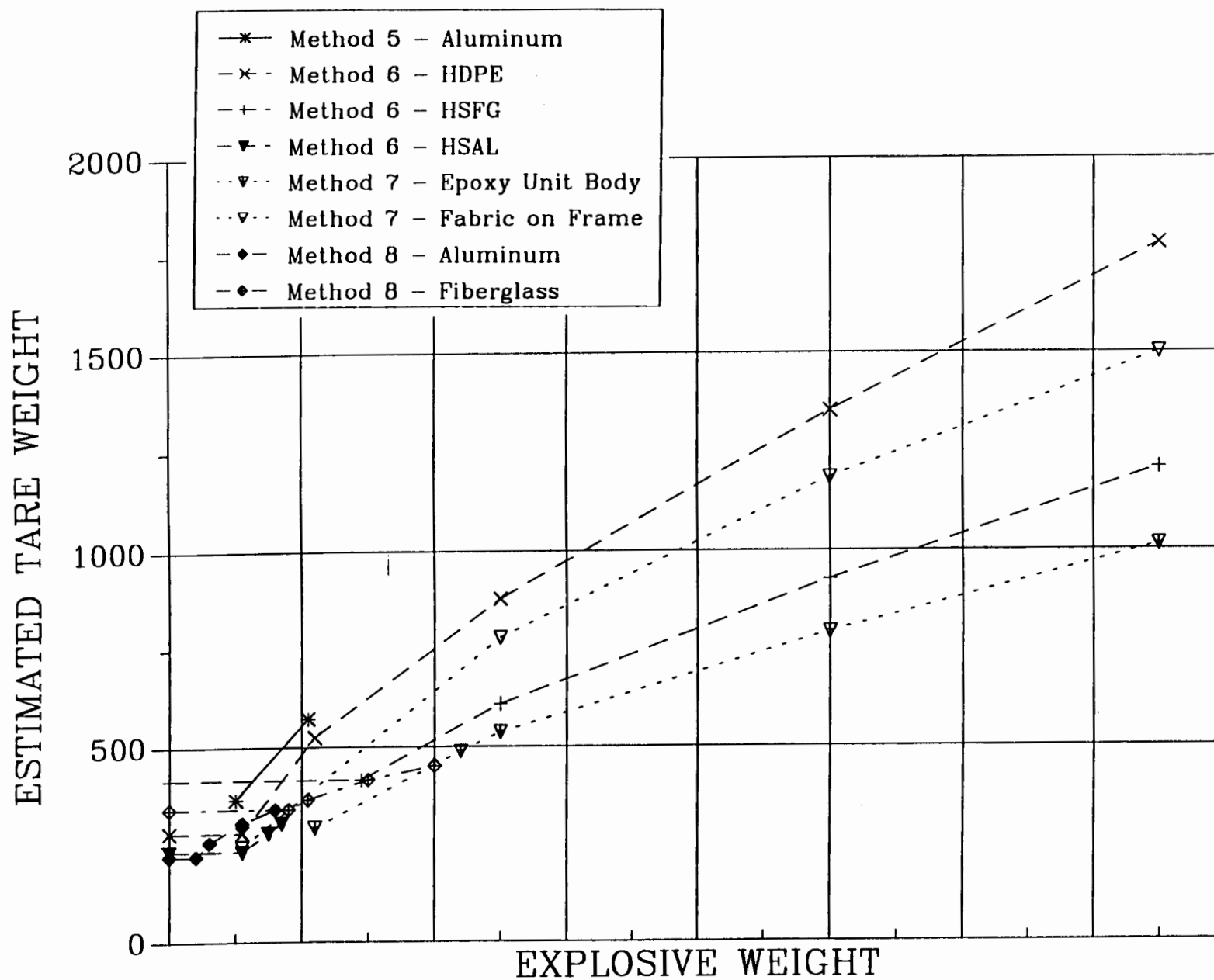
FIGURE 2.2-2 SUMMARY OF HARDENING COUNTERMEASURES 5 - 8
