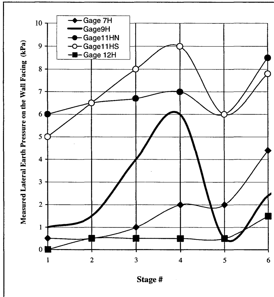
Figure 4.4. Lateral Earth Pressure against the Front Wall Facing of Section 800 Measured by the End of each Construction Stage.
