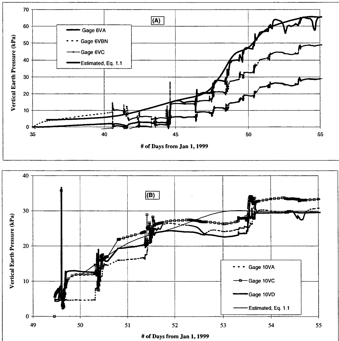
Figure 3.1. Typical Measured and Estimated Vertical Earth Pressure during Placement and Compaction of the Backfill from: (a) Layer 6 Gages, and (b) Layer 10 Gages.
