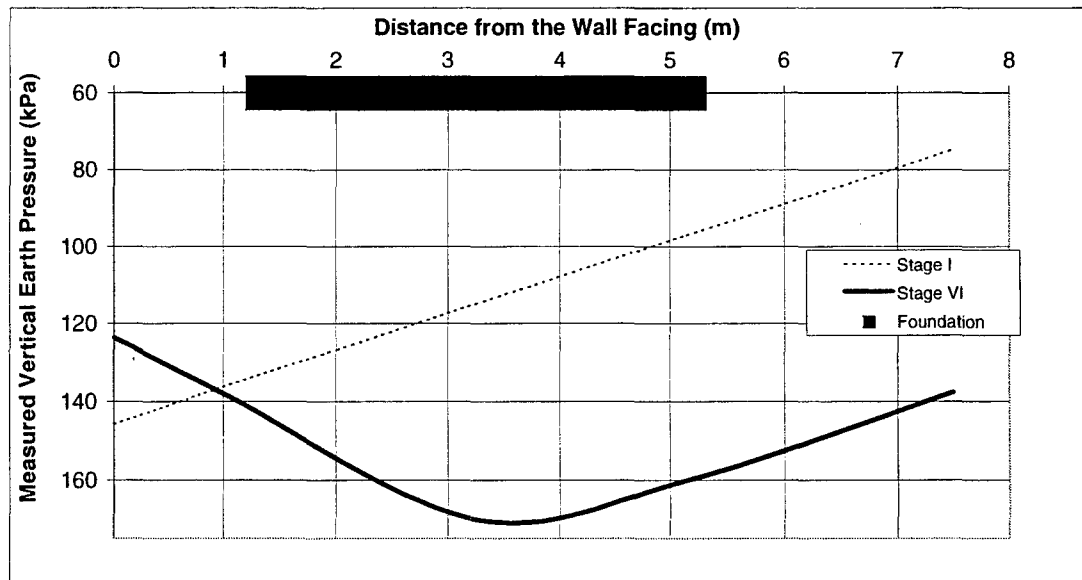
Fig. 3.3. Horizontal Profiles of the Vertical Earth Pressures Measured at the Base of the Reinforced Fill during Construction Stages.
