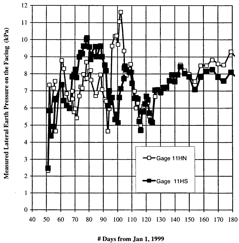
Figure 4.3. Time Records for the Measured Lateral Earth Pressure against the Front Wall Facing of Section 800 during all Construction Stages (from Gages 11 HN and 11HS).
