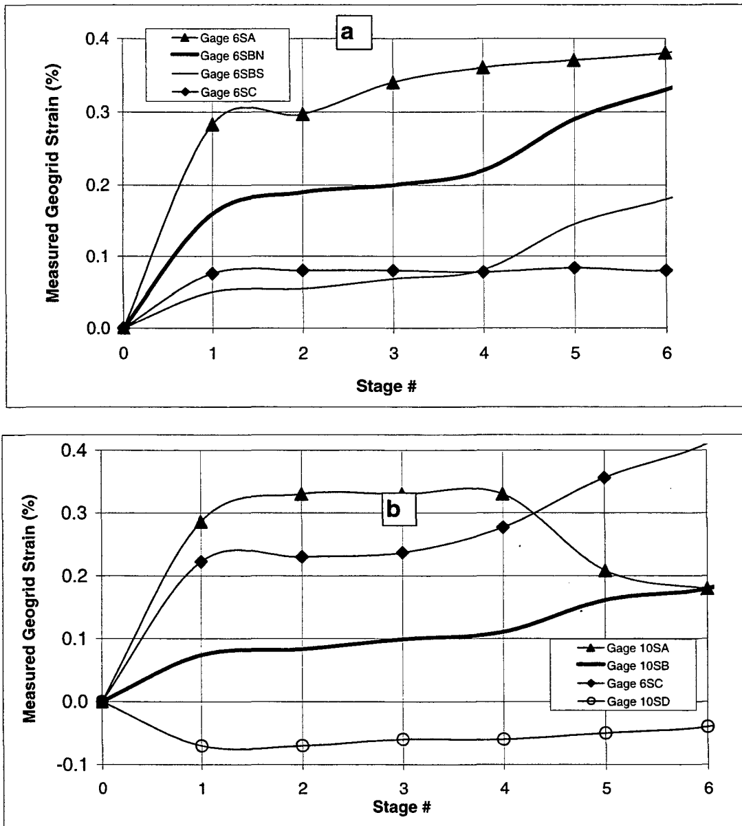
Fig. 5.6. Measured Geogrid Strains at Various Construction Stages along a) Geogrid Layers 6, and b) Geogrid Layer 10.
