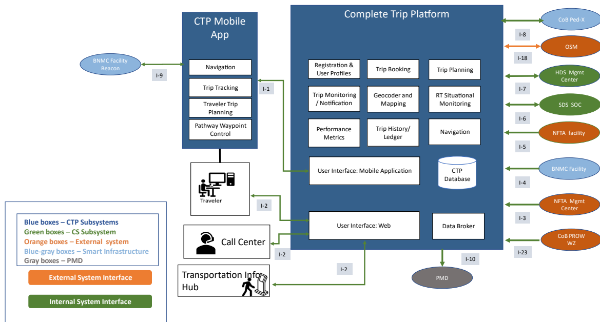
Figure 15. Complete Trip Platform Subsystem
