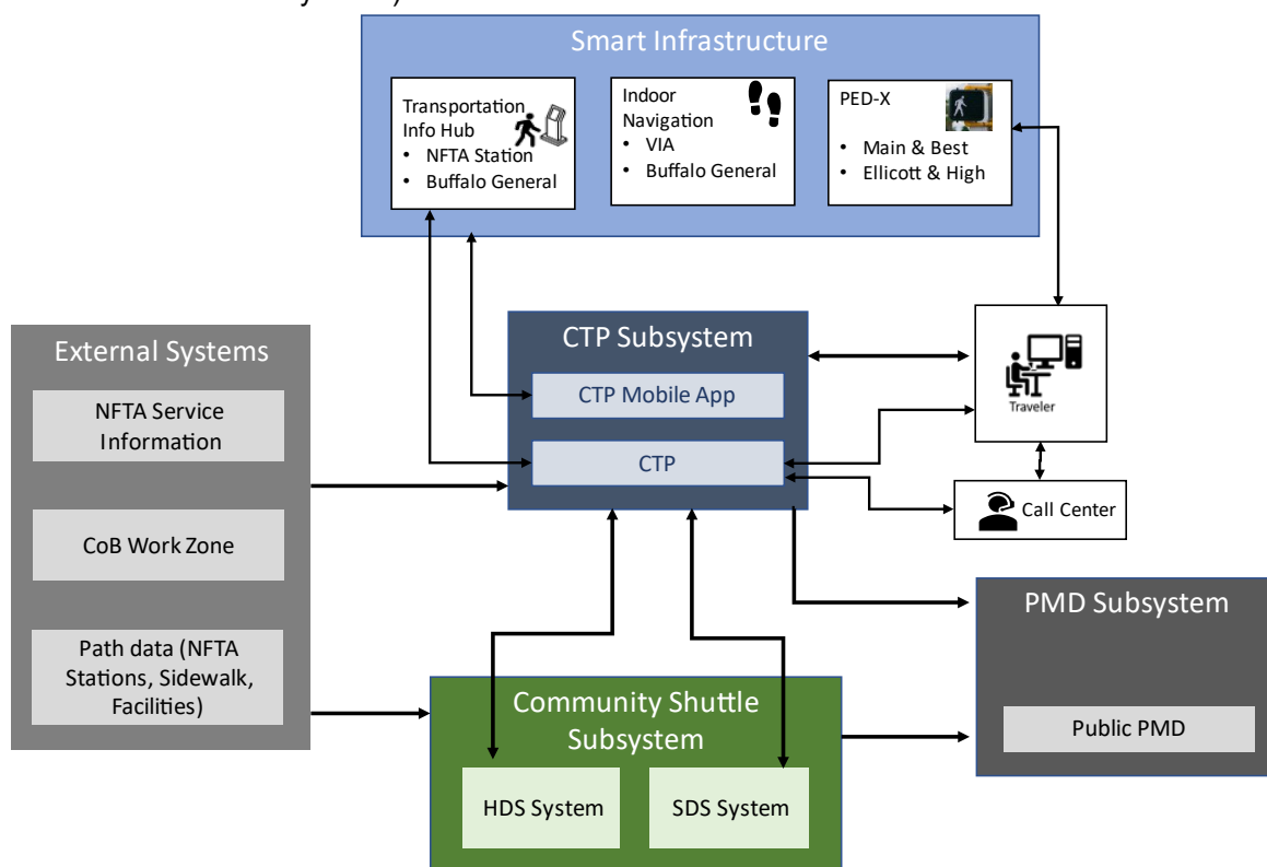
Figure 14. Buffalo, NY ITS4US Deployment Context Diagram with Interfaces.
