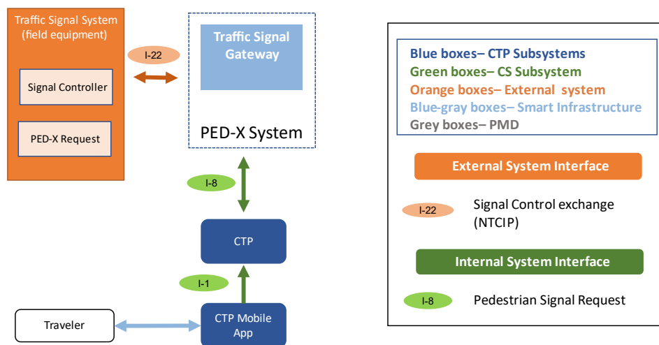
Figure 21. Pedestrian Signal Request (PED-X) Module
