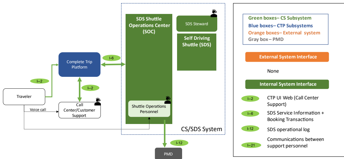
Figure 17. Community Shuttle SDS System
