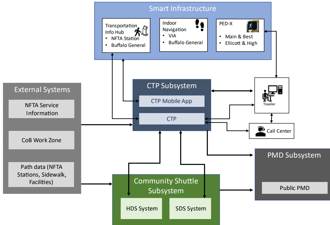
Figure 3. Buffalo Deployment Project Context Diagram
